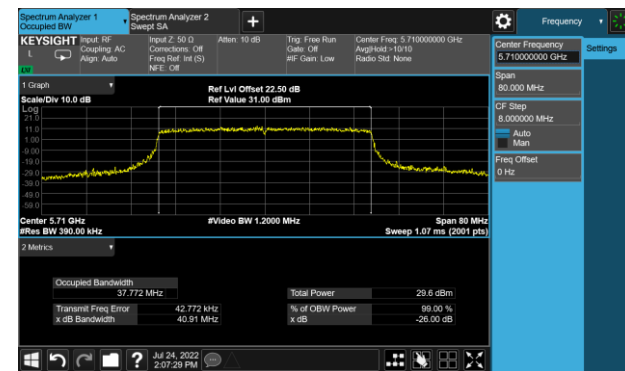
Channel 142(5710MHz)
