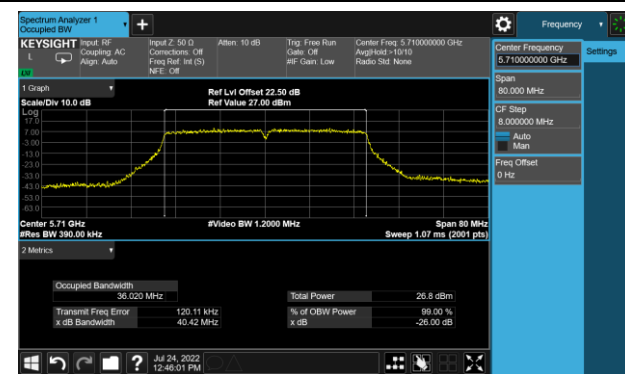
Channel 142(5710MHz)
