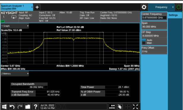
Channel 134 (5670MHz)
