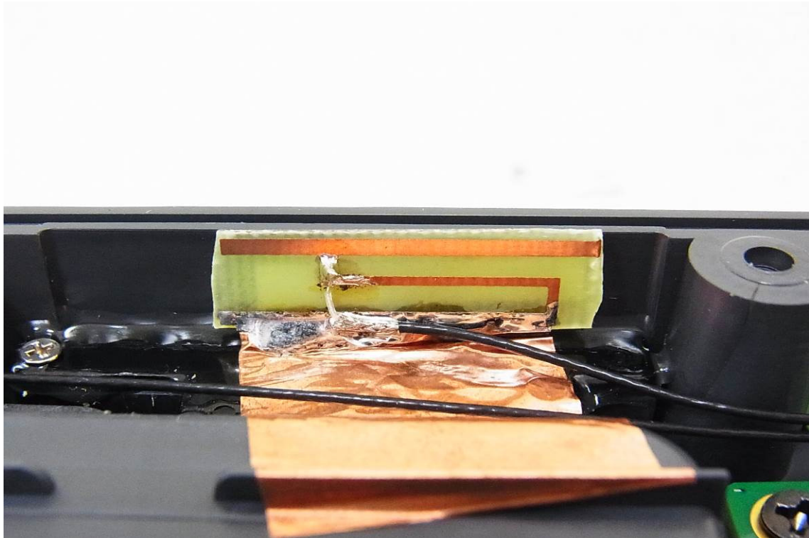
EUT 7 WiFi antenna 1
