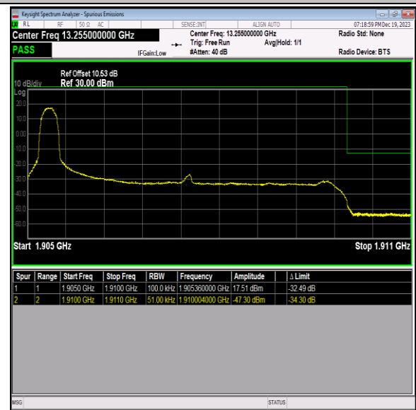
Band2_5MHz_64QAM_19175_1RB#0
