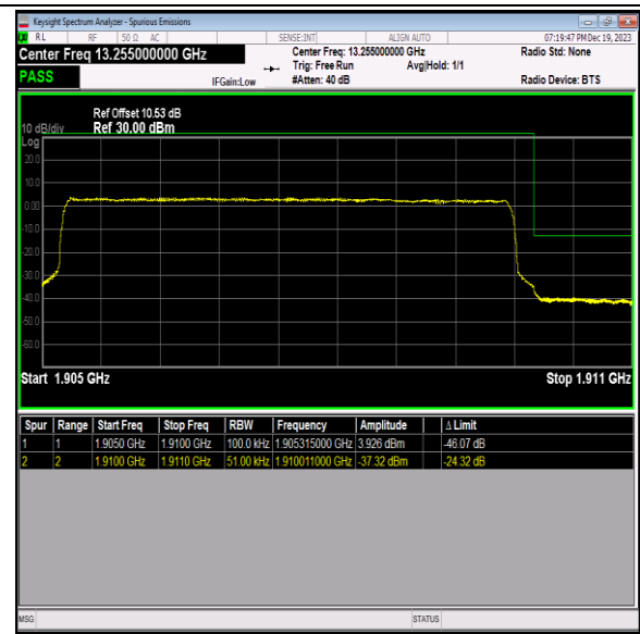
Band2_5MHz_QPSK_19175_25RB#0
