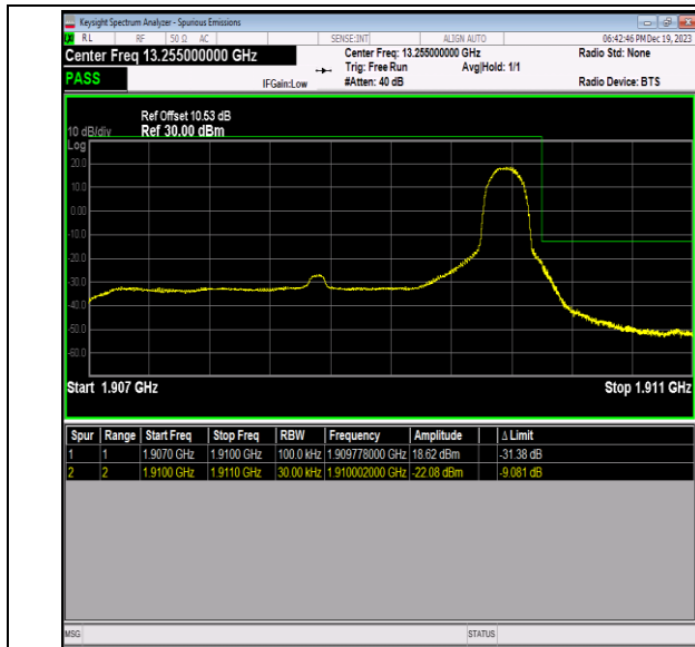
Band2_3MHz_16QAM_19185_1RB#14
