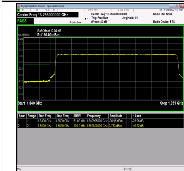
Band2_5MHz_QPSK_18625_25RB#0
