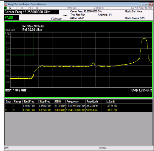
Band2_5MHz_16QAM_18625_1RB#24
