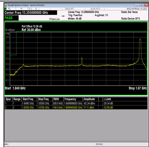
Band2_20MHz_64QAM_18700_1RB#99
