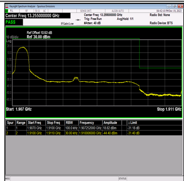
Band2_3MHz_16QAM_19185_1RB#0
