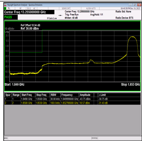
Band2_3MHz_16QAM_18615_1RB#14
