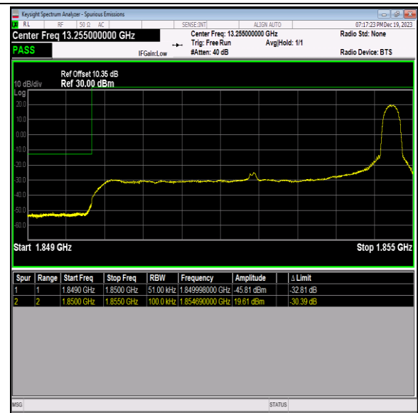
Band2_5MHz_QPSK_18625_1RB#24
