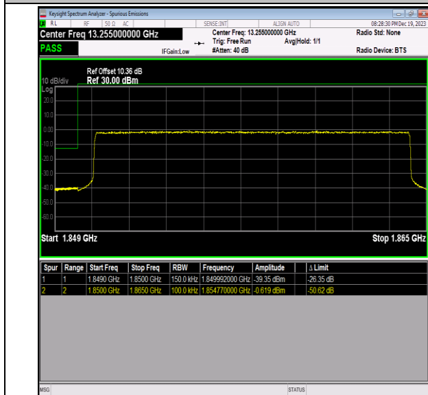
Band2_15MHz_QPSK_18675_75RB#0
