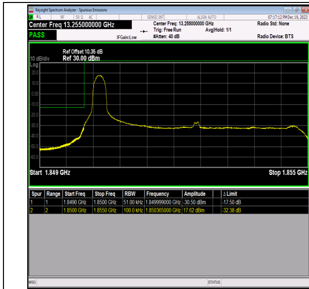
Band2_5MHz_64QAM_18625_1RB#0
