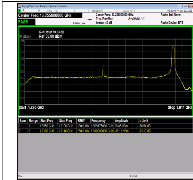
Band2_15MHz_QPSK_19125_1RB#74
