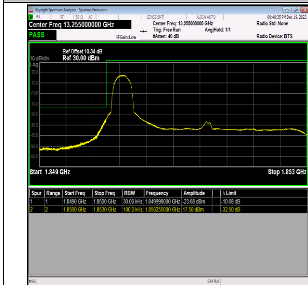
Band2_3MHz_64QAM_18615_1RB#0
