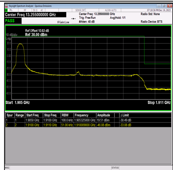
Band2_5MHz_QPSK_19175_1RB#0
