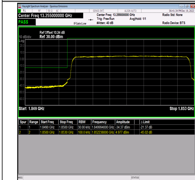
Band2_3MHz_16QAM_18615_15RB#0
