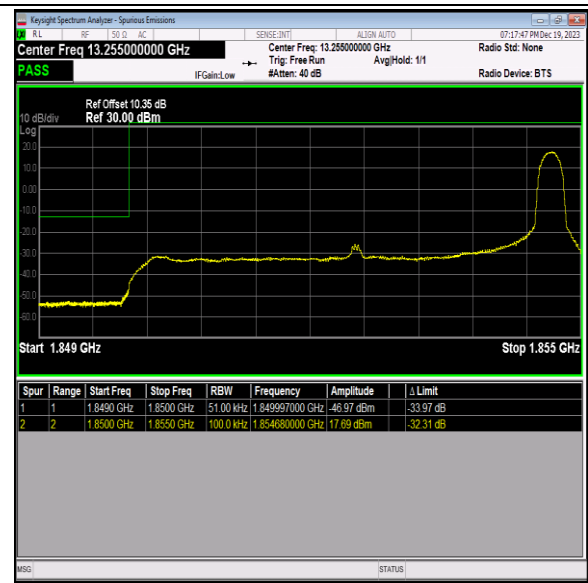
Band2_5MHz_64QAM_18625_1RB#24
