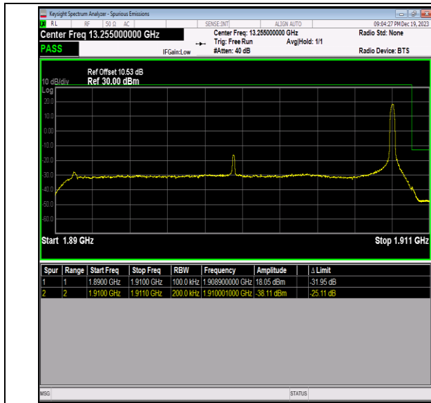
Band2_20MHz_16QAM_19100_1RB#99
