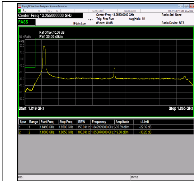
Band2_15MHz_QPSK_18675_1RB#0
