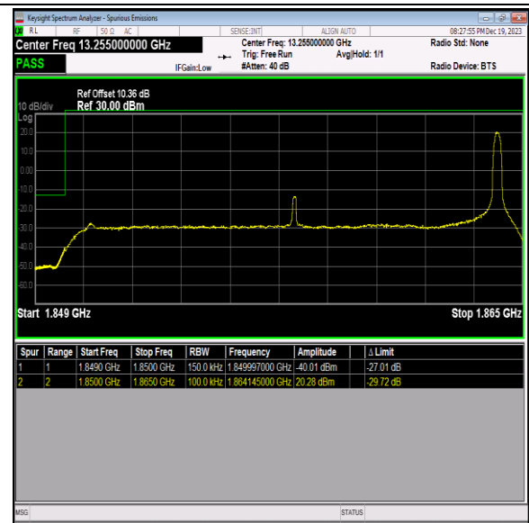
Band2_15MHz_QPSK_18675_1RB#74
