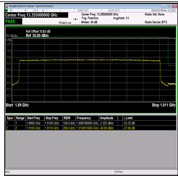
Band2_20MHz_16QAM_19100_100RB#0
