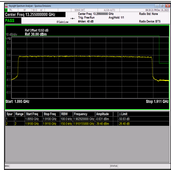
Band2_15MHz_QPSK_19125_75RB#0
