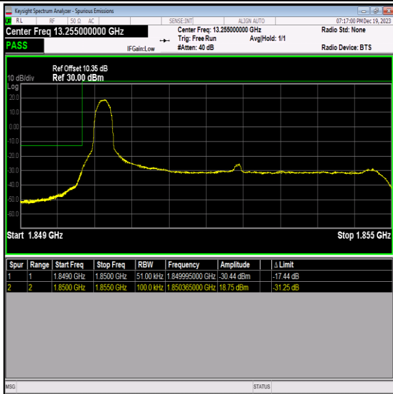
Band2_5MHz_16QAM_18625_1RB#0
