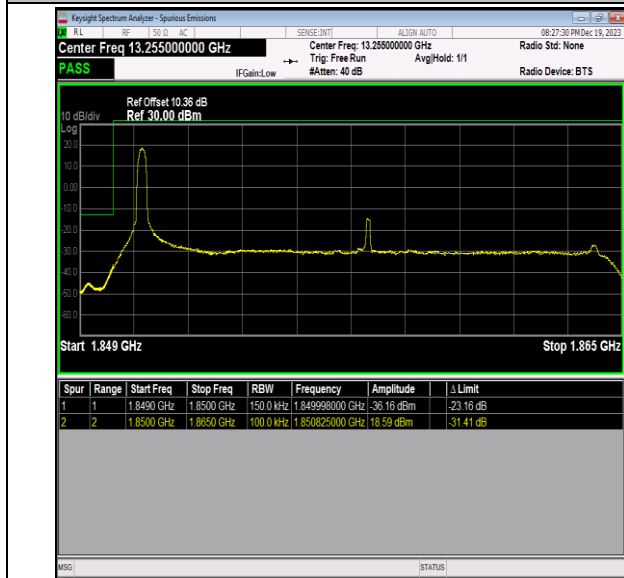
Band2_15MHz_16QAM_18675_1RB#0
