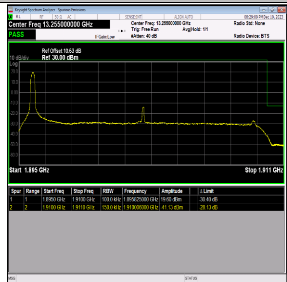
Band2_15MHz_QPSK_19125_1RB#0
