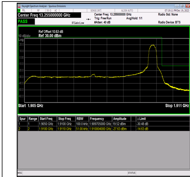
Band2_5MHz_QPSK_19175_1RB#24
