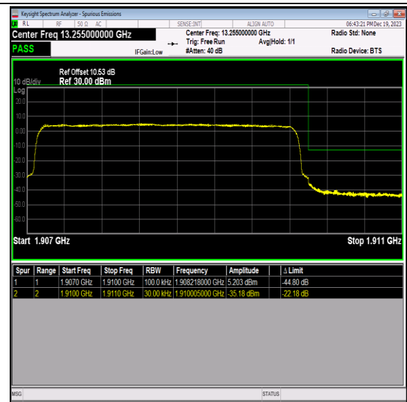
Band2_3MHz_16QAM_19185_15RB#0
