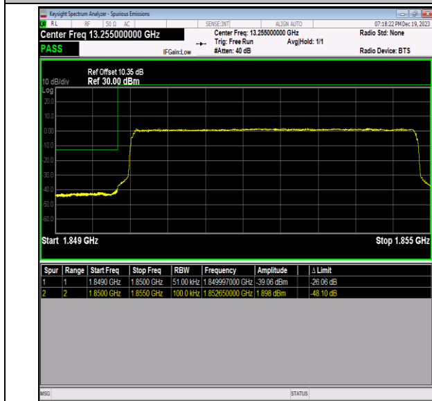
Band2_5MHz_64QAM_18625_25RB#0
