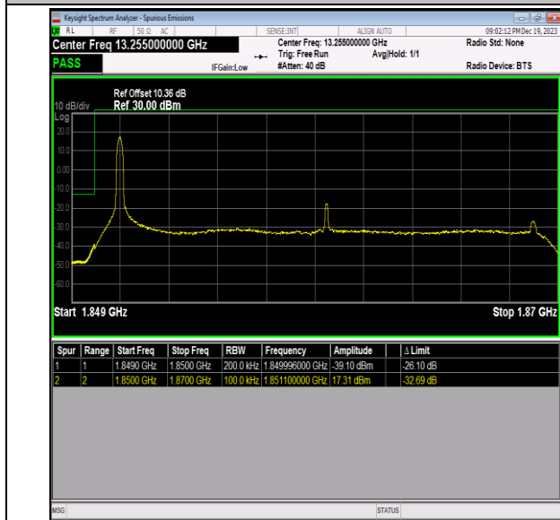
Band2_20MHz_64QAM_18700_1RB#0
