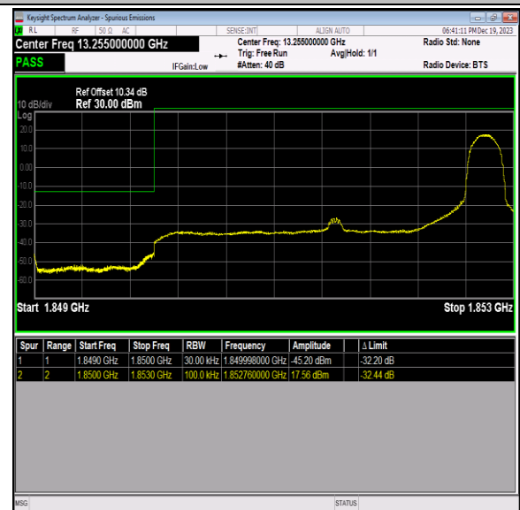
Band2_3MHz_64QAM_18615_1RB#14
