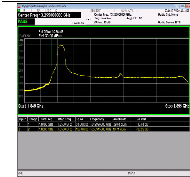
Band2_5MHz_QPSK_18625_1RB#0
