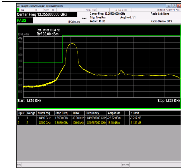
Band2_3MHz_16QAM_18615_1RB#0
