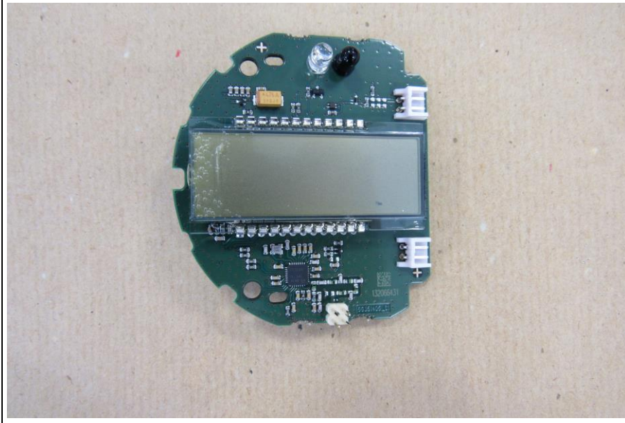
EUT PCB II front
