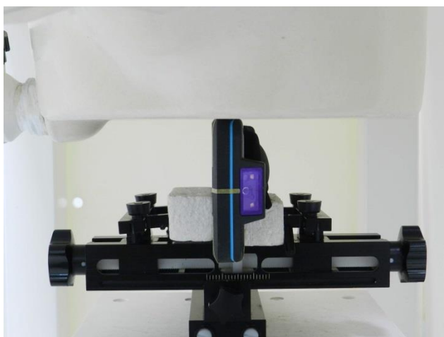
Left Side with Handstrap, Test Separation 0 mm
