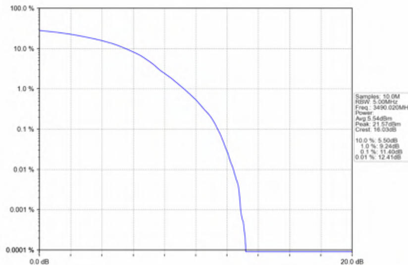
n78e_30kHz_SISO_NTNV_80MHz_DFT-s-OFDM 64 QAM_3490.02MHz_Outer_Full
