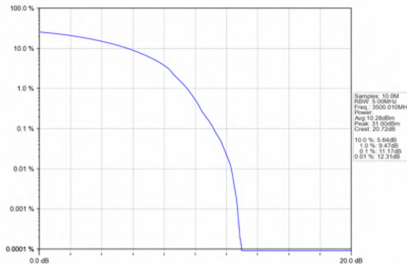
n78e_30kHz_SISO_NTNV_30MHz_DFT-s-OFDM_16_QAM_3500.01MHz_Outer_Full
