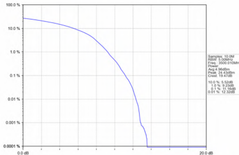
n78e_30kHz_SISO_NTNV_100MHz_DFT-s-OFDM 64 QAM_3500.01MHz_Outer_Full
