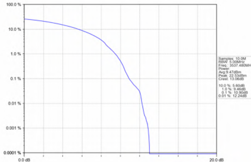
n78e_30kHz_SISO_NTNV_25MHz_DFT-s-OFDM_256_QAM_3537.48MHz_Outer_Full
