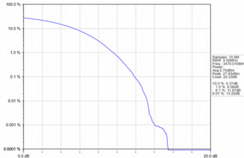
n78e_30kHz_SISO_NTNV_40MHz_CP-OFDM_256_QAM_3470.01MHz_Outer_Full
