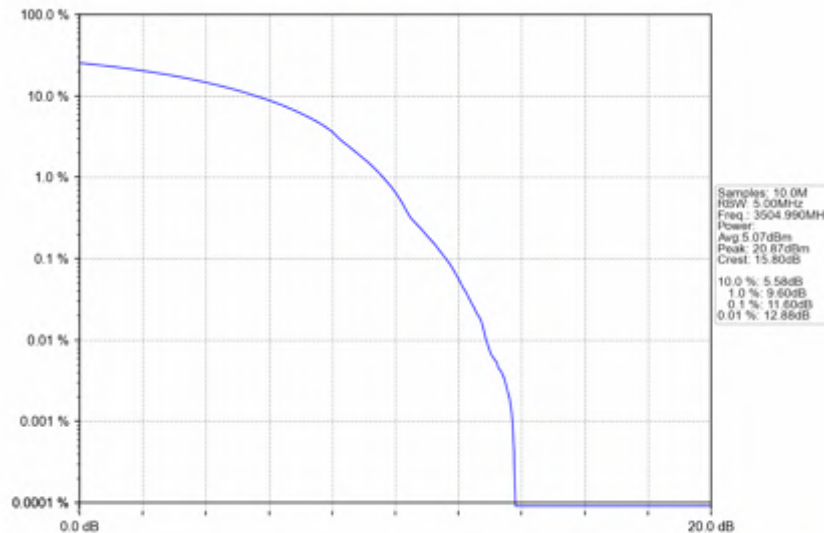
n78e_30kHz_SISO_NTNV_90MHz_DFT-s-OFDM_QPSK_3504.99MHz_Outer_Full
