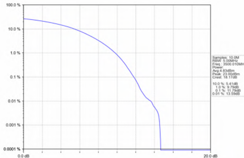
n78e_30kHz_SISO_NTNV_90MHz_CP-OFDM QPSK_3500.01MHz_Outer_Full
