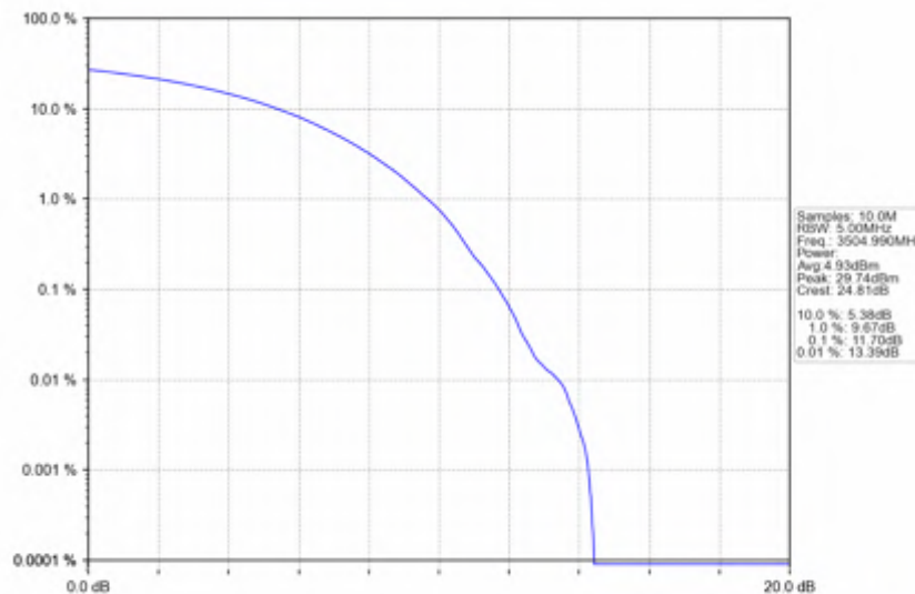
n78e_30kHz_SISO_NTNV_90MHz_CP-OFDM QPSK_3504.99MHz_Outer_Full
