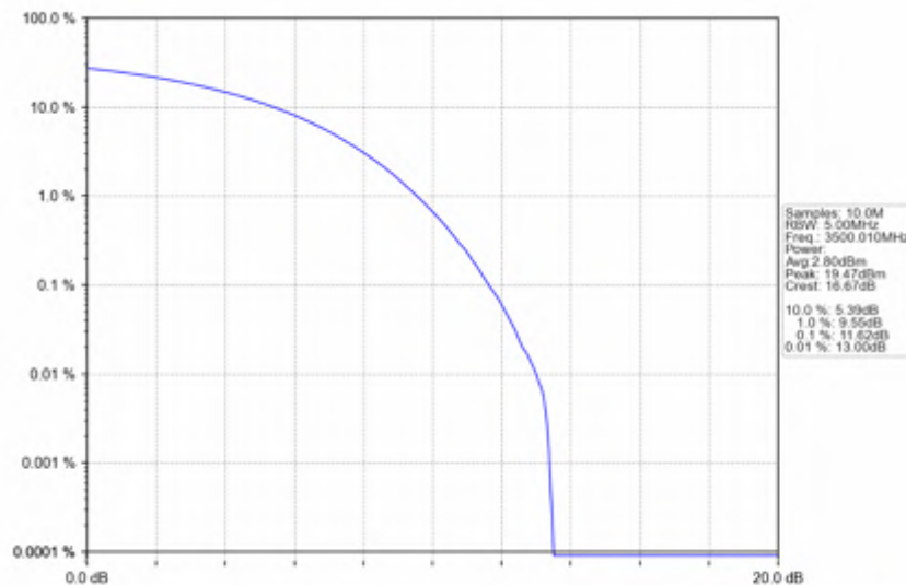
n78e_30kHz_SISO_NTNV_70MHz_CP-OFDM_256_QAM_3500.01MHz_Outer_Full
