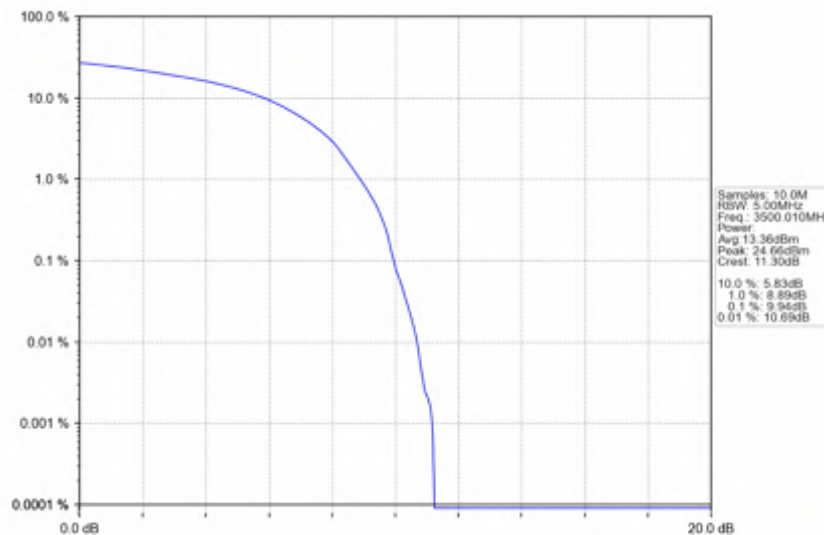
n78e_30kHz_SISO_NTNV_15MHz_DFT-s-OFDM_QPSK_3500.01MHz_Outer_Full
