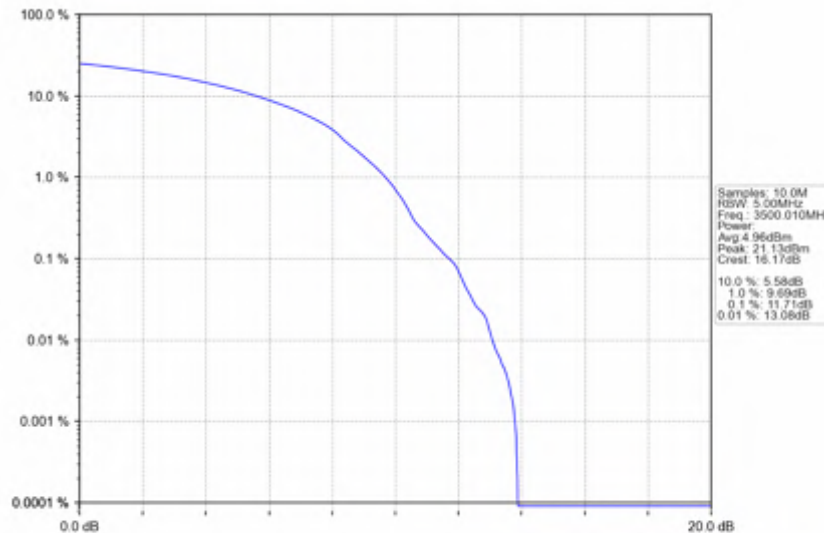
n78e_30kHz_SISO_NTNV_90MHz_DFT-s-OFDM_QPSK_3500.01MHz_Outer_Full
