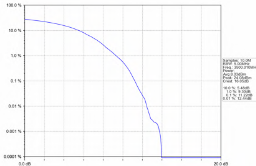
n78e_30kHz_SISO_NTV_50MHz_DFT-s-OFDM 64 QAM_3500.01MHz_Outer_Full
