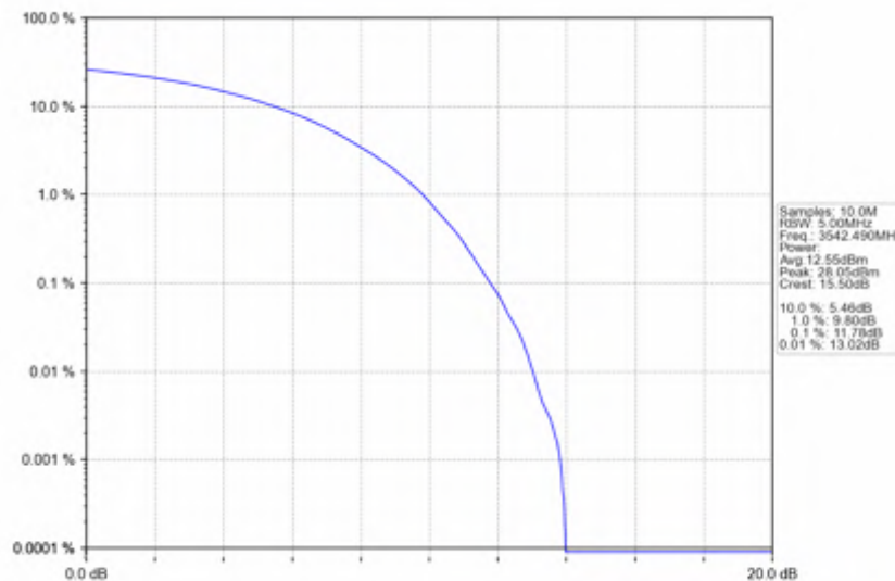
n78e_30kHz_SISO_NTNV_15MHz_CP-OFDM 64 QAM_3542.49MHz_Outer_Full
