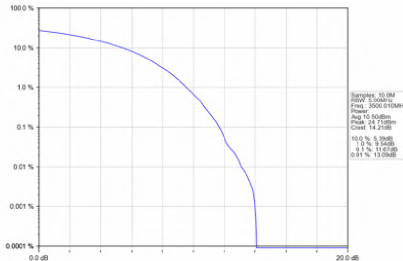
n78e_30kHz_SISO_NTNV_25MHz_CP-OFDM 64 QAM_3500.01MHz_Outer_Full
