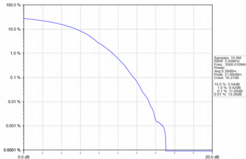
n78e_30kHz_SISO_NTNV_80MHz_DFT-s-OFDM_QPSK_3500.01MHz_Outer_Full
