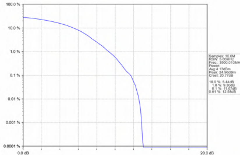
n78e_30kHz_SISO_NTNV_80MHz_DFT-s-OFDM_256_QAM_3500.01MHz_Outer_Full
