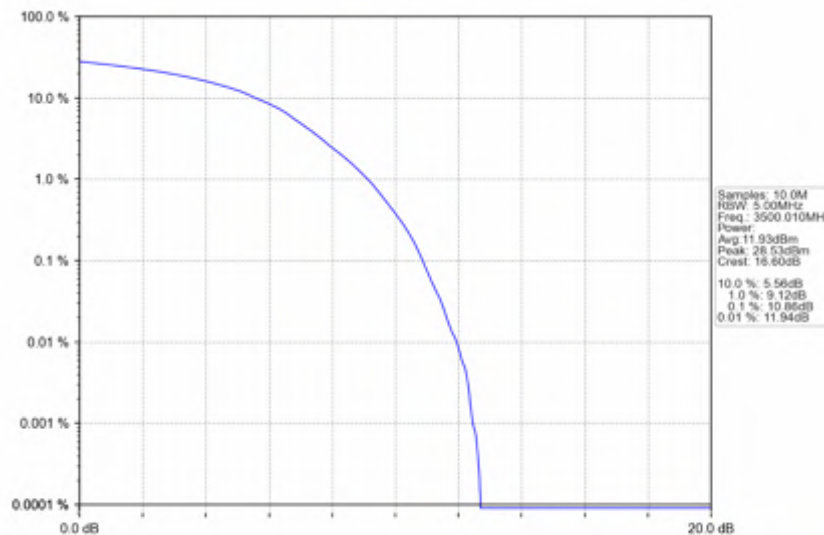
n78e_30kHz_SISO_NTV_20MHz_DFT-s-OFDM 64 QAM_3500.01MHz_Outer_Full
