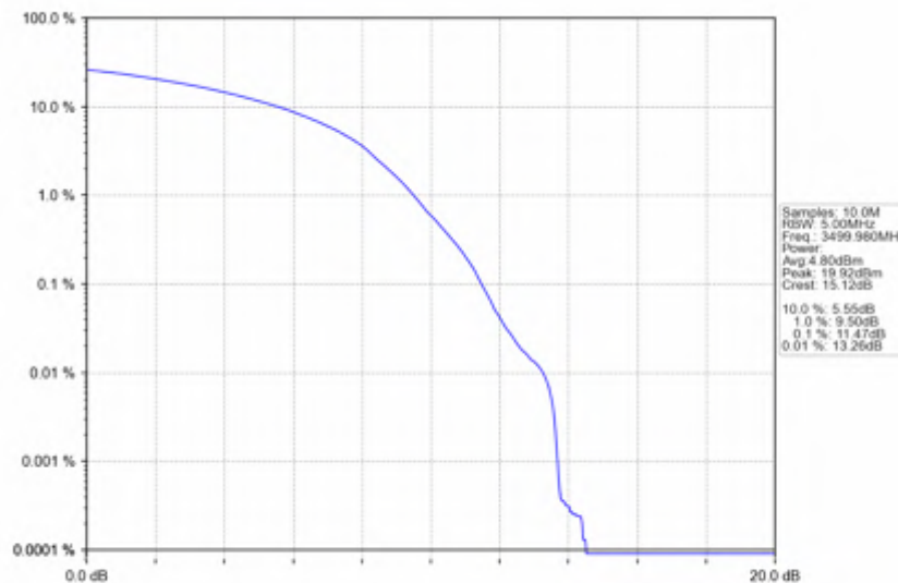
n78e_30kHz_SISO_NTNV_100MHz_DFT-s-OFDM 64 QAM_3499.98MHz_Outer_Full
