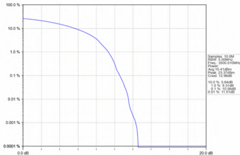
n78e_30kHz_SISO_NTNV_30MHz_DFT-s-OFDM_QPSK_3500.01MHz_Outer_Full
