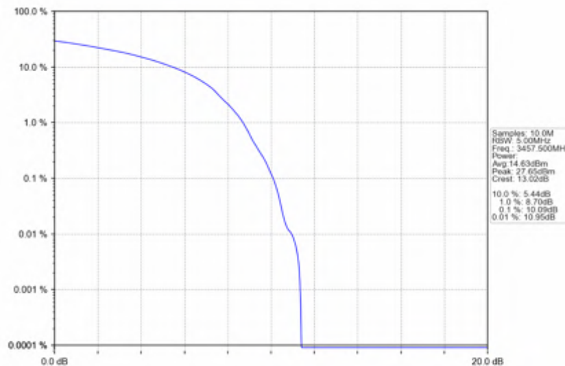
n78e_30kHz_SISO_NTNV_15MHz_DFT-s-OFDM_16_QAM_3457.5MHz_Outer_Full
