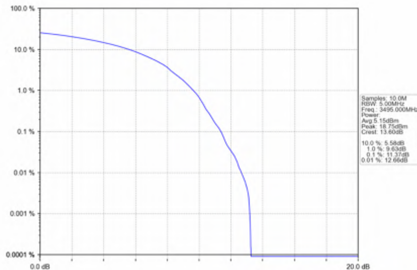
n78e_30kHz_SISO_NTNV_90MHz_DFT-s-OFDM 64 QAM_3495MHz_Outer_Full
