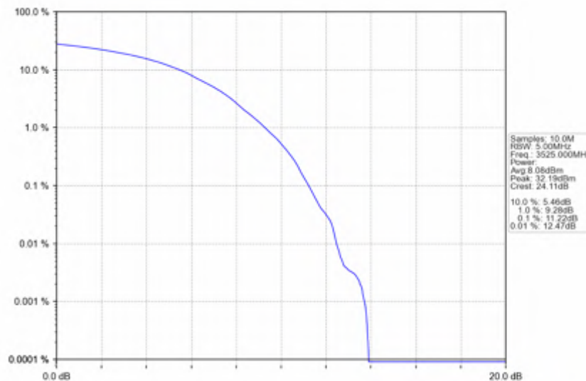
n78e_30kHz_SISO_NTV_50MHz_DFT-s-OFDM 64 QAM_3525MHz_Outer_Full
