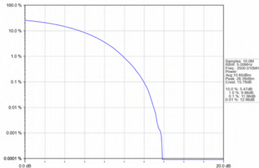
n78e_30kHz_SISO_NTNV_25MHz_CP-OFDM_16_QAM_3500.01MHz_Outer_Full
