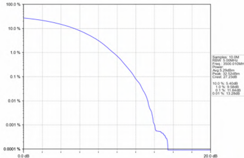
n78e_30kHz_SISO_NTNV_40MHz_CP-OFDM_256_QAM_3500.01MHz_Outer_Full
