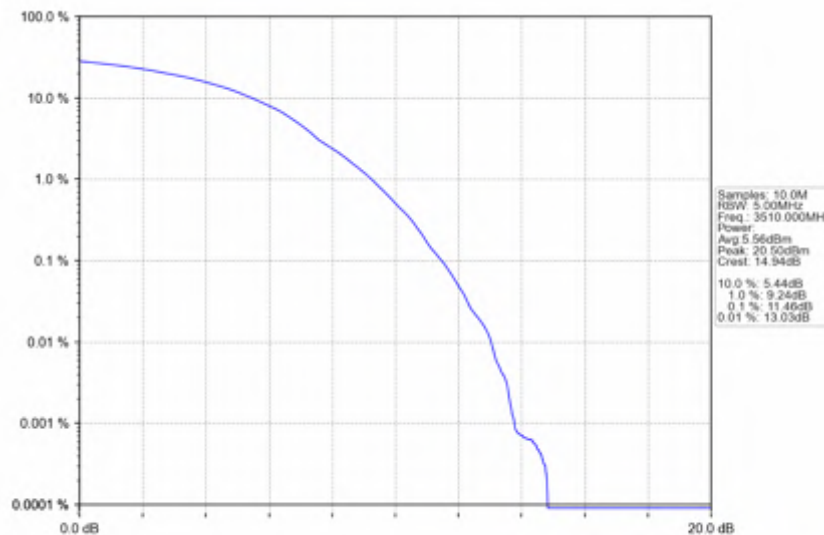
n78e_30kHz_SISO_NTNV_80MHz_DFT-s-OFDM_QPSK_3510MHz_Outer_Full
