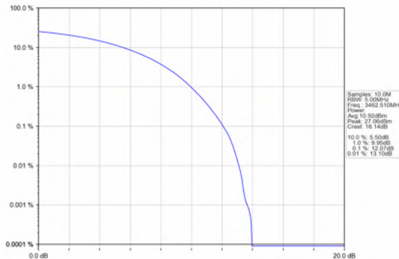
n78e_30kHz_SISO_NTNV_25MHz_CP-OFDM_16_QAM_3462.51MHz_Outer_Full
