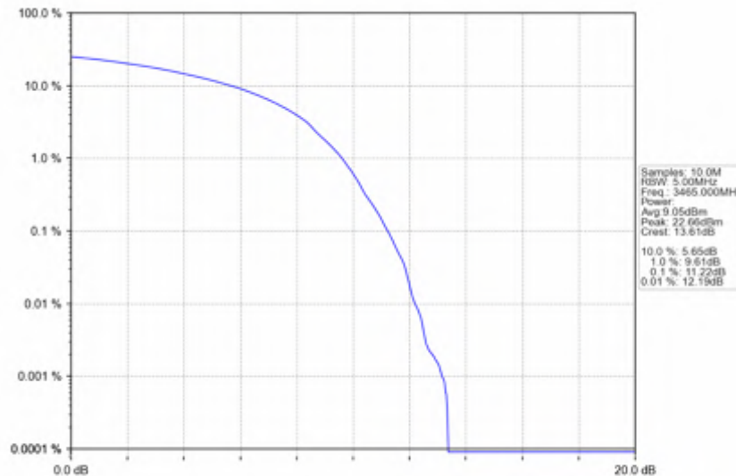
n78e_30kHz_SISO_NTNV_30MHz_DFT-s-OFDM_256_QAM_3465MHz_Outer_Full
