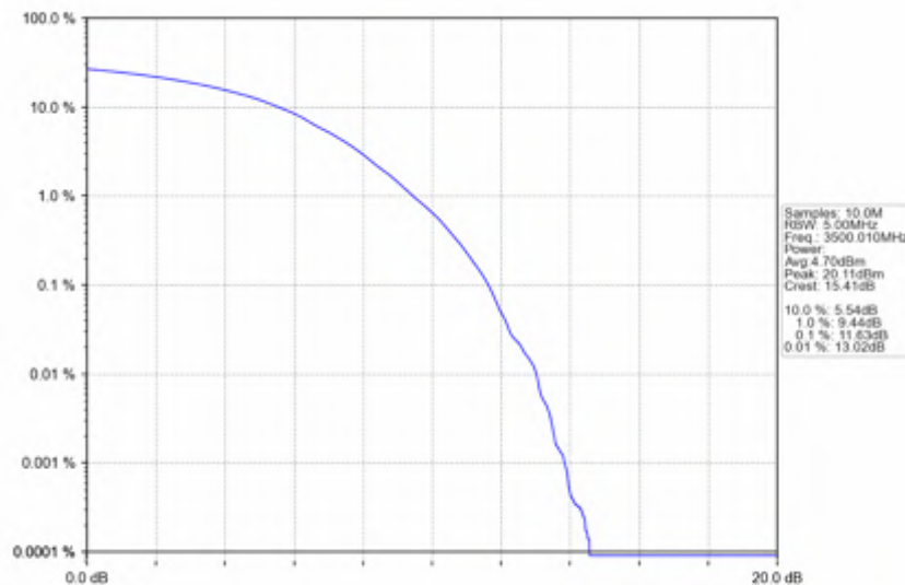
n78e_30kHz_SISO_NTNV_70MHz_DFT-s-OFDM_256_QAM_3500.01MHz_Outer_Full
