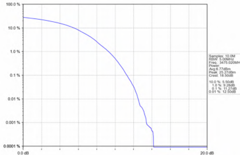
n78e_30kHz_SISO_NTNV_50MHz_DFT-s-OFDM_256_QAM_3475.02MHz_Outer_Full
