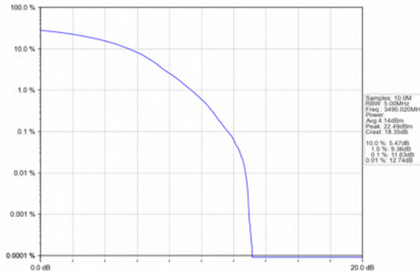
n78e_30kHz_SISO_NTNV_80MHz_DFT-s-OFDM_256_QAM_3490.02MHz_Outer_Full
