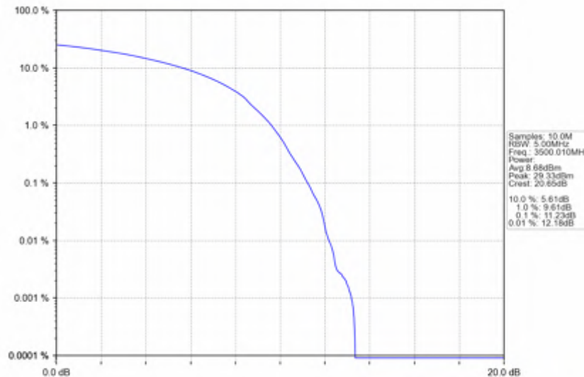
n78e_30kHz_SISO_NTNV_30MHz_DFT-s-OFDM_256_QAM_3500.01MHz_Outer_Full
