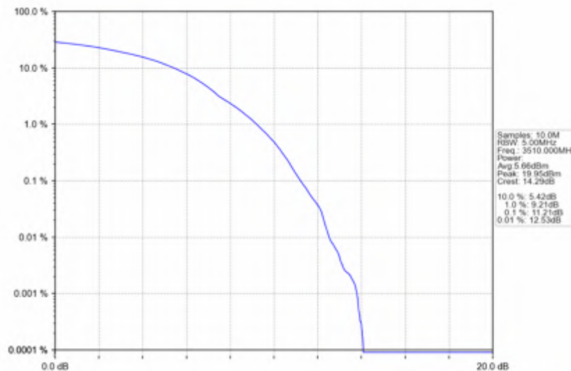
n78e_30kHz_SISO_NTNV_80MHz_DFT-s-OFDM 16 QAM_3510MHz_Outer_Full
