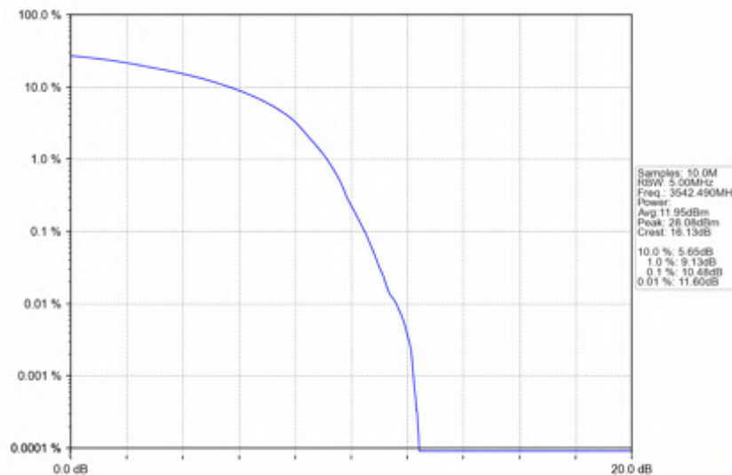
n78e_30kHz_SISO_NTNV_15MHz_DFT-s-OFDM_256_QAM_3542.49MHz_Outer_Full
