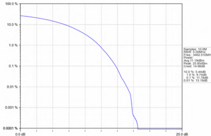
n78e_30kHz_SISO_NTNV_25MHz_CP-OFDM_QPSK_3462.51MHz_Outer_Full
