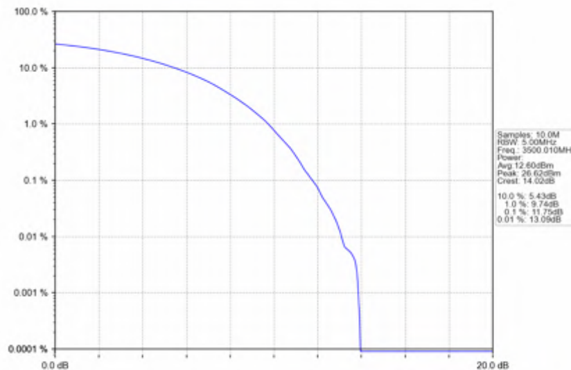
n78e_30kHz_SISO_NTNV_15MHz_CP-OFDM 64 QAM_3500.01MHz_Outer_Full
