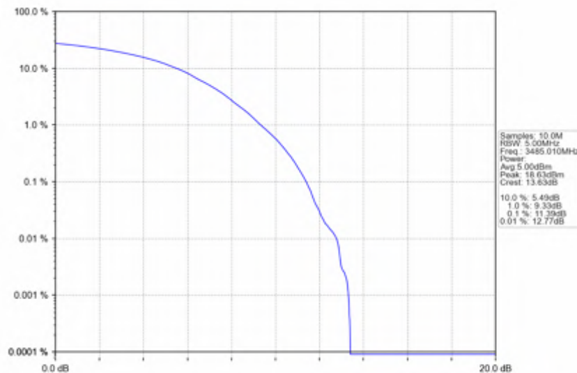
n78e_30kHz_SISO_NTNV_70MHz_DFT-s-OFDM_256_QAM_3485.01MHz_Outer_Full
