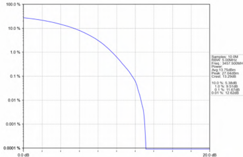
n78e_30kHz_SISO_NTNV_15MHz_CP-OFDM_16_QAM_3457.5MHz_Outer_Full
