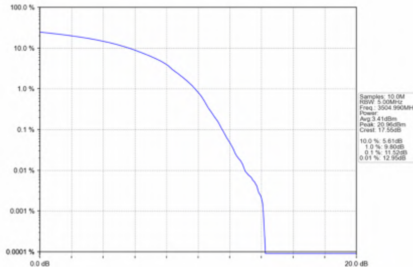
n78e_30kHz_SISO_NTNV_90MHz_DFT-s-OFDM_256_QAM_3504.99MHz_Outer_Full
