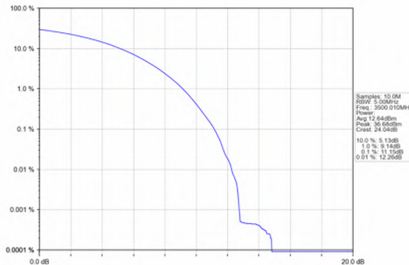
n78e_30kHz_SISO_NTNV_20MHz_CP-OFDM QPSK_3500.01MHz_Outer_Full
