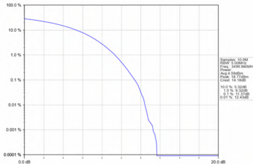
n78e_30kHz_SISO_NTNV_100MHz_CP-OFDM 64 QAM_3499.98MHz_Outer_Full
