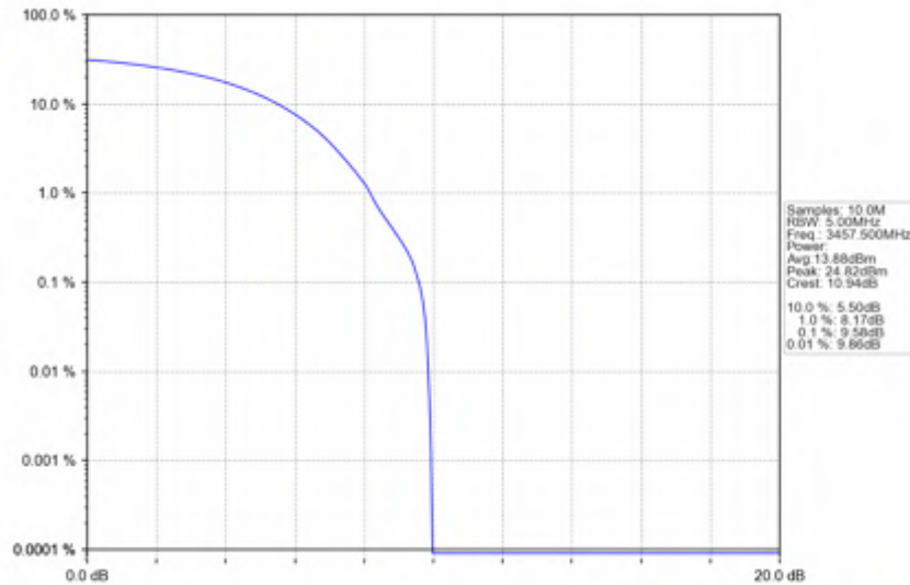
n78e_30kHz_SISO_NTNV_15MHz_DFT-s-OFDM_PI/2_BPSK_3457.5MHz_Outer_Full
