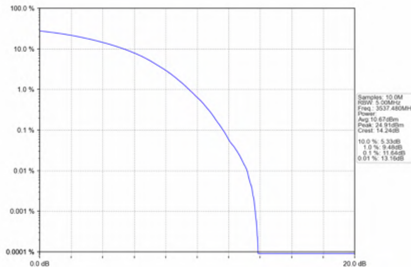
n78e_30kHz_SISO_NTNV_25MHz_CP-OFDM 64 QAM_3537.48MHz_Outer_Full
