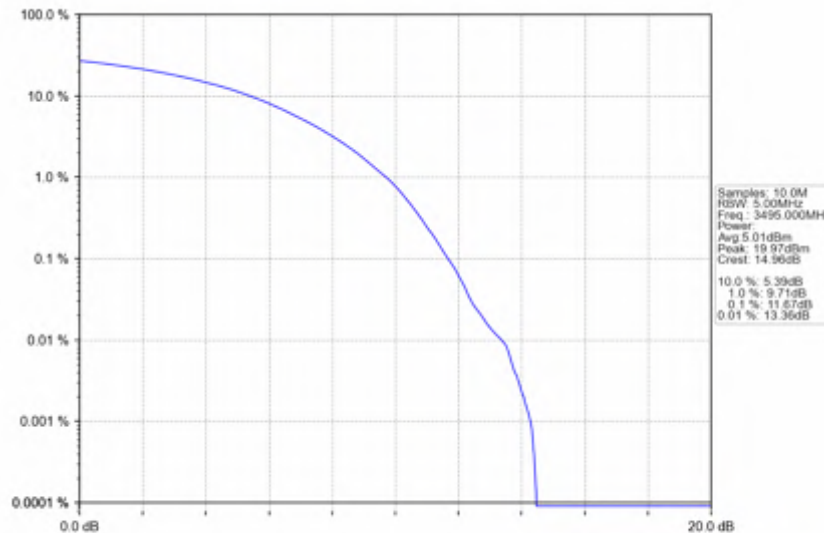
n78e_30kHz_SISO_NTNV_90MHz_CP-OFDM_QPSK_3495MHz_Outer_Full
