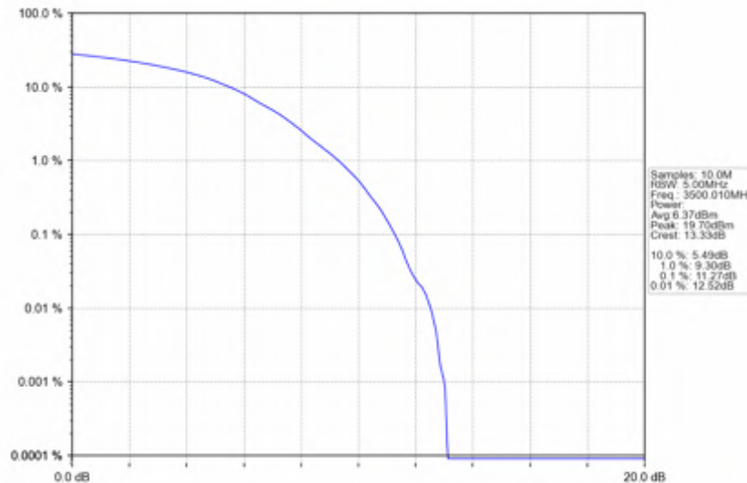
n78e_30kHz_SISO_NTNV_70MHz_DFT-s-OFDM_QPSK_3500.01MHz_Outer_Full
