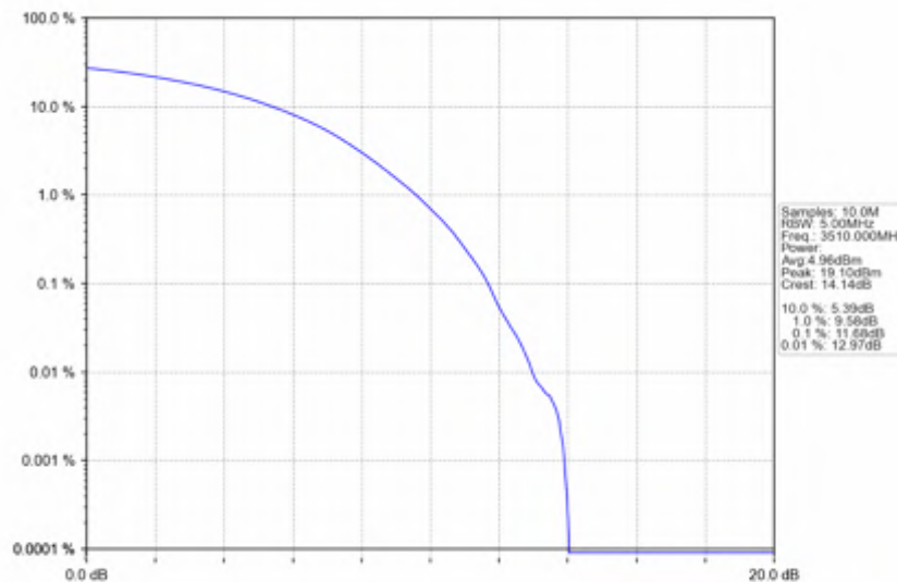
n78e_30kHz_SISO_NTNV_80MHz_CP-OFDM 64 QAM_3510MHz_Outer_Full
