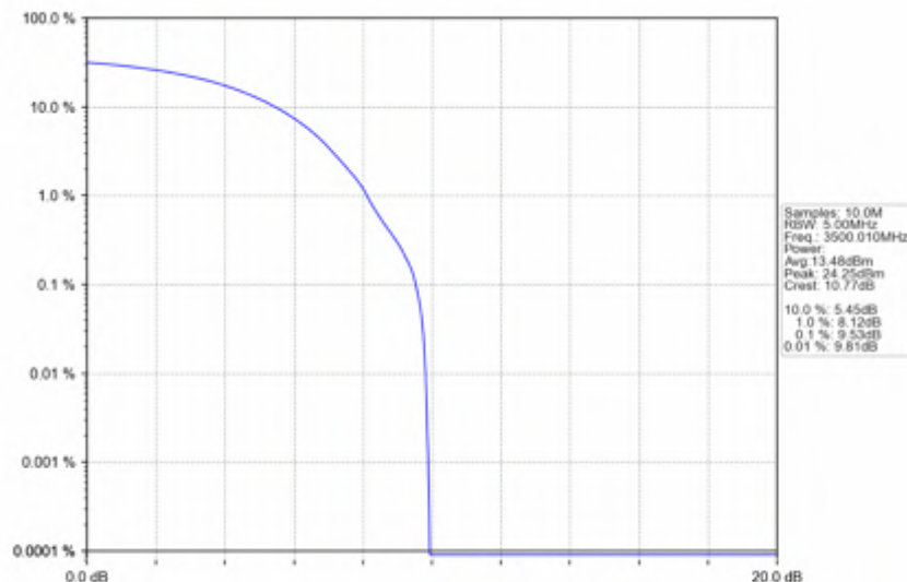
n78e_30kHz_SISO_NTNV_15MHz_DFT-s-OFDM_PI/2_BPSK_3500.01MHz_Outer_Full
