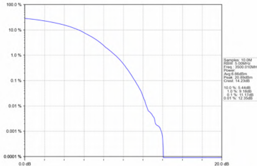
n78e_30kHz_SISO_NTNV_50MHz_DFT-s-OFDM_256_QAM_3500.01MHz_Outer_Full
