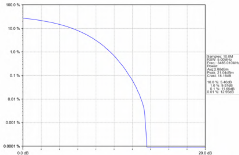
n78e_30kHz_SISO_NTNV_70MHz_CP-OFDM_256_QAM_3485.01MHz_Outer_Full
