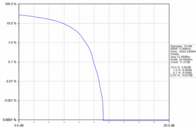
n78e_30kHz_SISO_NTNV_15MHz_DFT-s-OFDM_QPSK_3542.49MHz_Outer_Full
