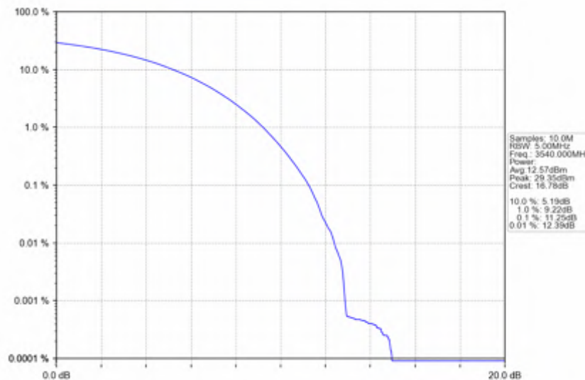
n78e_30kHz_SISO_NTNV_20MHz_CP-OFDM QPSK_3540MHz_Outer_Full
