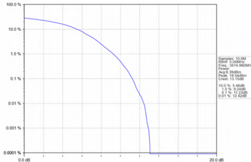
n78e_30kHz_SISO_NTNV_70MHz_DFT-s-OFDM_QPSK_3514.98MHz_Outer_Full
