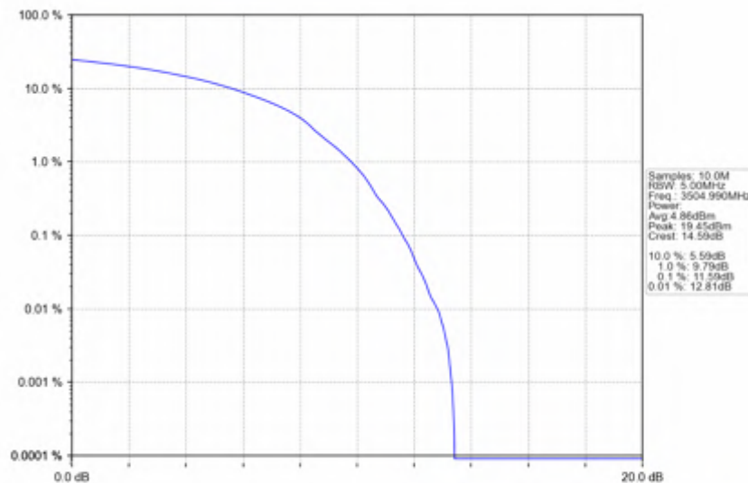
n78e_30kHz_SISO_NTNV_90MHz_DFT-s-OFDM 16 QAM_3504.99MHz_Outer_Full
