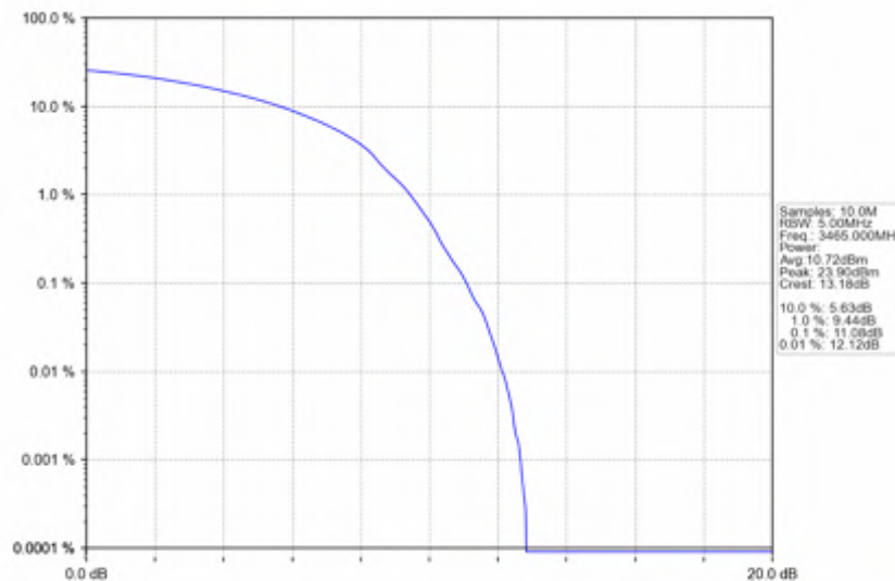
n78e_30kHz_SISO_NTNV_30MHz_DFT-s-OFDM_16_QAM_3465MHz_Outer_Full
