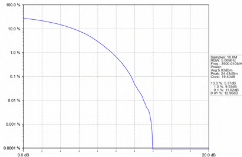
n78e_30kHz_SISO_NTNV_80MHz_CP-OFDM 64 QAM_3500.01MHz_Outer_Full
