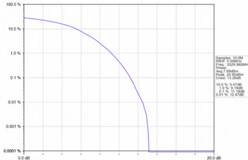
n78e_30kHz_SISO_NTNV_40MHz_DFT-s-OFDM_256_QAM_3529.98MHz_Outer_Full
