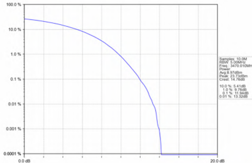
n78e_30kHz_SISO_NTNV_40MHz_CP-OFDM_QPSK_3470.01MHz_Outer_Full
