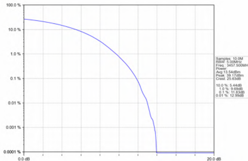
n78e_30kHz_SISO_NTNV_15MHz_CP-OFDM_QPSK_3457.5MHz_Outer_Full
