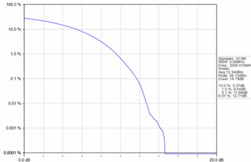
n78e_30kHz_SISO_NTNV_15MHz_CP-OFDM_16_QAM_3500.01MHz_Outer_Full
