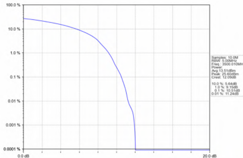
n78e_30kHz_SISO_NTNV_15MHz_DFT-s-OFDM_16_QAM_3500.01MHz_Outer_Full
