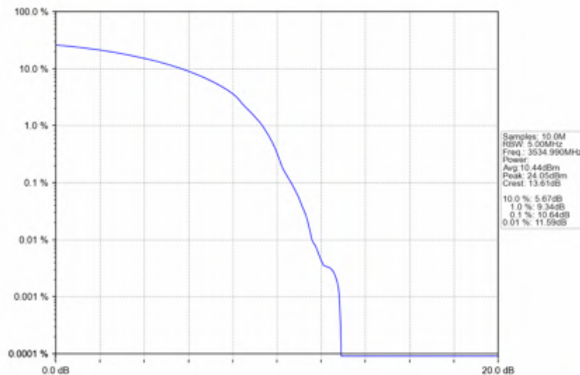
n78e_30kHz_SISO_NTNV_30MHz_DFT-s-OFDM_QPSK_3534.99MHz_Outer_Full
