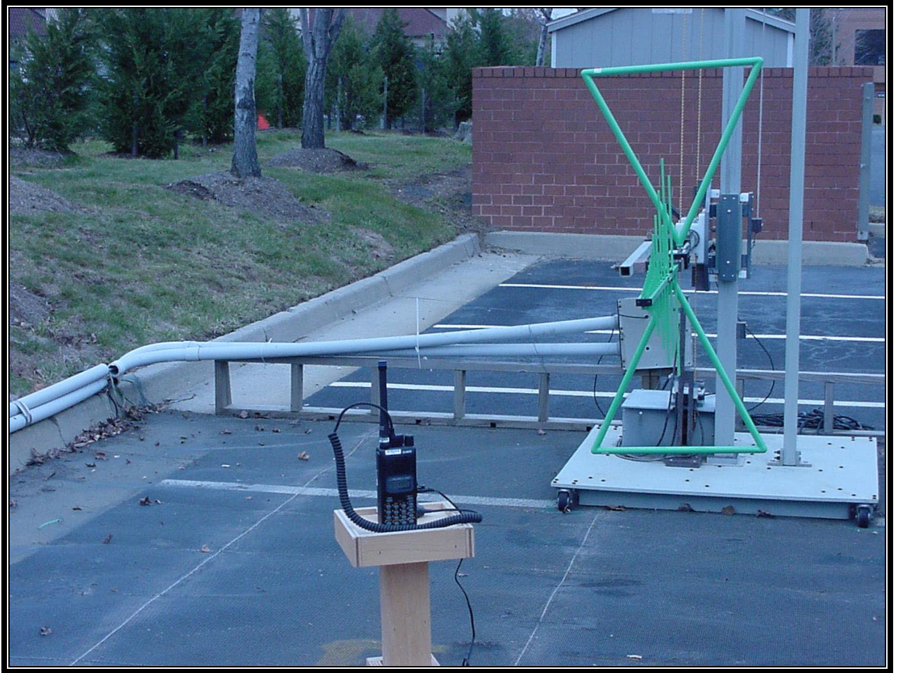
PHOTOGRAPH 4: RADIATED TEST CONFIGURATION (FRONT VIEW)
