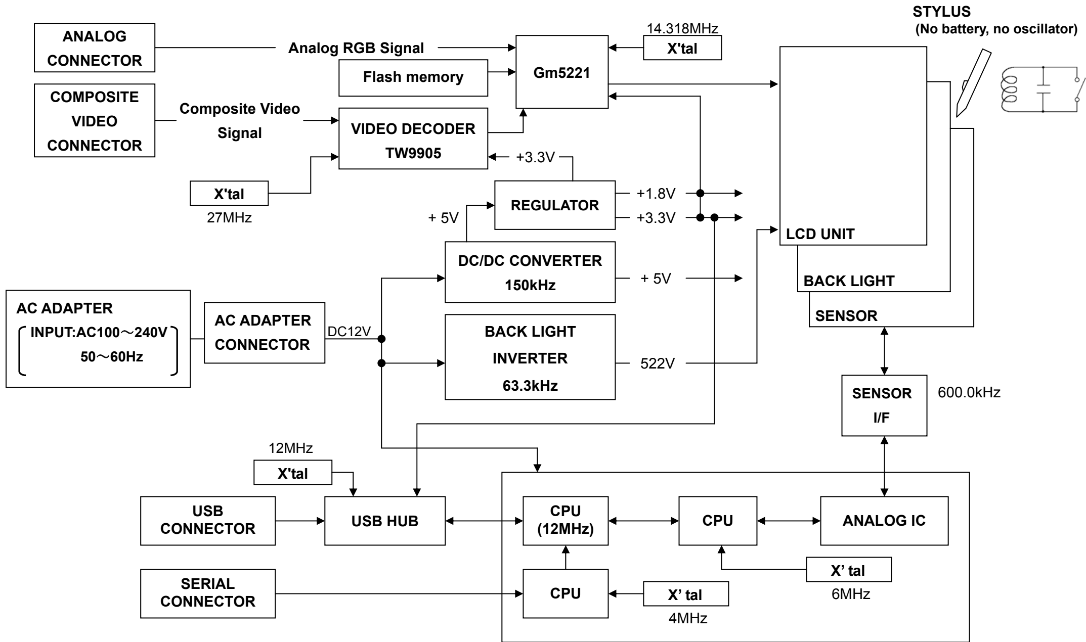
< DTF-520 Block Diagram >
