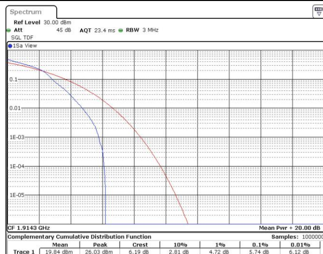
Band25-1.4MHz-16QAM-26683-1RB#0
