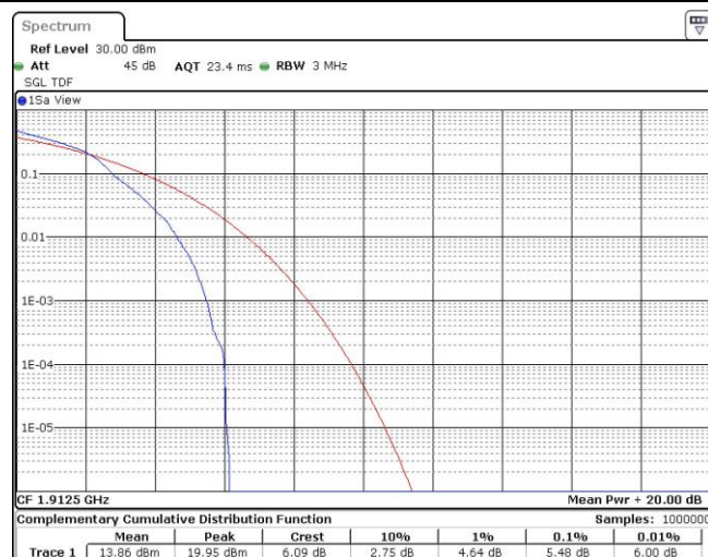
Band25-5MHz-16QAM-26665-1RB#0
