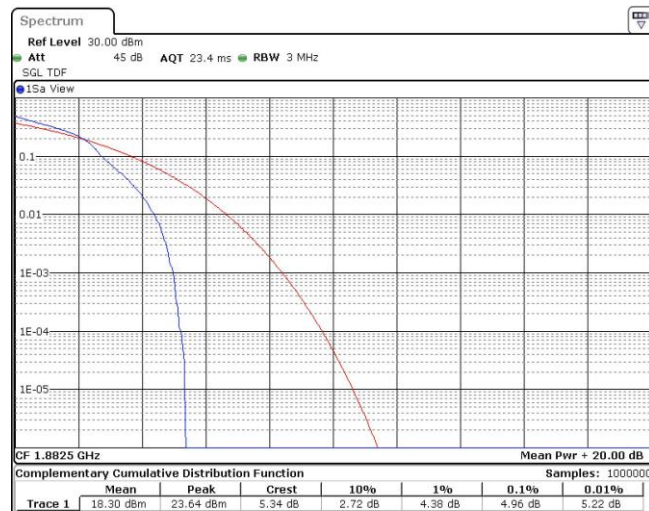
Band25-3MHz-16QAM-26365-15RB#0
