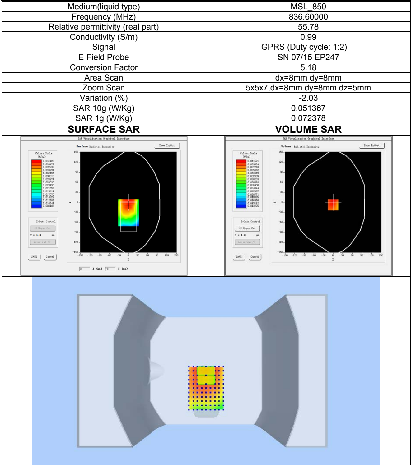
Plot 2: GPRS850MHz, Middle channel (Body-worn/Hotspot, Back Surface) Product Description:Mobile Phone Test Date: 2019-10-08
