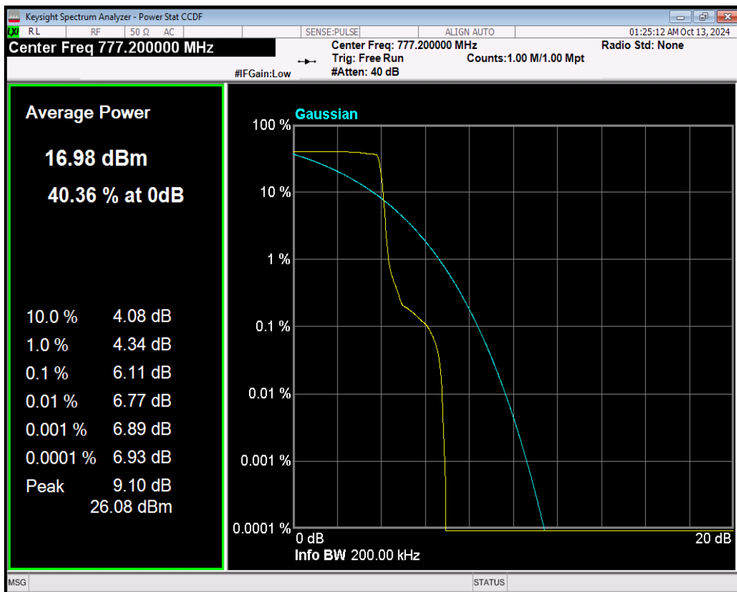
Band13 QPSK Channel=23182 nTones=1@0 Spacing=3.75kHz
