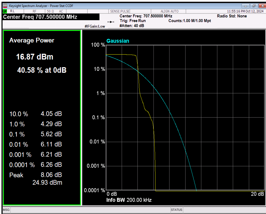
Band12 BPSK Channel=23095 nTones=1@0 Spacing=15kHz
