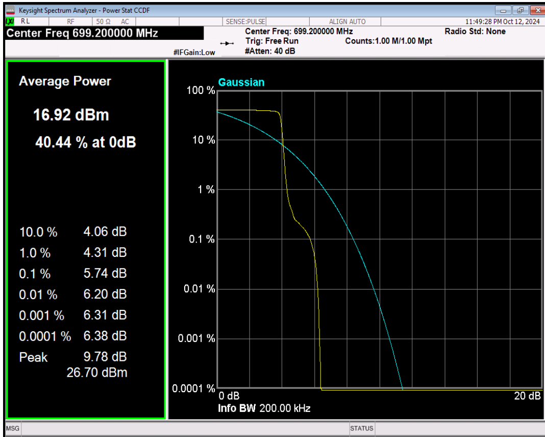
Band12 BPSK Channel=23012 nTones=1@0 Spacing=15kHz
