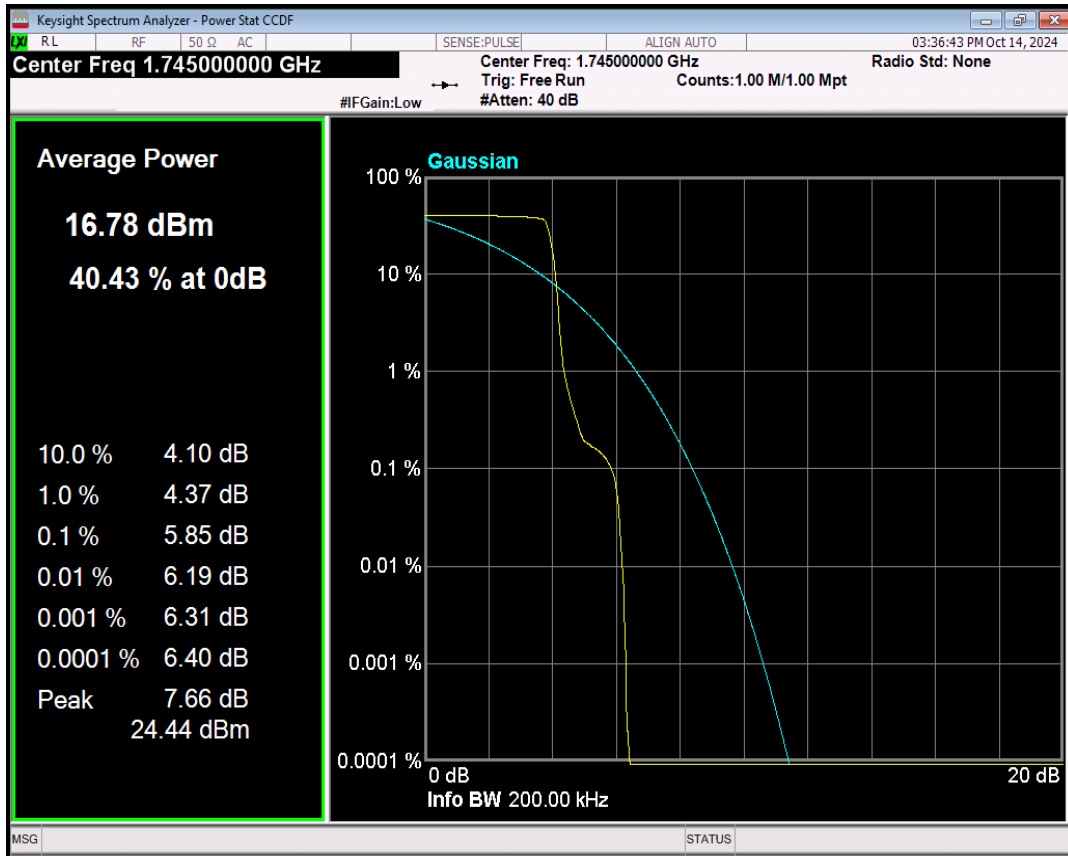
Band66 BPSK Channel=132322 nTones=1@0 Spacing=15kHz
