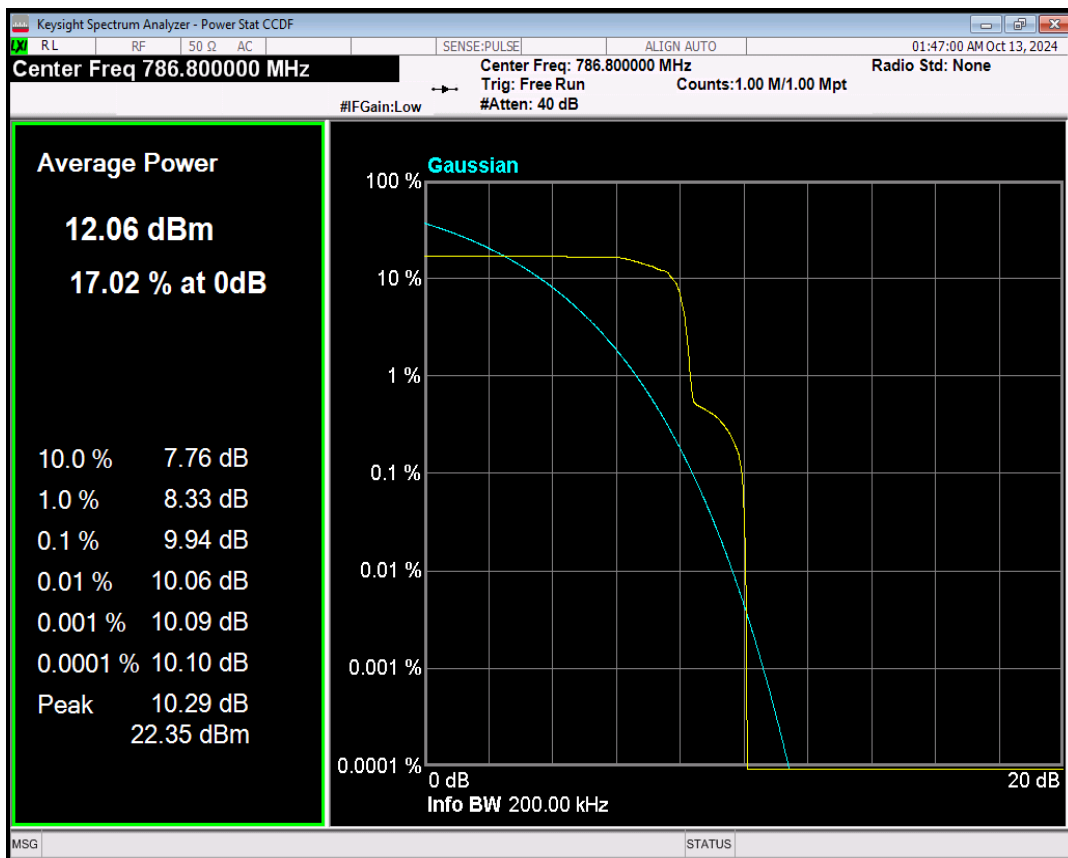
Band13 QPSK Channel=23278 nTones=1@0 Spacing=15kHz
