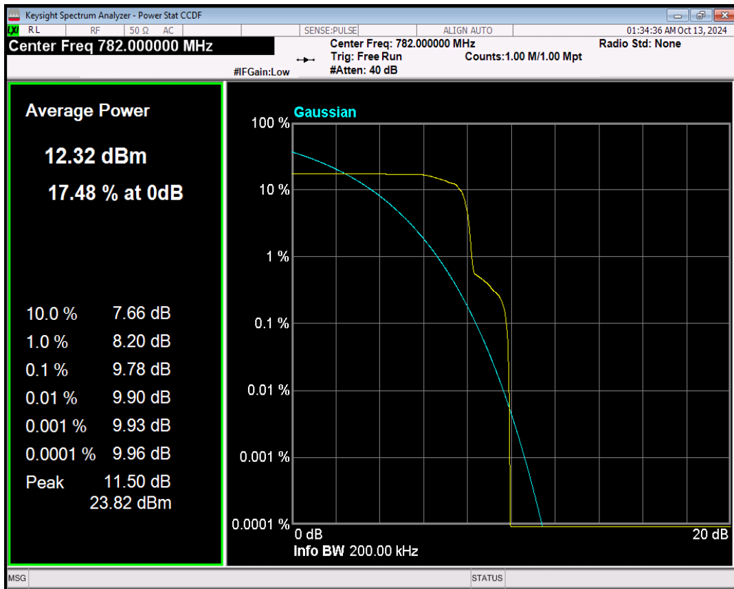
Band13 QPSK Channel=23230 nTones=1@0 Spacing=15kHz
