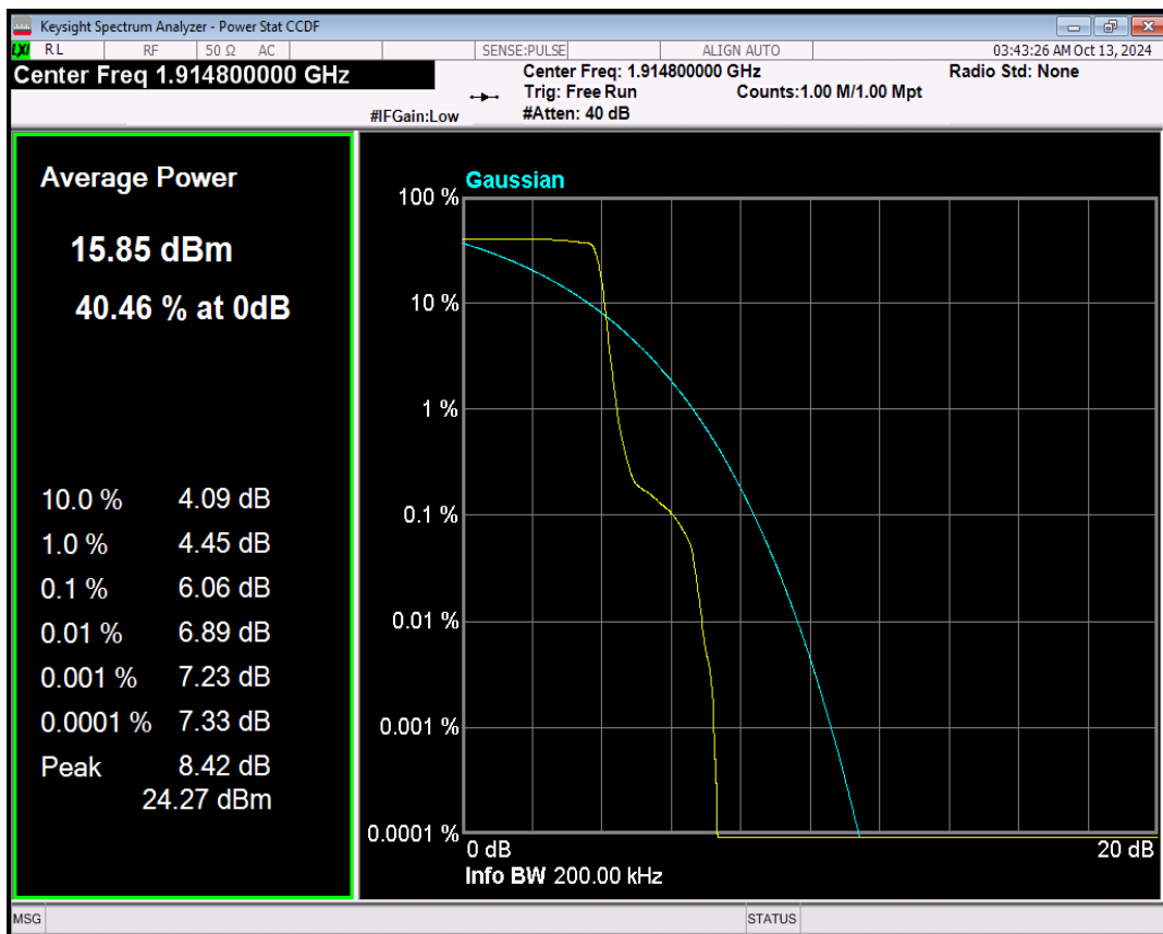
Band25 QPSK Channel=26688 nTones=1@0 Spacing=3.75kHz
