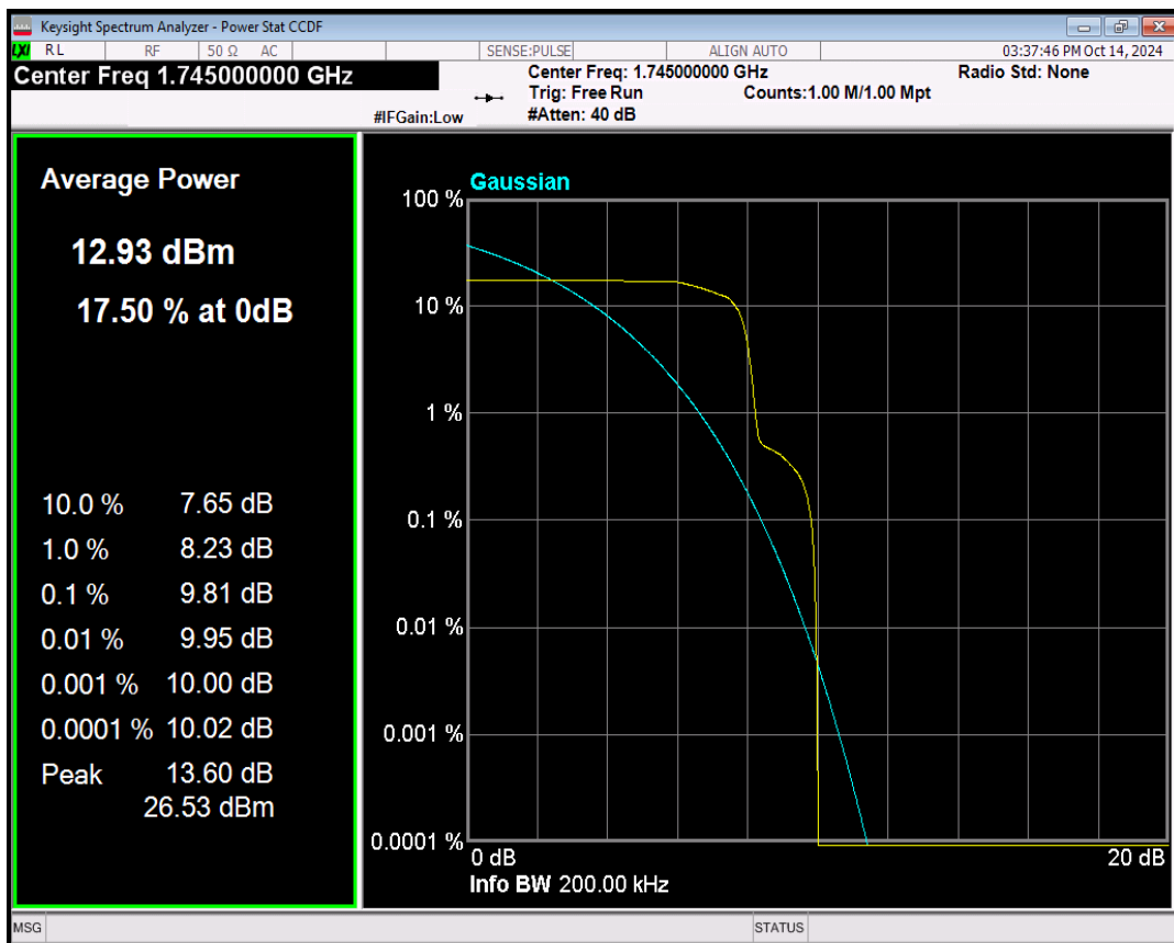
Band66 QPSK Channel=132322 nTones=1@0 Spacing=15kHz
