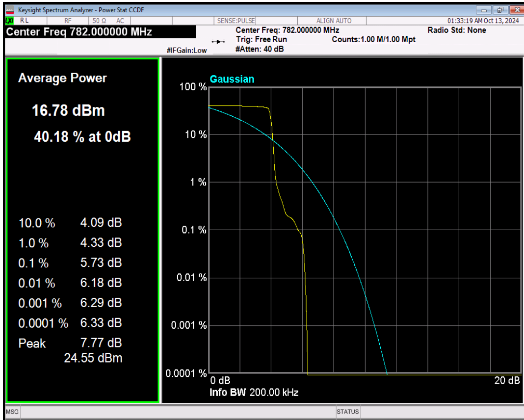
Band13 BPSK Channel=23230 nTones=1@0 Spacing=15kHz
