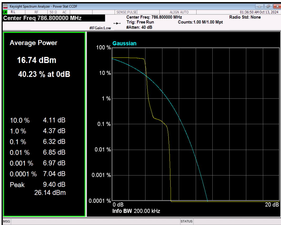
Band13 QPSK Channel=23278 nTones=1@0 Spacing=3.75kHz
