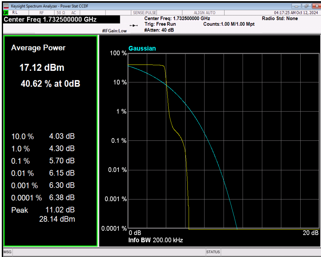
Band4 BPSK Channel=20175 nTones=1@0 Spacing=15kHz
