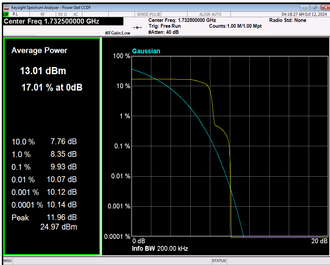
Band4 QPSK Channel=20175 nTones=1@0 Spacing=15kHz
