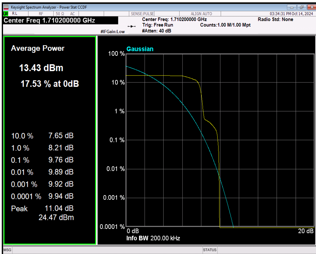
Band66 QPSK Channel=131974 nTones=1@0 Spacing=15kHz
