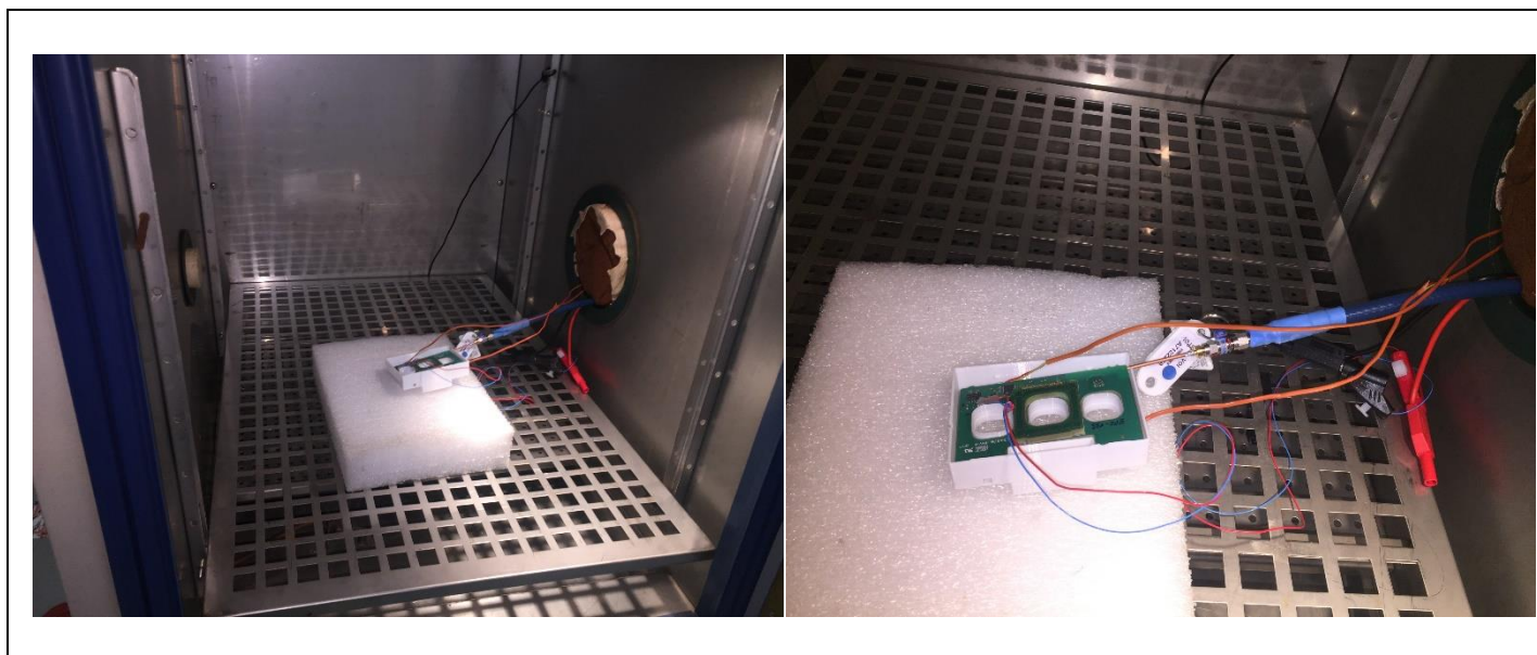
Photograph for Maximum Conducted Output Power
