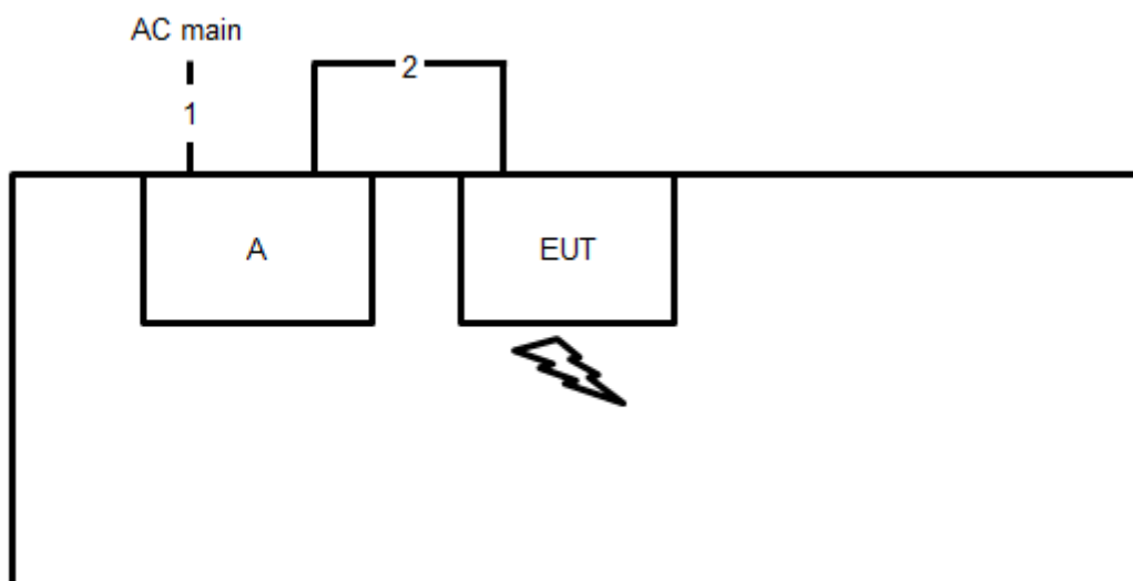
Test Setup Diagram - Transmitter Spurious Emissions below 1 GHz
