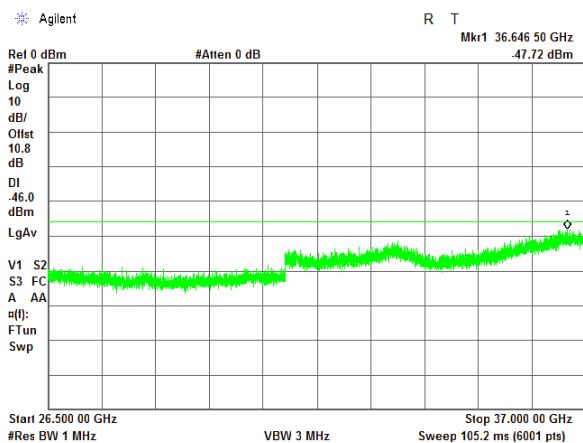
ANTENNA CHAIN: #3
