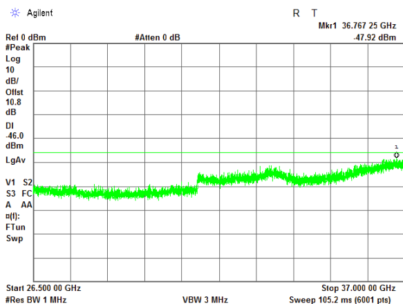
ANTENNA CHAIN: #3
