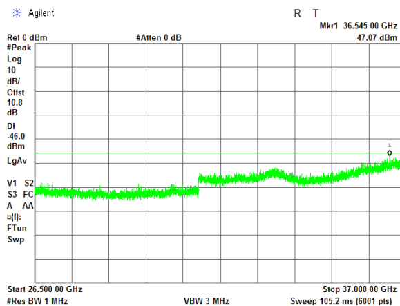
ANTENNA CHAIN: #4
