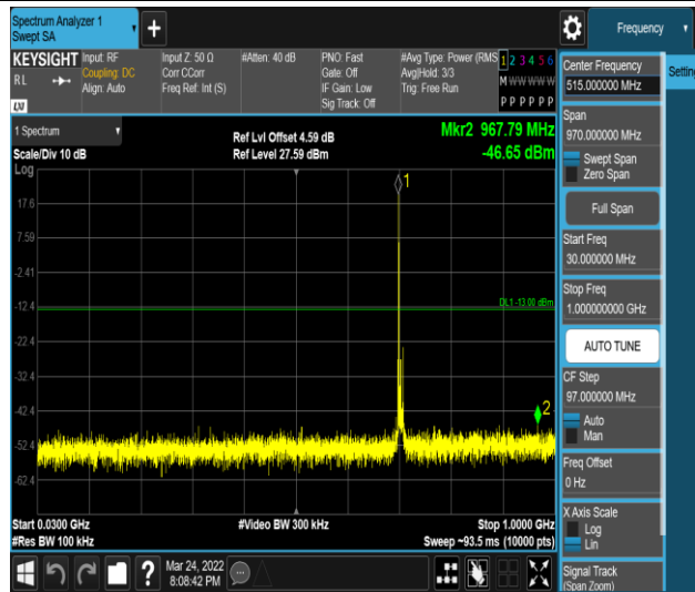
Band17-10MHz-16QAM-23780-1RB#0-Range1:30~1000MHz
