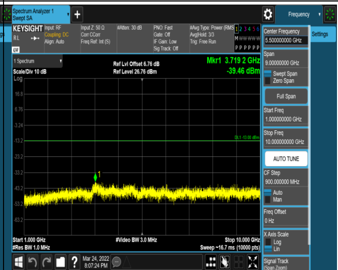
Band17-10MHz-16QAM-23790-1RB#0-Range2:1000~10000MHz
