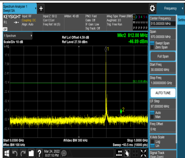
Band17-10MHz-16QAM-23790-1RB#0-Range1:30~1000MHz
