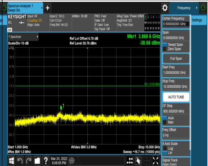
Band17-10MHz-16QAM-23780-1RB#0-Range2:1000~10000MHz
