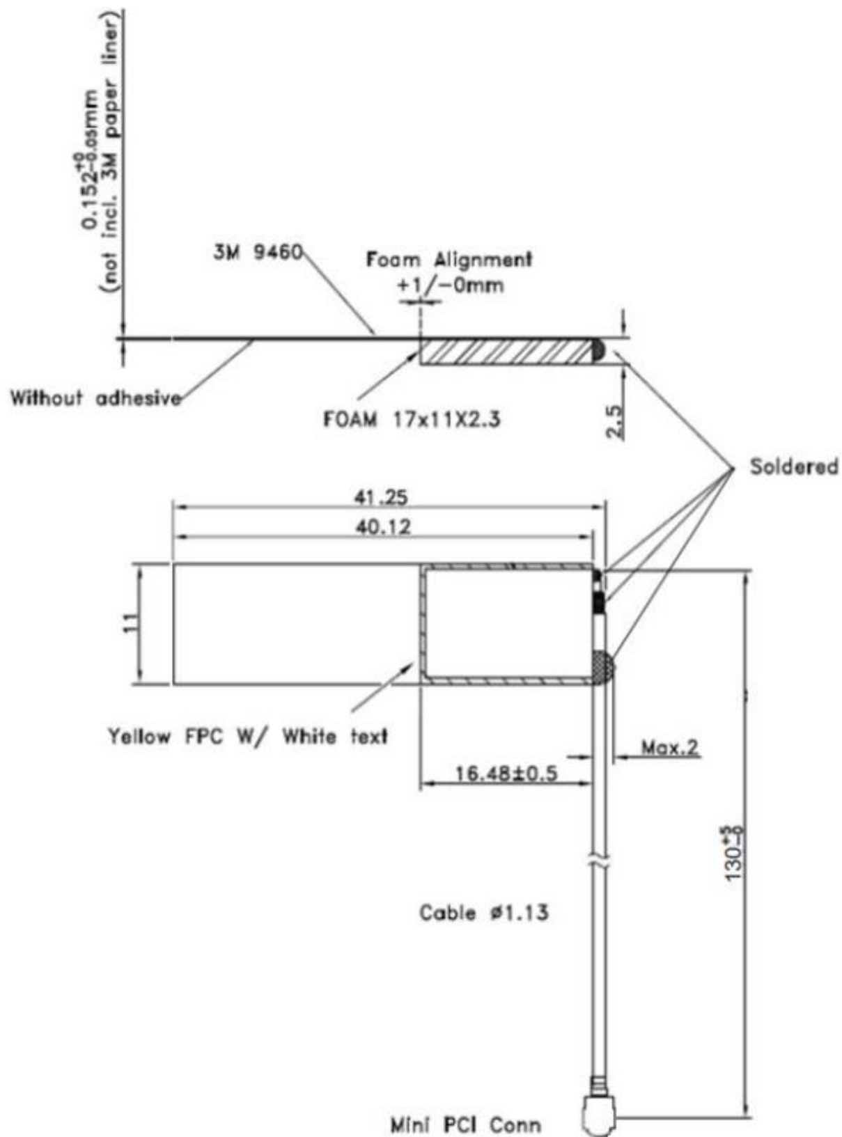
Figure 2: FlexPIFA mechanical drawing of EFB2400A3S-13MHF1
