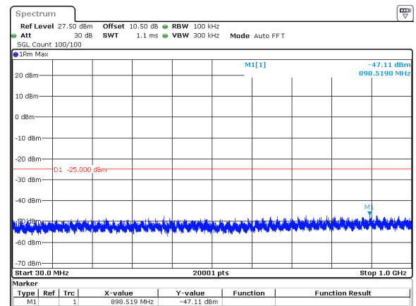
40MHz_30kHz_2670MHz_DFT-s-OFDM QPSK_RB1@105&amp;-47.11 dBm
