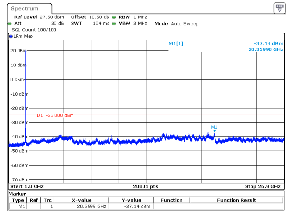
50MHz_30kHz_2592.99MHz_DFT-s-OFDM QPSK_RB1@0&amp;-37.14 dBm
