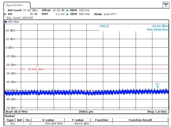
15MHz_30kHz_2682.48MHz_DFT-s-OFDM QPSK_RB1@0&amp;-46.64 dBm
