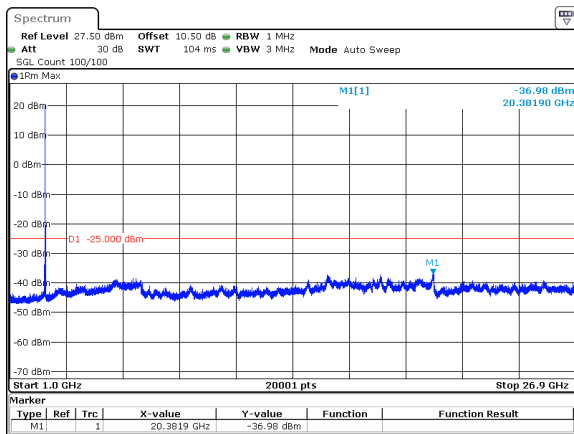
60MHz_30kHz_2592.99MHz_DFT-s-OFDM QPSK_RB1@161&amp;-36.98 dBm
