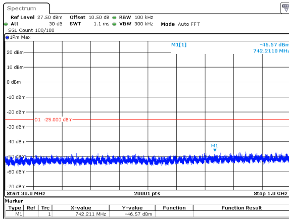
30MHz_30kHz_2511MHz_DFT-s-OFDM QPSK_RB1@0&amp;-46.57 dBm
