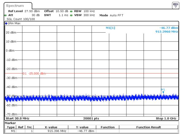
40MHz_30kHz_2516.01MHz_DFT-s-OFDM QPSK_RB1@105&amp;-46.77 dBm
