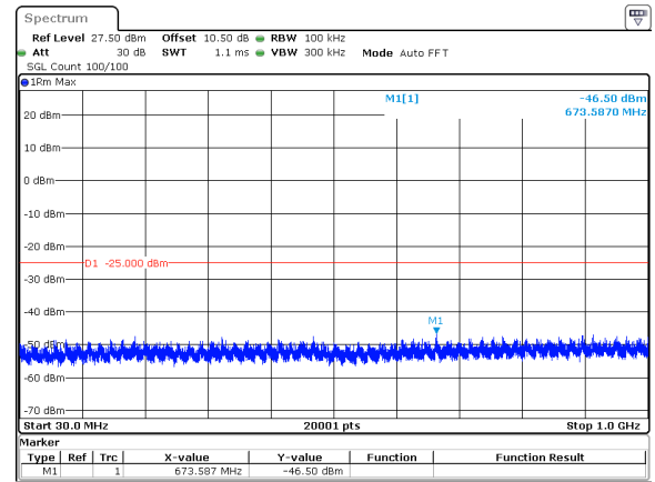
40MHz_30kHz_2670MHz_DFT-s-OFDM QPSK_RB1@0&amp;-46.50 dBm
