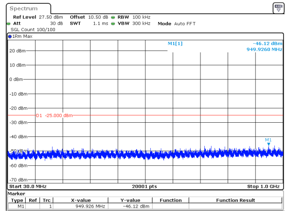
30MHz_15kHz_2674.995MHz_DFT-s-OFDM QPSK_RB1@0&amp;-46.12 dBm
