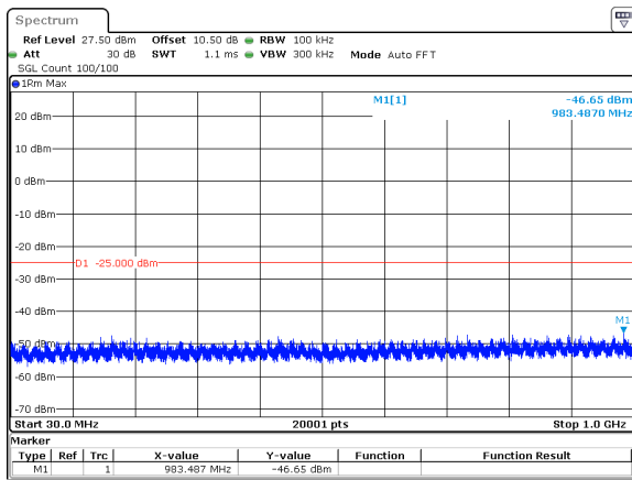
50MHz_30kHz_2521.02MHz_DFT-s-OFDM QPSK_RB1@132&amp;-46.65 dBm
