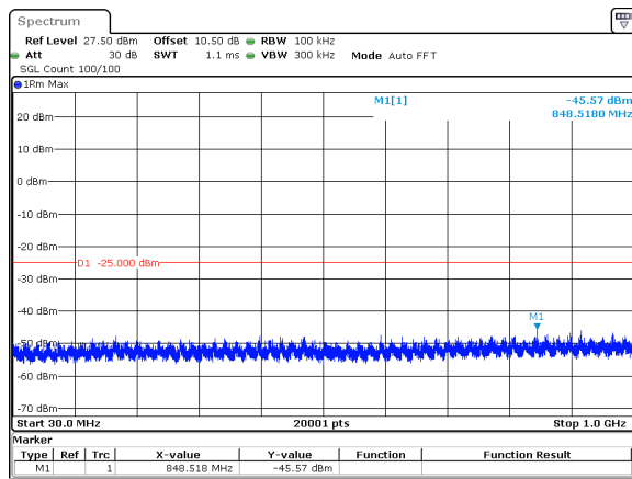
15MHz_15kHz_2682.495MHz_DFT-s-OFDM QPSK_RB1@0&amp;-45.57 dBm
