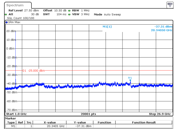
15MHz_30kHz_2592.99MHz_DFT-s-OFDM QPSK_RB1@0&amp;-37.31 dBm
