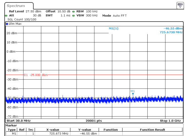
50MHz_30kHz_2592.99MHz_DFT-s-OFDM QPSK_RB1@132&amp;-46.55 dBm
