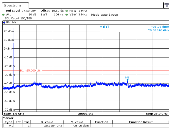
20MHz_15kHz_2679.99MHz_DFT-s-OFDM QPSK_RB1@105&amp;-36.96 dBm
