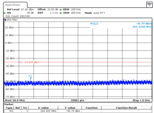
15MHz_15kHz_2503.5MHz_DFT-s-OFDM QPSK_RB1@78&amp;-46.79 dBm
