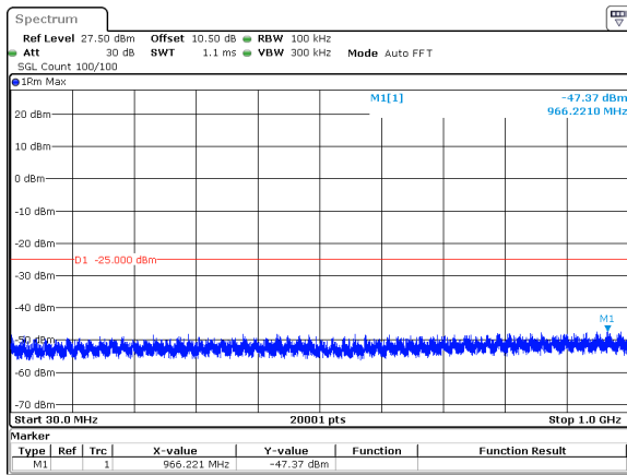
15MHz_30kHz_2592.99MHz_DFT-s-OFDM QPSK_RB1@0&amp;-47.37 dBm
