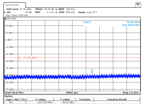
60MHz_30kHz_2592.99MHz_DFT-s-OFDM QPSK_RB162@0&amp;-46.85 dBm
