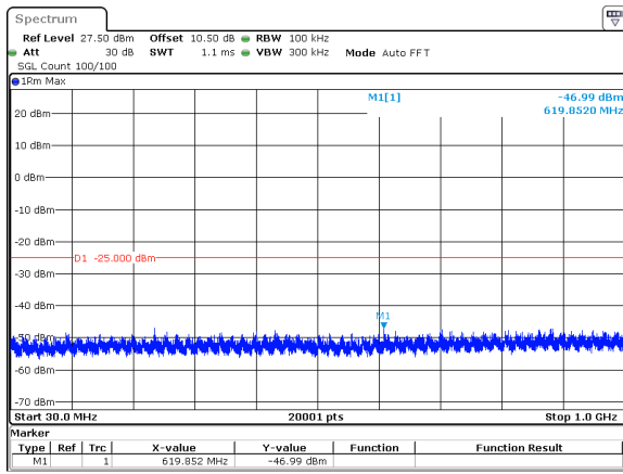
60MHz_30kHz_2592.99MHz_DFT-s-OFDM QPSK_RB1@0&amp;-46.99 dBm
