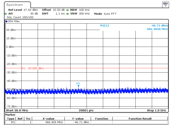
60MHz_30kHz_2526MHz_DFT-s-OFDM QPSK_RB1@0&amp;-46.71 dBm
