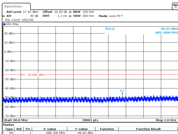
30MHz_15kHz_2593.005MHz_DFT-s-OFDM QPSK_RB160@0&amp;-46.62 dBm
