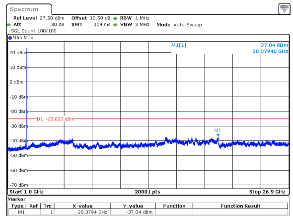
30MHz_15kHz_2674.995MHz_DFT-s-OFDM QPSK_RB1@159&amp;-37.04 dBm
