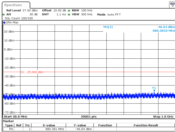
10MHz_30kHz_2501.01MHz_DFT-s-OFDM QPSK_RB1@23&amp;-46.64 dBm
