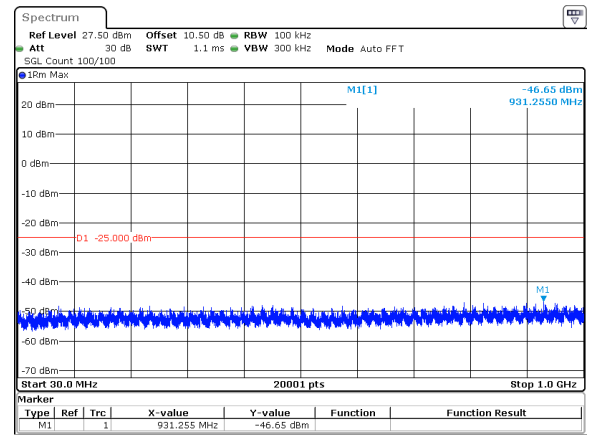
50MHz_30kHz_2521.02MHz_DFT-s-OFDM QPSK_RB1@0&amp;-46.65 dBm
