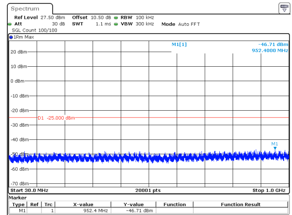
30MHz_30kHz_2511MHz_DFT-s-OFDM QPSK_RB1@77&amp;-46.71 dBm
