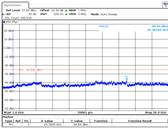
30MHz_30kHz_2592.99MHz_DFT-s-OFDM QPSK_RB1@0&amp;-36.84 dBm
