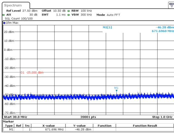
10MHz_30kHz_2592.99MHz_DFT-s-OFDM QPSK_RB1@0&amp;-46.28 dBm
