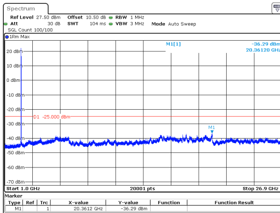
30MHz_30kHz_2511MHz_DFT-s-OFDM QPSK_RB1@77&amp;-36.29 dBm
