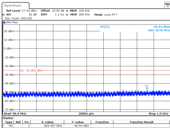
50MHz_30kHz_2664.99MHz_DFT-s-OFDM QPSK_RB1@132&amp;-46.64 dBm
