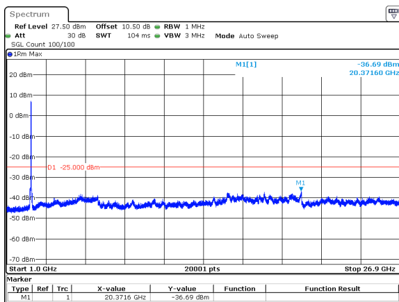
60MHz_30kHz_2592.99MHz_DFT-s-OFDM QPSK_RB162@0&amp;-36.69 dBm
