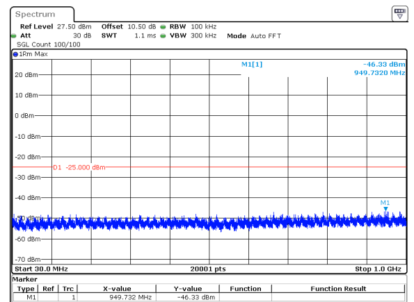
50MHz_30kHz_2664.99MHz_DFT-s-OFDM QPSK_RB128@0&amp;-46.33 dBm
