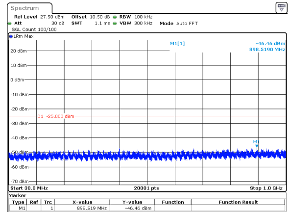
40MHz_15kHz_2593.005MHz_DFT-s-OFDM QPSK_RB1@215&amp;-46.46 dBm
