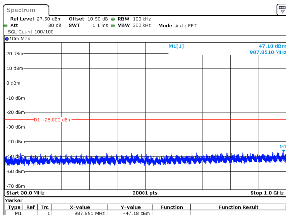
50MHz_15kHz_2521.005MHz_DFT-s-OFDM QPSK_RB270@0&amp;-47.18 dBm
