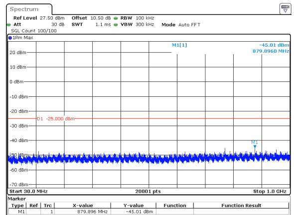
15MHz_30kHz_2682.48MHz_DFT-s-OFDM QPSK_RB36@0&amp;-45.01 dBm
