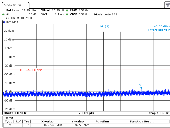
50MHz_30kHz_2664.99MHz_DFT-s-OFDM QPSK_RB1@0&amp;-46.50 dBm
