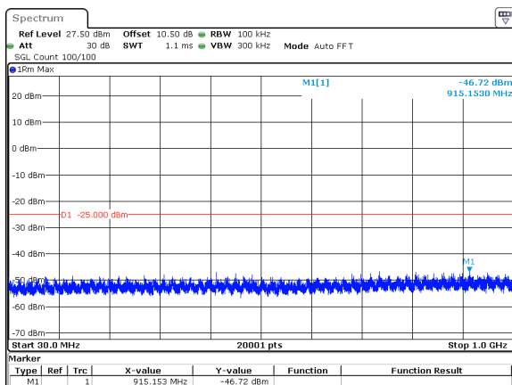
15MHz_30kHz_2592.99MHz_DFT-s-OFDM QPSK_RB36@0&amp;-46.72 dBm
