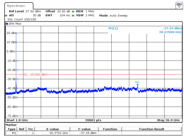
50MHz_30kHz_2521.02MHz_DFT-s-OFDM QPSK_RB1@132&amp;-37.34 dBm
