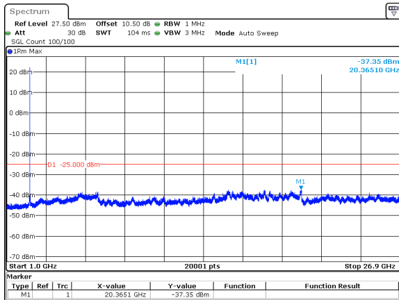
20MHz_15kHz_2506.005MHz_DFT-s-OFDM QPSK_RB1@105&amp;-37.35 dBm
