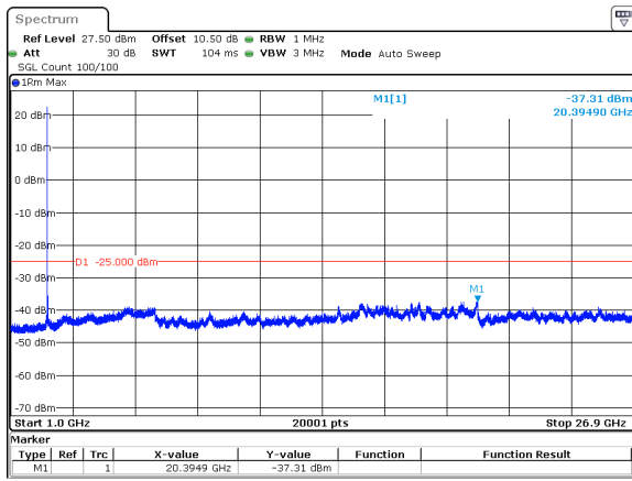
50MHz_30kHz_2521.02MHz_DFT-s-OFDM QPSK_RB1@0&amp;-37.31 dBm
