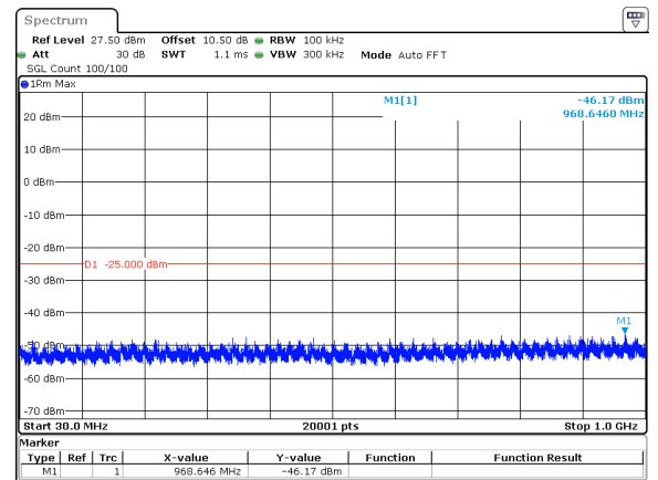
60MHz_30kHz_2592.99MHz_DFT-s-OFDM QPSK_RB1@161&amp;-46.17 dBm
