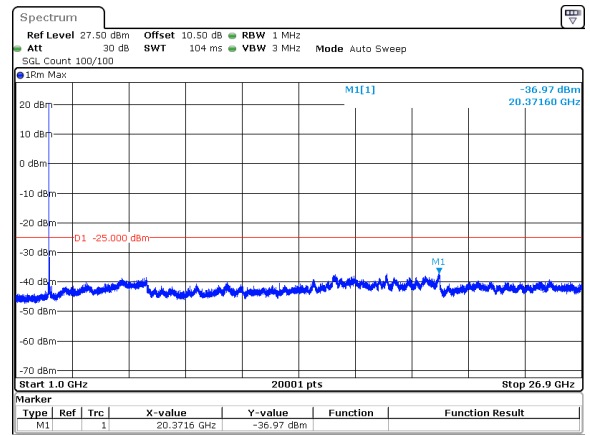
50MHz_15kHz_2521.005MHz_DFT-s-OFDM QPSK_RB1@0&amp;-36.97 dBm
