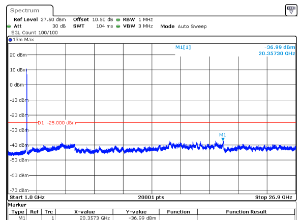
30MHz_15kHz_2674.995MHz_DFT-s-OFDM QPSK_RB160@0&amp;-36.99 dBm
