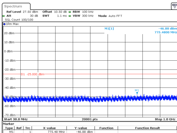
30MHz_15kHz_2674.995MHz_DFT-s-OFDM QPSK_RB160@0&amp;-46.88 dBm
