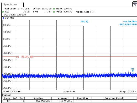
30MHz_15kHz_2674.995MHz_DFT-s-OFDM QPSK_RB1@159&amp;-46.50 dBm
