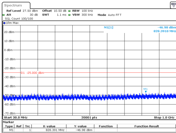
50MHz_15kHz_2521.005MHz_DFT-s-OFDM QPSK_RB1@0&amp;-46.98 dBm
