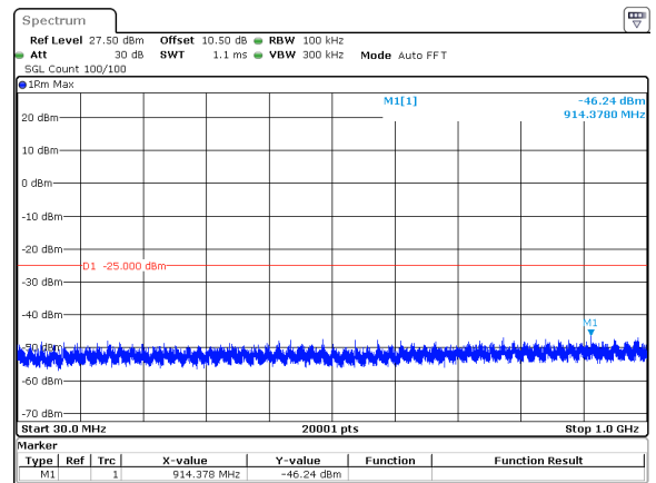
10MHz_30kHz_2592.99MHz_DFT-s-OFDM QPSK_RB1@23&amp;-46.24 dBm
