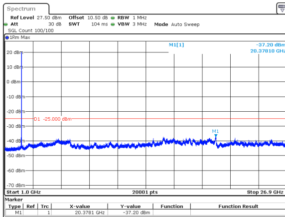
30MHz_15kHz_2511MHz_DFT-s-OFDM QPSK_RB1@159&amp;-37.20 dBm
