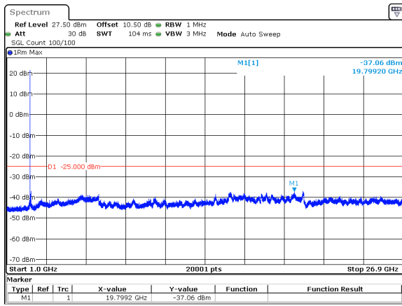
40MHz_15kHz_2516.01MHz_DFT-s-OFDM QPSK_RB1@0&amp;-37.06 dBm
