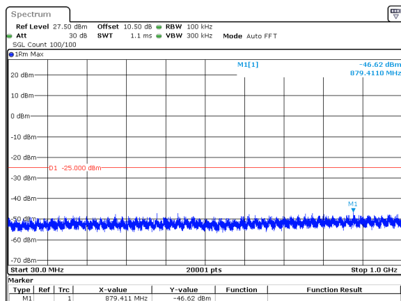
15MHz_15kHz_2503.5MHz_DFT-s-OFDM QPSK_RB75@0&amp;-46.62 dBm
