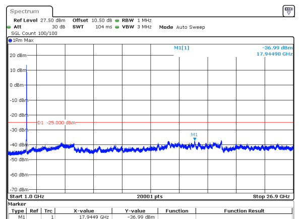
15MHz_15kHz_2682.495MHz_DFT-s-OFDM QPSK_RB75@0&amp;-36.99 dBm
