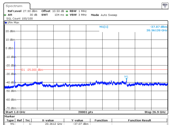
40MHz_30kHz_2592.99MHz_DFT-s-OFDM QPSK_RB100@0&amp;-37.07 dBm
