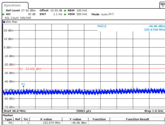
50MHz_15kHz_2521.005MHz_DFT-s-OFDM QPSK_RB1@269&amp;-46.86 dBm
