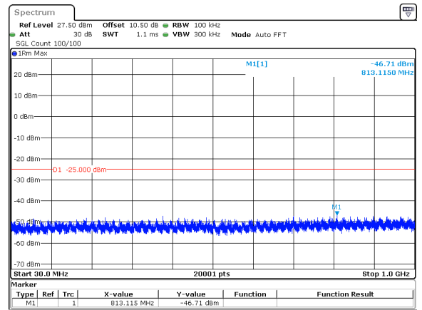
30MHz_15kHz_2593.005MHz_DFT-s-OFDM QPSK_RB1@0&amp;-46.71 dBm
