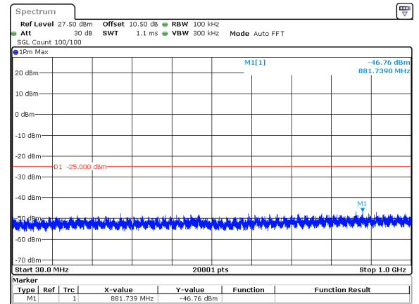
20MHz_15kHz_2506.005MHz_DFT-s-OFDM QPSK_RB1@105&amp;-46.76 dBm
