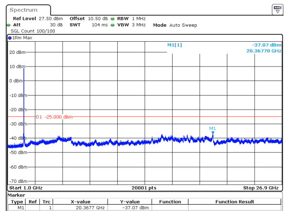
40MHz_30kHz_2516.01MHz_DFT-s-OFDM QPSK_RB100@0&amp;-37.07 dBm
