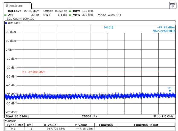
15MHz_30kHz_2503.5MHz_DFT-s-OFDM QPSK_RB1@37&amp;-47.15 dBm
