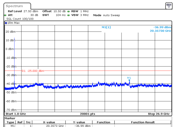
15MHz_15kHz_2503.5MHz_DFT-s-OFDM QPSK_RB75@0&amp;-36.99 dBm
