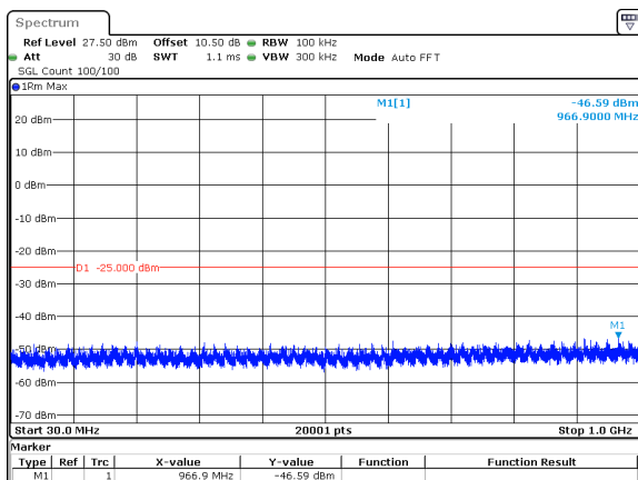
50MHz_15kHz_2664.99MHz_DFT-s-OFDM QPSK_RB270@0&amp;-46.59 dBm
