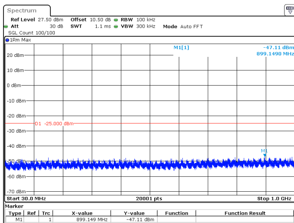
40MHz_30kHz_2516.01MHz_DFT-s-OFDM QPSK_RB100@0&amp;-47.11 dBm
