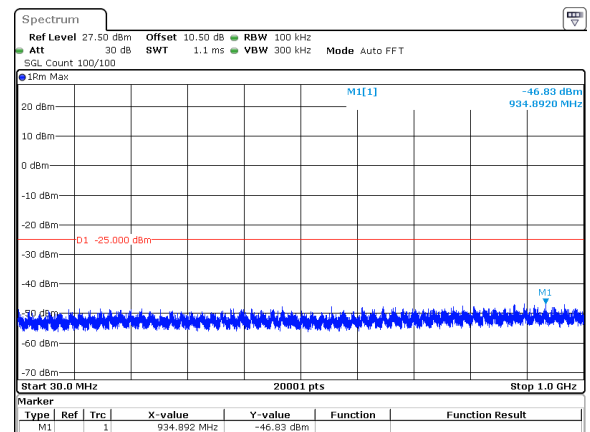
60MHz_30kHz_2526MHz_DFT-s-OFDM QPSK_RB162@0&amp;-46.83 dBm
