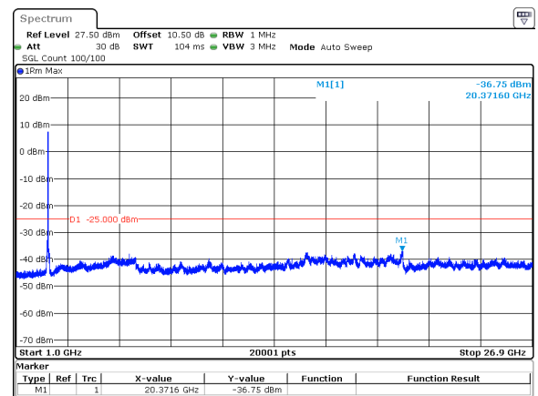
50MHz_30kHz_2592.99MHz_DFT-s-OFDM QPSK_RB128@0&amp;-36.75 dBm
