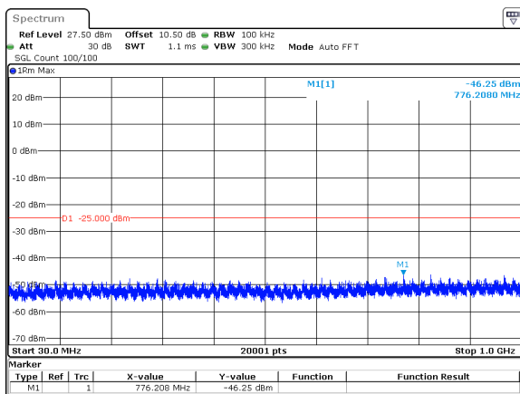
50MHz_30kHz_2592.99MHz_DFT-s-OFDM QPSK_RB128@0&amp;-46.25 dBm
