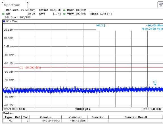
50MHz_30kHz_2592.99MHz_DFT-s-OFDM QPSK_RB1@0&amp;-46.45 dBm
