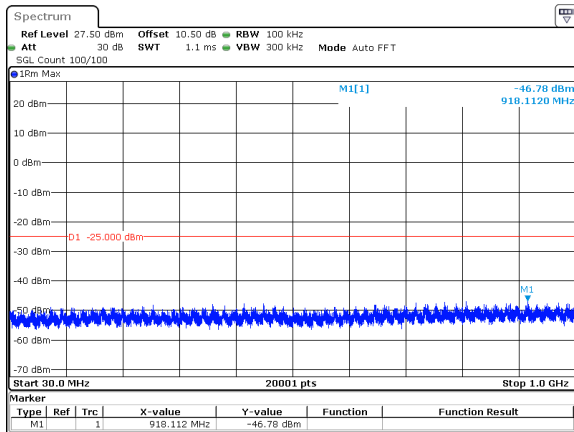
15MHz_30kHz_2592.99MHz_DFT-s-OFDM QPSK_RB1@37&amp;-46.78 dBm
