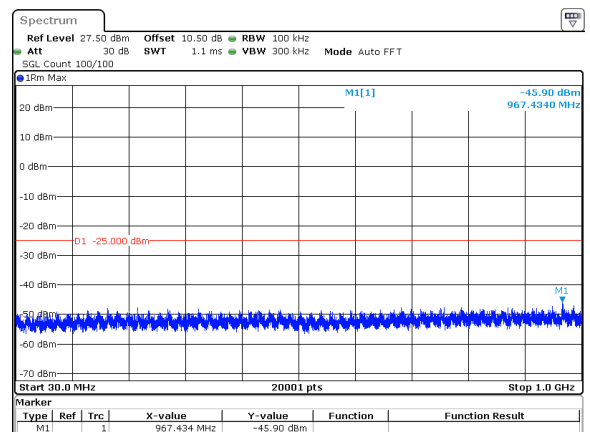
15MHz_30kHz_2503.5MHz_DFT-s-OFDM QPSK_RB36@0&amp;-45.90 dBm
