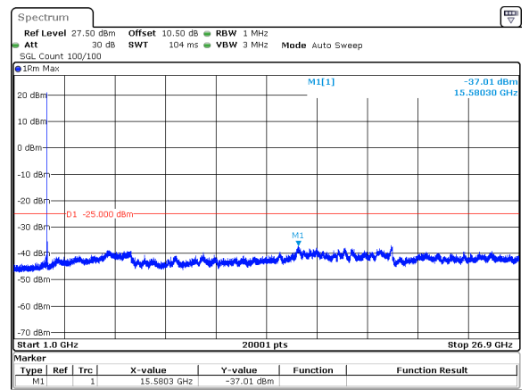
15MHz_15kHz_2682.495MHz_DFT-s-OFDM QPSK_RB1@0&amp;-37.01 dBm
