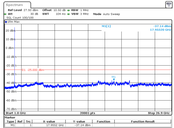
40MHz_15kHz_2516.01MHz_DFT-s-OFDM QPSK_RB1@215&amp;-37.14 dBm
