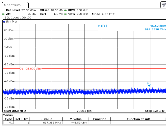
50MHz_15kHz_2593.005MHz_DFT-s-OFDM QPSK_RB1@0&amp;-46.52 dBm
