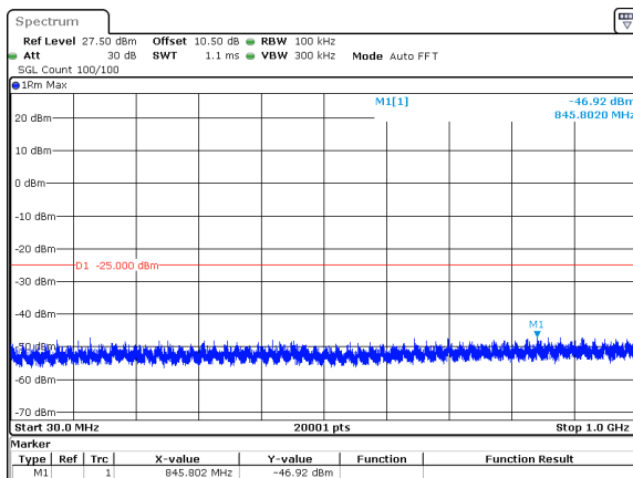
30MHz_15kHz_2511MHz_DFT-s-OFDM QPSK_RB160@0&amp;-46.92 dBm
