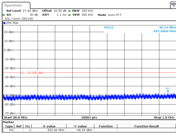
40MHz_15kHz_2593.005MHz_DFT-s-OFDM QPSK_RB1@0&amp;-46.54 dBm
