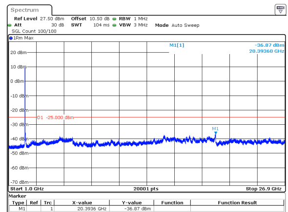
50MHz_30kHz_2521.02MHz_DFT-s-OFDM QPSK_RB128@0&amp;-36.87 dBm
