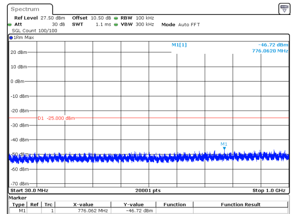
40MHz_15kHz_2593.005MHz_DFT-s-OFDM QPSK_RB216@0&amp;-46.72 dBm
