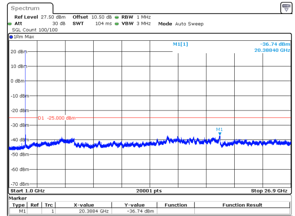
30MHz_15kHz_2511MHz_DFT-s-OFDM QPSK_RB1@0&amp;-36.74 dBm
