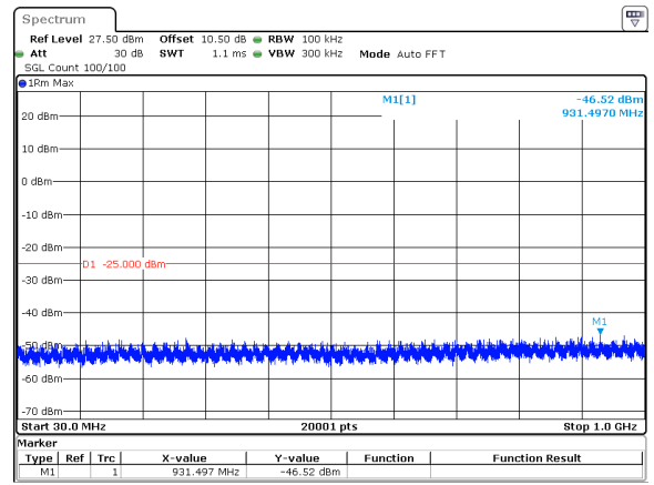
30MHz_30kHz_2592.99MHz_DFT-s-OFDM QPSK_RB1@0&amp;-46.52 dBm
