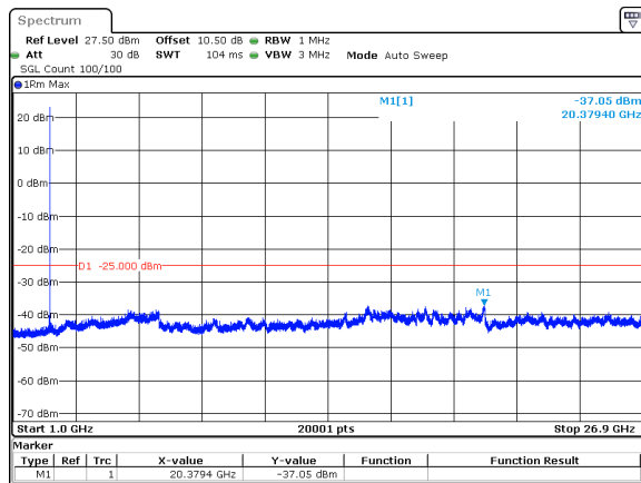
15MHz_15kHz_2503.5MHz_DFT-s-OFDM QPSK_RB1@78&amp;-37.05 dBm
