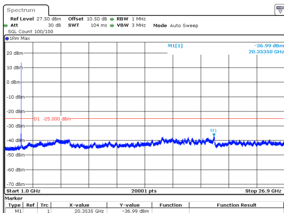
15MHz_30kHz_2503.5MHz_DFT-s-OFDM QPSK_RB36@0&amp;-36.99 dBm
