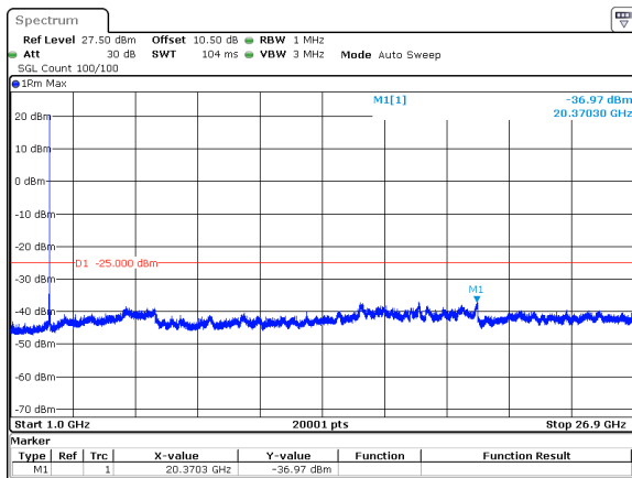
50MHz_30kHz_2592.99MHz_DFT-s-OFDM QPSK_RB1@132&amp;-36.97 dBm
