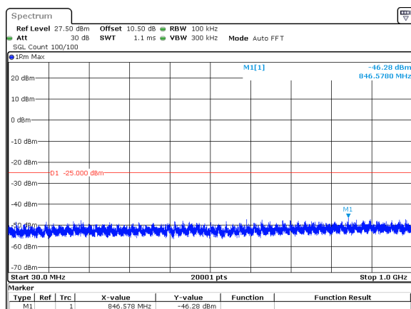
15MHz_15kHz_2682.495MHz_DFT-s-OFDM QPSK_RB75@0&amp;-46.28 dBm
