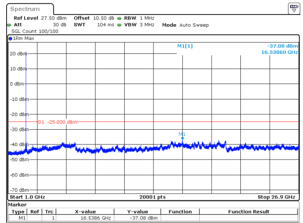
40MHz_30kHz_2592.99MHz_DFT-s-OFDM QPSK_RB1@0&amp;-37.08 dBm
