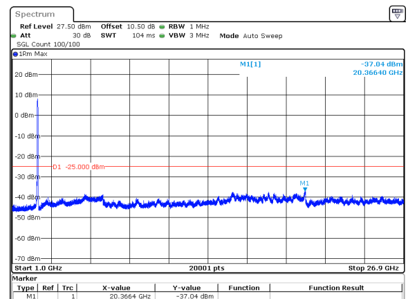
50MHz_15kHz_2664.99MHz_DFT-s-OFDM QPSK_RB270@0&amp;-37.04 dBm
