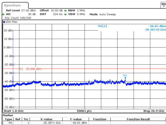
30MHz_30kHz_2592.99MHz_DFT-s-OFDM QPSK_RB1@77&amp;-36.81 dBm
