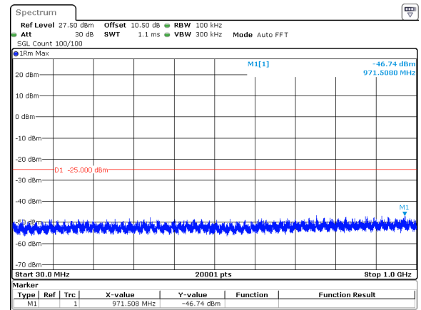
60MHz_30kHz_2526MHz_DFT-s-OFDM QPSK_RB1@161&amp;-46.74 dBm
