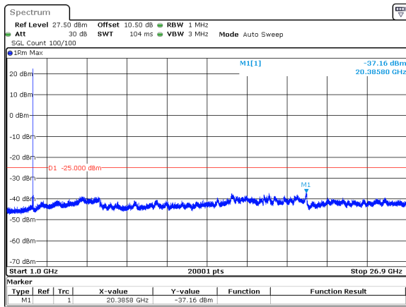
30MHz_15kHz_2674.995MHz_DFT-s-OFDM QPSK_RB1@0&amp;-37.16 dBm
