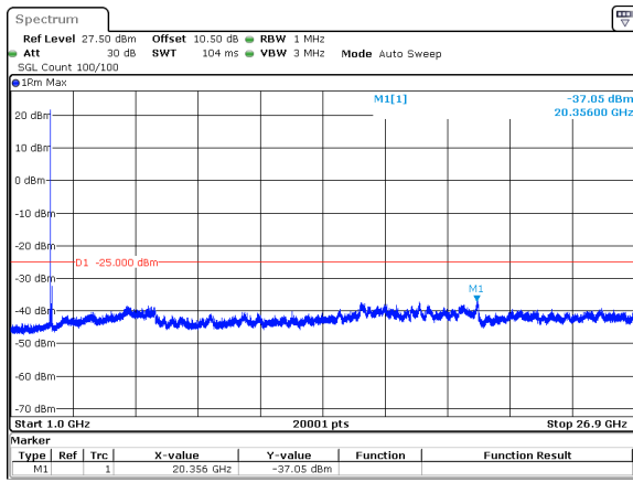
50MHz_15kHz_2664.99MHz_DFT-s-OFDM QPSK_RB1@0&amp;-37.05 dBm
