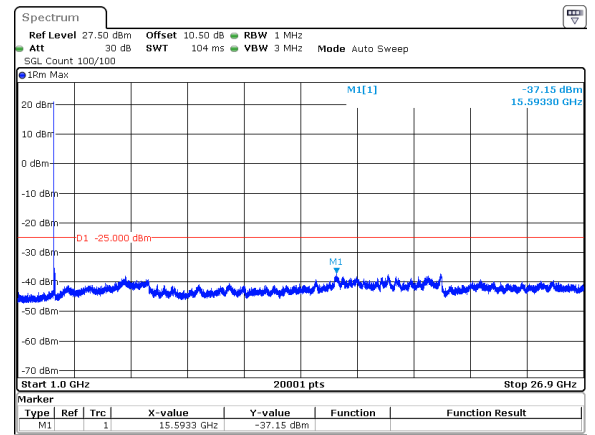
50MHz_30kHz_2664.99MHz_DFT-s-OFDM QPSK_RB1@0&amp;-37.15 dBm
