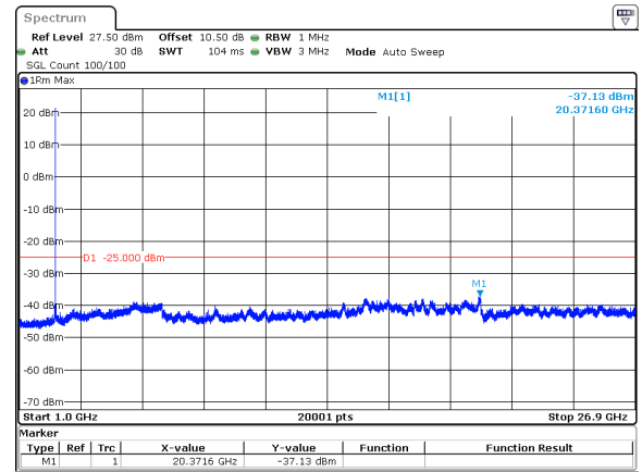
30MHz_30kHz_2511MHz_DFT-s-OFDM QPSK_RB1@0&amp;-37.13 dBm
