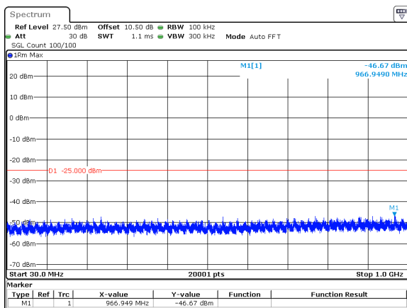
50MHz_30kHz_2521.02MHz_DFT-s-OFDM QPSK_RB128@0&amp;-46.67 dBm
