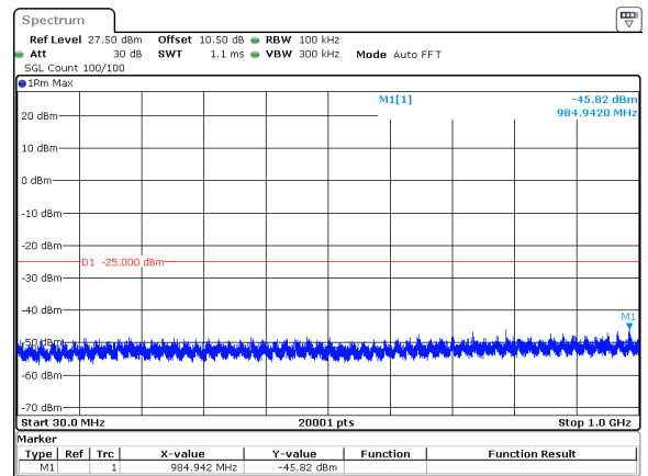
30MHz_30kHz_2592.99MHz_DFT-s-OFDM QPSK_RB1@77&amp;-45.82 dBm
