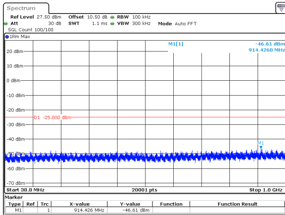
40MHz_15kHz_2516.01MHz_DFT-s-OFDM QPSK_RB1@215&amp;-46.61 dBm
