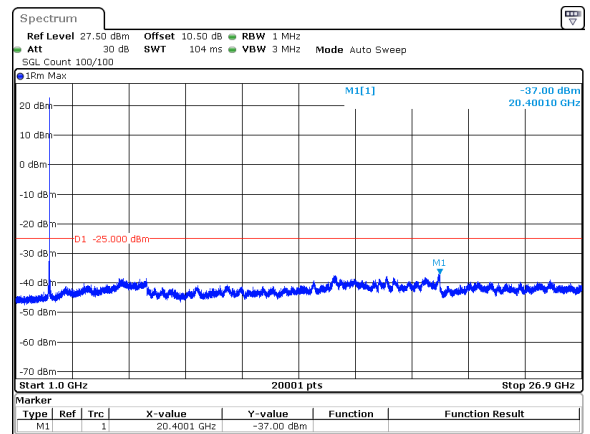
50MHz_15kHz_2521.005MHz_DFT-s-OFDM QPSK_RB1@269&amp;-37.00 dBm
