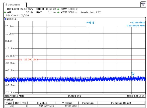
20MHz_15kHz_2679.99MHz_DFT-s-OFDM QPSK_RB1@105&amp;-47.06 dBm
