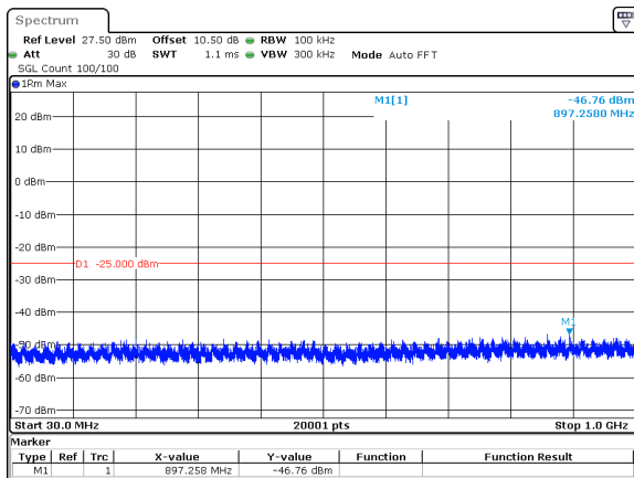
40MHz_15kHz_2516.01MHz_DFT-s-OFDM QPSK_RB216@0&amp;-46.76 dBm
