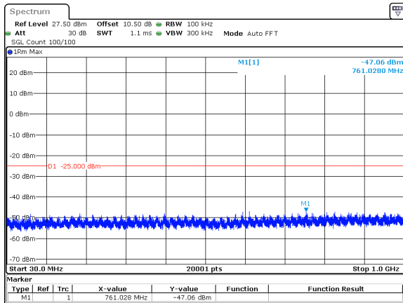
30MHz_15kHz_2593.005MHz_DFT-s-OFDM QPSK_RB1@159&amp;-47.06 dBm
