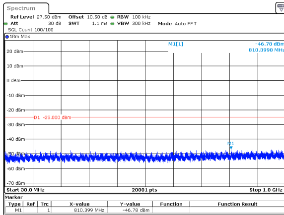
30MHz_15kHz_2511MHz_DFT-s-OFDM QPSK_RB1@0&amp;-46.78 dBm
