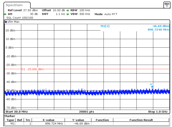
40MHz_15kHz_2516.01MHz_DFT-s-OFDM QPSK_RB1@0&amp;-46.69 dBm
