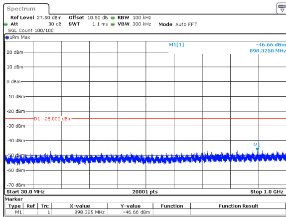
40MHz_30kHz_2592.99MHz_DFT-s-OFDM QPSK_RB1@0&amp;-46.66 dBm
