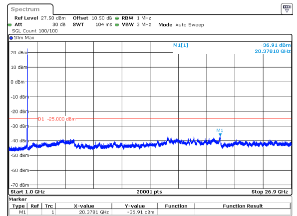
50MHz_30kHz_2664.99MHz_DFT-s-OFDM QPSK_RB1@132&amp;-36.91 dBm
