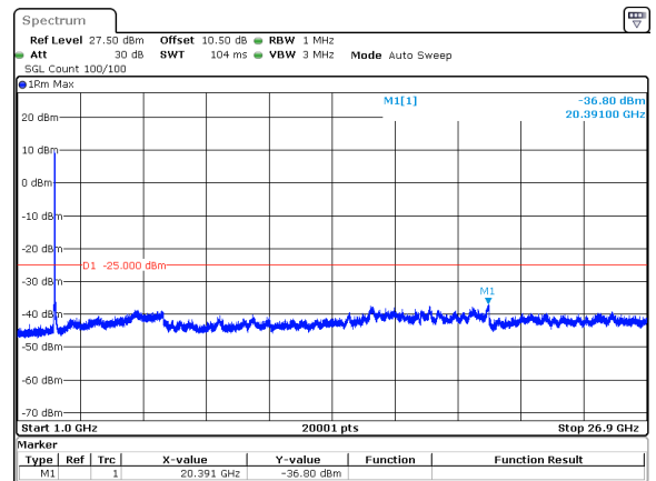
40MHz_15kHz_2516.01MHz_DFT-s-OFDM QPSK_RB216@0&amp;-36.80 dBm
