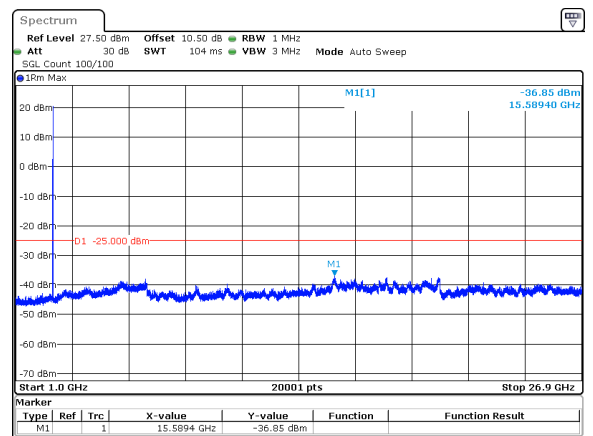
15MHz_15kHz_2682.495MHz_DFT-s-OFDM QPSK_RB1@78&amp;-36.85 dBm
