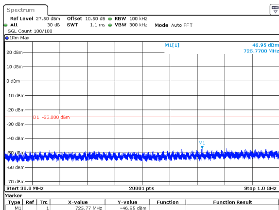
40MHz_30kHz_2592.99MHz_DFT-s-OFDM QPSK_RB100@0&amp;-46.95 dBm
