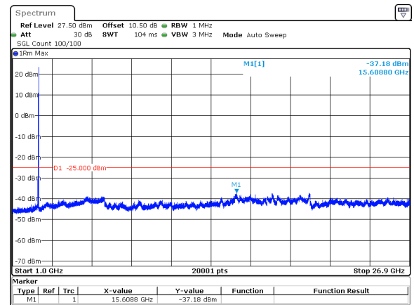
50MHz_15kHz_2664.99MHz_DFT-s-OFDM QPSK_RB1@269&amp;-37.18 dBm
