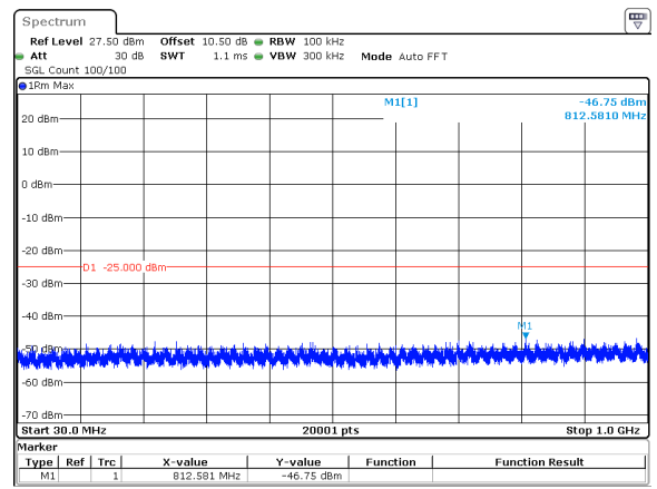
40MHz_30kHz_2516.01MHz_DFT-s-OFDM QPSK_RB1@0&amp;-46.75 dBm
