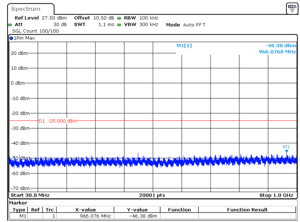
50MHz_15kHz_2664.99MHz_DFT-s-OFDM QPSK_RB1@0&amp;-46.38 dBm
