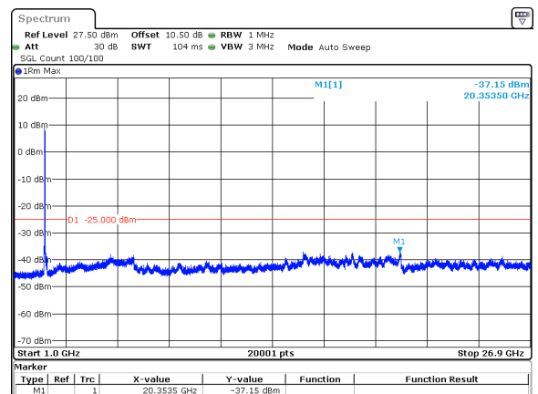
50MHz_15kHz_2521.005MHz_DFT-s-OFDM QPSK_RB270@0&amp;-37.15 dBm
