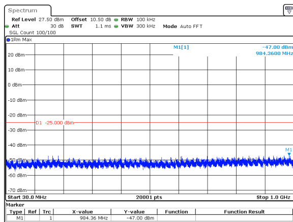
15MHz_15kHz_2682.495MHz_DFT-s-OFDM QPSK_RB1@78&amp;-47.00 dBm
