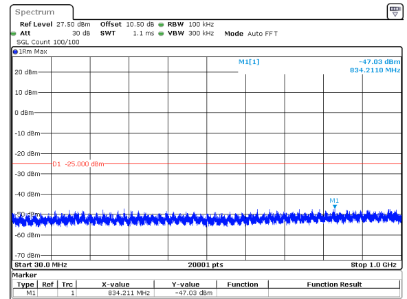
30MHz_15kHz_2511MHz_DFT-s-OFDM QPSK_RB1@159&amp;-47.03 dBm
