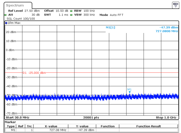
15MHz_30kHz_2503.5MHz_DFT-s-OFDM QPSK_RB1@0&amp;-47.39 dBm
