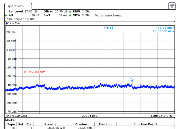
15MHz_30kHz_2592.99MHz_DFT-s-OFDM QPSK_RB36@0&amp;-36.56 dBm
