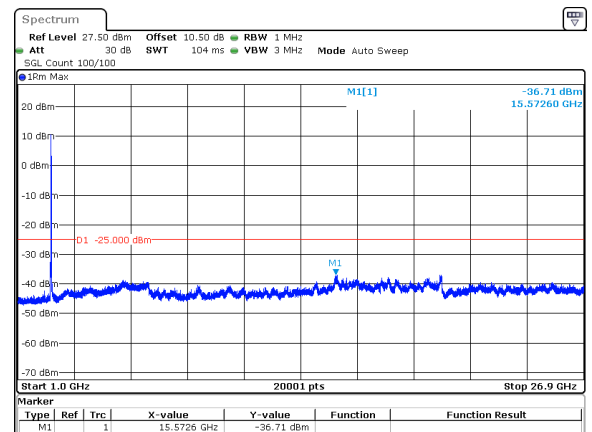
30MHz_15kHz_2511MHz_DFT-s-OFDM QPSK_RB160@0&amp;-36.71 dBm
