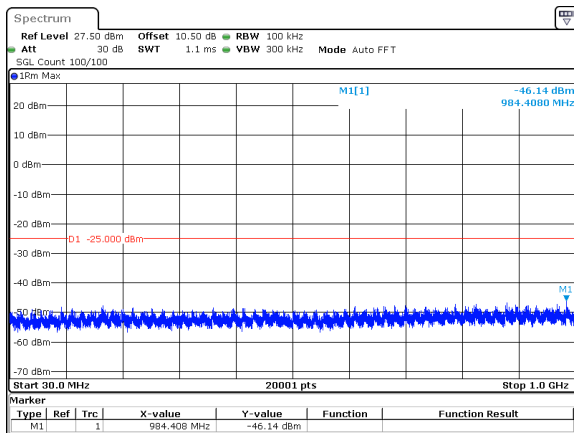
20MHz_15kHz_2506.005MHz_DFT-s-OFDM QPSK_RB100@0&amp;-46.14 dBm
