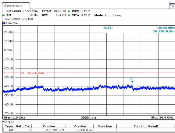
40MHz_30kHz_2516.01MHz_DFT-s-OFDM QPSK_RB1@105&amp;-36.00 dBm
