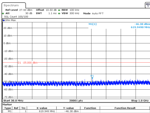
20MHz_15kHz_2679.99MHz_DFT-s-OFDM QPSK_RB100@0&amp;-46.38 dBm
