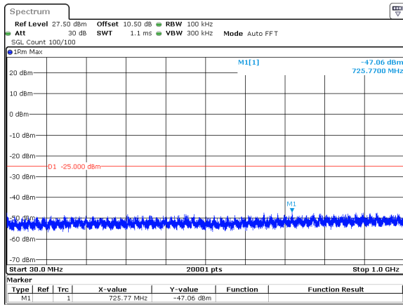
15MHz_30kHz_2682.48MHz_DFT-s-OFDM QPSK_RB1@37&amp;-47.06 dBm
