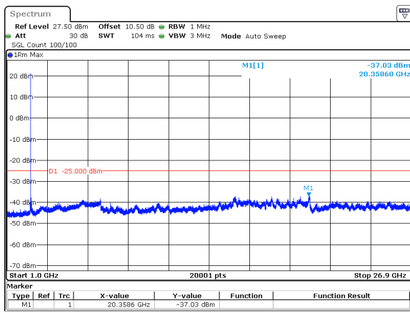
40MHz_30kHz_2516.01MHz_DFT-s-OFDM QPSK_RB1@0&amp;-37.03 dBm
