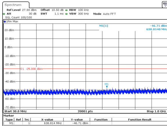
40MHz_15kHz_2670MHz_DFT-s-OFDM QPSK_RB1@0&amp;-46.71 dBm
