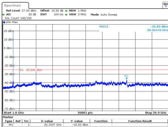
40MHz_30kHz_2592.99MHz_DFT-s-OFDM QPSK_RB1@105&amp;-35.83 dBm
