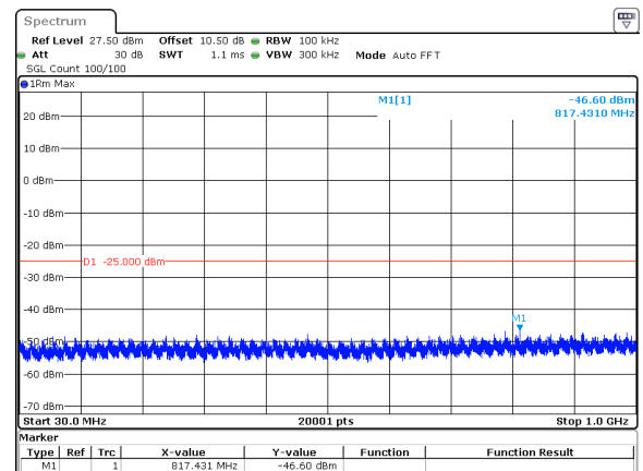
30MHz_30kHz_2511MHz_DFT-s-OFDM QPSK_RB75@0&amp;-46.60 dBm
