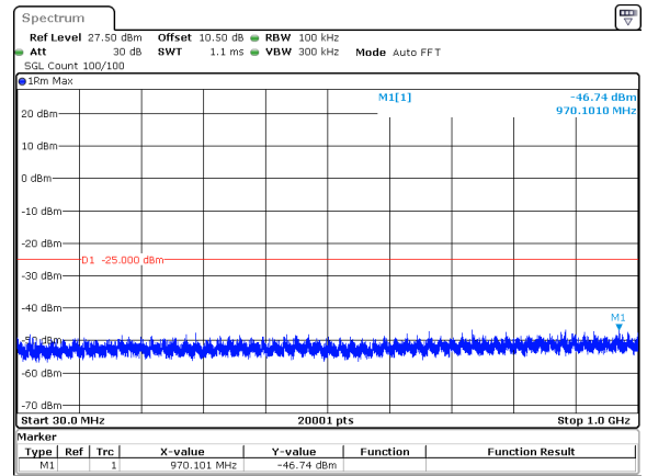
50MHz_15kHz_2593.005MHz_DFT-s-OFDM QPSK_RB1@269&amp;-46.74 dBm
