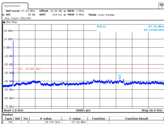
50MHz_30kHz_2664.99MHz_DFT-s-OFDM QPSK_RB128@0&amp;-37.18 dBm
