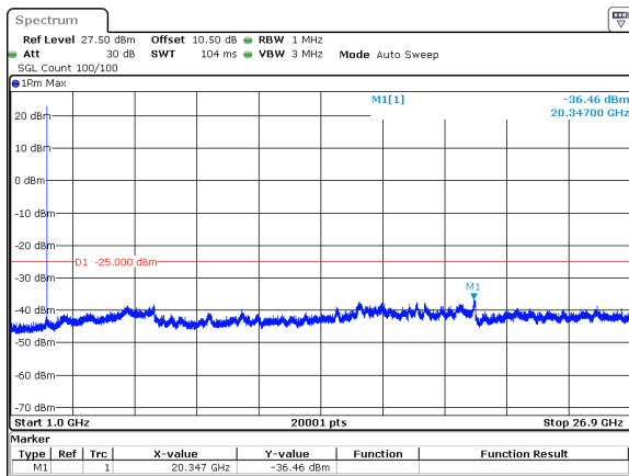
15MHz_30kHz_2503.5MHz_DFT-s-OFDM QPSK_RB1@37&amp;-36.46 dBm
