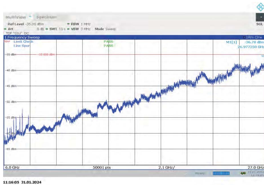
Spurious Emissions (6GHz – 27GHz) – 256QAM (1962.5MHz) (Band 25 E-UTRA 20MHz Channel BW)
