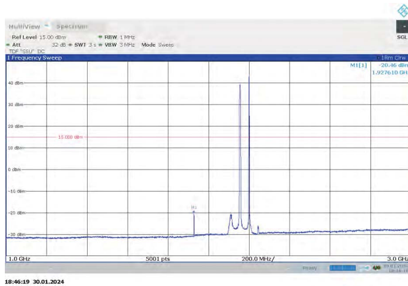
Spurious Emissions (1GHz – 3GHz) - QPSK (2199.8 MHz) (Band 66 NB-IoT SA 200kHz Channel BW)
