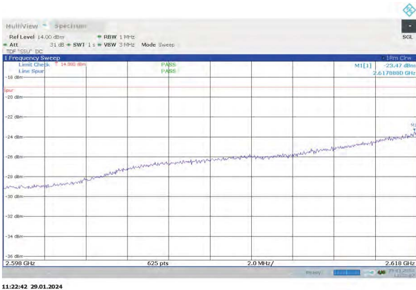
Spurious Emissions (Lower Band Edge 2598-2618MHz) – QPSK (2625 MHz) (Band 7 NB-IoT GB 10MHz Channel BW)
