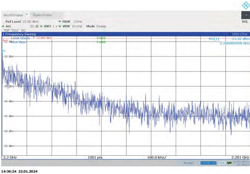
Spurious Emissions (Upper Band Edge 2200-2201MHz) – QPSK (2199.8 MHz) (Band 66 NB-IoT SA 200kHz Channel BW)
