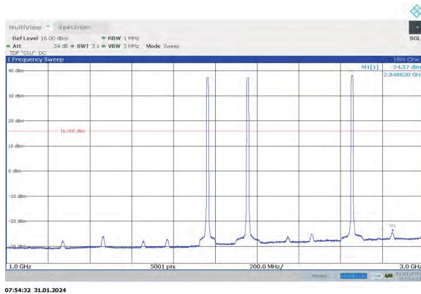
Spurious Emissions (1GHz - 3GHz) - QPSK (2655 MHz) (Band 7 NB-IoT GB 10MHz Channel BW)
