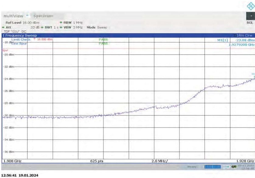
Spurious Emissions (Lower Band Edge 1908-1928MHz) – 256QAM (1940 MHz) (Band 25 E-UTRA 20MHz Channel BW)
