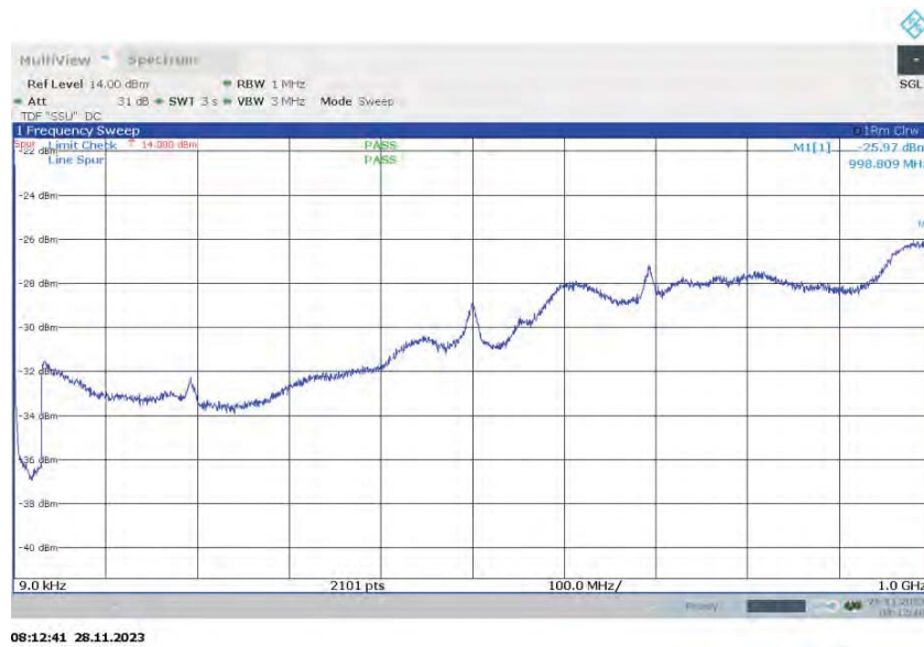
Spurious Emissions (9kHz - 1GHz) - QPSK (2655 MHz) (Band 7 NB-IoT GB 10MHz Channel BW)
