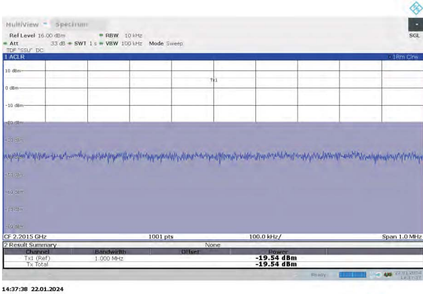
Spurious Emissions (Upper Band Edge 2201-2202MHz) – QPSK (2199.8 MHz) (Band 66 NB-IoT SA 200kHz Channel BW)
