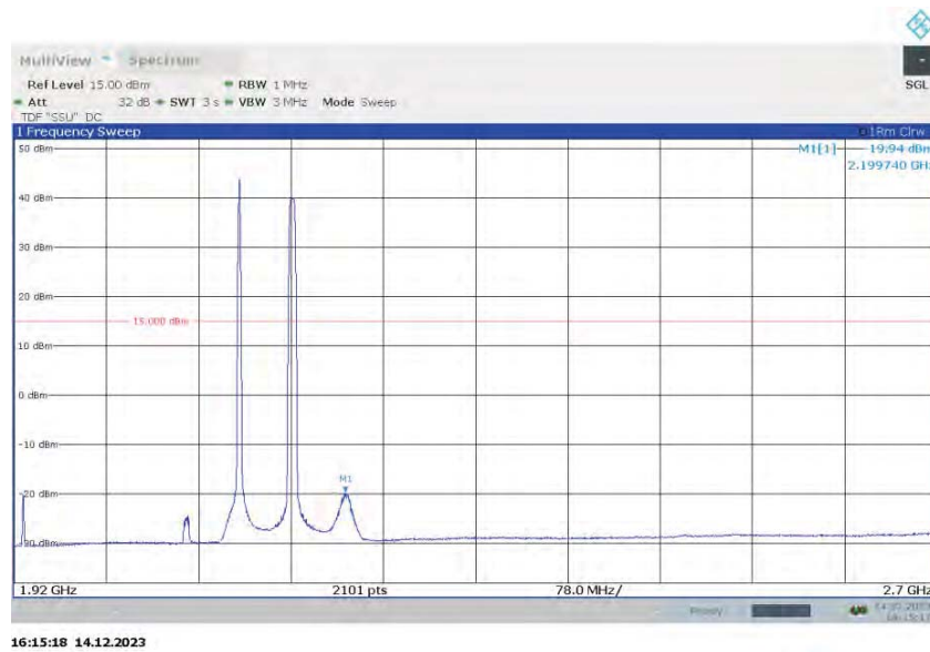
Spurious Emissions (1.92GHz – 2.7GHz) - QPSK (2110.2 MHz) (Band 66 NB-IoT SA 200kHz Channel BW)
