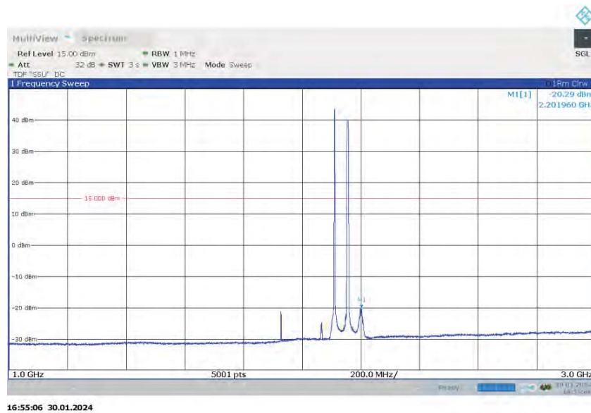
Spurious Emissions (1GHz – 3GHz) - QPSK (2110.2 MHz) (Band 66 NB-IoT SA 200kHz Channel BW)
