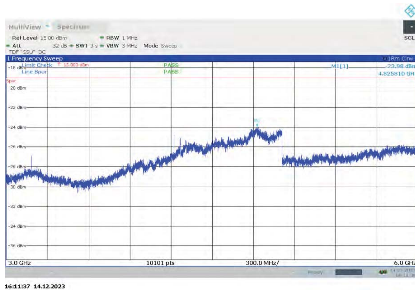
Spurious Emissions (3GHz – 6GHz) - QPSK (2110.2 MHz) (Band 66 NB-IoT SA 200kHz Channel BW)
