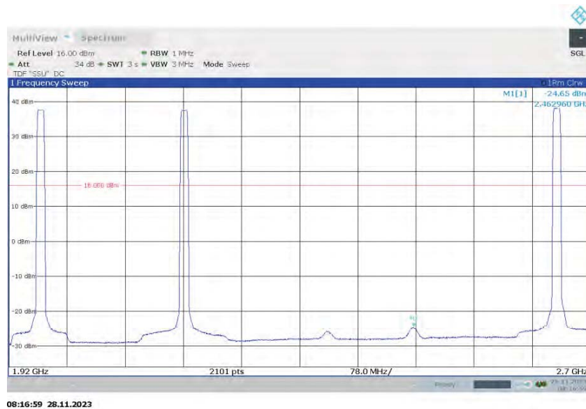
Spurious Emissions (1.92GHz - 2.7GHz) - QPSK (2655 MHz) (Band 7 NB-IoT GB 10MHz Channel BW)
