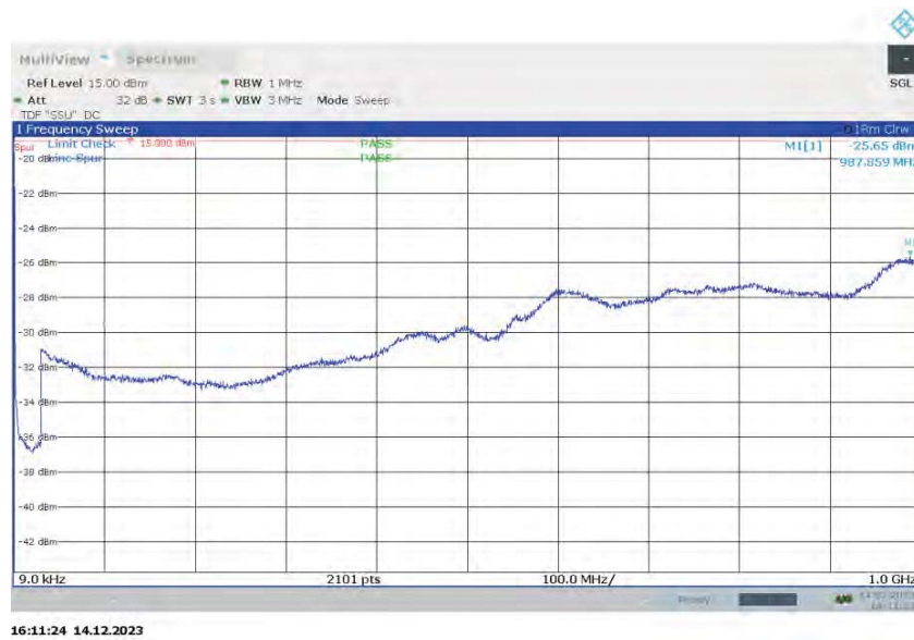
Spurious Emissions (9kHz - 1GHz) - QPSK (2110.2 MHz) (Band 66 NB-IoT SA 200kHz Channel BW)
