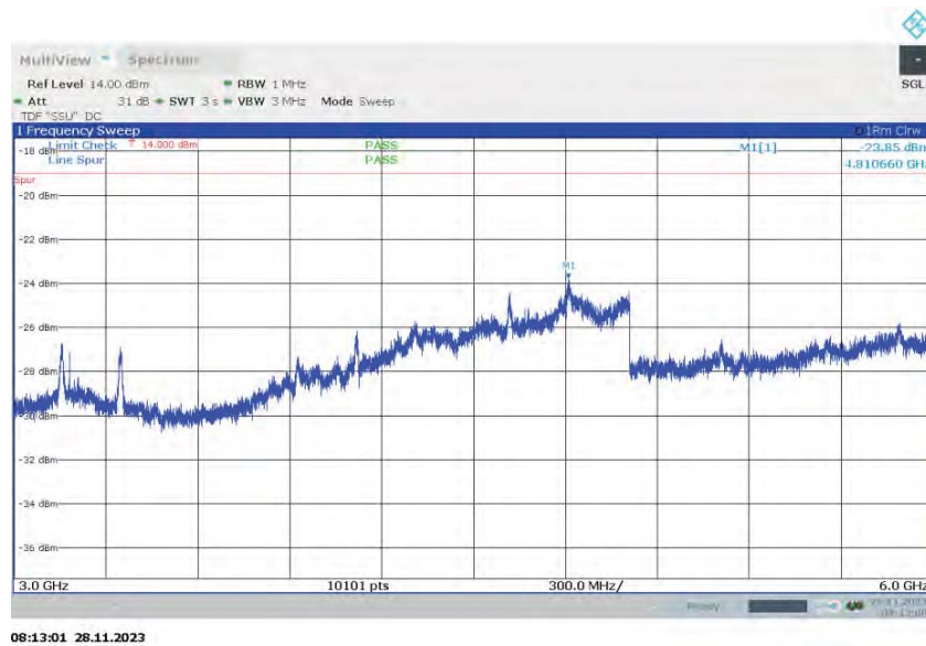
Spurious Emissions (3GHz - 6GHz) - QPSK (2655 MHz) (Band 7 NB-IoT GB 10MHz Channel BW)
