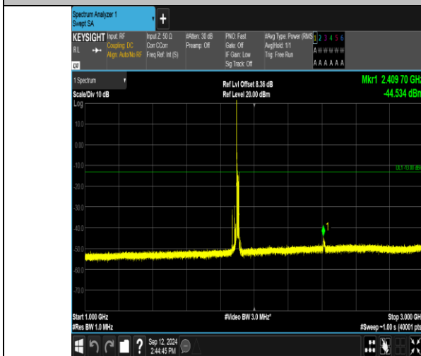
Band2_15MHz_16QAM_19125_1RB#0_1000~3000_1000~3000
