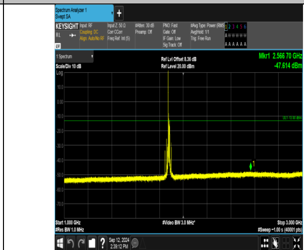
Band2_15MHz_QPSK_18900_1RB#0_1000~3000_1000~3000
