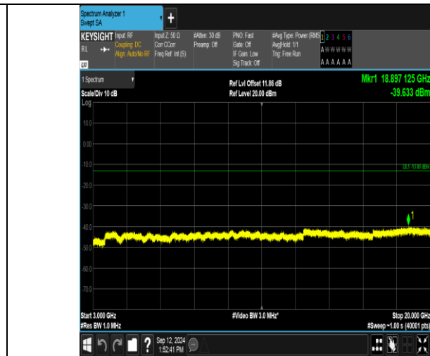
Band2_10MHz_16QAM_19150_1RB#49_3000~20000_3000~20000
