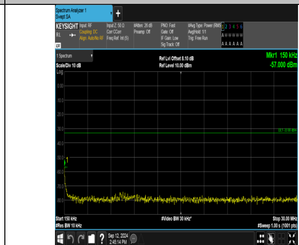
Band2_15MHz_QPSK_19125_1RB#74_0.15~30_0.15~30
