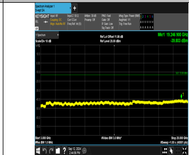
Band2_15MHz_16QAM_19125_1RB#0_3000~20000_3000~20000
