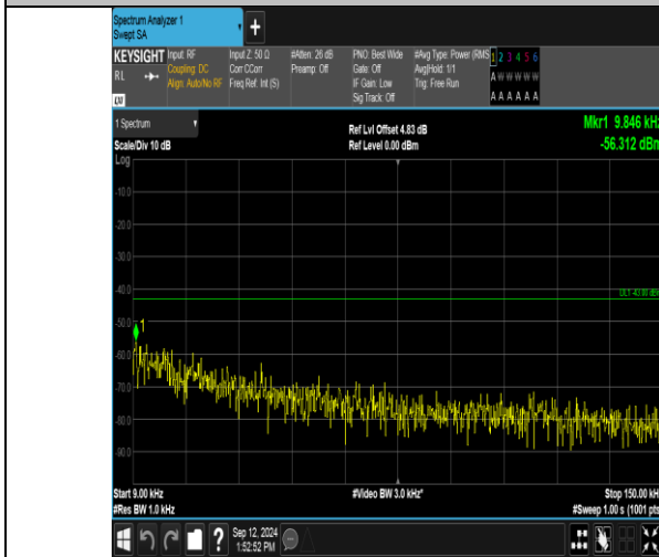
Band2_10MHz_QPSK_19150_50RB#0_0.009~0.15_0.009~0.15
