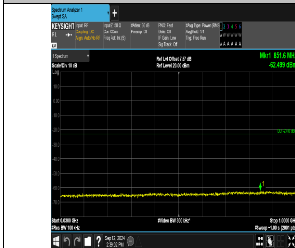
Band2_15MHz_QPSK_18900_1RB#0_30~1000_30~1000
