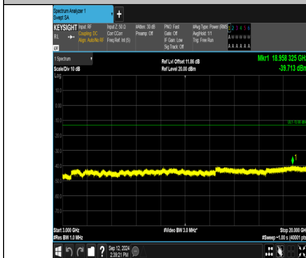
Band2_15MHz_QPSK_18900_1RB#0_3000~20000_3000~20000
