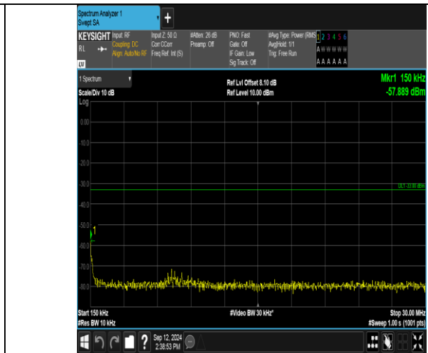
Band2_15MHz_QPSK_18900_1RB#0_0.15~30_0.15~30
