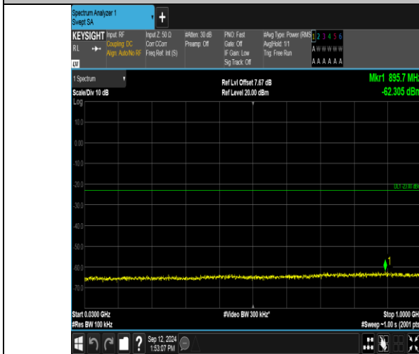
Band2_10MHz_QPSK_19150_50RB#0_30~1000_30~1000
