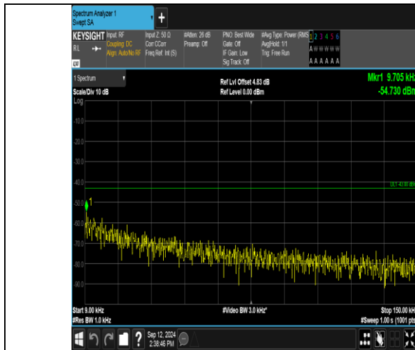
Band2_15MHz_QPSK_18900_1RB#0_0.009~0.15_0.009~0.15
