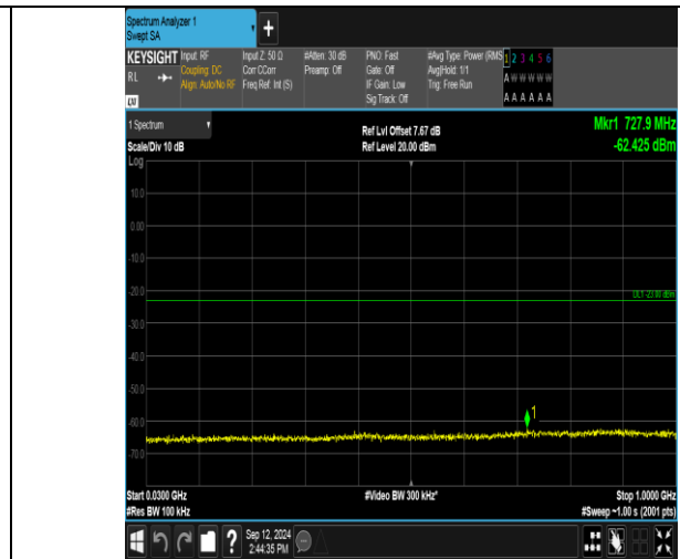
Band2_15MHz_16QAM_19125_1RB#0_30~1000_30~1000
