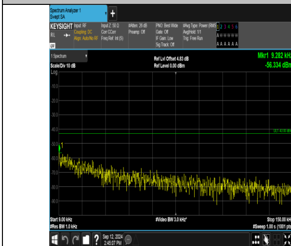
Band2_15MHz_QPSK_19125_1RB#74_0.009~0.15_0.009~0.15
