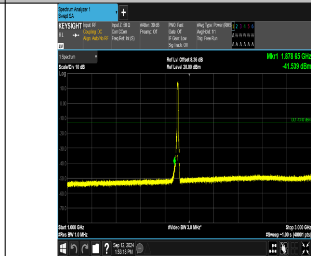
Band2_10MHz_QPSK_19150_50RB#0_1000~3000_1000~3000
