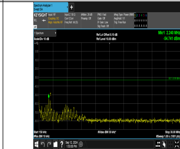
Band2_10MHz_QPSK_19150_50RB#0_0.15~30_0.15~30
