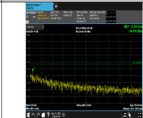
Band2_15MHz_16QAM_18900_1RB#0_0.009~0.15_0.009~0.15
