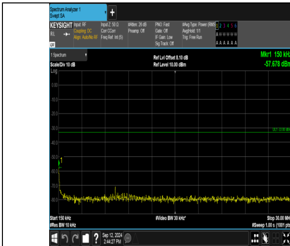
Band2_15MHz_16QAM_19125_1RB#0_0.15~30_0.15~30
