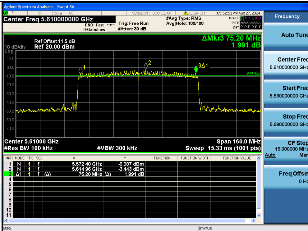
11AX80MIMO-Ant3-5610-PASS
