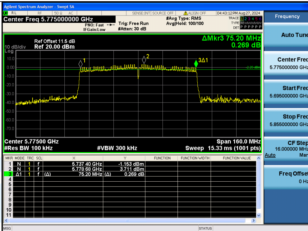
11AC80MIMO-Ant3-5775-PASS
