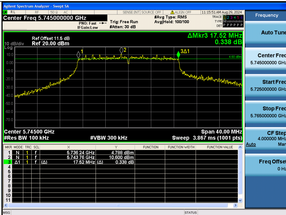
11AC20MIMO-Ant3-5745-PASS
