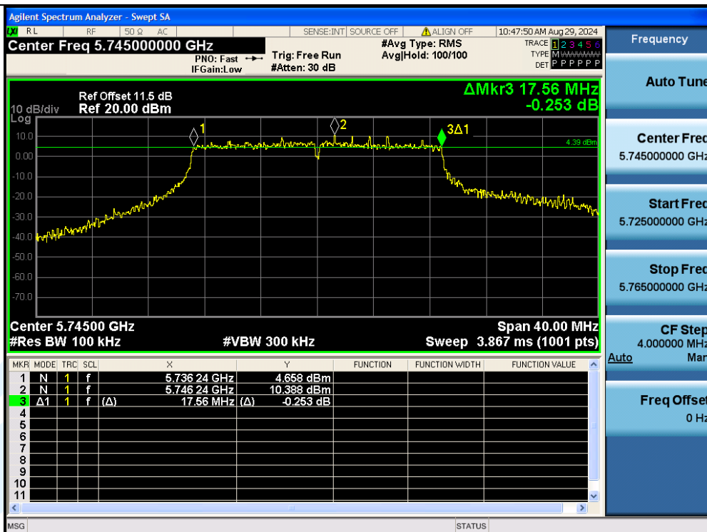
11N20MIMO-Ant3-5745-PASS
