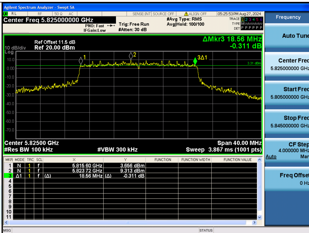
11AX20MIMO-Ant3-5825-PASS
