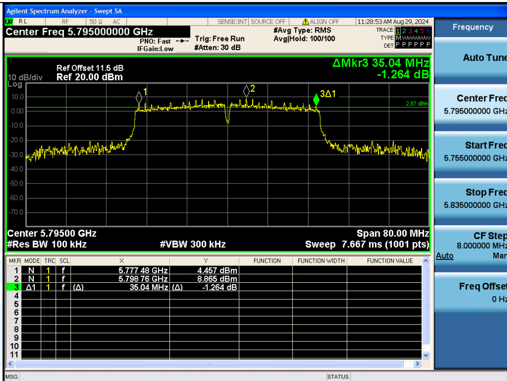
11AC40MIMO-Ant3-5795-PASS
