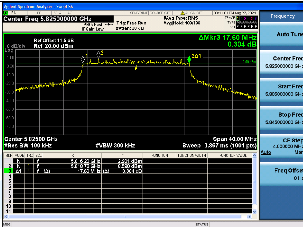
11N20MIMO-Ant3-5825-PASS
