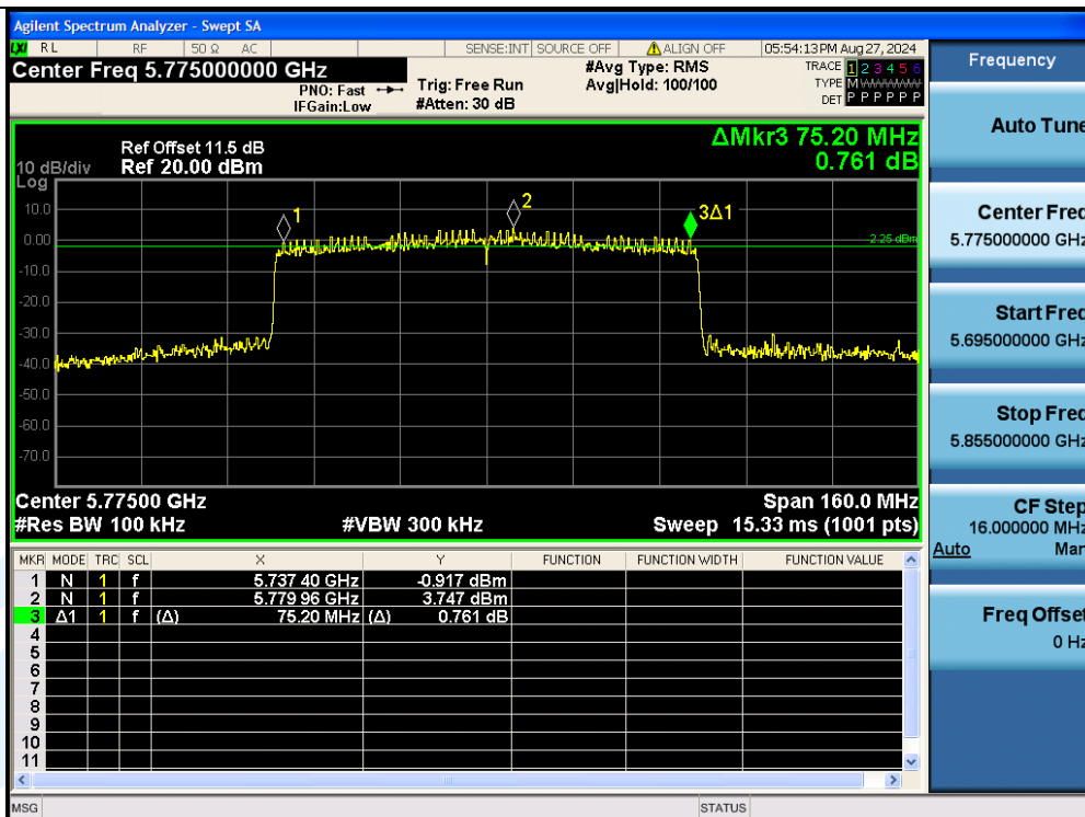
11AX80MIMO-Ant3-5775-PASS
