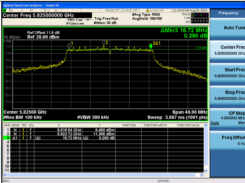
11AC20MIMO-Ant3-5825-PASS
