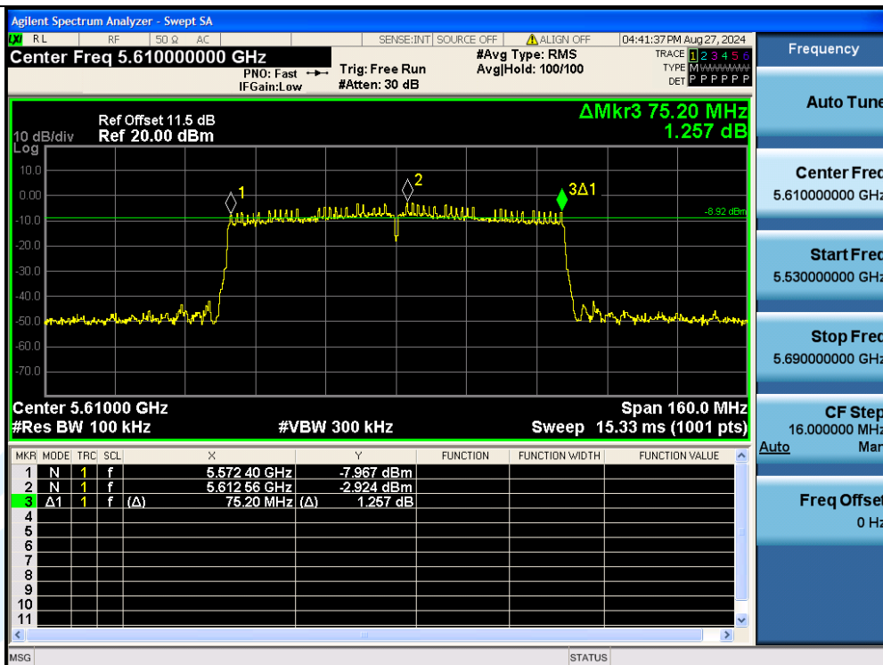
11AC80MIMO-Ant3-5610-PASS
