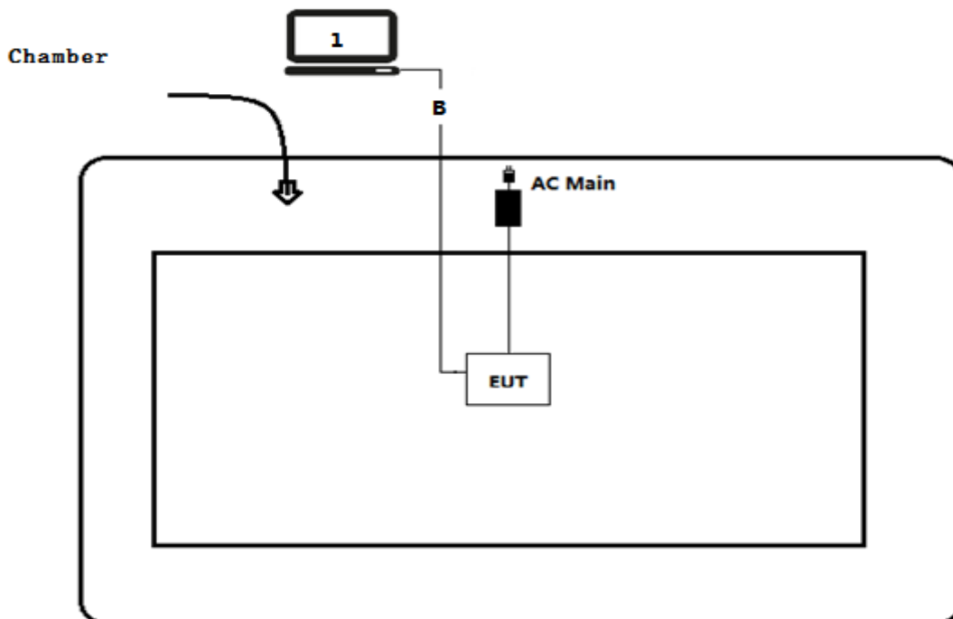
Test setup Diagram- Radiated Emission
