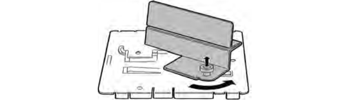
Figure 5 Attaching the adapter to the main bracket
