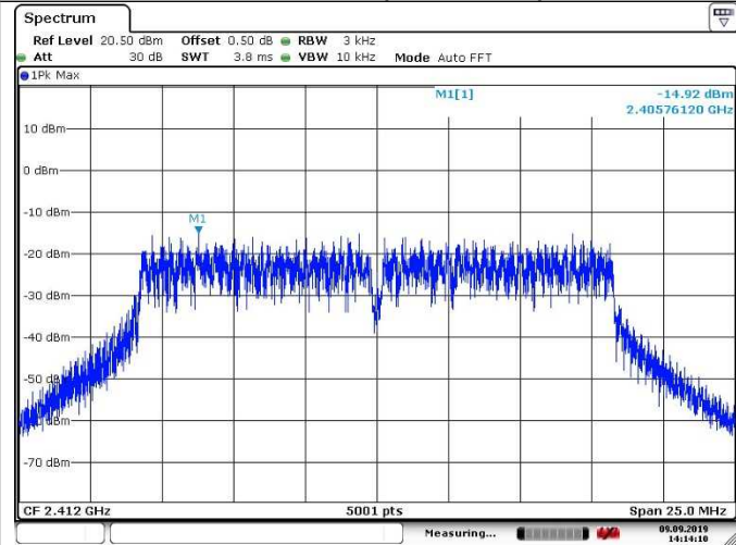
Channel 01 (2412MHz)
