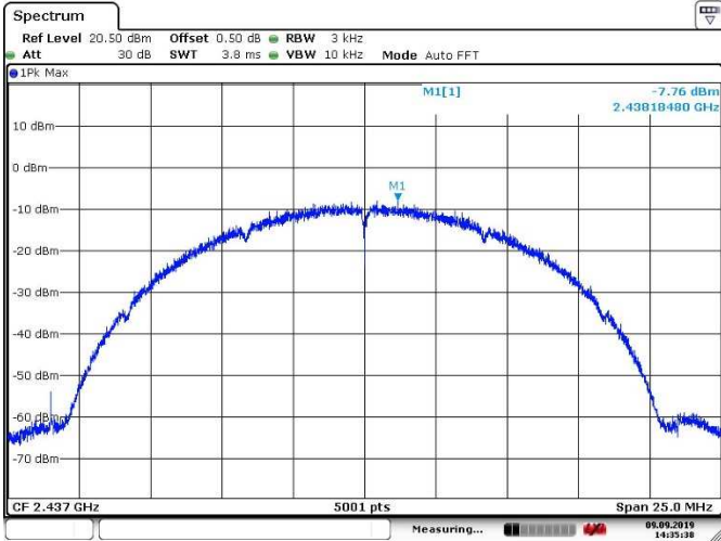
Channel 06 (2437MHz)
