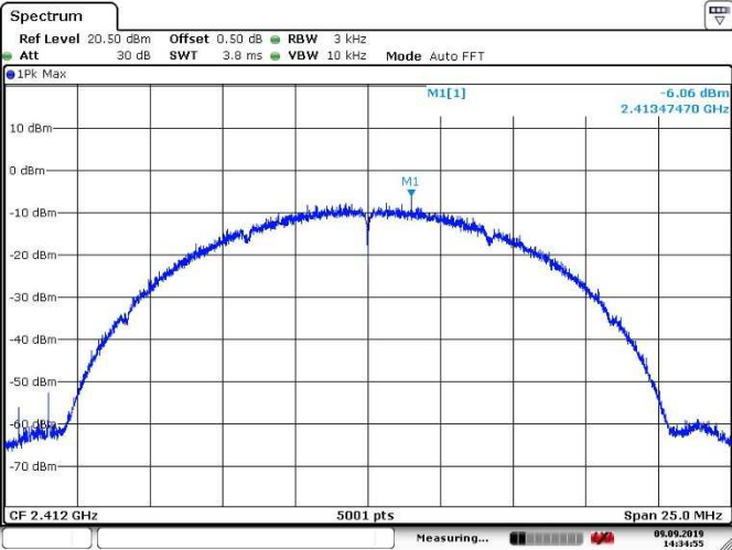
Channel 01 (2412MHz)
