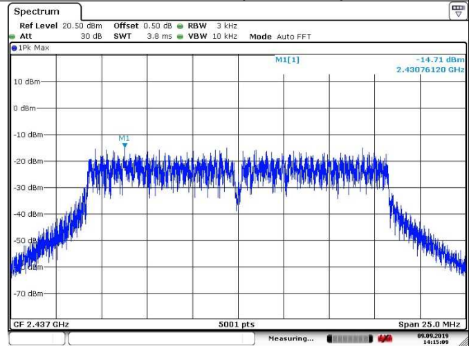
Channel 06 (2437MHz)
