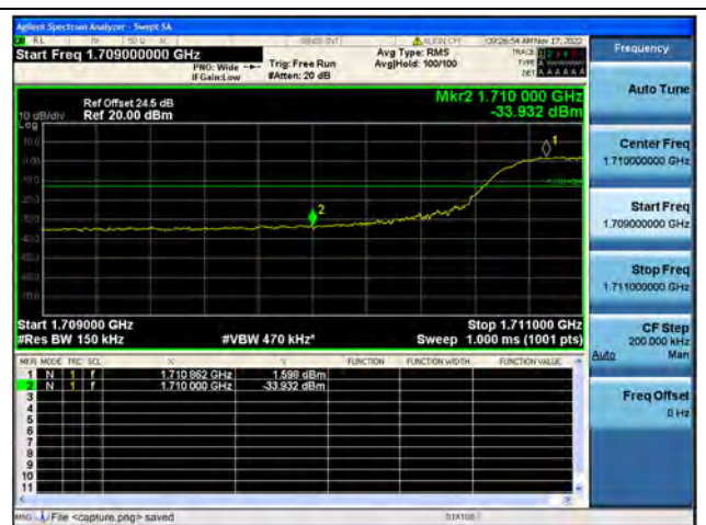
Band66 / 15MHz / Low CH / QPSK / FULL RB
