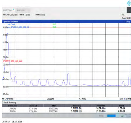
1-N66-PC3-15-40-L-4-CP-QPSK-Edge_1RB_Left-1@0-Ant3-1-seegraph-PASS-see graph
