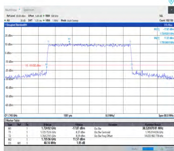
1-N66-PC3-15-40-M-6-CP-QPSK-Outer_Full-216@0 -Ant3-38.521-40.160-≤40-PASS
