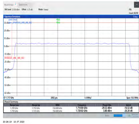
1-N66-PC3-15-15-L-3-DFT-PI2BPSK-Outer_Full-75@0-Ant3-1-seegraph-PASS-see graph
