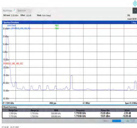
1-N66-PC3-15-40-L-4-CP-QPSK-Edge_1RB_Left-1@0-Ant3-1-seegraph-PASS-see graph
