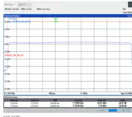
1-N66-PC3-15-40-L-3-DFT-PI2BPSK-Outer_Full-216@0-Ant3-1-seegraph-PASS-see graph
