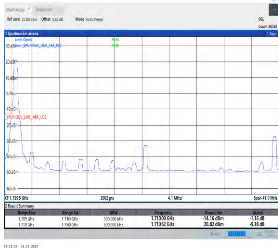
1-N66-PC3-15-40-L-1-DFT-PI2BPSK-Edge_1RB_Left-1@0-Ant3-1-seegraph-PASS-see graph
