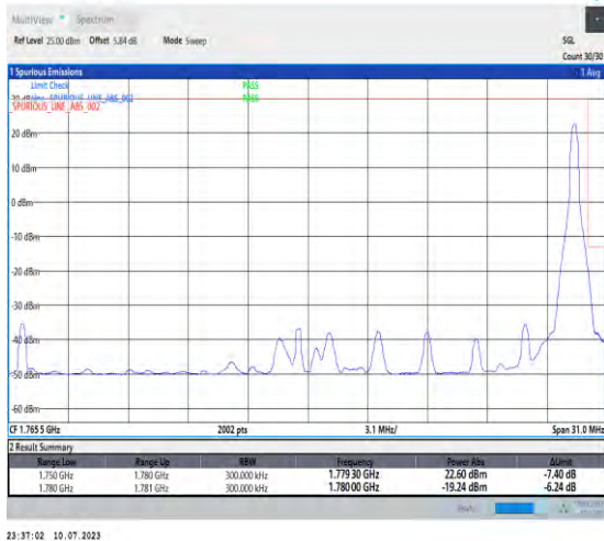
1-N66-PC3-15-30-H-2-DFT-PI2BPSK-Edge_1RB_Right-t-1@159-Ant3-1-seegraph-PASS-see graph
