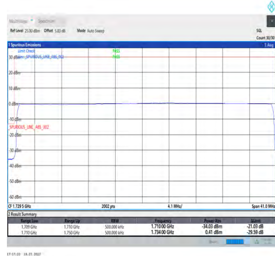
1-N66-PC3-15-40-L-6-CP-QPSK-Outer_Full-216@0-Ant3-1-seegraph-PASS-see graph
