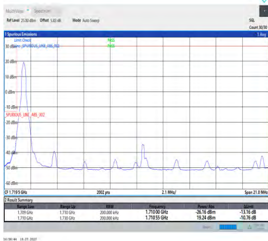
1-N66-PC3-15-20-L-4-CP-QPSK-Edge_1RB_Left-1@0-Ant3-1-seegraph-PASS-see graph
