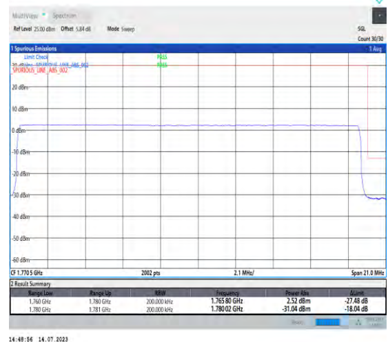
1-N66-PC3-15-20-H-6-CP-QPSK-Outer_Full-106@0-Ant3-1-seegraph-PASS-see graph
