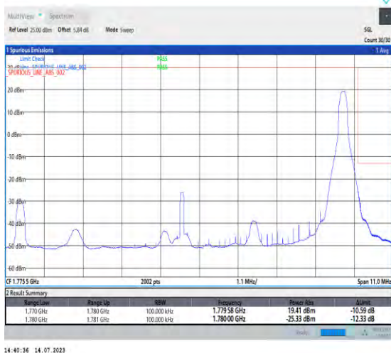
1-N66-PC3-15-10-H-5-CP-QPSK-Edge_1RB_Right-1@51-Ant3-1-seegraph-PASS-see graph
