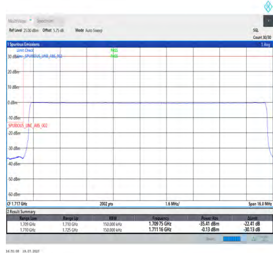
1-N66-PC3-15-15-L-6-CP-QPSK-Outer_Full-79@0-Ant3-1-seegraph-PASS-see graph
