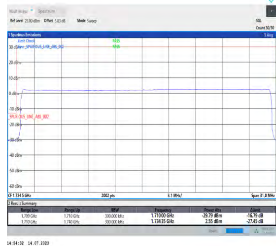
1-N66-PC3-15-30-L-6-CP-QPSK-Outer_Full-160@0-Ant3-1-seegraph-PASS-see graph
