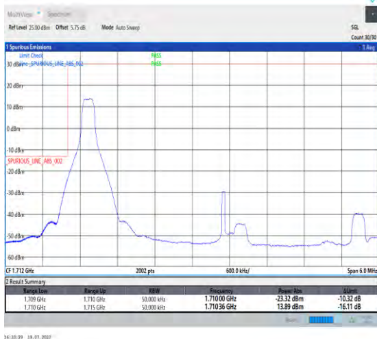
1-N66-PC3-15-5-L-4-CP-QPSK-Edge_1RB_Left-1@0- Ant3-1-seegraph-PASS-see graph
