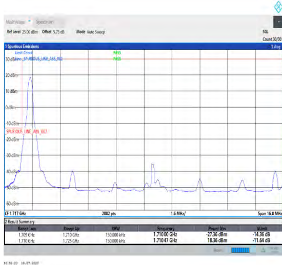
1-N66-PC3-15-15-L-4-CP-QPSK-Edge_1RB_Left-1@0-Ant3-1-seegraph-PASS-see graph
