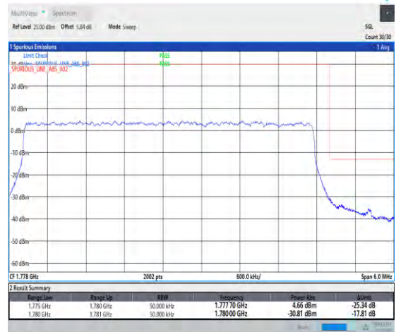
1-N66-PC3-15-5-H-3-DFT-PI2BPSK-Outer_Full-25@0-Ant3-1-seegraph-PASS-see graph
