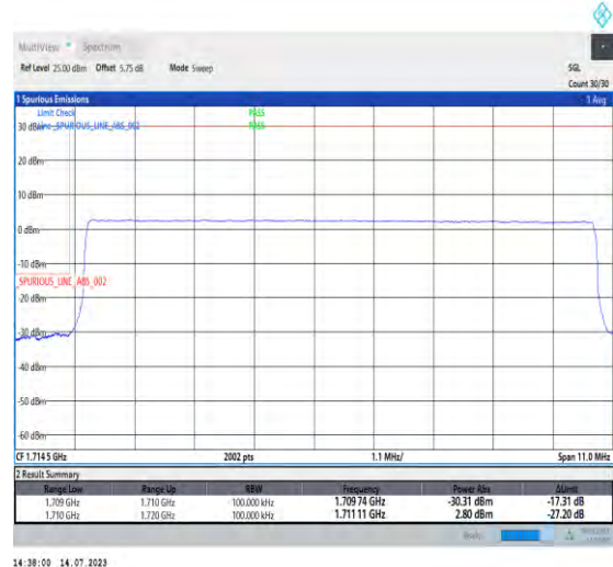
1-N66-PC3-15-10-L-6-CP-QPSK-Outer_Full-52@0-Ant3-1-seegraph-PASS-see graph
