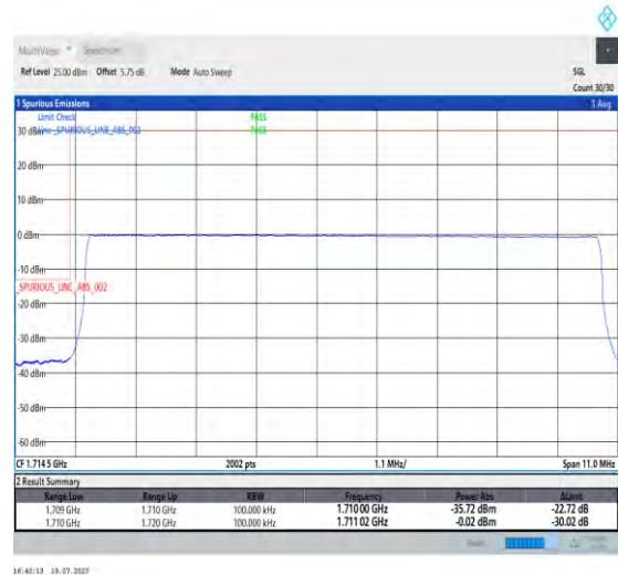
1-N66-PC3-15-10-L-6-CP-QPSK-Outer_Full-52@0-Ant3-1-seegraph-PASS-see graph
