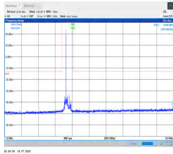
1-N66-PC3-15-40-M-1-DFT-PI2BPSK-Inner_1RB_Lef t-1@1-1000-3000-Ant3-2991.50--44.68--13-PASS
