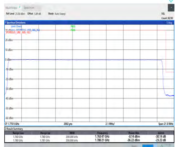
1-N66-PC3-15-20-H-6-CP-QPSK-Outer_Full-106@0-Ant3-1-seegraph-PASS-see graph
