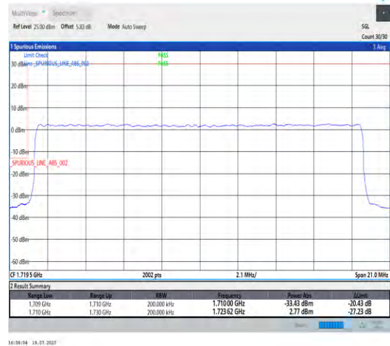
1-N66-PC3-15-20-L-3-DFT-PI2BPSK-Outer_Full-100@0-Ant3-1-seegraph-PASS-see graph
