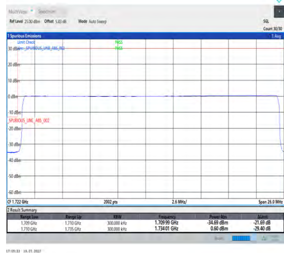
1-N66-PC3-15-25-L-6-CP-QPSK-Outer_Full-133@0-Ant3-1-seegraph-PASS-see graph
