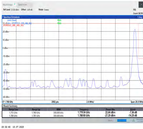
1-N66-PC3-15-25-H-2-DFT-PI2BPSK-Edge_1RB_Right-t-1@132-Ant3-1-seegraph-PASS-see graph
