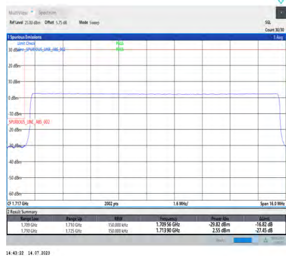
1-N66-PC3-15-15-L-6-CP-QPSK-Outer_Full-79@0-Ant3-1-seegraph-PASS-see graph
