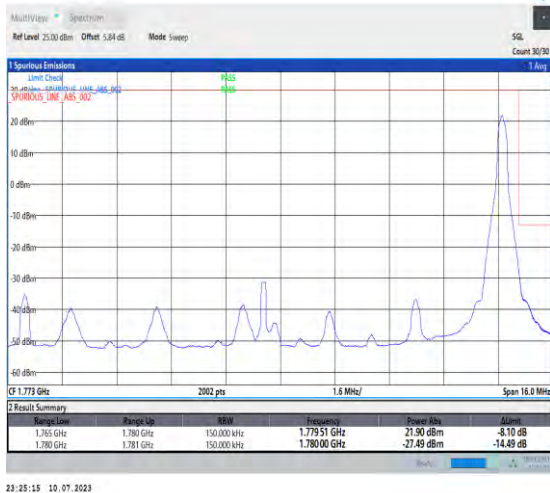
1-N66-PC3-15-15-H-2-DFT-PI2BPSK-Edge_1RB_Right-1@78-Ant3-1-seegraph-PASS-see graph
