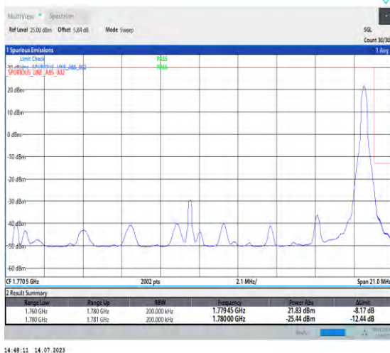
1-N66-PC3-15-20-H-5-CP-QPSK-Edge_1RB_Right-1@105-Ant3-1-seegraph-PASS-see graph
