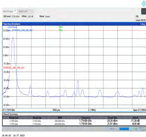
1-N66-PC3-15-20-L-4-CP-QPSK-Edge_1RB_Left-1@0-Ant3-1-seegraph-PASS-see graph
