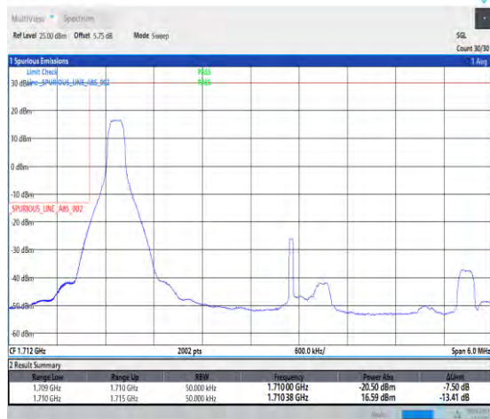
1-N66-PC3-15-5-L-4-CP-QPSK-Edge_1RB_Left-1@0-Ant3-1-seegraph-PASS-see graph
