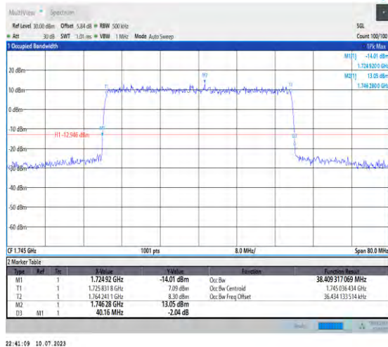
1-N66-PC3-15-40-M-3-DFT-16QAM-Outer_Full-216 @0-Ant3-38.409-40.160-≤40-PASS
