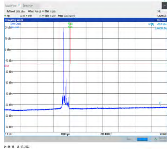
1-N66-PC3-15-40-M-1-DFT-PI2BPSK-Inner_1RB_Lef t-1@1-1000-3000-Ant3-2908.20--44.68--13-PASS
