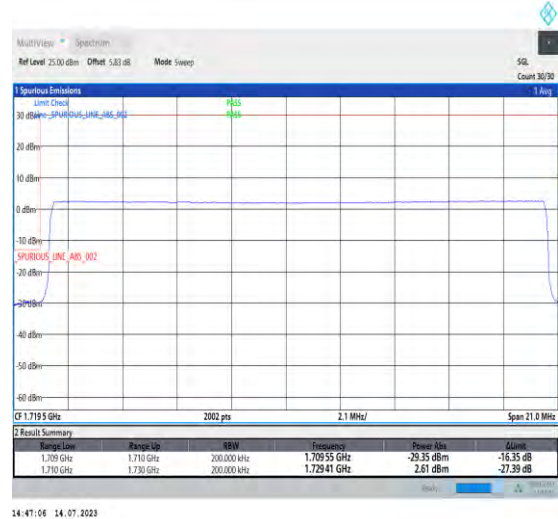
1-N66-PC3-15-20-L-6-CP-QPSK-Outer_Full-106@0-Ant3-1-seegraph-PASS-see graph
