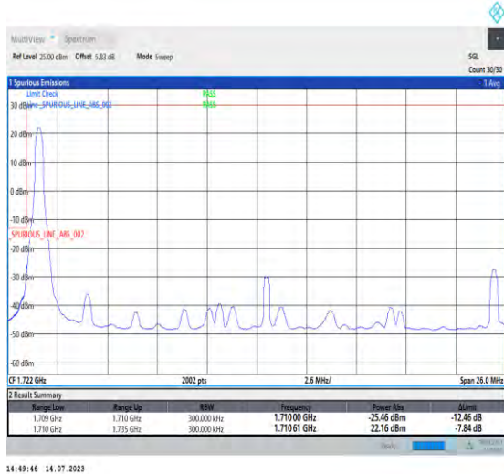
1-N66-PC3-15-25-L-4-CP-QPSK-Edge_1RB_Left-1@0-Ant3-1-seegraph-PASS-see graph
