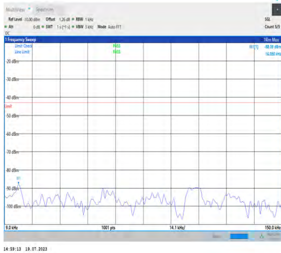
1-N66-PC3-15-40-H-1-DFT-PI2BPSK-Inner_1RB_Lef t-1@1-0.009-0.15-Ant3-16.050--88.09--43-PASS
