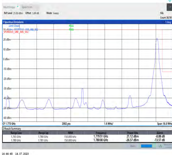
1-N66-PC3-15-15-H-5-CP-QPSK-Edge_1RB_Right-1@78-Ant3-1-seegraph-PASS-see graph
