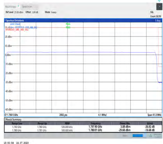
1-N66-PC3-15-40-H-6-CP-QPSK-Outer_Full-216@0-Ant3-1-seegraph-PASS-see graph
