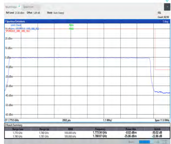
1-N66-PC3-15-10-H-6-CP-QPSK-Outer_Full-52@0-Ant3-1-seegraph-PASS-see graph
