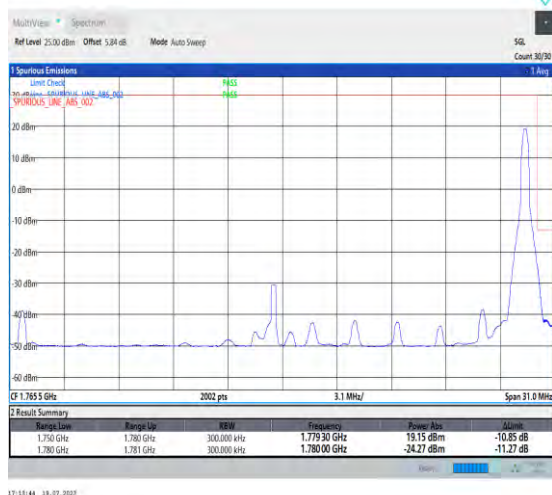
1-N66-PC3-15-30-H-5-CP-QPSK-Edge_1RB_Right-1@159-Ant3-1-seegraph-PASS-see graph
