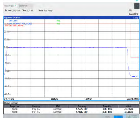
1-N66-PC3-15-15-H-6-CP-QPSK-Outer_Full-79@0-Ant3-1-seegraph-PASS-see graph
