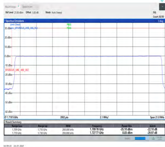
1-N66-PC3-15-20-L-6-CP-QPSK-Outer_Full-106@0-Ant3-1-seegraph-PASS-see graph
