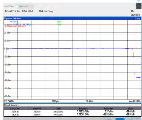
1-N66-PC3-15-25-H-6-CP-QPSK-Outer_Full-133@0-Ant3-1-seegraph-PASS-see graph
