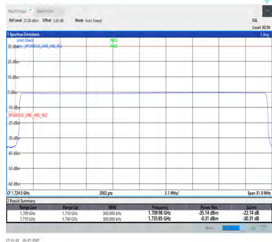
1-N66-PC3-15-30-L-6-CP-QPSK-Outer_Full-160@0-Ant3-1-seegraph-PASS-see graph
