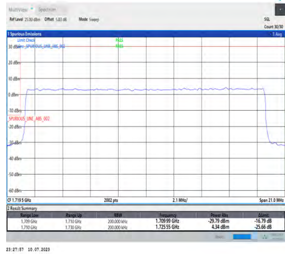
1-N66-PC3-15-20-L-3-DFT-PI2BPSK-Outer_Full-100@0-Ant3-1-seegraph-PASS-see graph
