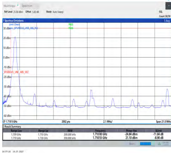
1-N66-PC3-15-20-L-1-DFT-PI2BPSK-Edge_1RB_Left-1@0-Ant3-1-seegraph-PASS-see graph
