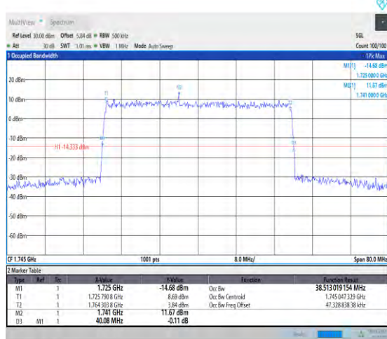
1-N66-PC3-15-40-M-5-DFT-256QAM-Outer_Full-216 @0-Ant3-38.513-40.080-≤40-PASS
