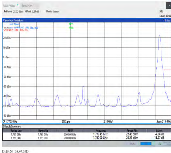
1-N66-PC3-15-20-H-2-DFT-PI2BPSK-Edge_1RB_Right-t-1@105-Ant3-1-seegraph-PASS-see graph
