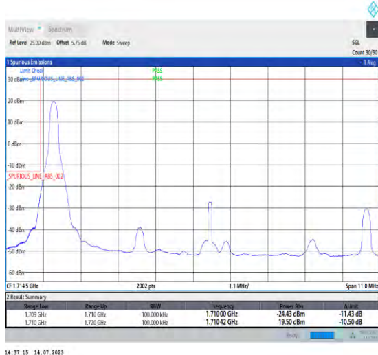
1-N66-PC3-15-10-L-4-CP-QPSK-Edge_1RB_Left-1@0-Ant3-1-seegraph-PASS-see graph
