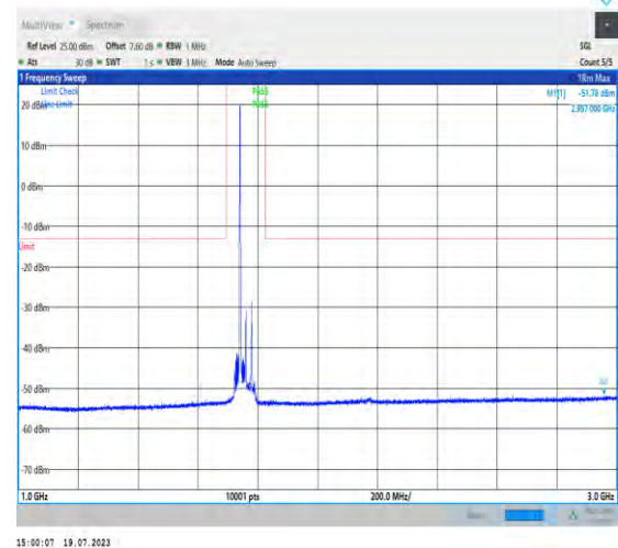
1-N66-PC3-15-40-H-1-DFT-PI2BPSK-Inner_1RB_Lef t-1@1-1000-3000-Ant3-2597.00--51.78--13-PASS
