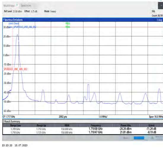
1-N66-PC3-15-15-L-1-DFT-PI2BPSK-Edge_1RB_Left-1@0-Ant3-1-seegraph-PASS-see graph
