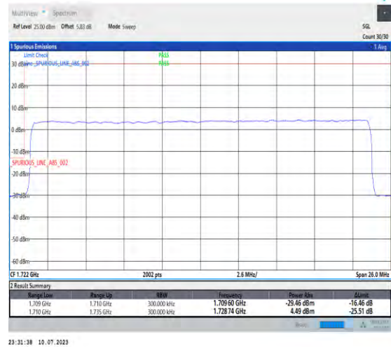
1-N66-PC3-15-25-L-3-DFT-PI2BPSK-Outer_Full-128@0-Ant3-1-seegraph-PASS-see graph
