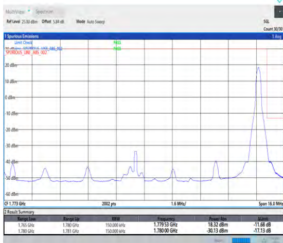
1-N66-PC3-15-15-H-5-CP-QPSK-Edge_1RB_Right-1@78-Ant3-1-seegraph-PASS-see graph
