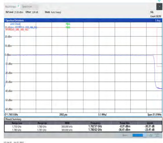
1-N66-PC3-15-30-H-6-CP-QPSK-Outer_Full-160@0-Ant3-1-seegraph-PASS-see graph
