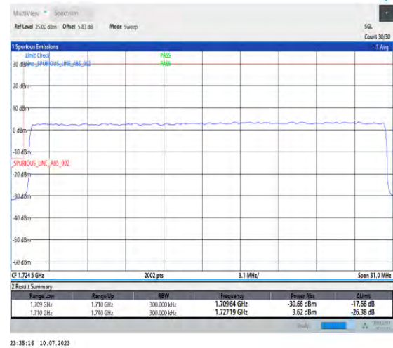
1-N66-PC3-15-30-L-3-DFT-PI2BPSK-Outer_Full-160@0-Ant3-1-seegraph-PASS-see graph
