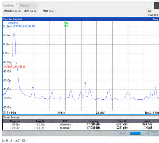
1-N66-PC3-15-20-L-1-DFT-PI2BPSK-Edge_1RB_Left-1@0-Ant3-1-seegraph-PASS-see graph
