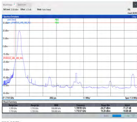
1-N66-PC3-15-10-L-1-DFT-PI2BPSK-Edge_1RB_Left-1@0-Ant3-1-seegraph-PASS-see graph
