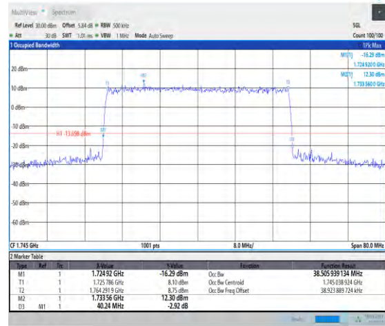
1-N66-PC3-15-40-M-4-DFT-64QAM-Outer_Full-216 @0-Ant3-38.506-40.240-≤40-PASS
