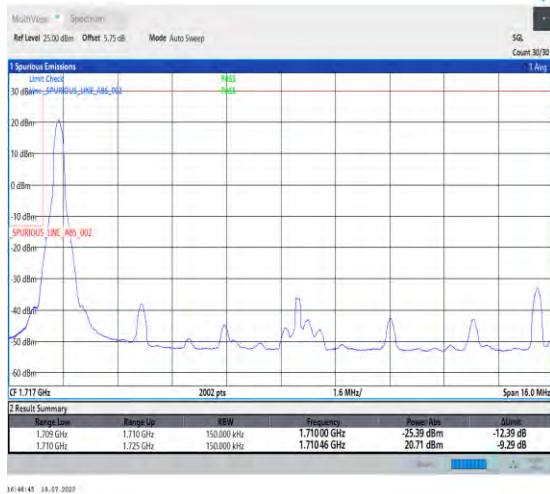
1-N66-PC3-15-15-L-1-DFT-PI2BPSK-Edge_1RB_Left-1@0-Ant3-1-seegraph-PASS-see graph
