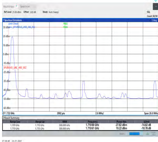
1-N66-PC3-15-25-L-4-CP-QPSK-Edge_1RB_Left-1@0-Ant3-1-seegraph-PASS-see graph
