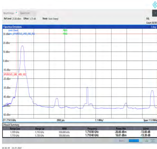
1-N66-PC3-15-10-L-4-CP-QPSK-Edge_1RB_Left-1@0-Ant3-1-seegraph-PASS-see graph
