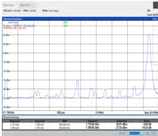
1-N66-PC3-15-25-H-2-DFT-PI2BPSK-Edge_1RB_Right-t-1@132-Ant3-1-seegraph-PASS-see graph
