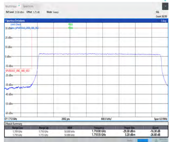
1-N66-PC3-15-5-L-6-CP-QPSK-Outer_Full-25@0-Ant3-1-seegraph-PASS-see graph
