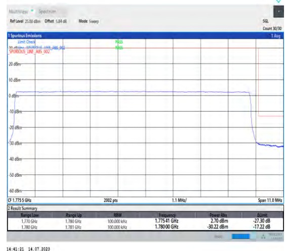
1-N66-PC3-15-10-H-6-CP-QPSK-Outer_Full-52@0-Ant3-1-seegraph-PASS-see graph
