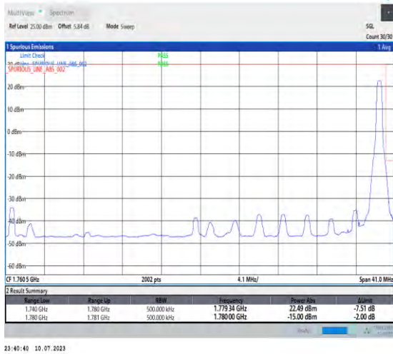
1-N66-PC3-15-40-H-2-DFT-PI2BPSK-Edge_1RB_Right-t-1@215-Ant3-1-seegraph-PASS-see graph
