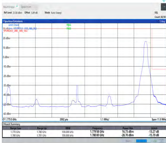
1-N66-PC3-15-10-H-5-CP-QPSK-Edge_1RB_Right-1@51-Ant3-1-seegraph-PASS-see graph
