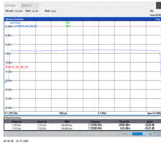
1-N66-PC3-15-40-L-3-DFT-PI2BPSK-Outer_Full-216@0-Ant3-1-seegraph-PASS-see graph
