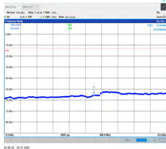
1-N66-PC3-15-40-M-1-DFT-PI2BPSK-Inner_1RB_Lef t-1@1-12000-20000-Ant3-16416.00--51.54--13-PASS
