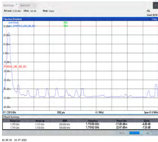
1-N66-PC3-15-40-L-1-DFT-PI2BPSK-Edge_1RB_Left-1@0-Ant3-1-seegraph-PASS-see graph
