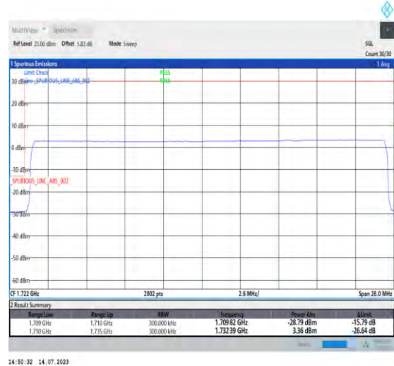
1-N66-PC3-15-25-L-6-CP-QPSK-Outer_Full-133@0-Ant3-1-seegraph-PASS-see graph
