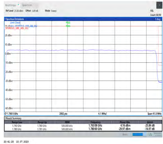
1-N66-PC3-15-40-H-3-DFT-PI2BPSK-Outer_Full-216@0-Ant3-1-seegraph-PASS-see graph
