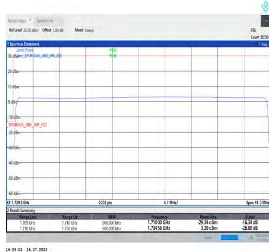
1-N66-PC3-15-40-L-6-CP-QPSK-Outer_Full-216@0-Ant3-1-seegraph-PASS-see graph
