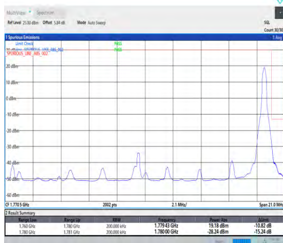
1-N66-PC3-15-20-H-5-CP-QPSK-Edge_1RB_Right-1@105-Ant3-1-seegraph-PASS-see graph
