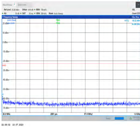
1-N66-PC3-15-40-M-1-DFT-PI2BPSK-Inner_1RB_L eff-1@1-30-1000-Ant3-34.37--59.22--23-PASS
