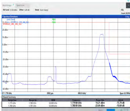
1-N66-PC3-15-5-H-5-CP-QPSK-Edge_1RB_Right-1@24-Ant3-1-seegraph-PASS-see graph
