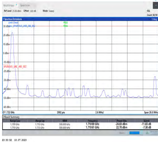
1-N66-PC3-15-25-L-1-DFT-PI2BPSK-Edge_1RB_Left-1@0-Ant3-1-seegraph-PASS-see graph
