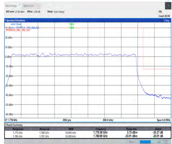
1-N66-PC3-15-5-H-3-DFT-PI2BPSK-Outer_Full-25@0-Ant3-1-seegraph-PASS-see graph
