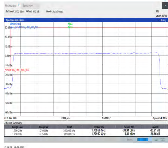
1-N66-PC3-15-25-L-3-DFT-PI2BPSK-Outer_Full-128@0-Ant3-1-seegraph-PASS-see graph
