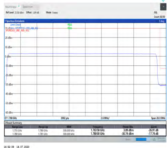
1-N66-PC3-15-25-H-6-CP-QPSK-Outer_Full-133@0-Ant3-1-seegraph-PASS-see graph
