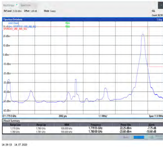
1-N66-PC3-15-10-H-2-DFT-PI2BPSK-Edge_1RB_Right-t-1@51-Ant3-1-seegraph-PASS-see graph
