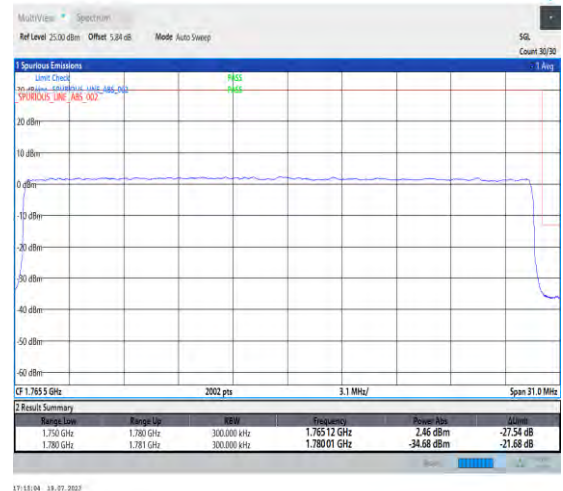
1-N66-PC3-15-30-H-3-DFT-PI2BPSK-Outer_Full-160@0-Ant3-1-seegraph-PASS-see graph
