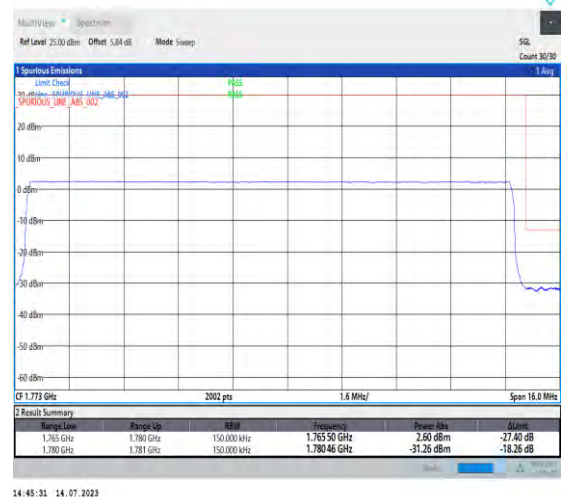
1-N66-PC3-15-15-H-6-CP-QPSK-Outer_Full-79@0-Ant3-1-seegraph-PASS-see graph
