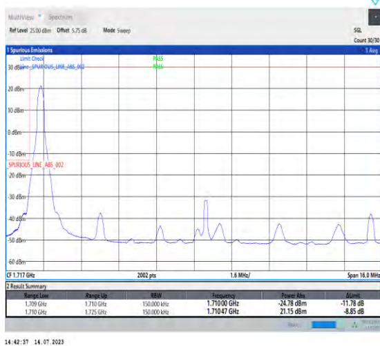
1-N66-PC3-15-15-L-4-CP-QPSK-Edge_1RB_Left-1@0-Ant3-1-seegraph-PASS-see graph
