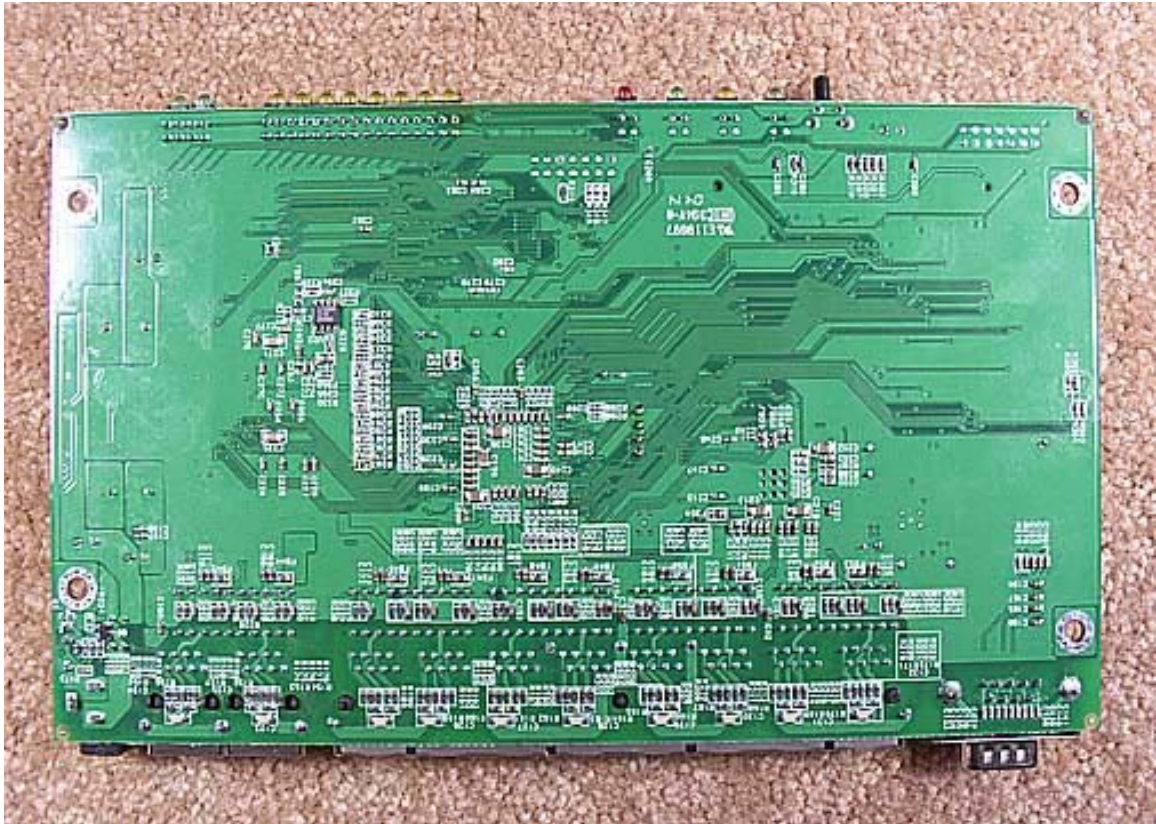
Main PCB Bottom
