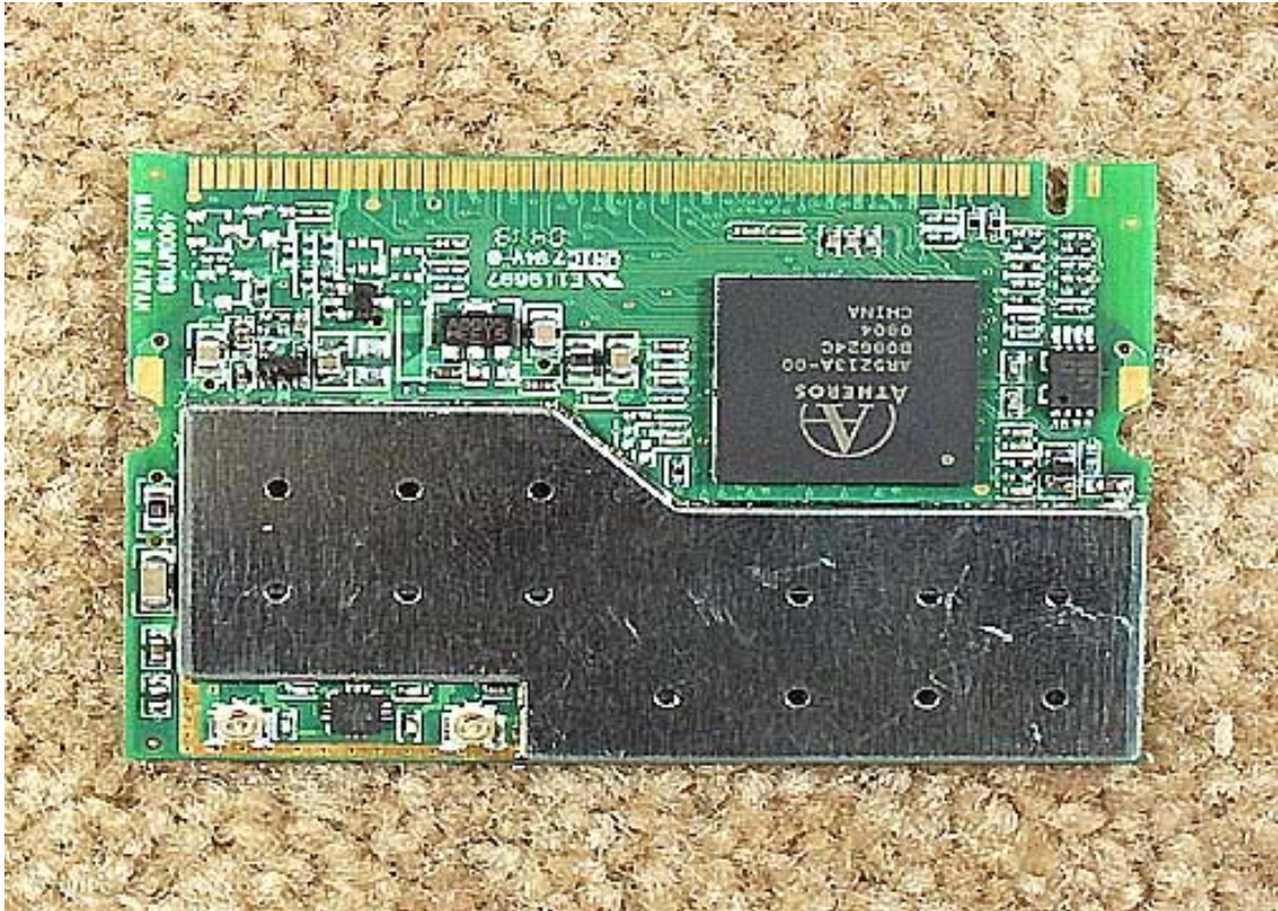
Transmitter PCB Top
