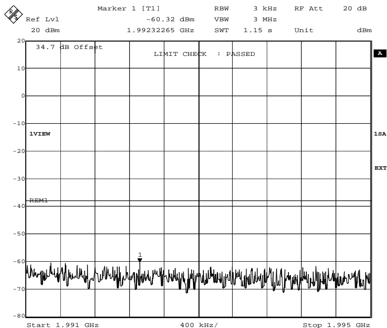
Fig. 84 – Spurious emissions in the frequency range 1991 MHz – 1995 MHz (GMSK modulation). Limit: -13dBm-25.2dB=-38.2dBm
