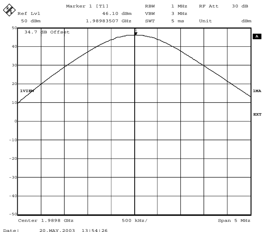
Fig. 23 – RF power at the antenna connector (8PSK modulation) for ECUPV2.
