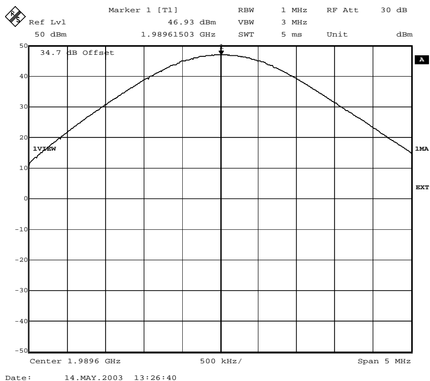
Fig. 17 – RF power at the antenna connector (8PSK modulation).
