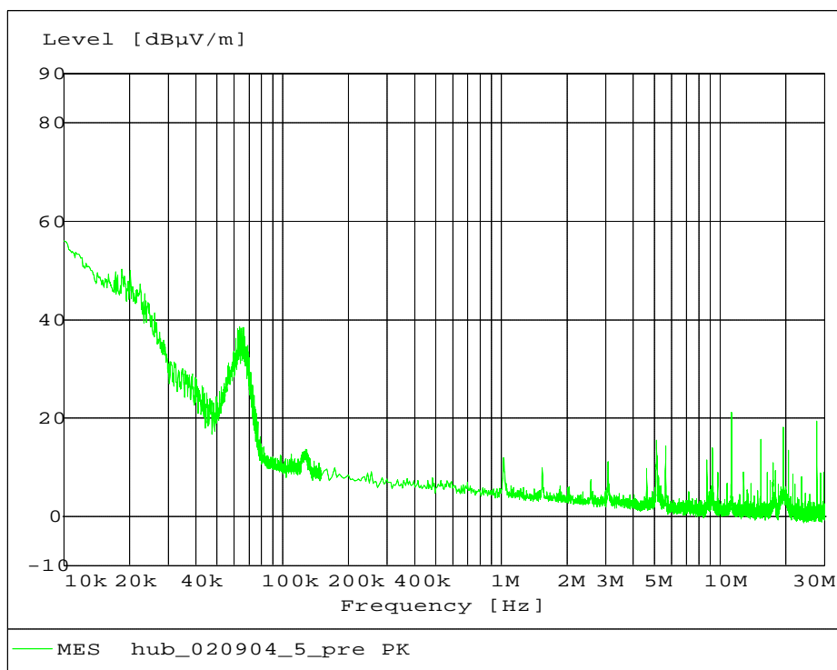
Fig. 94 – Radiated Emission 10 kHz – 30 MHz, 8PSK modulation.
