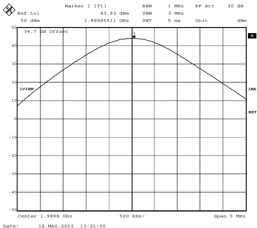
Fig. 21 – RF power at the antenna connector (8PSK modulation).
