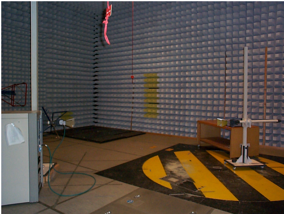
Fig. 92 – Photograph of the anechoic chamber with the test configuration for substitution method
