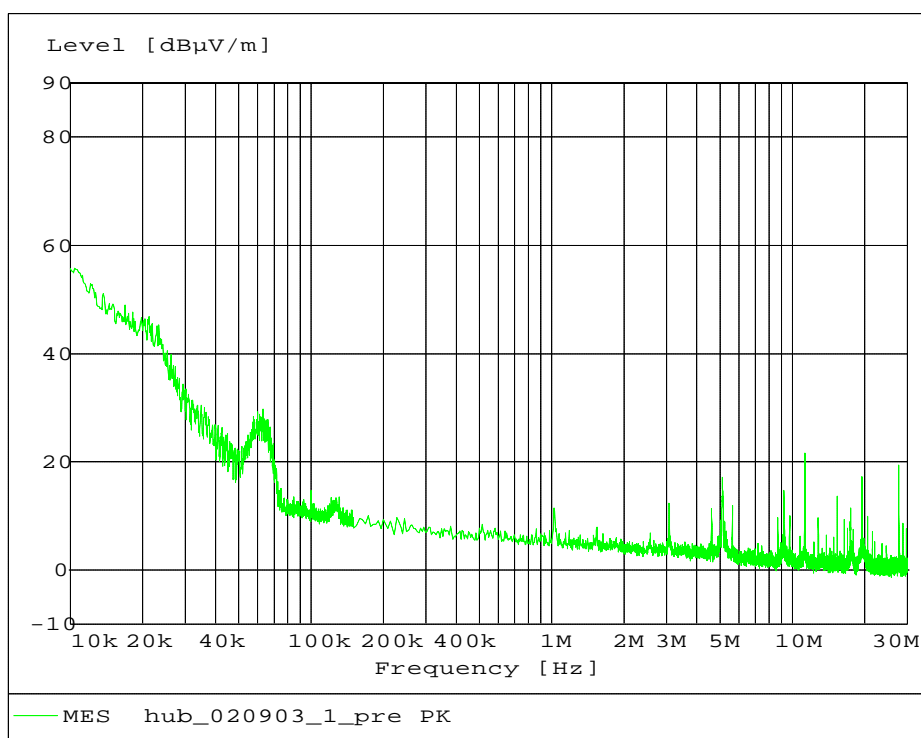
Fig. 93 – Radiated Emission 10 kHz – 30 MHz, GMSK modulation.
