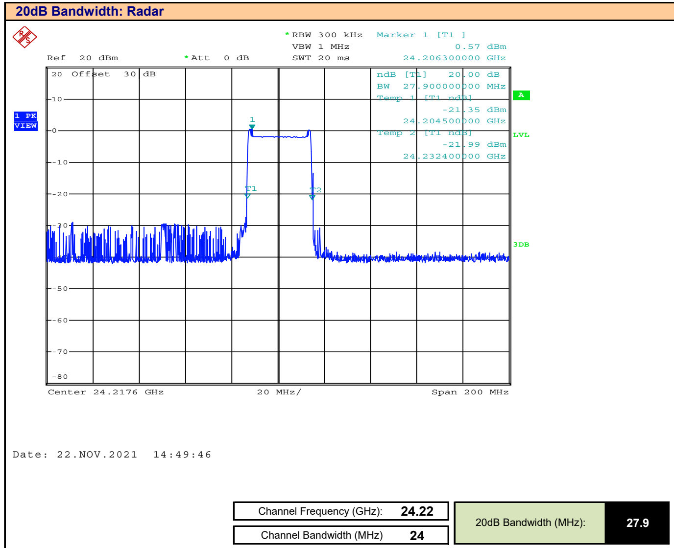
Plot 9.5 – 20dB BW, 24GHz Radar, 24MHz BW, Channel Hi
