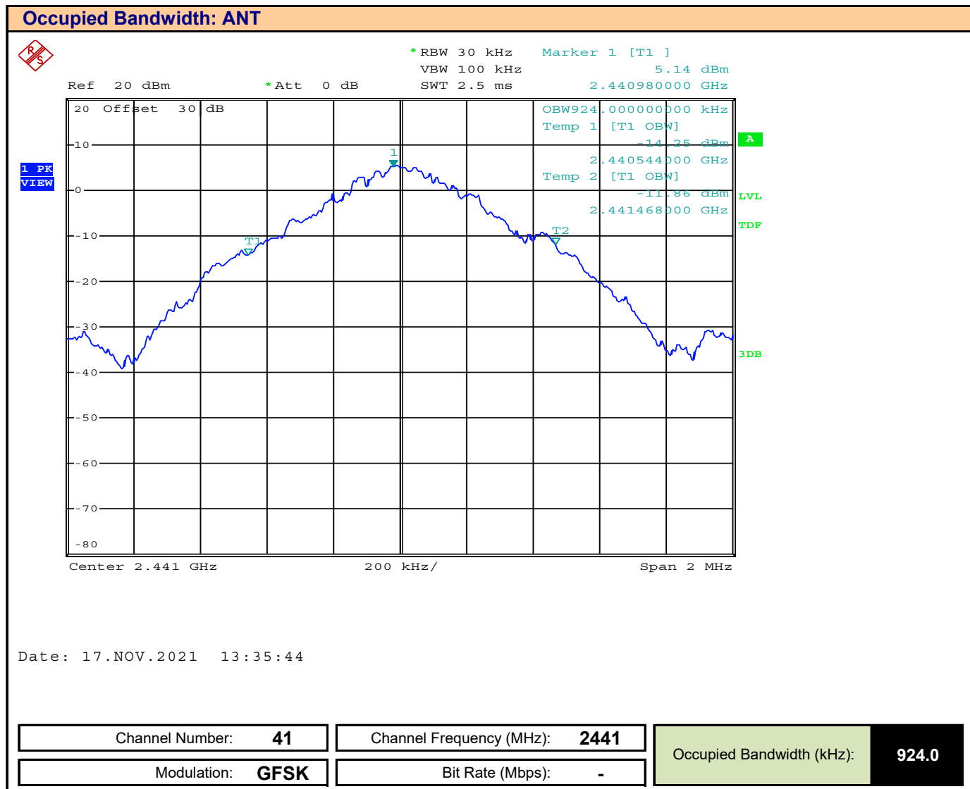
Plot 7.2 – Occupied Bandwidth, ANT, CH 41
