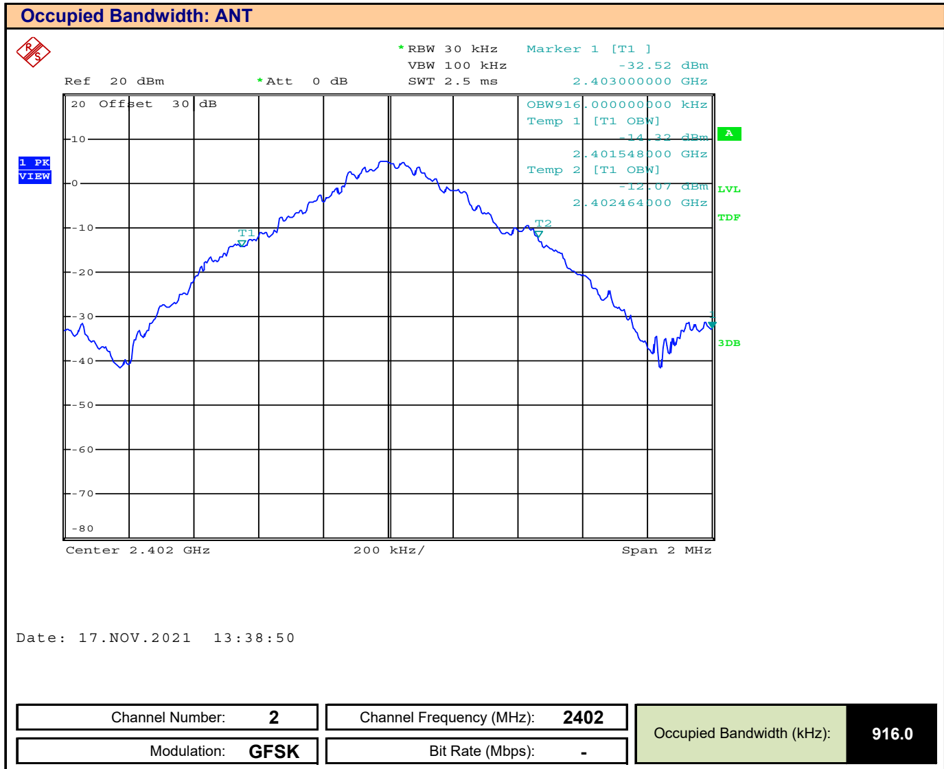
Plot 7.1 – Occupied Bandwidth, ANT, CH 2
