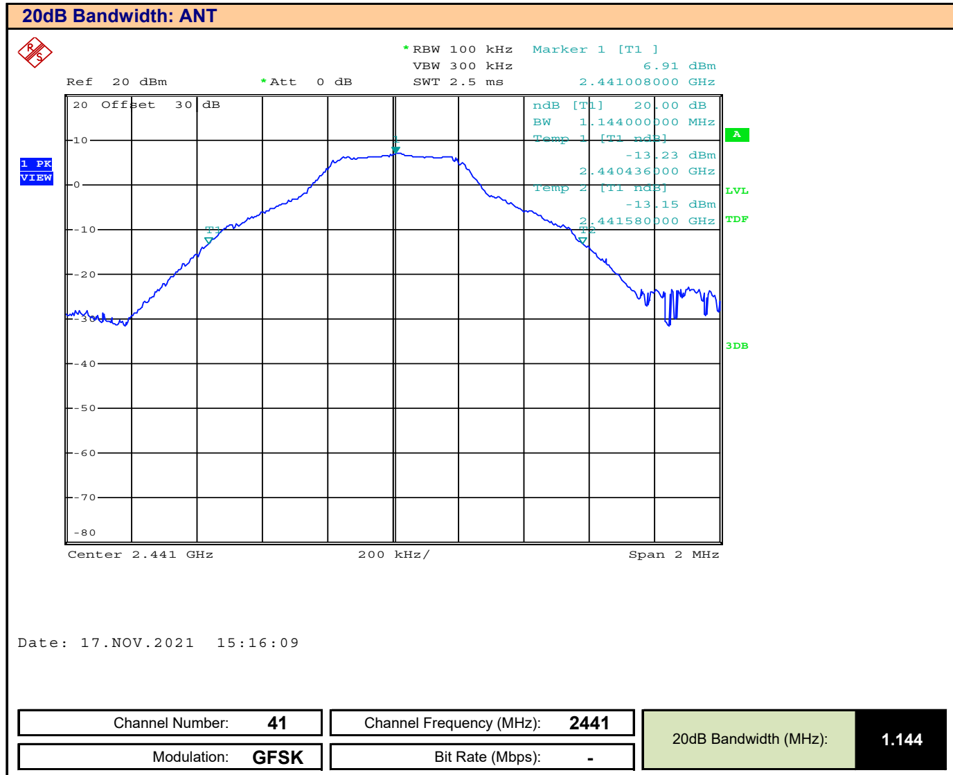
Plot 9.2 – 20dB BW, ANT, Ch 41
