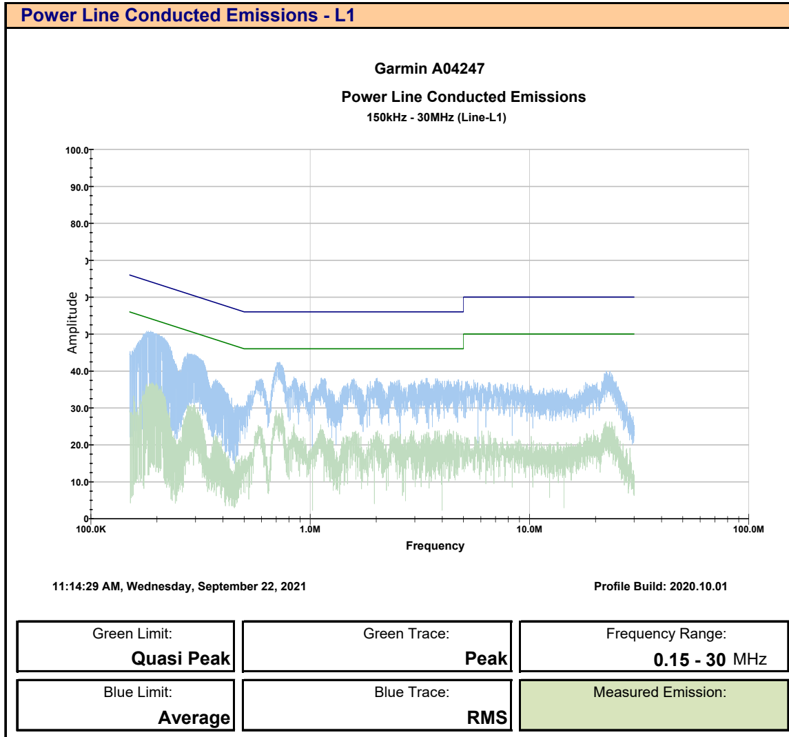
Plot 12.1 – Power Line Conducted Emissions, Line 1
