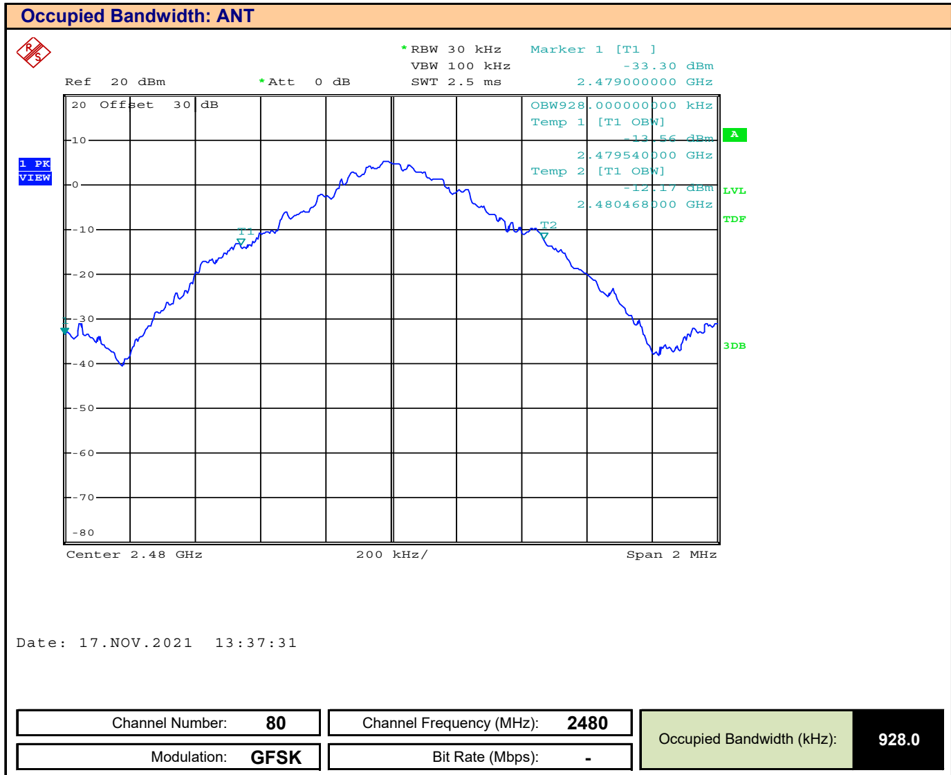
Plot 7.3 – Occupied Bandwidth, ANT, CH 80
