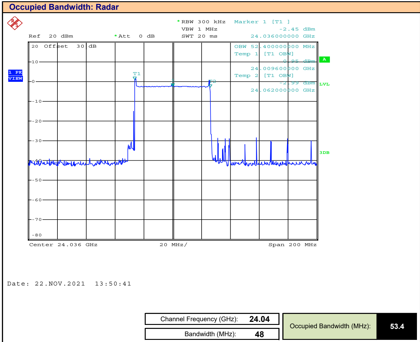
Plot 7.7 – Occupied Bandwidth, 24GHz Radar, 48MHz BW, Channel Lo
