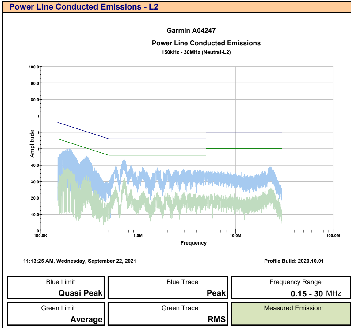
Plot 12.2 – Power Line Conducted Emissions, Line 2
