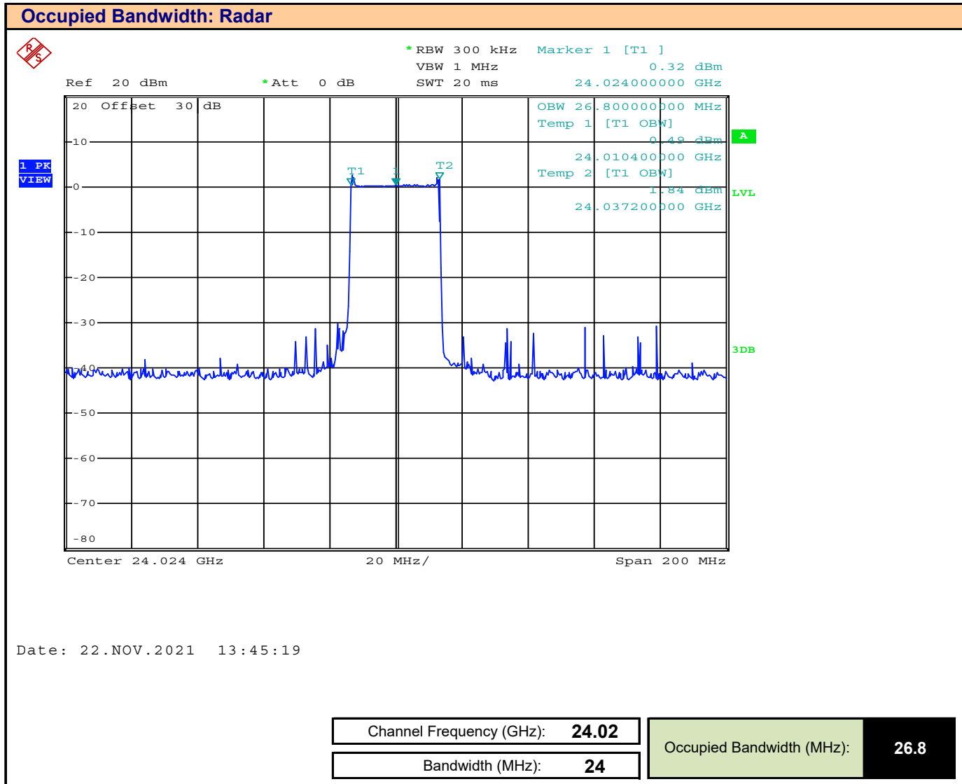
Plot 7.4 – Occupied Bandwidth, 24GHz Radar, 24MHz BW, Channel Lo
