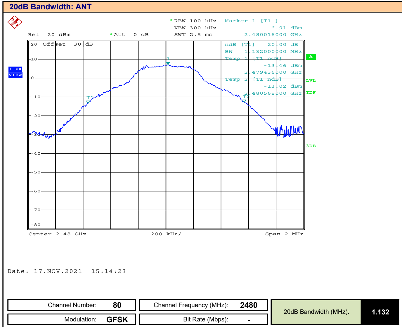
Plot 9.3 – 20dB BW, ANT, Ch 80
