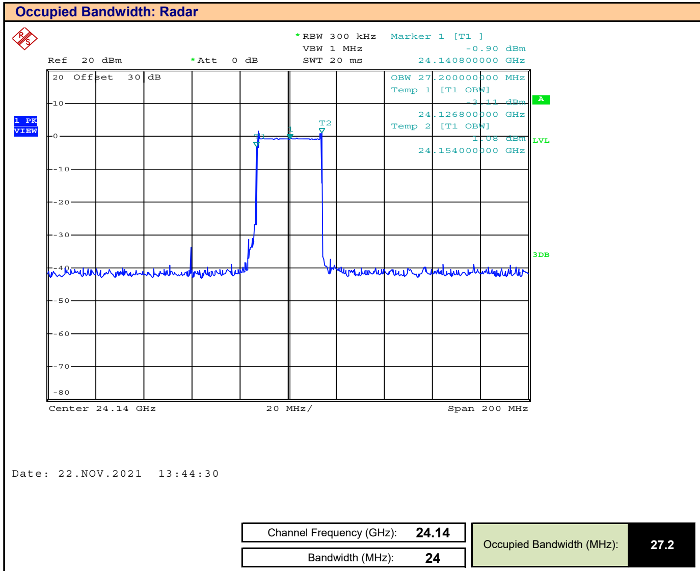
Plot 7.5 – Occupied Bandwidth, 24GHz Radar, 24MHz BW, Channel Mid
