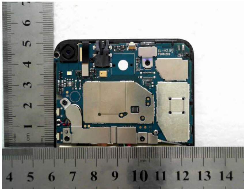
Mainboard With shielding Front View
