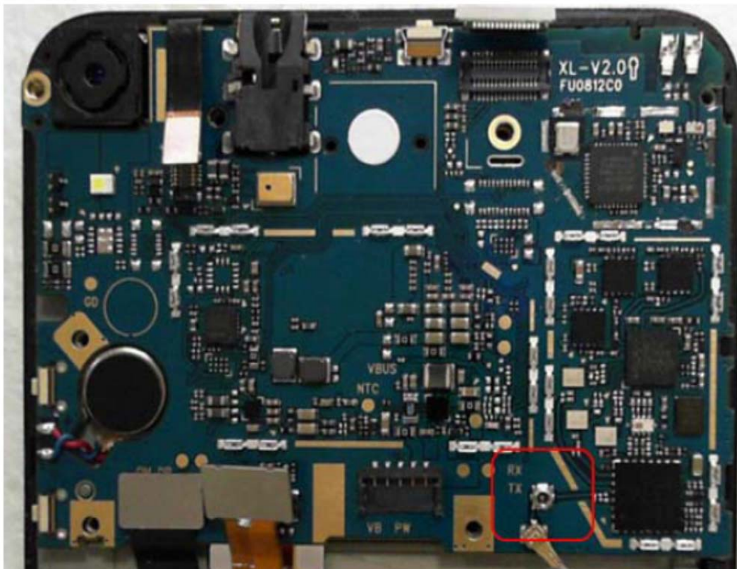
GSM/DCS/UMTS Antenna View
