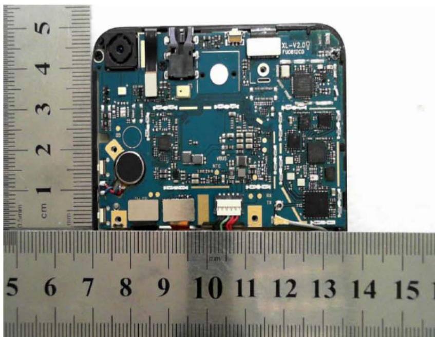
Mainboard Without shielding Front View
