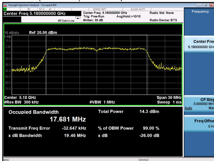
(802.11n20) Bandwidth plot on channel 36
