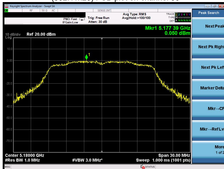
(802.11n20) PSD plot on channel 36
