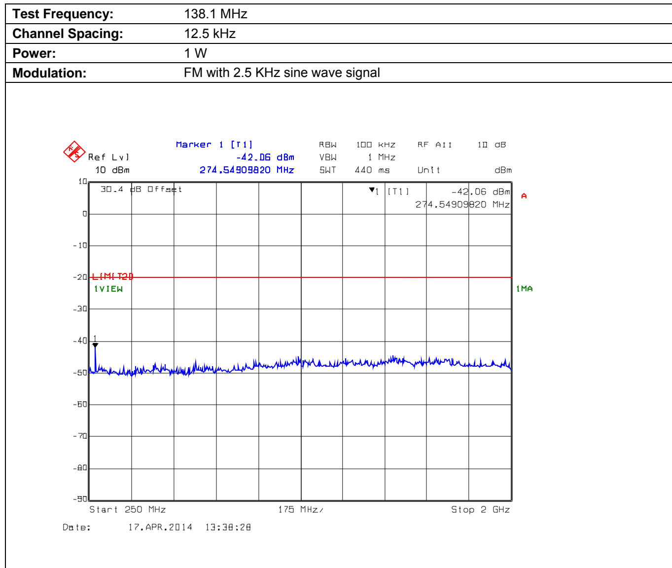
Plot 5.9.4.1.4. Conducted Transmitter Spurious Emissions for 138.1 MHz, Low Power, 250 MHz - 2 GHz
