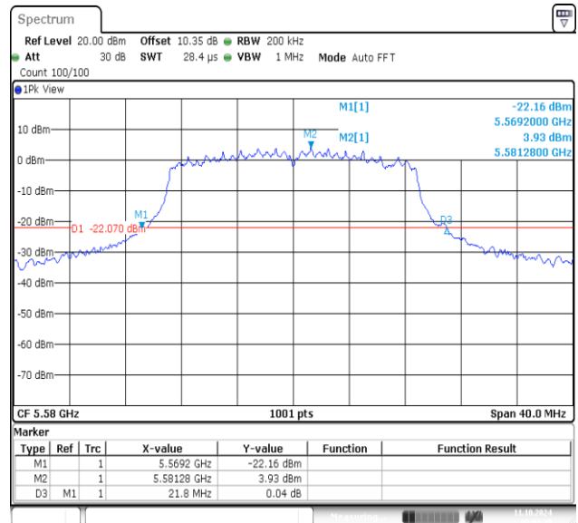
11AC20MIMO-Ant2-5580
