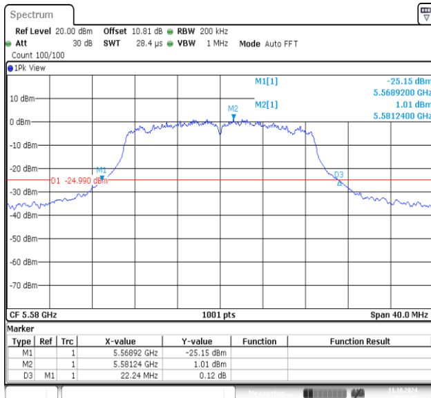
11AC20MIMO-Ant1-5580
