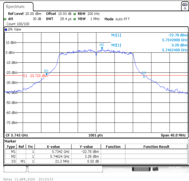
11A-Ant2-5745
