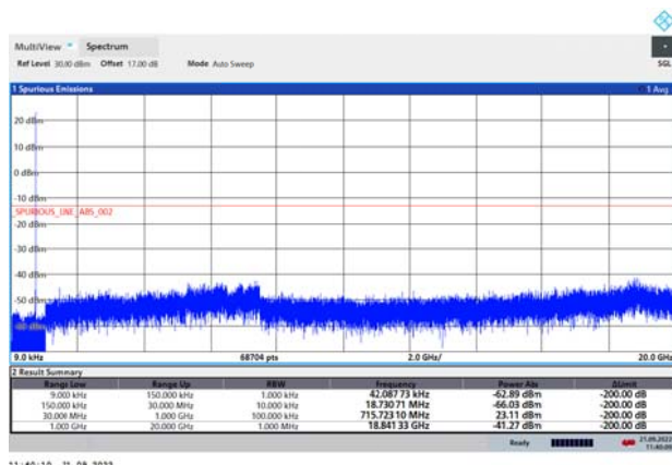
NB-IoT Band 12 CH-High 9kHz~20GHz
