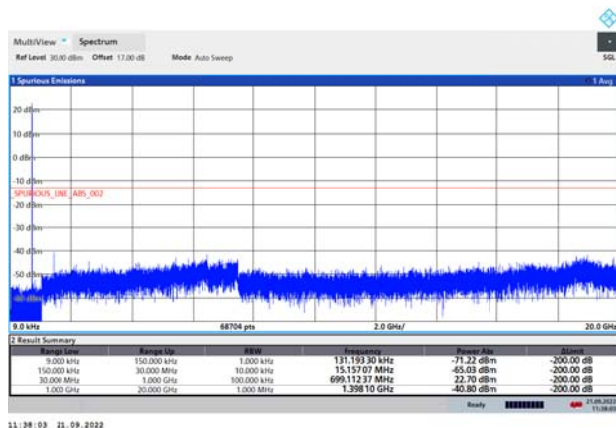
NB-IoT Band 12 CH-Middle 9kHz~20GHz
