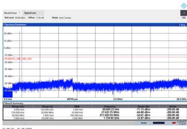
NB-IoT Band 4 CH-High 9kHz~20GHz
