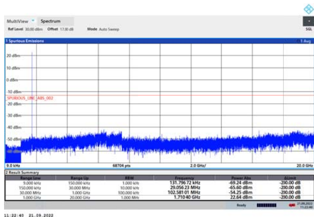
NB-IoT Band 4 CH-Middle 9kHz~20GHz
