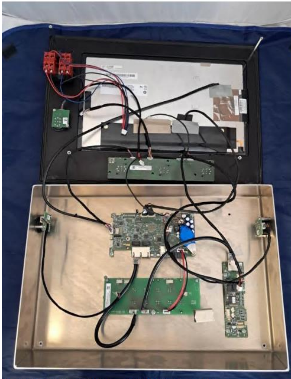
Fig. 4 Touch Industrial Webpanel OEM 13.3, internal view
