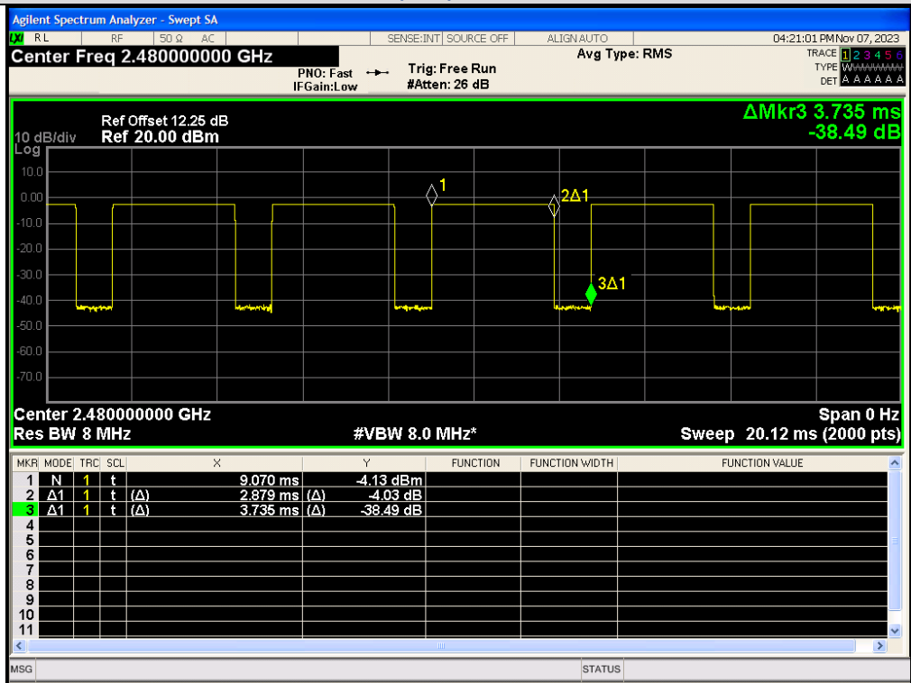
GFSK(DH5)_Channel 78
