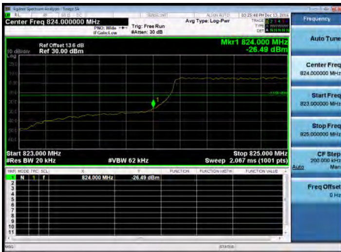
Band Edge_Band5_1.4MHz_QPSK_6_0_LowCH20407-824.7
