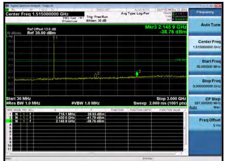
30MHz-3GHz_Band12_1.4MHz_QPSK_1_0_HighCH23173-715.3
