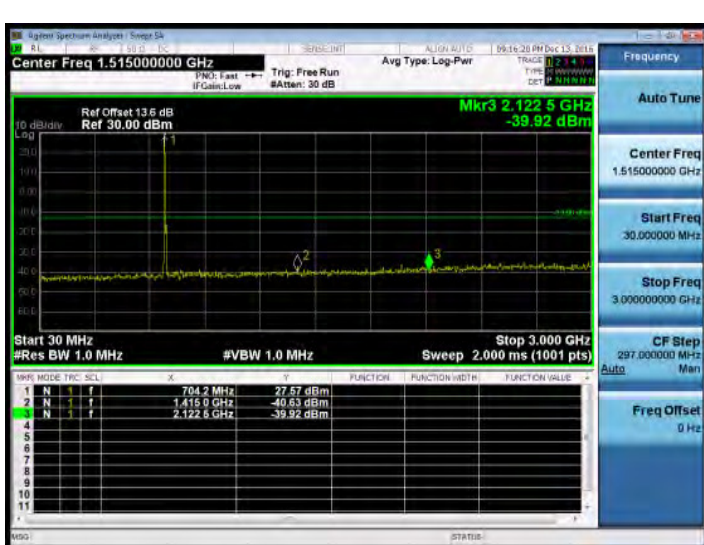
30MHz~3GHz_Band12_10MHz_QPSK_1_0_MidCH23095-707.5
