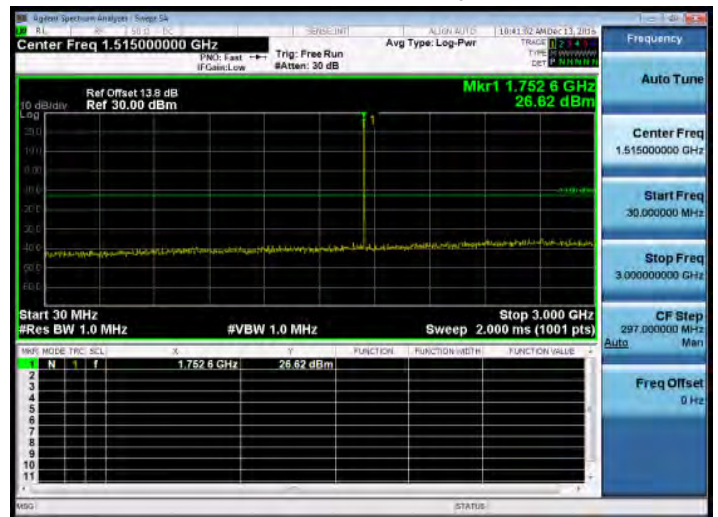
30MHz~3GHz_Band4_3MHz_QPSK_1_0_HighCH20385-1753.5
