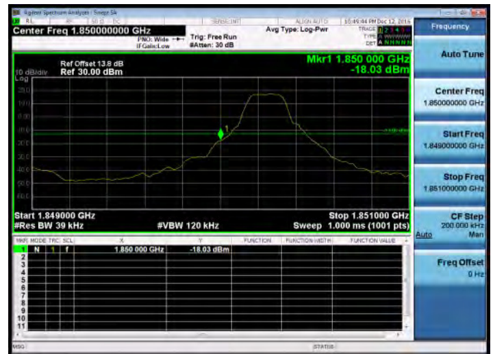
Band Edge_Band2_3MHz_QPSK_1_0_LowCH18615-1851.5
