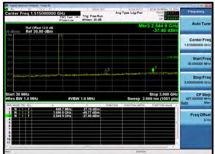
30MHz~3GHz_Band5_1.4MHz_QPSK_1_0_HighCH20643-848.3
