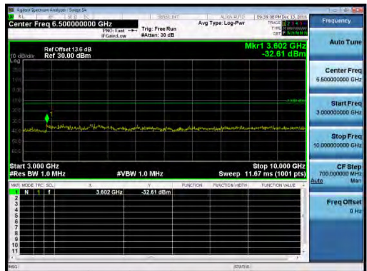
3GHz~10GHz_Band12_5MHz_QPSK_1_0_HighCH23155-713.5
