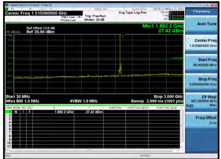
30MHz~3GHz_Band2_20MHz_QPSK_1_0_HighCH19100-1900
