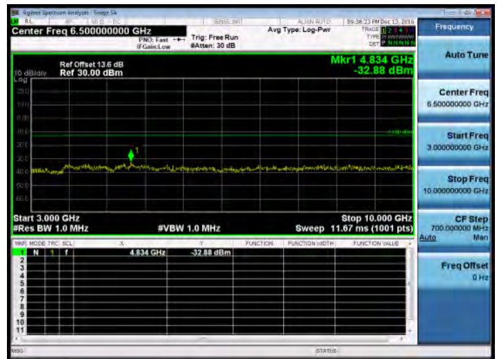
3GHz~10GHz_Band12_5MHz_QPSK_1_0_MidCH23095-707.5
