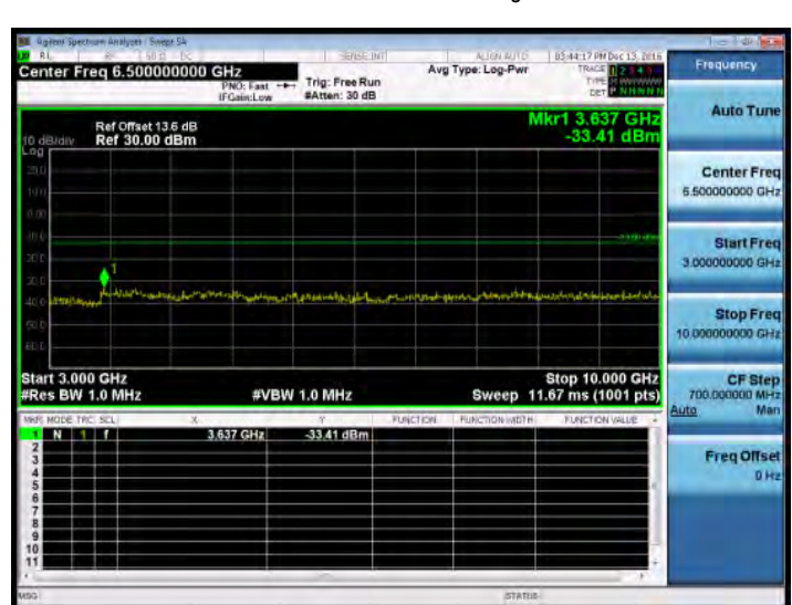
3GHz~10GHz_Band5_3MHz_QPSK_1_0_HighCH20635-847.5
