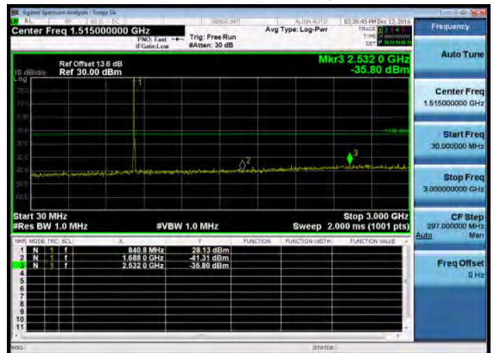
30MHz~3GHz_Band5_10MHz_QPSK_1_0_HighCH20600-844
