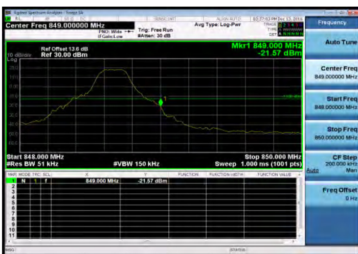
Band Edge_Band5_5MHz_QPSK_1_24_HighCH20625-846.5
