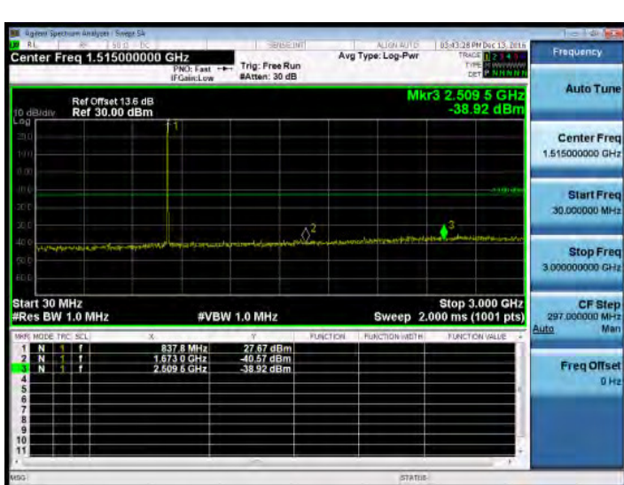
30MHz~3GHz_Band5_3MHz_QPSK_1_0_MidCH20525-836.5
