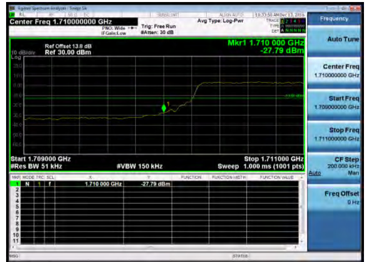
Band Edge_Band4_5MHz_QPSK_25_0_LowCH19975-1712.5
