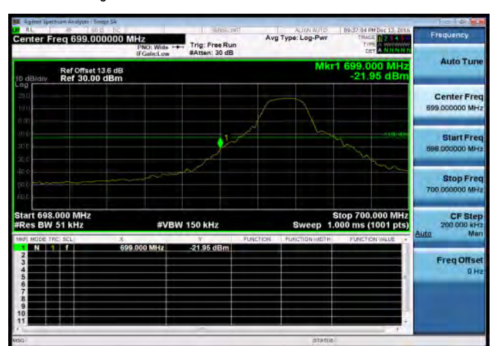
Band Edge_Band12_5MHz_QPSK_1_0_LowCH23035-701.5
