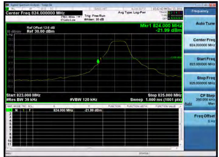
Band Edge_Band5_3MHz_QPSK_1_0_LowCH20415-825.5
