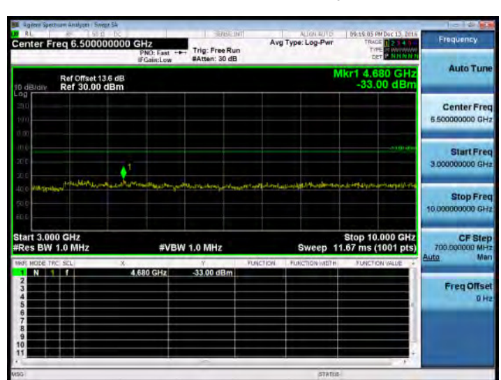
3GHz~10GHz_Band12_10MHz_QPSK_1_0_HighCH23130-711
