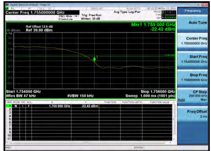
Band Edge_WCDMA_B4_HighCH1513-1752.6
