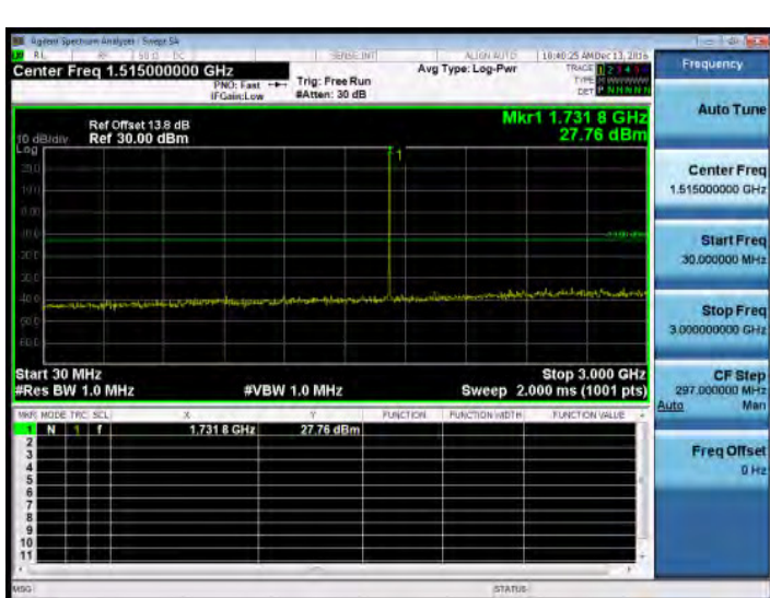
30MHz~3GHz_Band4_3MHz_QPSK_1_0_MidCH20175-1732.5
