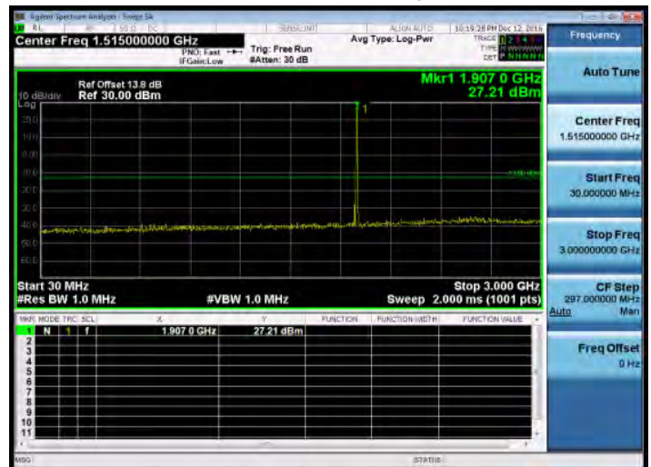
30MHz~3GHz_Band2_5MHz_QPSK_1_0_HighCH19175-1907.5
