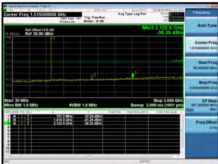
30MHz~3GHz_Band12_5MHz_QPSK_1_0_MidCH23095-707.5
