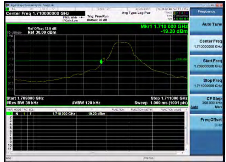
Band Edge_Band4_3MHz_QPSK_1_0_LowCH19965-1711.5
