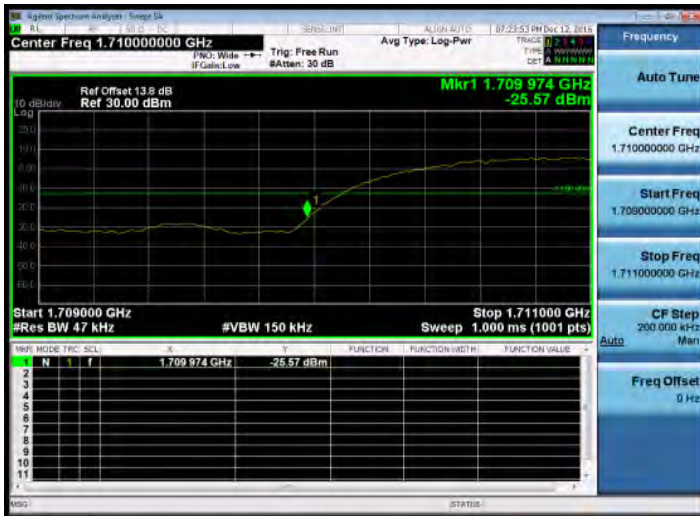
Band Edge_HSUPA_B4_LowCH1312-1712.4
