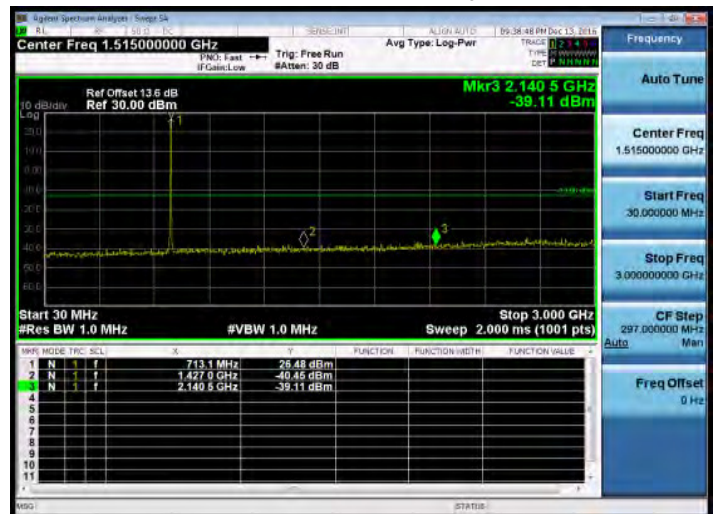
30MHz~3GHz_Band12_5MHz_QPSK_1_0_HighCH23155-713.5
