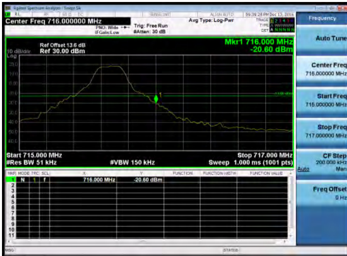
Band Edge_Band12_5MHz_QPSK_1_24_HighCH23155-713.5
