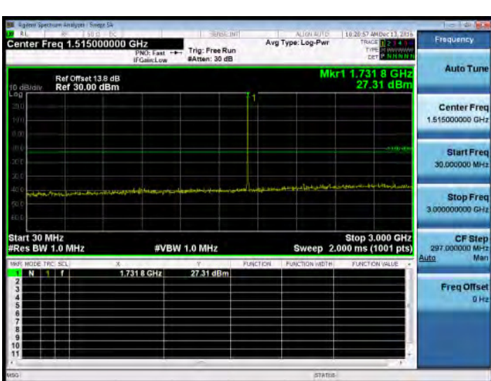
30MHz~3GHz_Band4_5MHz_QPSK_1_0_MidCH20175-1732.5
