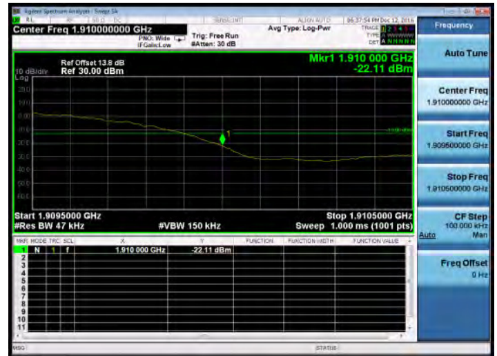
Band Edge_WCDMA_B2_HighCH9538-1907.6
