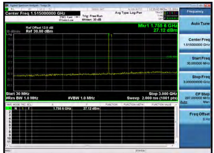
30MHz-3GHz_Band4_1.4MHz_QPSK_1_0_HighCH20393-1754.3
