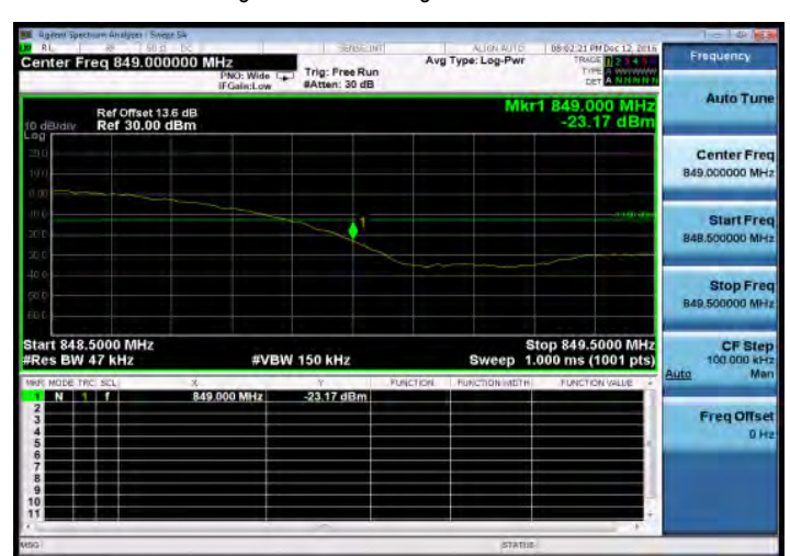
Band Edge_HSDPA_B5_HighCH4233-846.6
