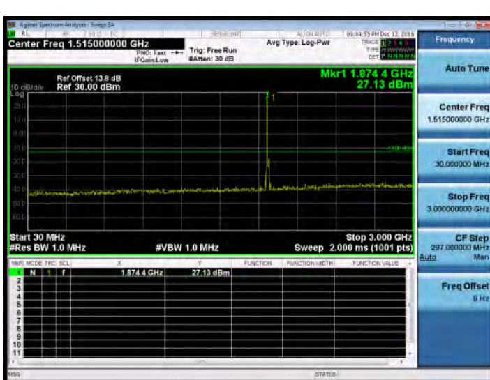
30MHz~3GHz_Band2_15MHz_QPSK_1_0_MidCH18900-1880
