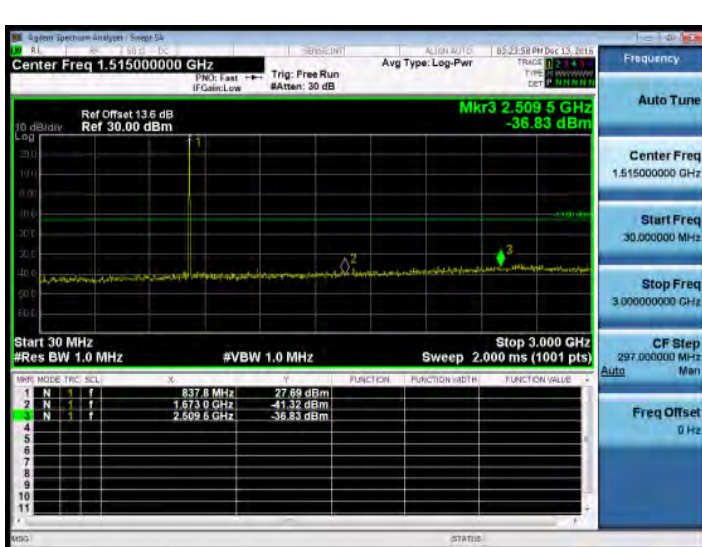
30MHz~3GHz_Band5_1.4MHz_QPSK_1_0_MidCH20525-836.5
