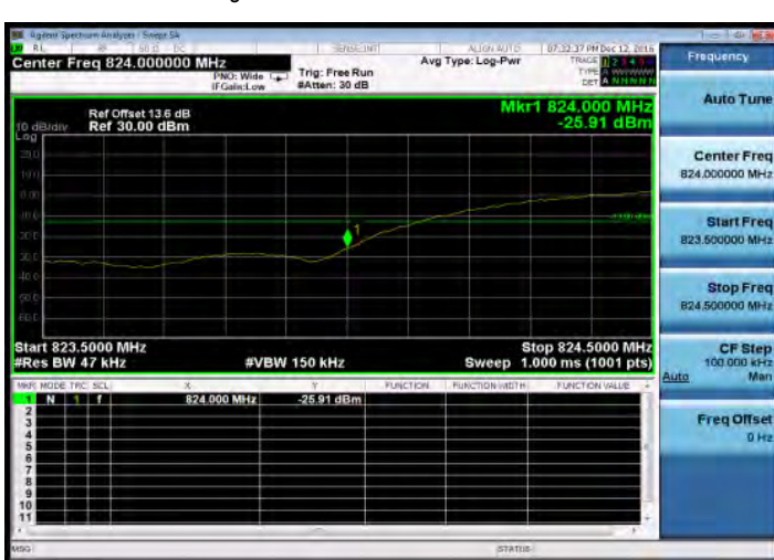
Band Edge_WCDMA_B5_LowCH4132-826.4
