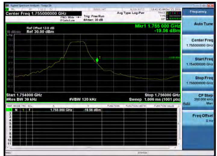
Band Edge_Band4_3MHz_QPSK_1_14_HighCH20385-1753.5
