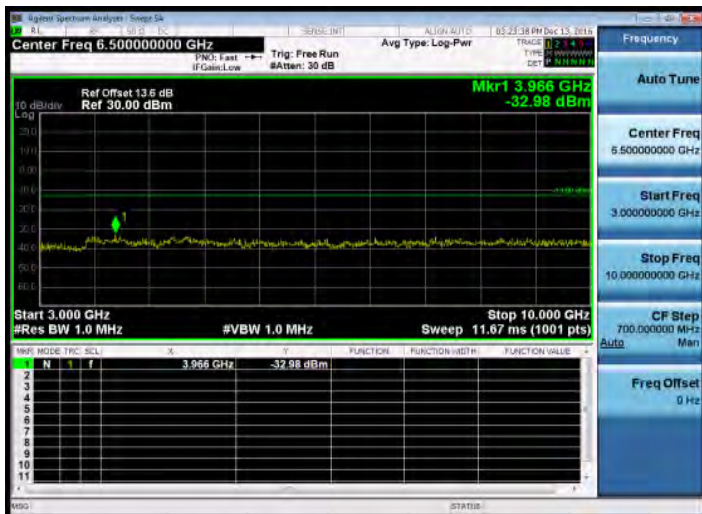
3GHz~10GHz_Band5_1.4MHz_QPSK_1_0_LowCH20407-824.7
