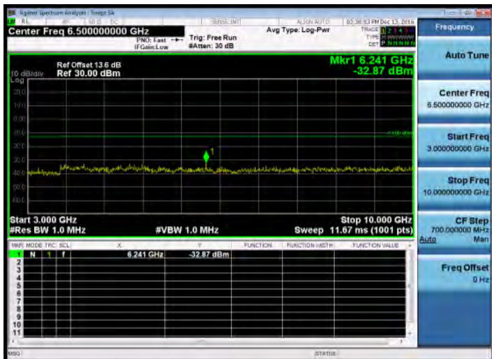
3GHz~10GHz_Band5_10MHz_QPSK_1_0_LowCH20450-829
