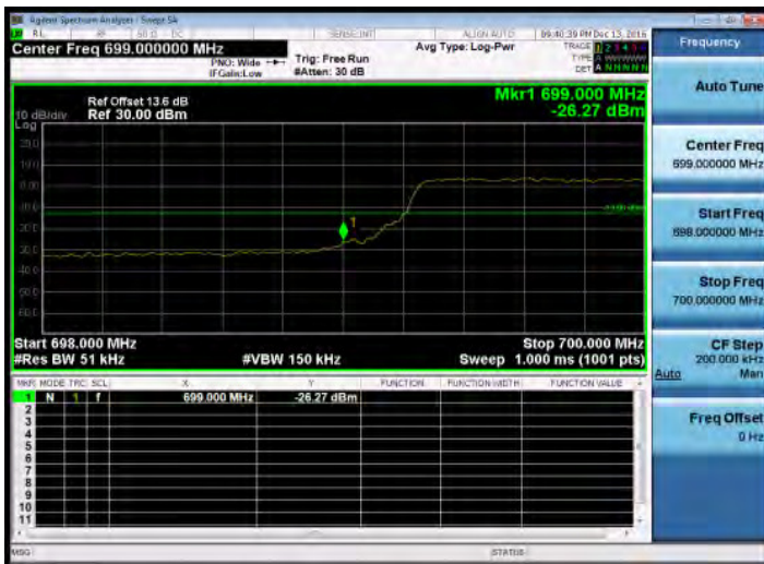
Band Edge_Band12_5MHz_QPSK_25_0_LowCH23035-701.5
