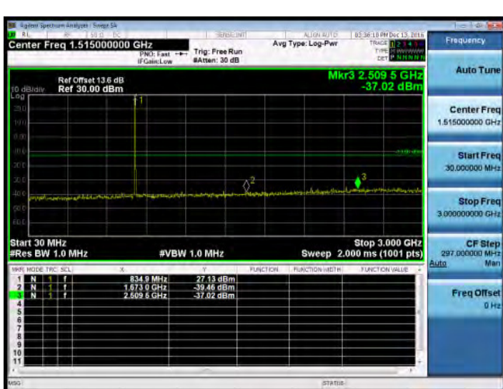
30MHz~3GHz_Band5_5MHz_QPSK_1_0_MidCH20525-836.5
