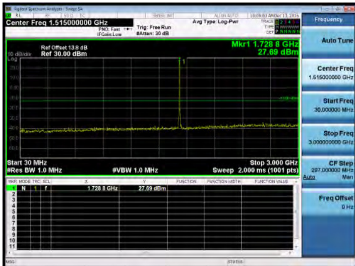
30MHz~3GHz_Band4_10MHz_QPSK_1_0_MidCH20175-1732.5
