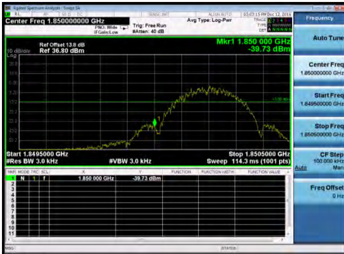
Band Edge_EDGE_1900MHz_LowCH512-1850.2
