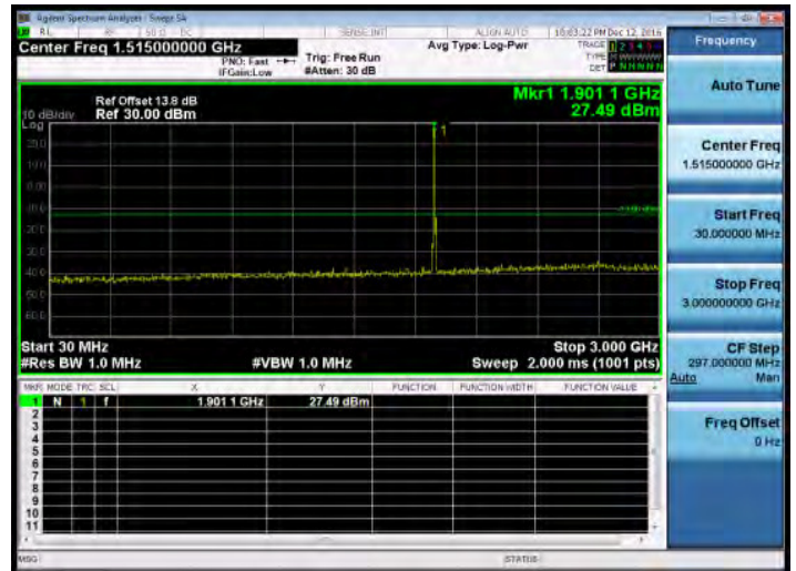
30MHz~3GHz_Band2_10MHz_QPSK_1_0_HighCH19150-1905
