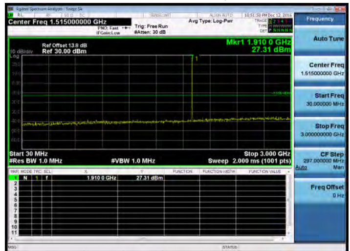
30MHz~3GHz_Band2_3MHz_QPSK_1_0_HighCH19185-1908.5
