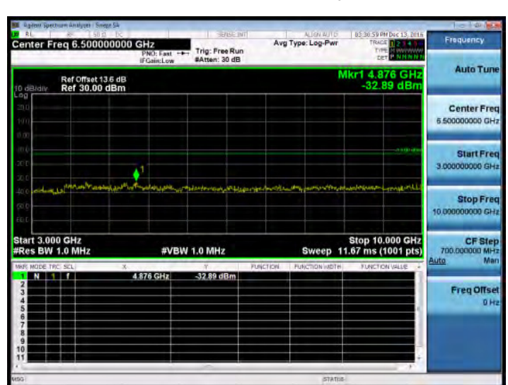
3GHz~10GHz_Band5_10MHz_QPSK_1_0_HighCH20600-844
