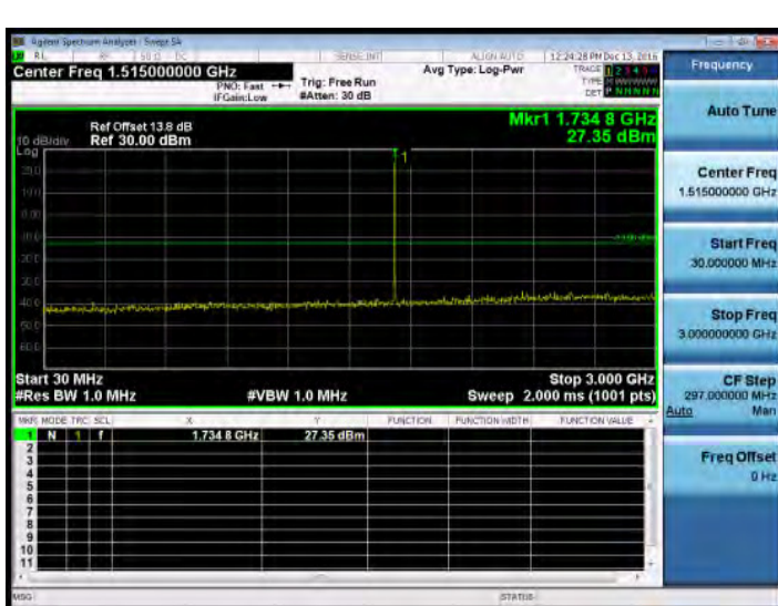
30MHz-3GHz_Band4_1.4MHz_QPSK_1_0_MidCH20175-1732.5
