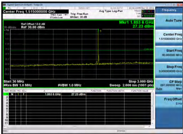
30MHz~3GHz_Band2_5MHz_QPSK_1_0_LowCH18625-1852.5
