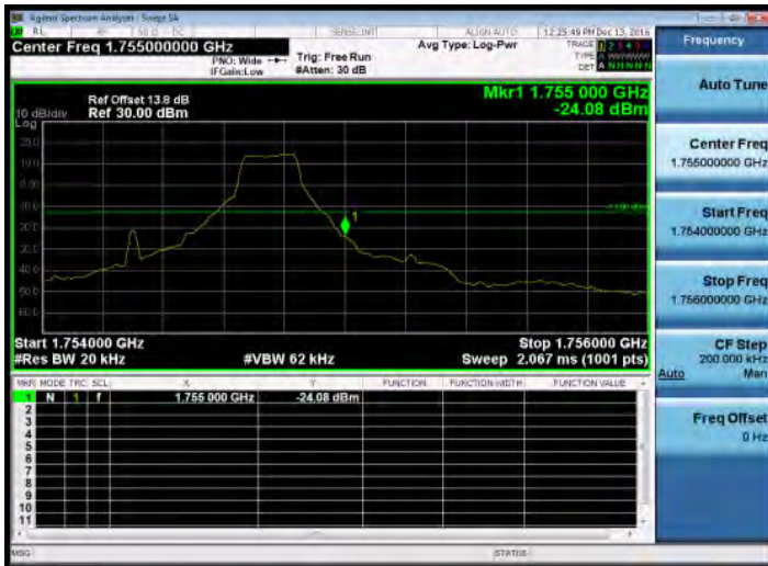
Band Edge_Band4_1.4MHz_QPSK_1_5_HighCH20393-1754.3
