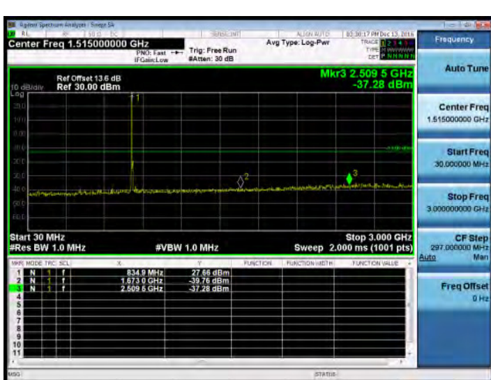
30MHz~3GHz_Band5_10MHz_QPSK_1_0_MidCH20525-836.5
