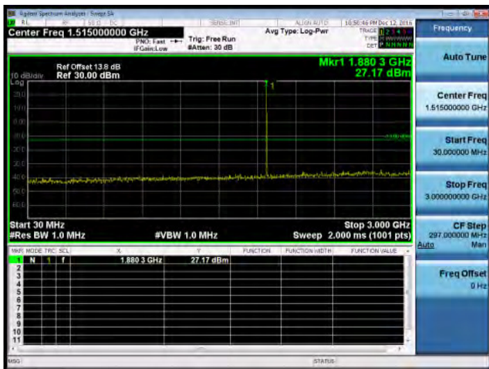
30MHz~3GHz_Band2_3MHz_QPSK_1_0_MidCH18900-1880
