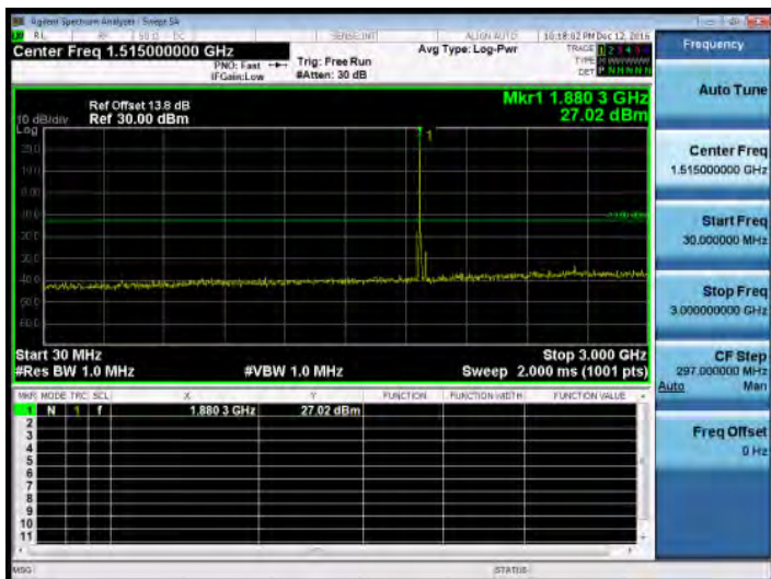
30MHz~3GHz_Band2_5MHz_QPSK_1_0_MidCH18900-1880
