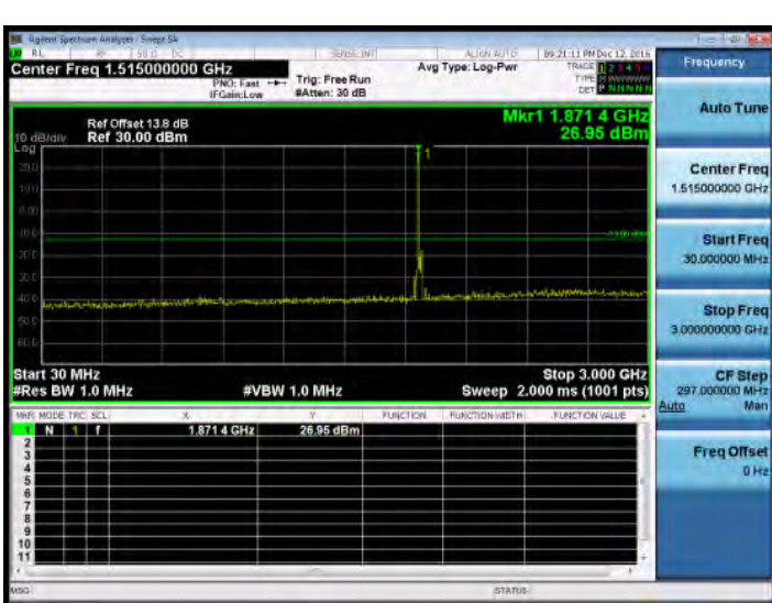
30MHz~3GHz_Band2_20MHz_QPSK_1_0_MidCH18900-1880
