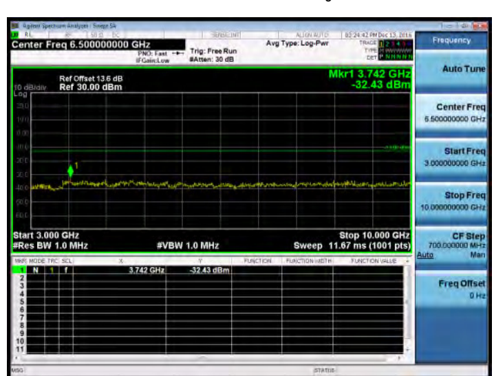
3GHz~10GHz_Band5_1.4MHz_QPSK_1_0_HighCH20643-848.3
