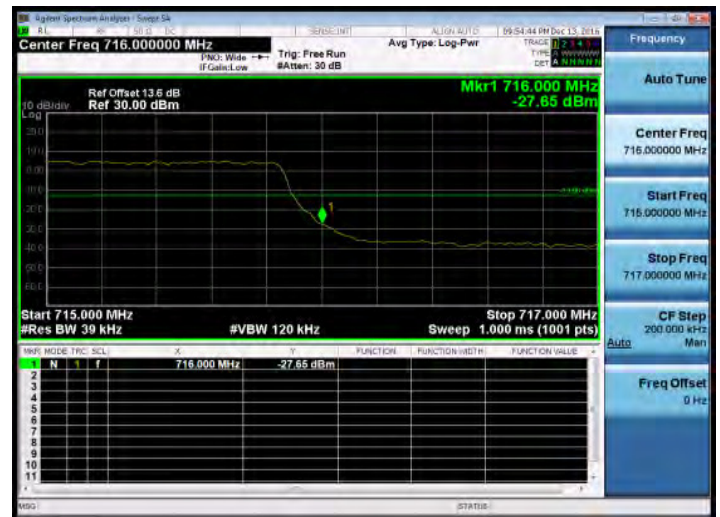
Band Edge_Band12_3MHz_QPSK_15_0_HighCH23165-714.5
