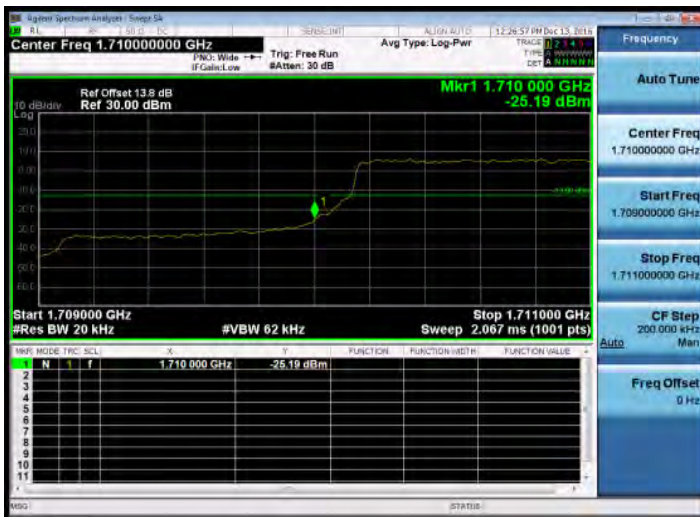
Band Edge_Band4_1.4MHz_QPSK_6_0_LowCH19957-1710.7
