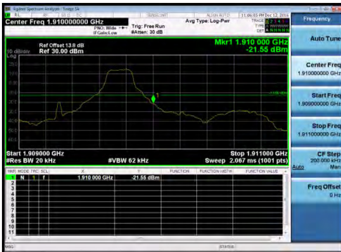
Band Edge_Band2_1.4MHz_QPSK_1_5_HighCH19193-1909.3
