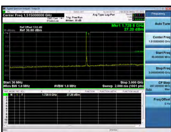
30MHz~3GHz_Band4_15MHz_QPSK_1_0_MidCH20175-1732.5
