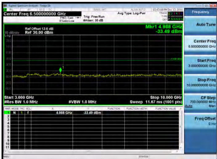
3GHz~10GHz_Band5_3MHz_QPSK_1_0_LowCH20415-825.5
