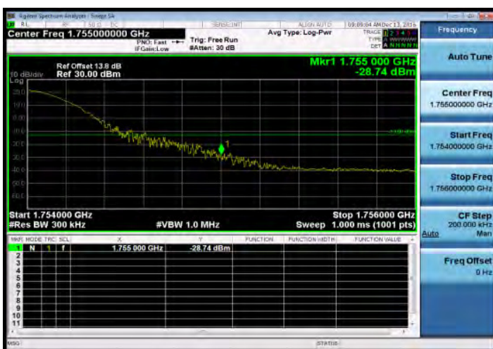
Band Edge_Band4_20MHz_QPSK_1_99_HighCH20300-1745
