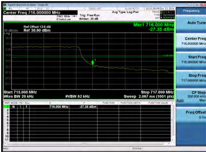
Band Edge_Band12_1.4MHz_QPSK_6_0_HighCH23173-715.3
