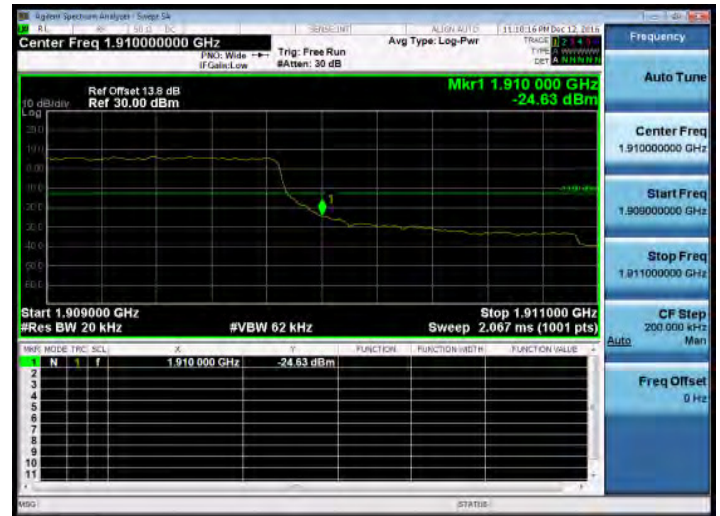
Band Edge_Band2_1.4MHz_QPSK_6_0_HighCH19193-1909.3
