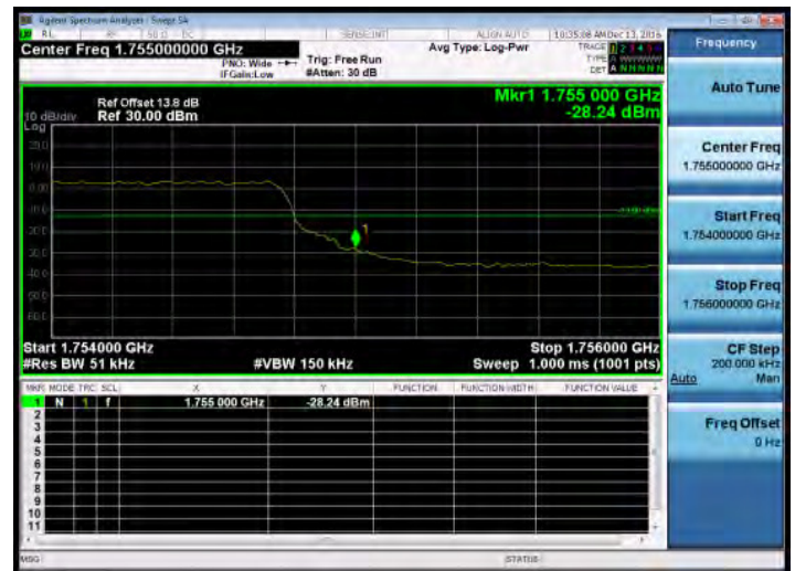
Band Edge_Band4_5MHz_QPSK_25_0_HighCH20375-1752.5
