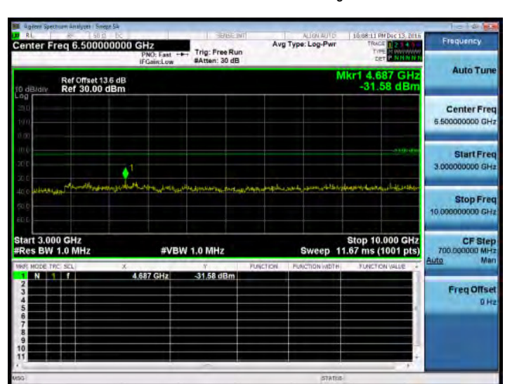
3GHz-10GHz_Band12_1_4MHz_QPSK_1_0_HighCH23173-715.3
