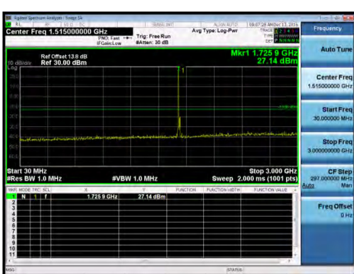
30MHz~3GHz_Band4_20MHz_QPSK_1_0_MidCH20175-1732.5
