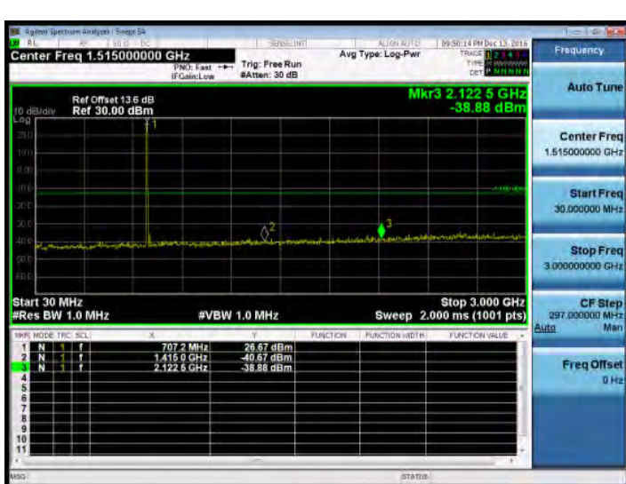
30MHz~3GHz_Band12_3MHz_QPSK_1_0_MidCH23095-707.5
