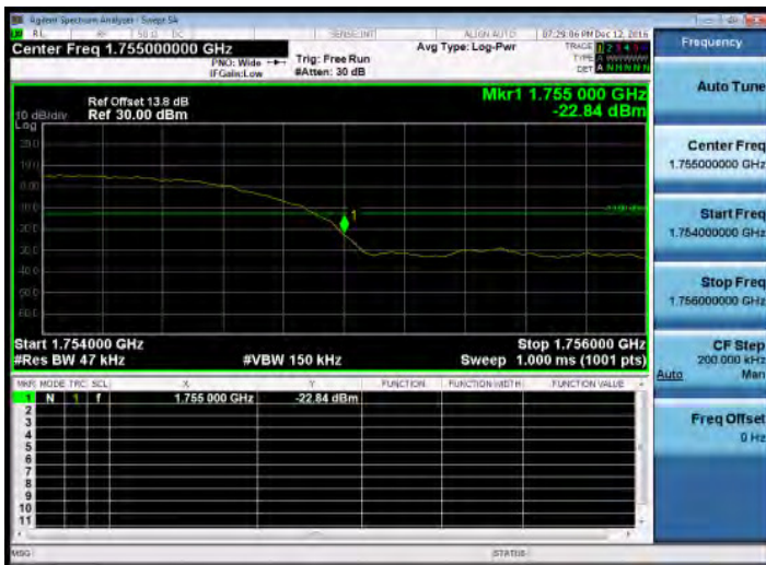
Band Edge_HSUPA_B4_HighCH1513-1752.6
