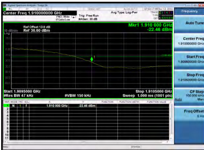
Band Edge_HSUPA_B2_HighCH9538-1907.6
