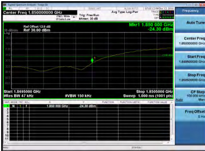
Band Edge_HSUPA_B2_LowCH9262-1852.4
