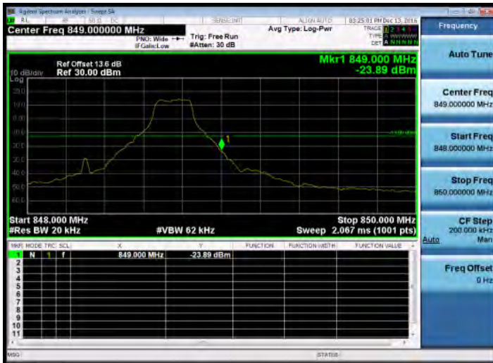
Band Edge_Band5_1.4MHz_QPSK_1_5_HighCH20643-848.3
