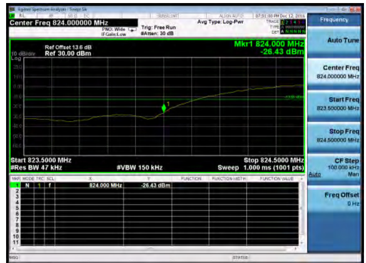
Band Edge_HSDPA_B5_LowCH4132-826.4
