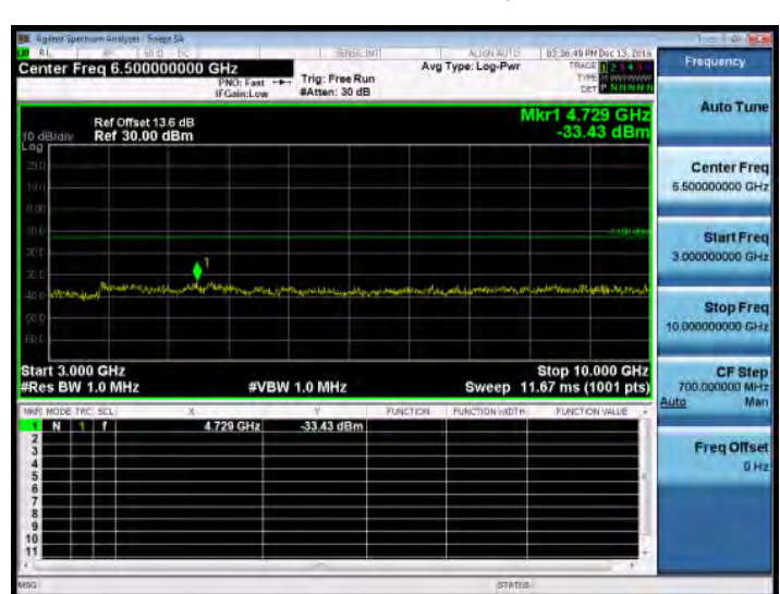
3GHz~10GHz_Band5_5MHz_QPSK_1_0_HighCH20625-846.5
