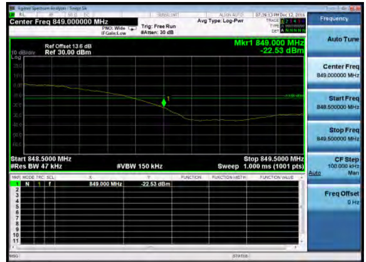
Band Edge_WCDMA_B5_HighCH4233-846.6
