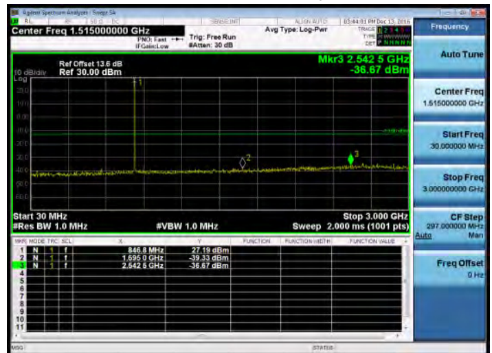
30MHz~3GHz_Band5_3MHz_QPSK_1_0_HighCH20635-847.5
