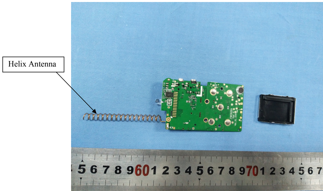
EUT –Mainboard Bottom Uncovered View
