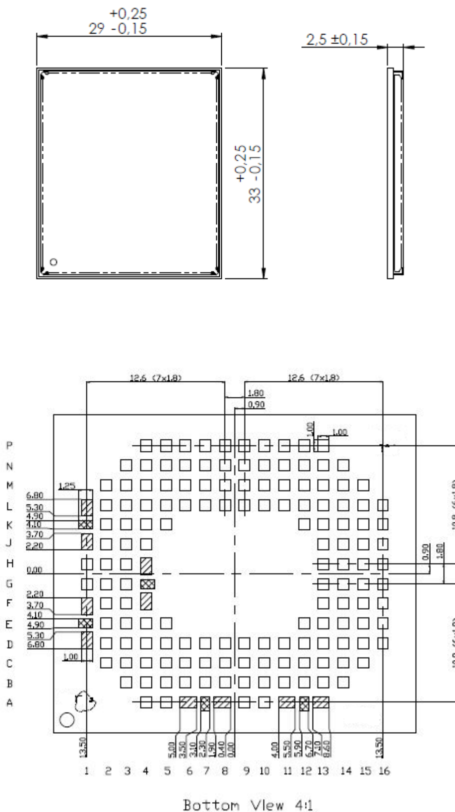
Figure 31: Dimensions of PLSx3 (all dimensions in mm)
