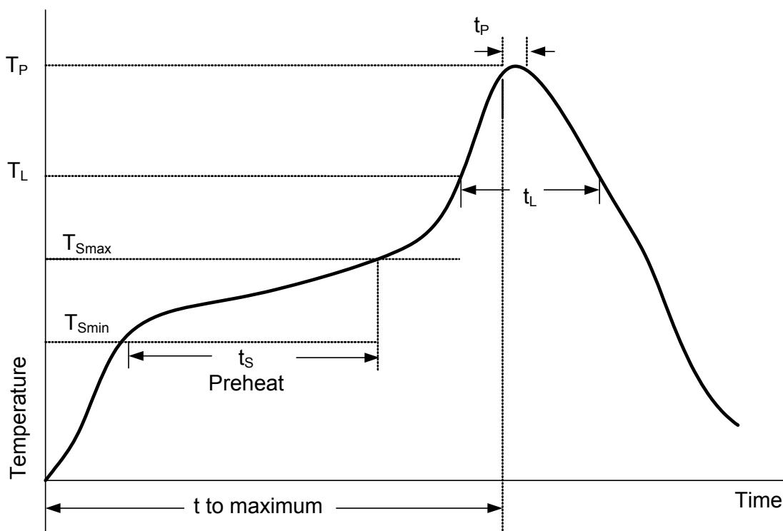
Figure 36: Reflow Profile
