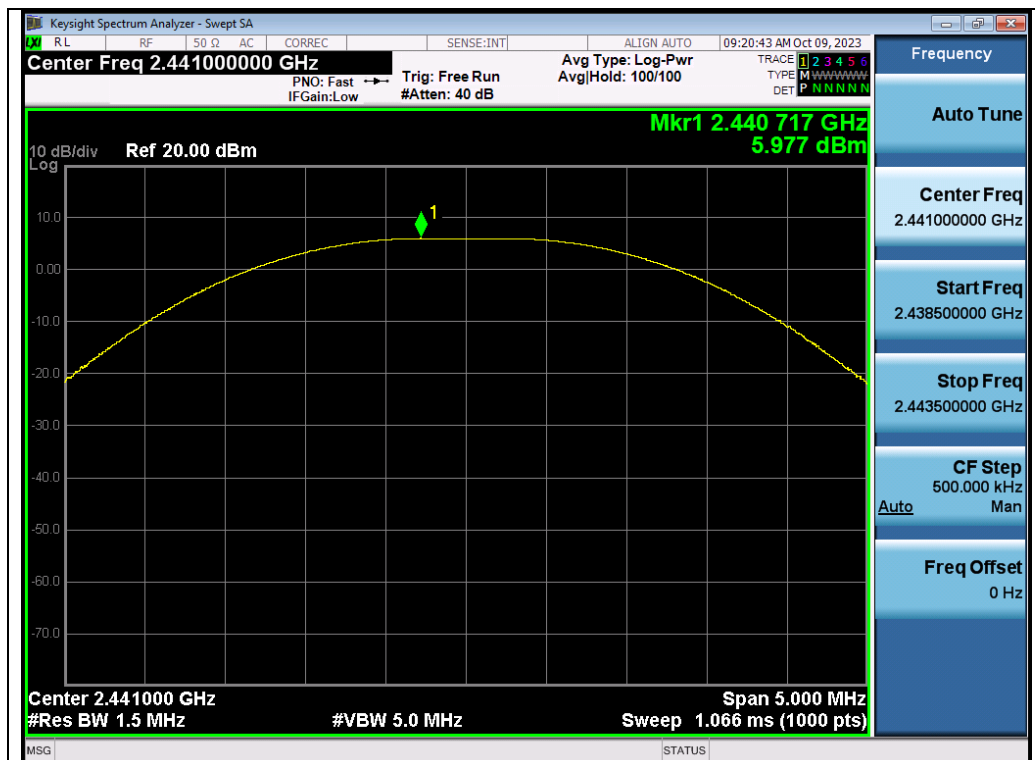
Test_Graph_GFSK_ANT2_2441_Peak Power
