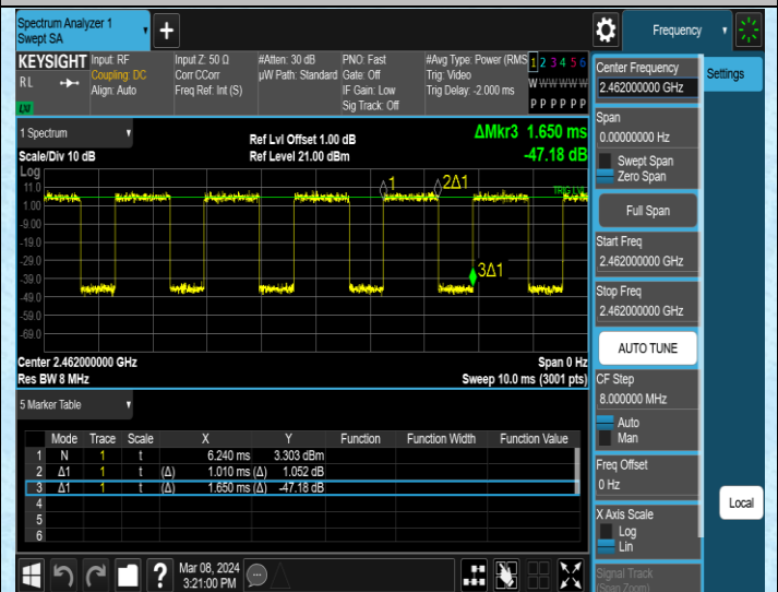
NTNV-11AX20MIMO-Ant2-2462
