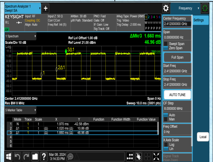
NTNV-11AX20MIMO-Ant2-2412
