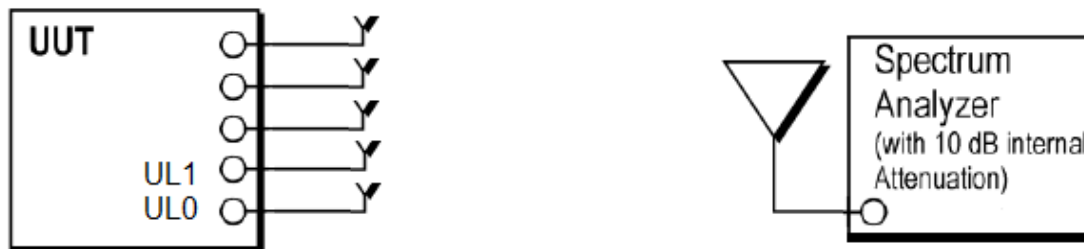
Figure 2. Block Diagram of Test Configuration, Radiated Emissions (as modules)
