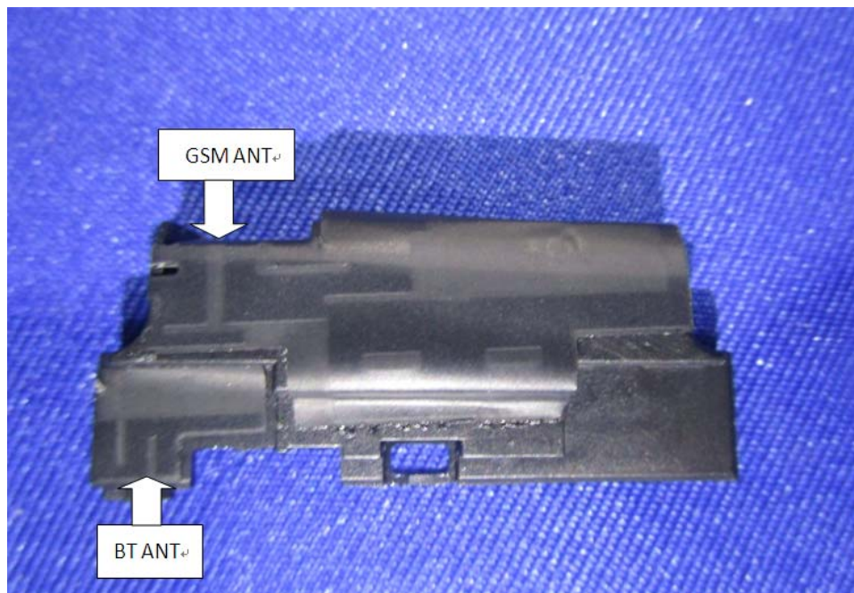
EUT –GSM&BT Antenna View
