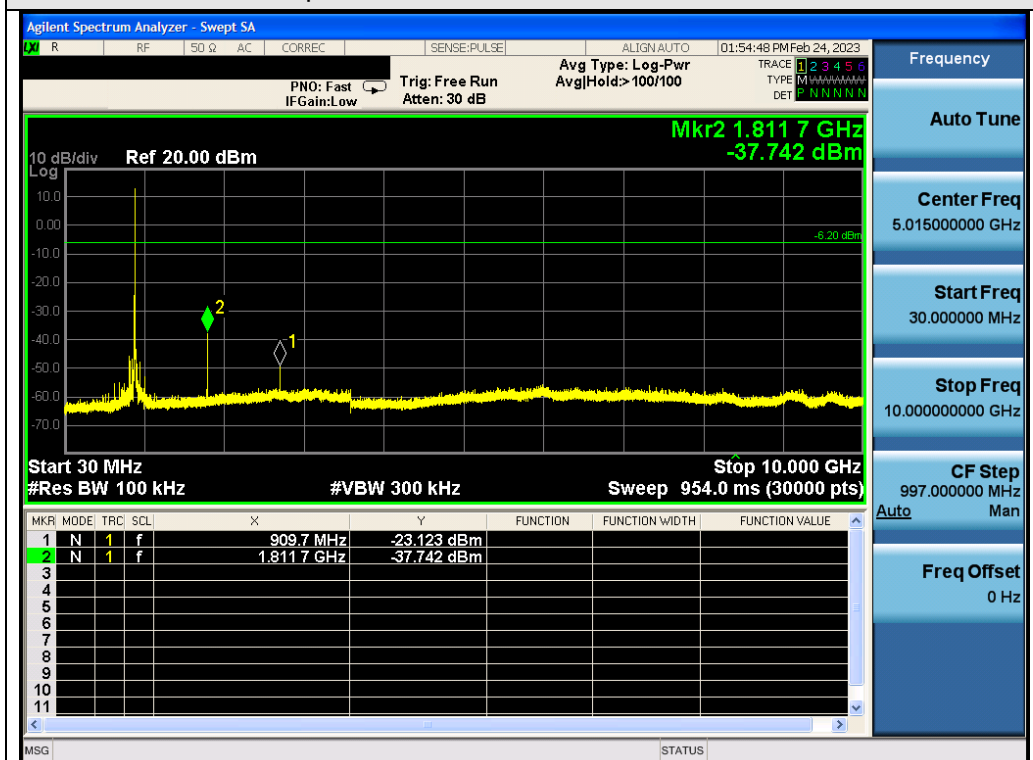
Test_Graph_OFDM_ANT1_906_4M_Band Emissions
