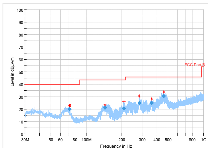
Fig 18. Radiated Spurious Emission (802.11 n-40MHz,Ch3,30MHz~1GHz)
