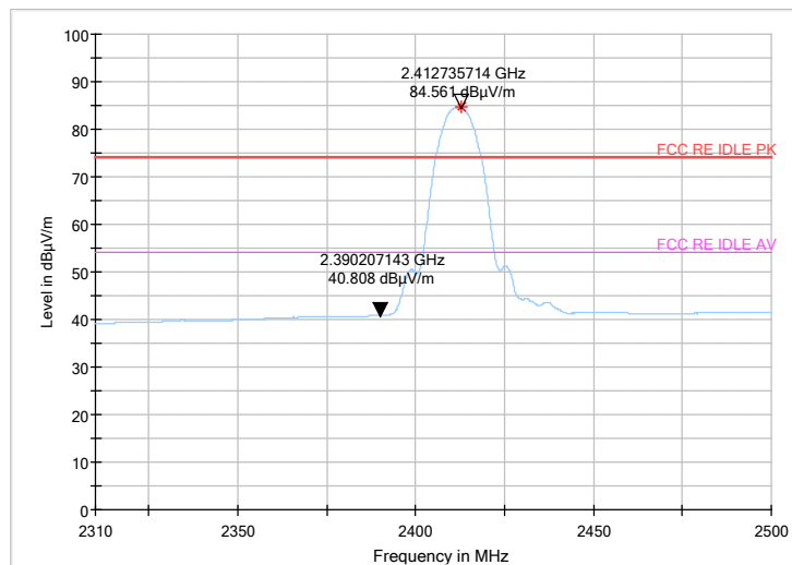
Fig 1. Radiated emission (Power): 802.11b, low channel
