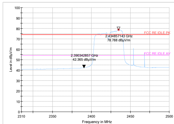
Fig 16. Radiated emission (Power): 802.11n (40M) , low channel
