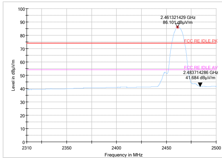
Fig 2. Fig.58 Radiated emission (Power): 802.11b, high channel
