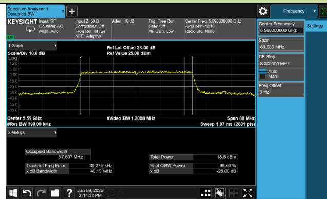
Channel 118 (5590MHz)
