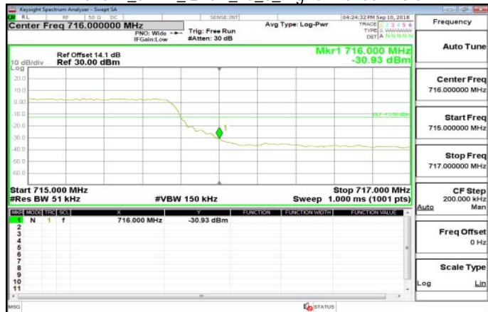
Band12_5MHz_QPSK_25_0_HighCH23155-713.5
