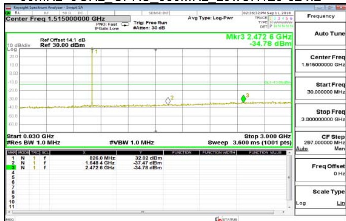
30MHz~3GHz_GPRS_850MHz_LowCH128-824.2
