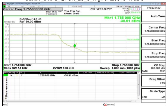
Band4_5MHz_QPSK_25_0_HighCH20375-1752.5
