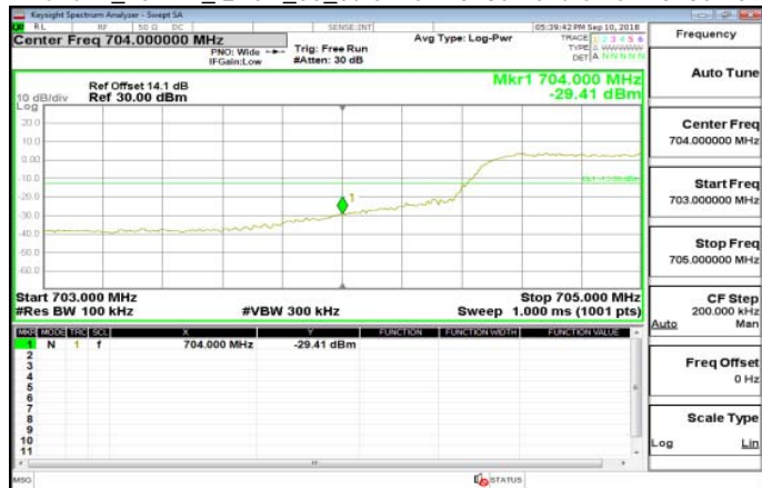
Band17_10MHz_QPSK_50_0\Low CH23780-709\LowCH23780-709
