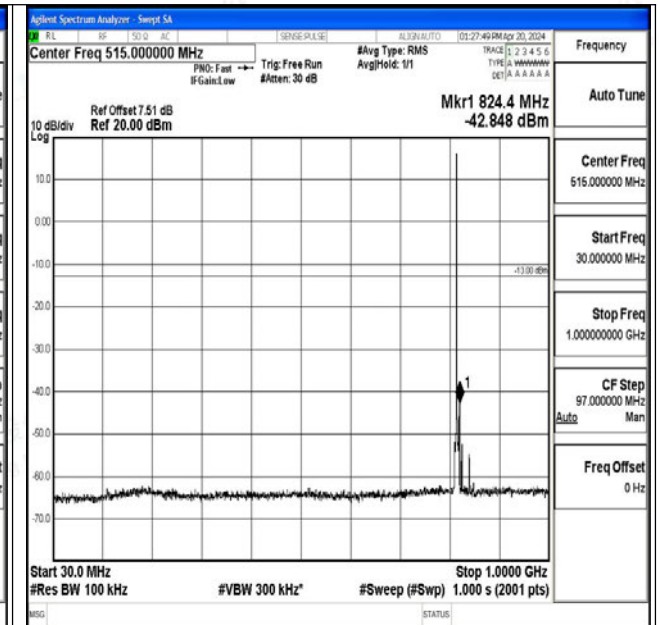
Band26_1.4MHz_16QAM_26740_1RB#0_30~1000_30~ 1000
