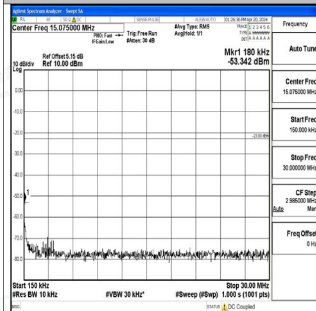
Band26_1.4MHz_16QAM_26697_1RB#0_0.15~30_0.15 ~30
