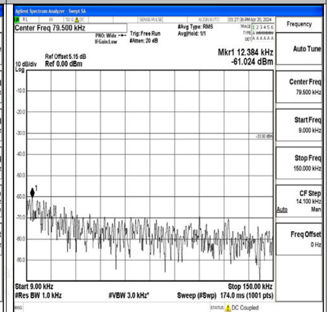
Band26_1.4MHz_16QAM_26740_1RB#0_0.009~0.15_0. 009~0.15
