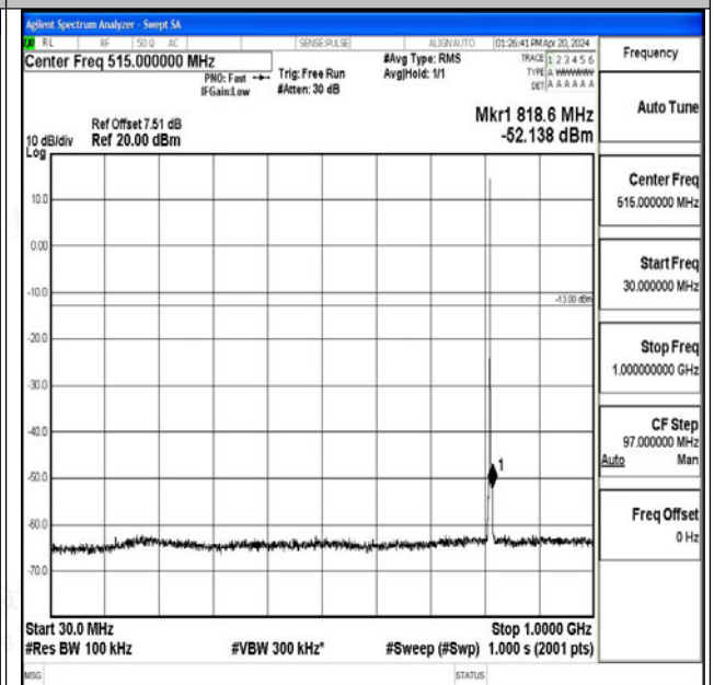
Band26_1.4MHz_16QAM_26697_1RB#0_30~1000_30~ 1000
