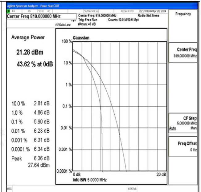
26(814-824)-5MHz-16QAM-26740-1RB#0-PASS
