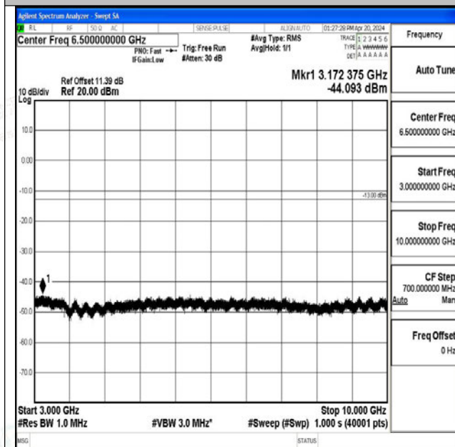
Band26_1.4MHz_QPSK_26740_1RB#0_3000~10000_30 00~10000
