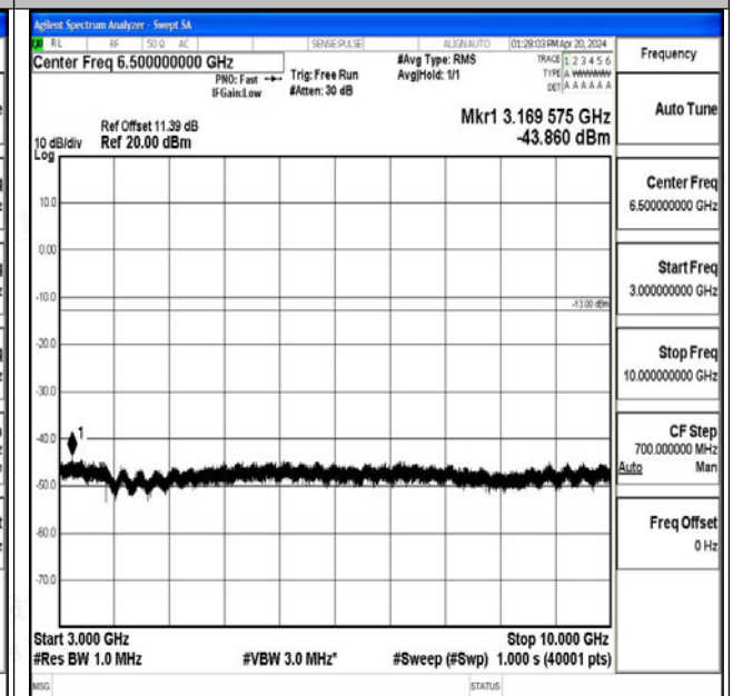
Band26_1.4MHz_16QAM_26740_1RB#0_3000~10000_ 3000~10000
