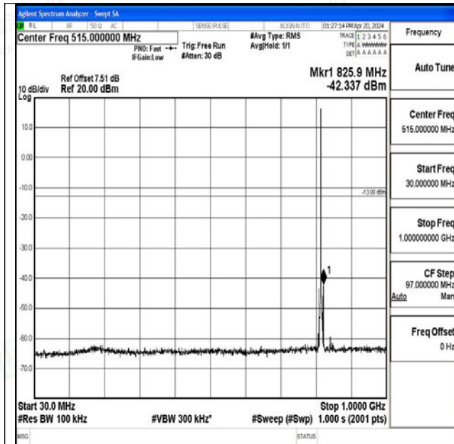
Band26_1.4MHz_QPSK_26740_1RB#0_30~1000_30~10 00
