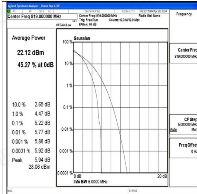
26(814-824)-5MHz-QPSK-26740-1RB#0-PASS
