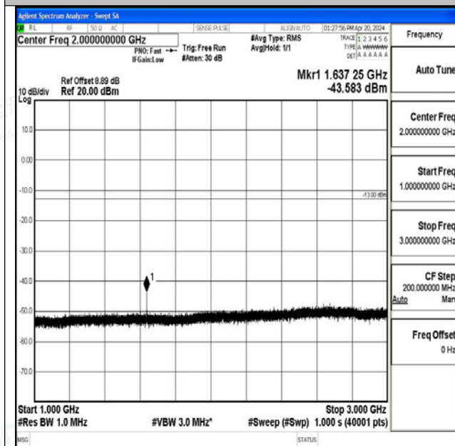
Band26_1.4MHz_16QAM_26740_1RB#0_1000~3000_1 000~3000
