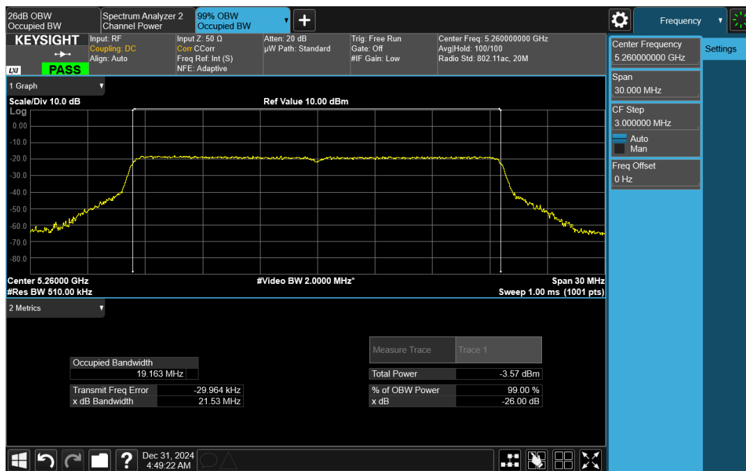
Wave-MLO5_UNII-2A_99_HE20_5260_CH0
