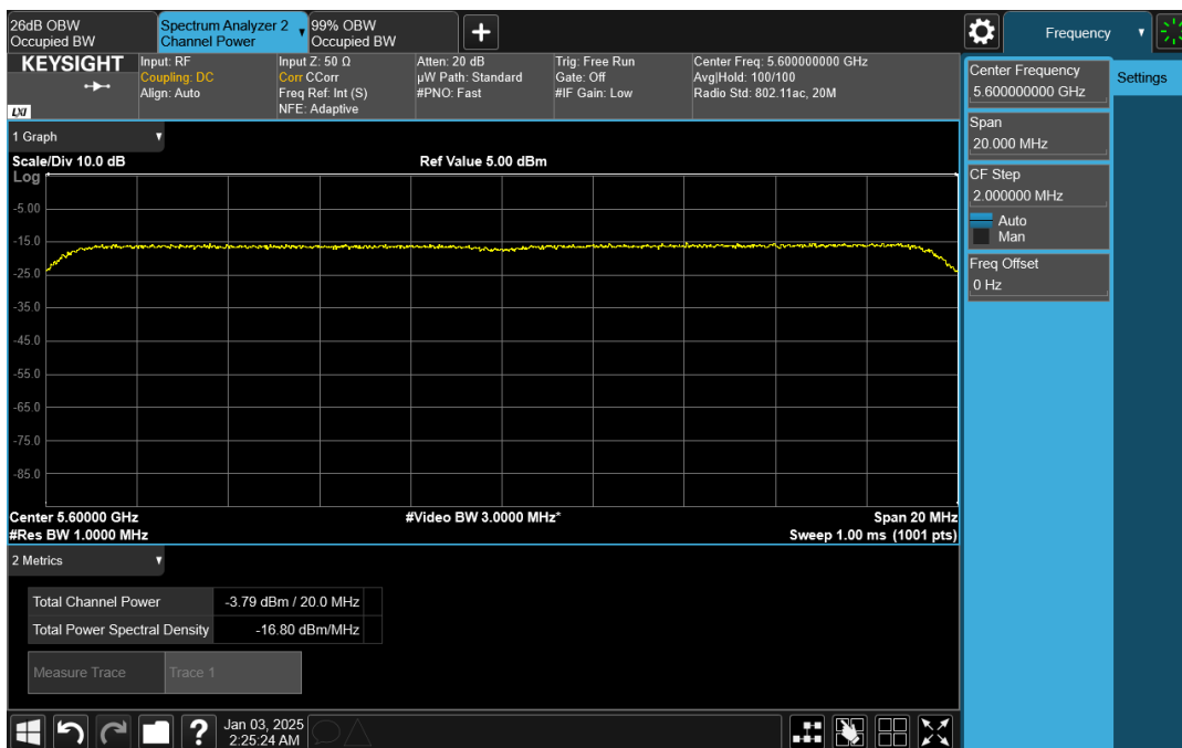
Wave-MLO5_UNII-2C_HE20_5600_CH0
