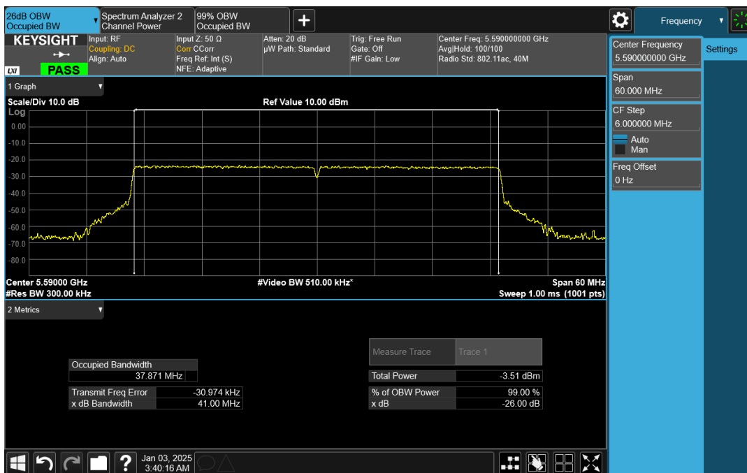
Wave-MLO5_UNII-2C_26dB_HE40_5590_CH1
