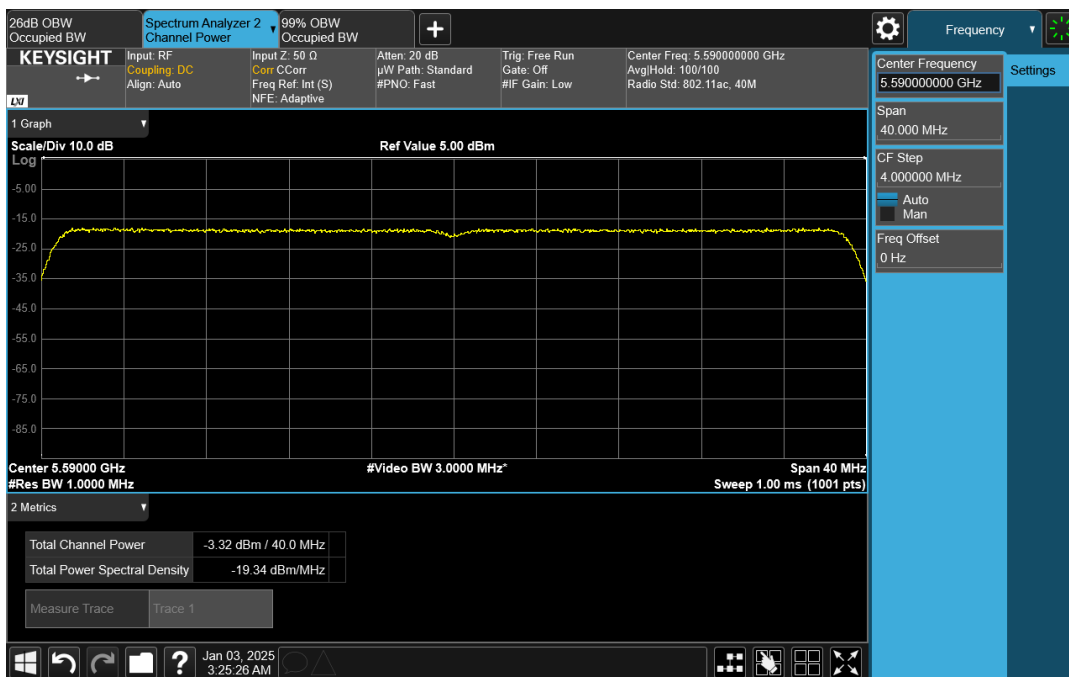
Wave-MLO5_UNII-2C_HE40_5590_CH0
