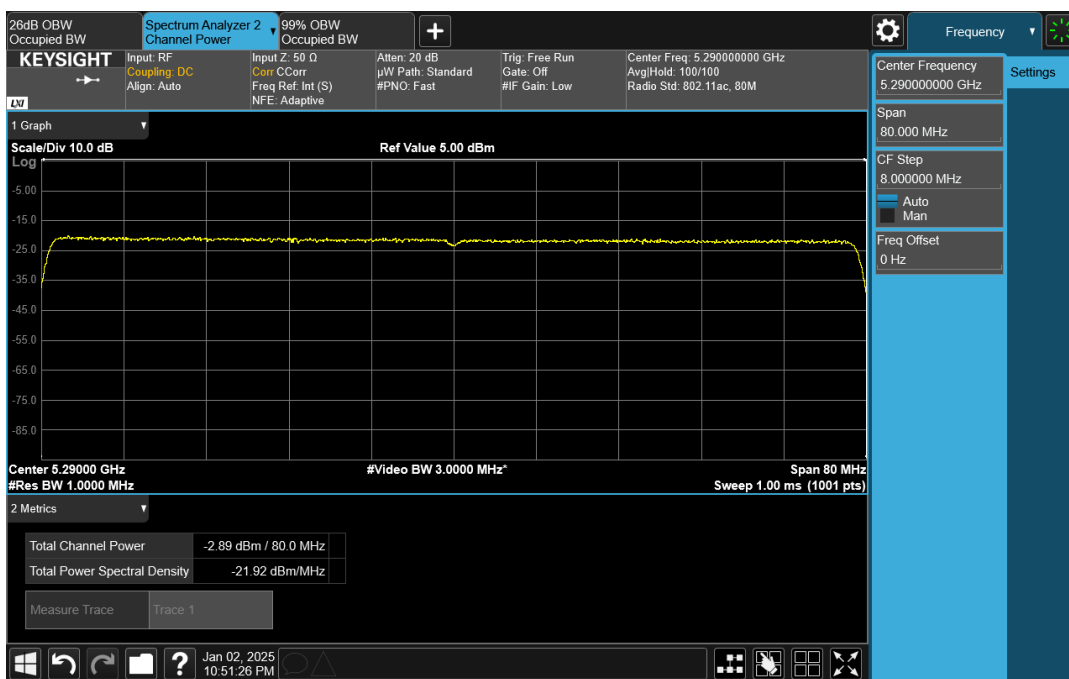
Wave-MLO5_UNII-2A_HE80_5290_CH1
