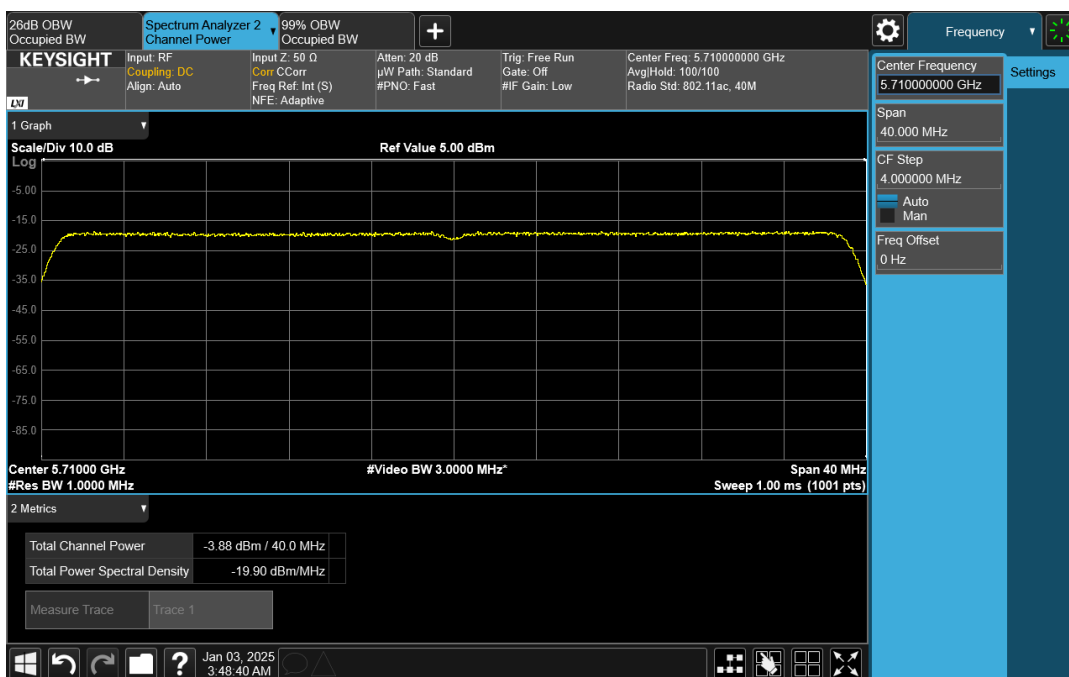
Wave-MLO5_UNII-2C_HE40_5710_CH1
