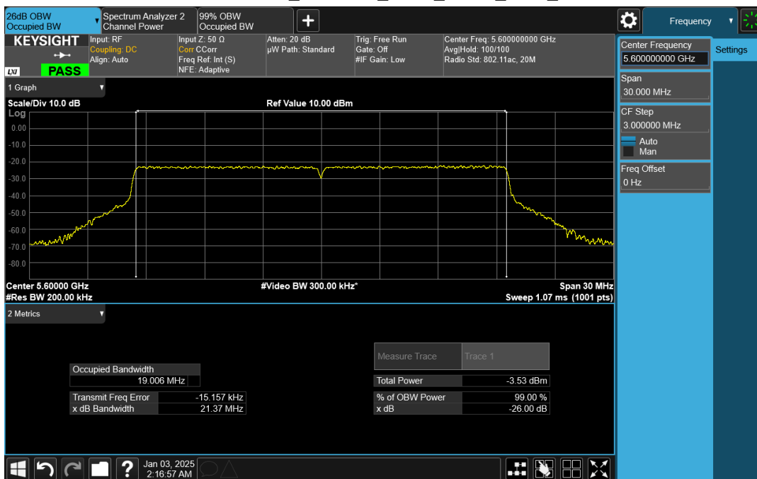
Wave-MLO5_UNII-2C_26dB_HE20_5600_CH0
