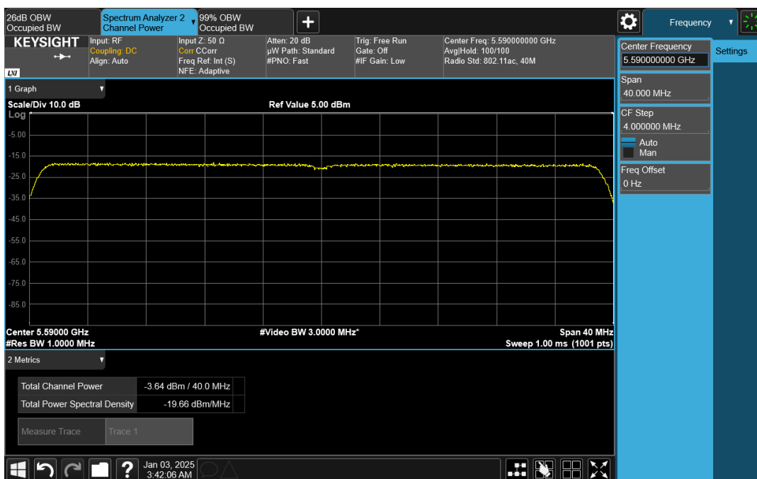
Wave-MLO5_UNII-2C_HE40_5590_CH1
