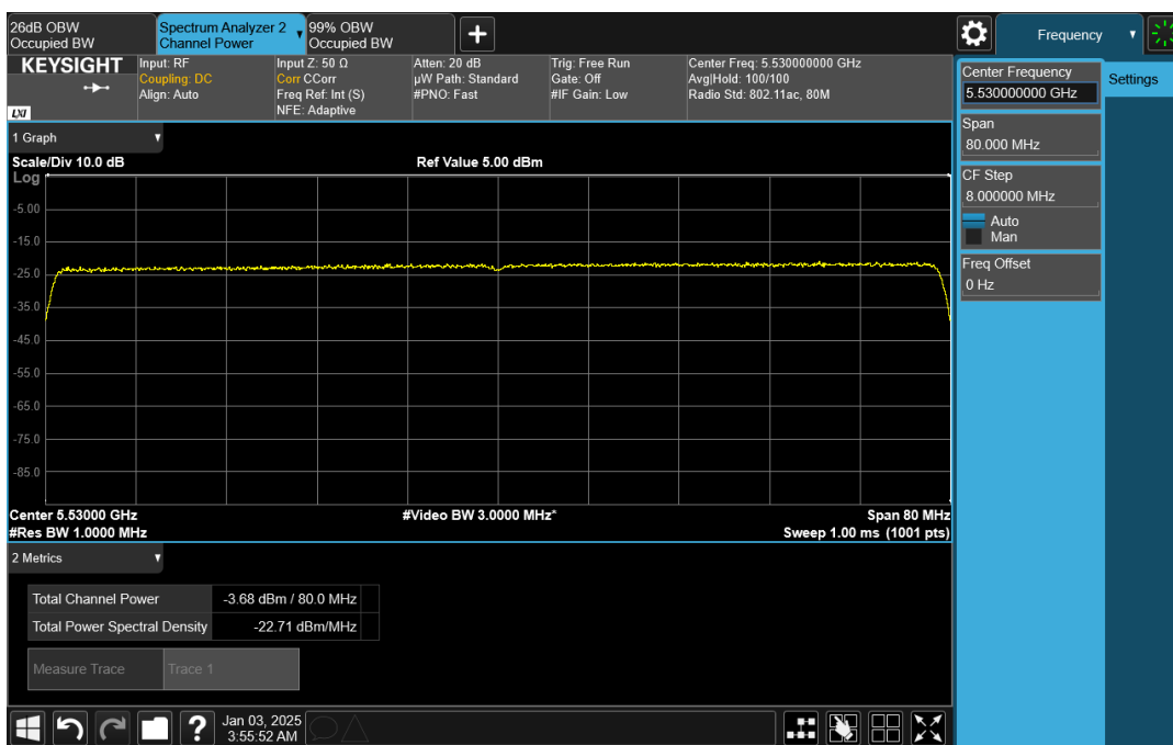
Wave-MLO5_UNII-2C_HE80_5530_CH1
