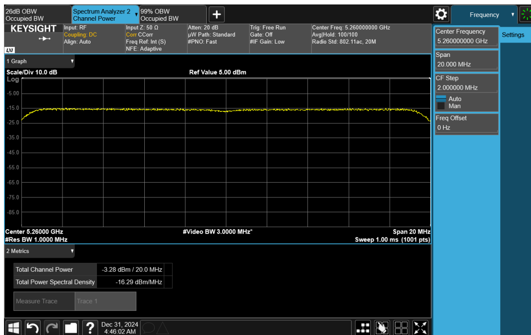
Wave-MLO5_UNII-2A_HE20_5260_CH0
