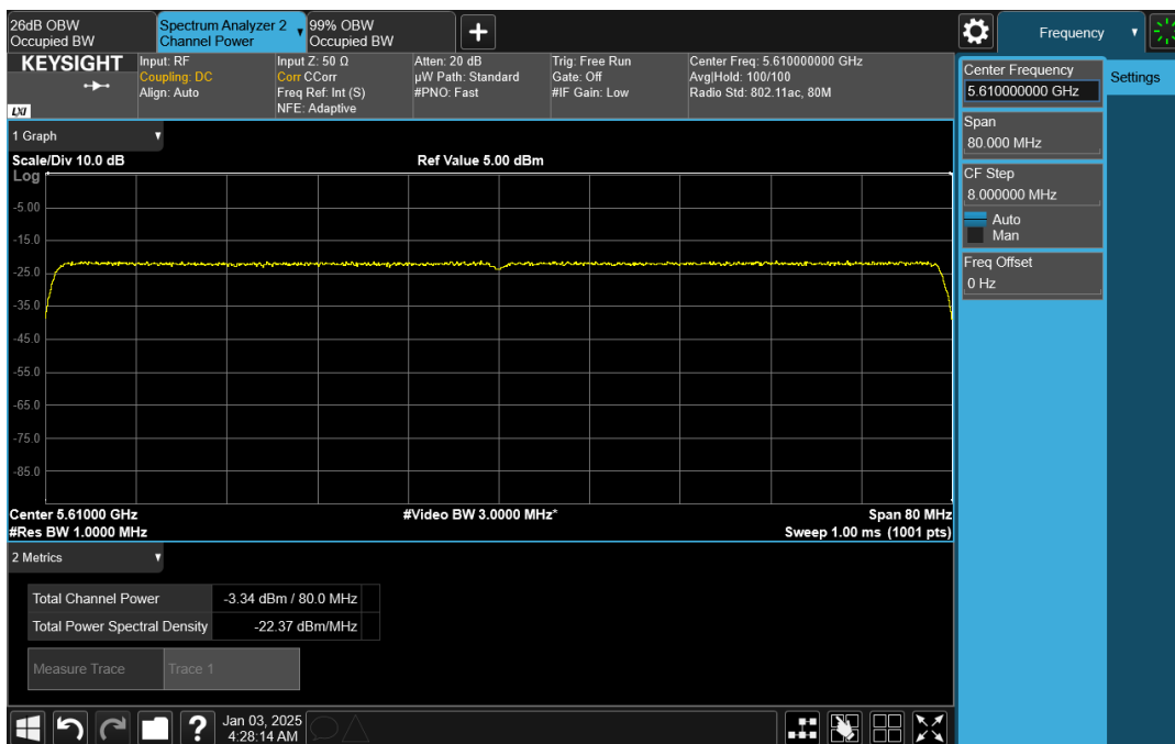
Wave-MLO5_UNII-2C_HE80_5610_CH0
