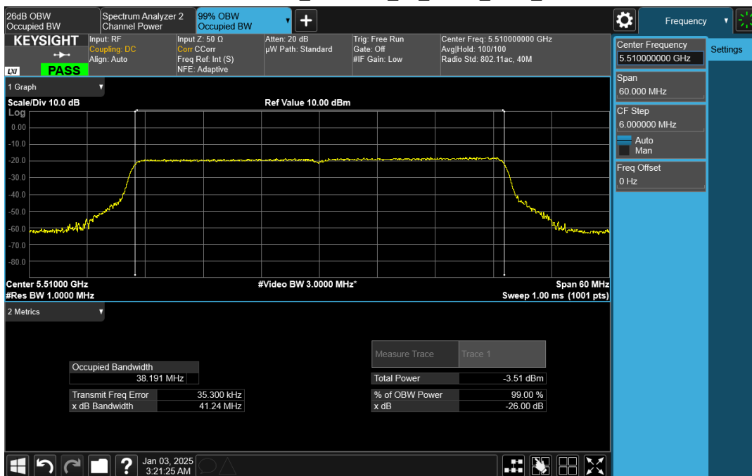
Wave-MLO5_UNII-2C_99_HE40_5510_CH0
