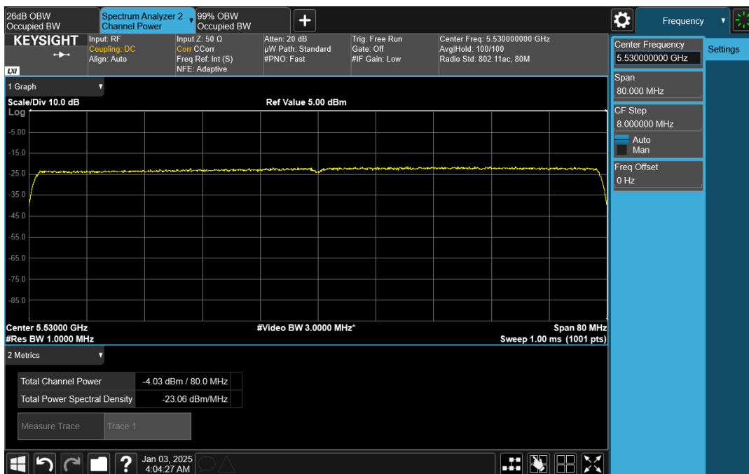
Wave-MLO5_UNII-2C_HE80_5530_CH0
