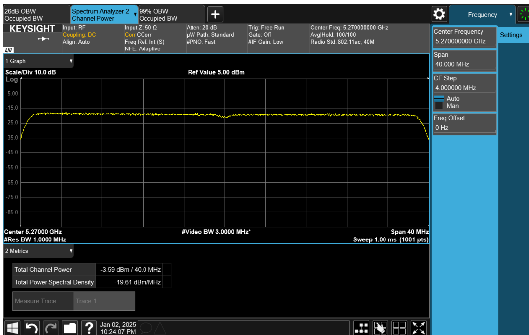
Wave-MLO5_UNII-2A_HE40_5270_CH0
