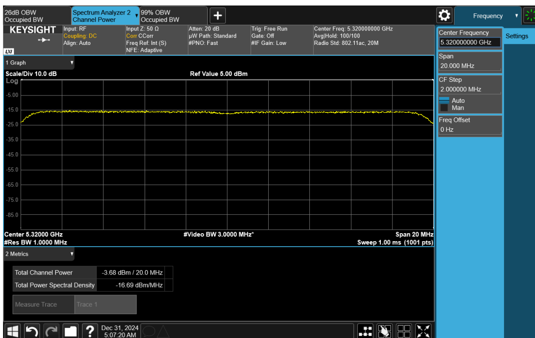
Wave-MLO5_UNII-2A_HE20_5320_CH1
