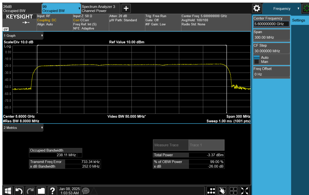
Wave-MLO5_UNII-2C_99_HE240_5600_CH0
