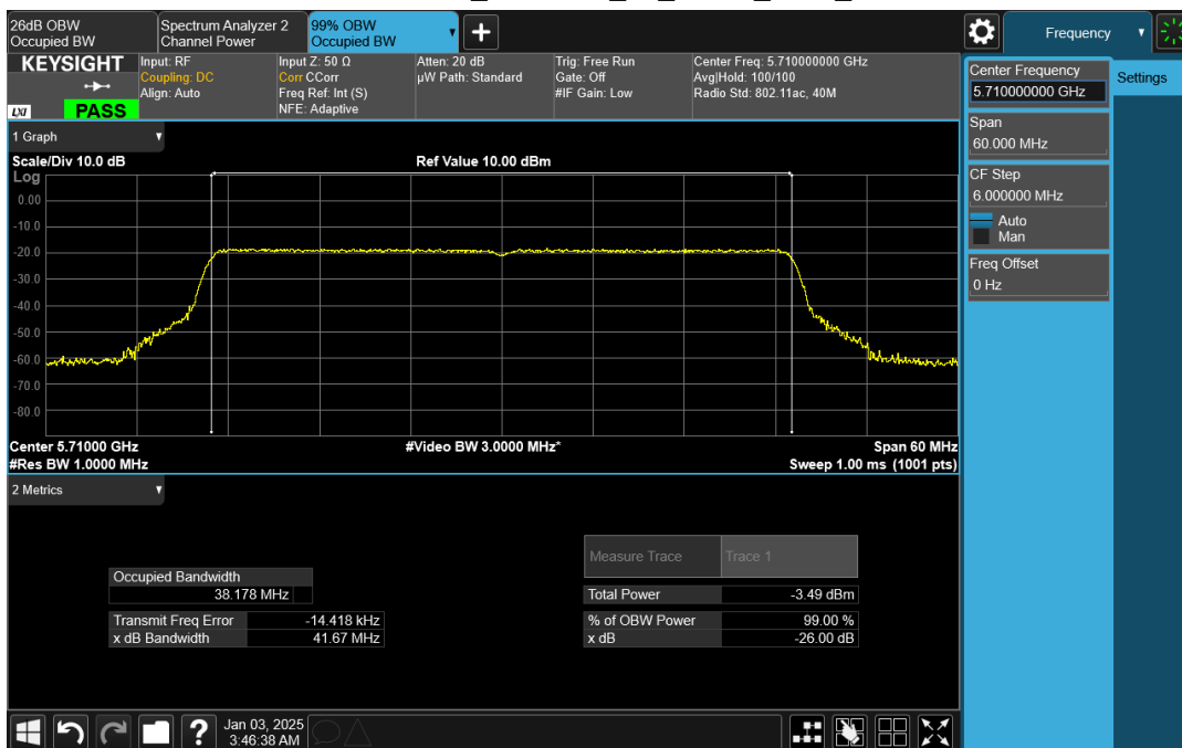
Wave-MLO5_UNII-2C_99_HE40_5710_CH1
