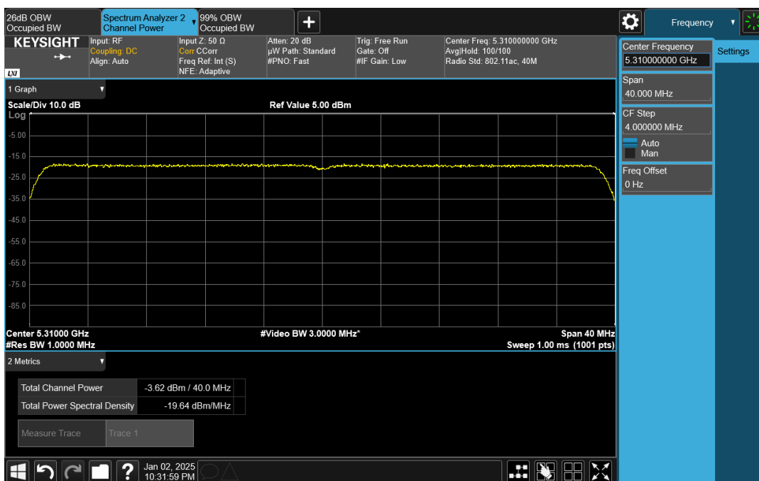
Wave-MLO5_UNII-2A_HE40_5310_CH1
