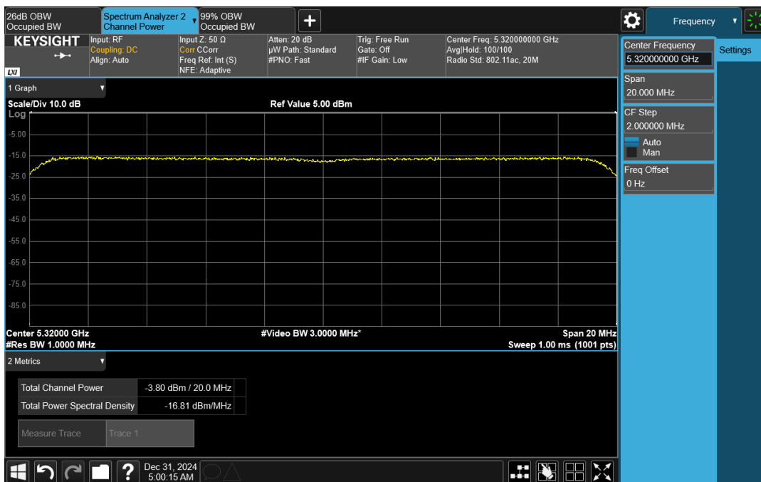
Wave-MLO5_UNII-2A_HE20_5320_CH0
