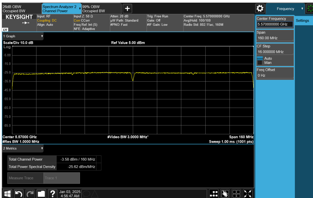
Wave-MLO5_UNII-2C_HE160_5570_CH0
