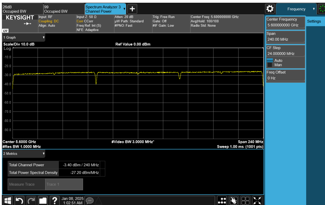
Wave-MLO5_UNII-2C_HE240_5600_CH0
