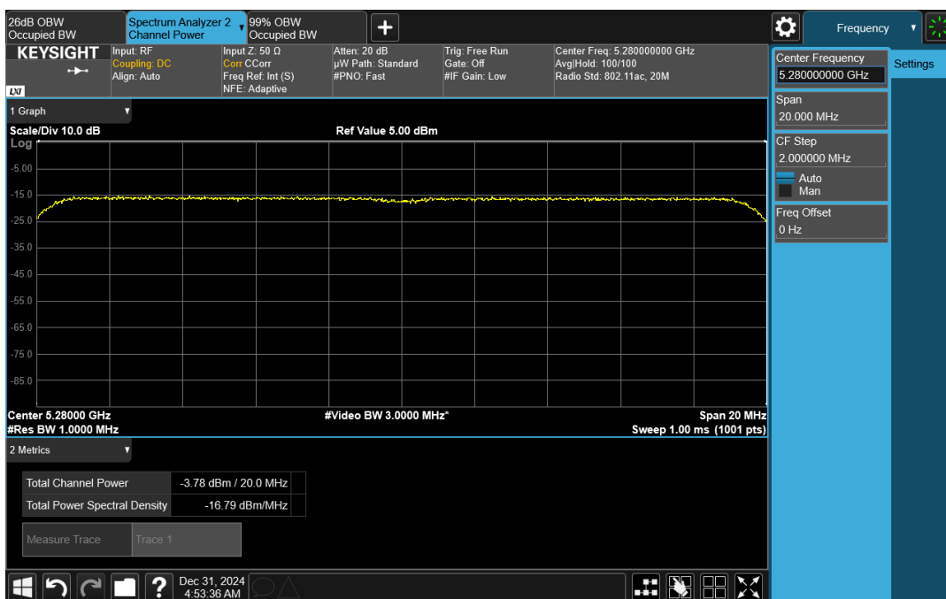
Wave-MLO5_UNII-2A_HE20_5280_CH1
