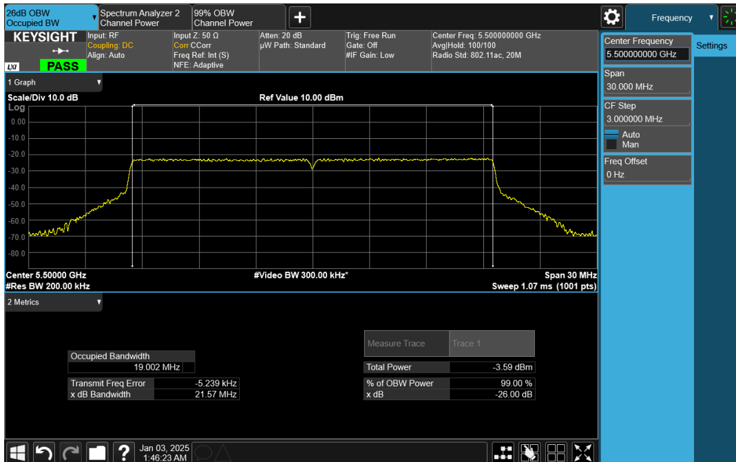
Wave-MLO5_UNII-2C_26dB_HE20_5500_CH1
