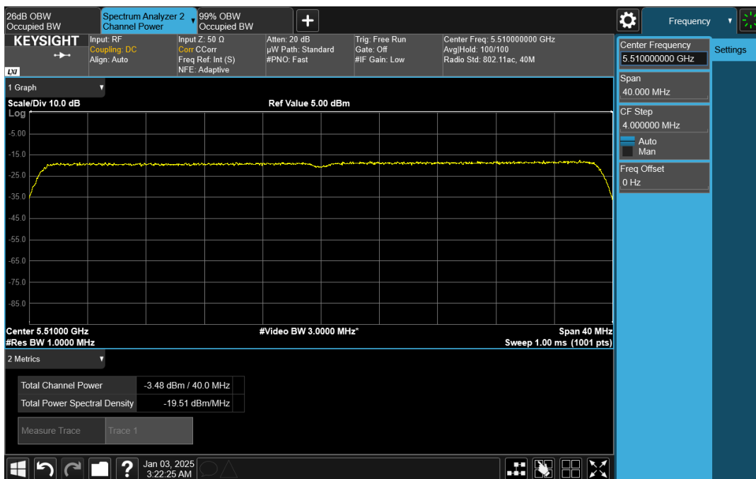
Wave-MLO5_UNII-2C_HE40_5510_CH0
