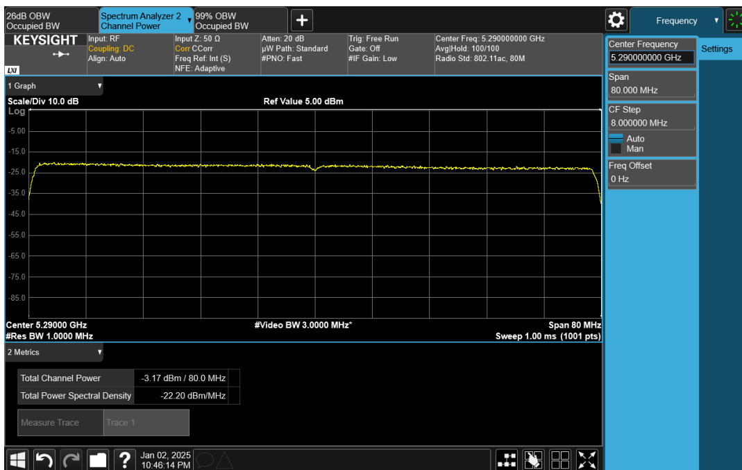
Wave-MLO5_UNII-2A_HE80_5290_CH0
