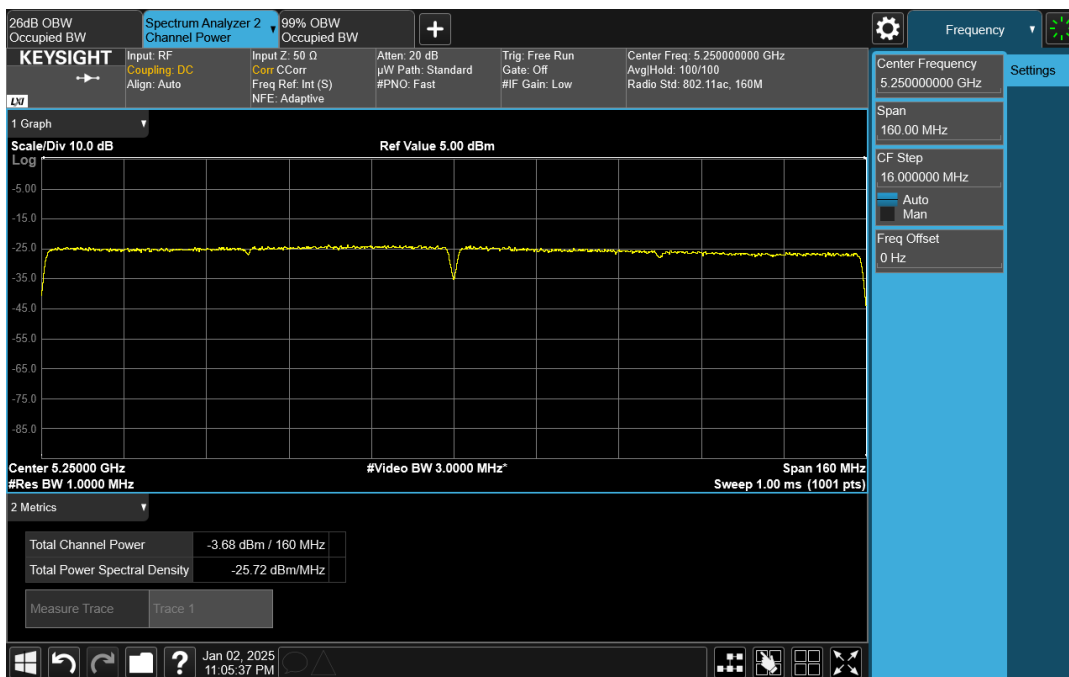
Wave-MLO5_UNII-2A_HE160_5250_CH0
