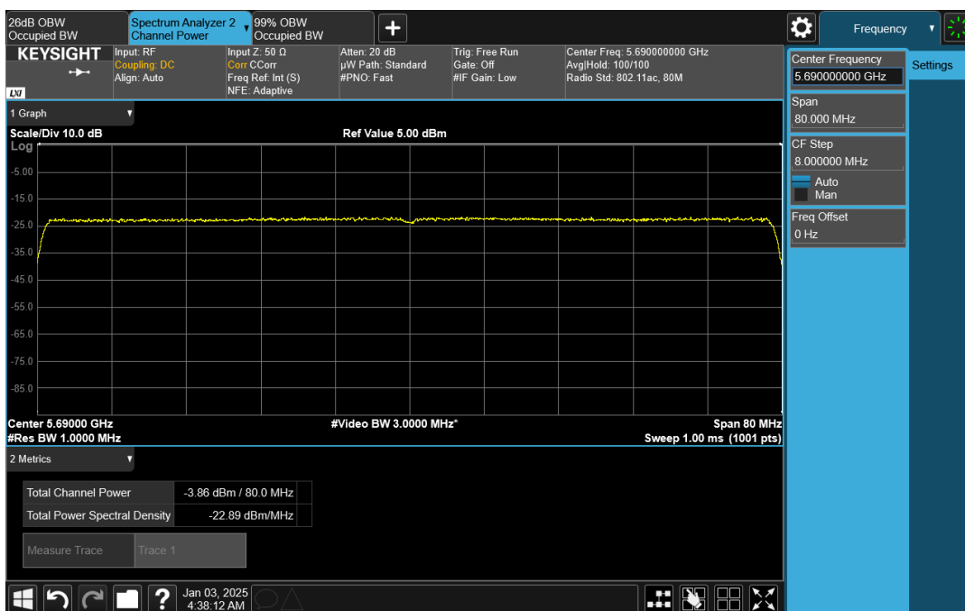
Wave-MLO5_UNII-2C_HE80_5690_CH1
