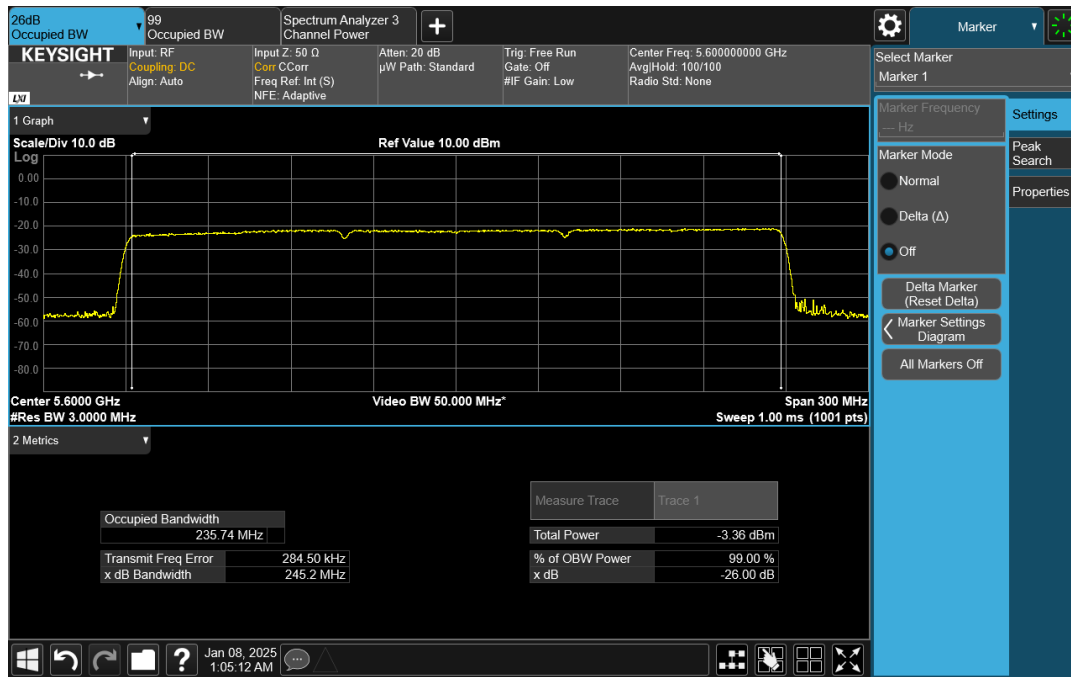
Wave-MLO5_UNII-2C_26dB_HE240_5600_CH0
