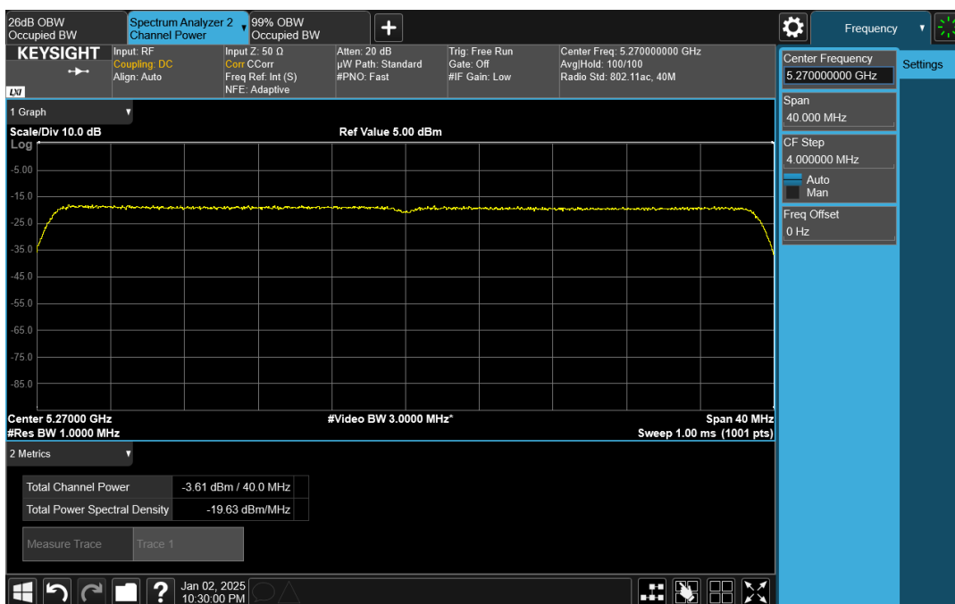
Wave-MLO5_UNII-2A_HE40_5270_CH1
