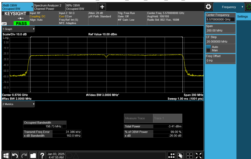
Wave-MLO5_UNII-2C_26dB_HE160_5570_CH1
