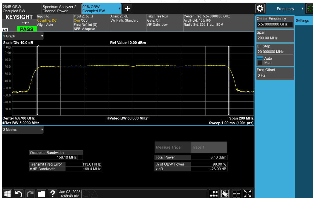
Wave-MLO5_UNII-2C_99_HE160_5570_CH1
