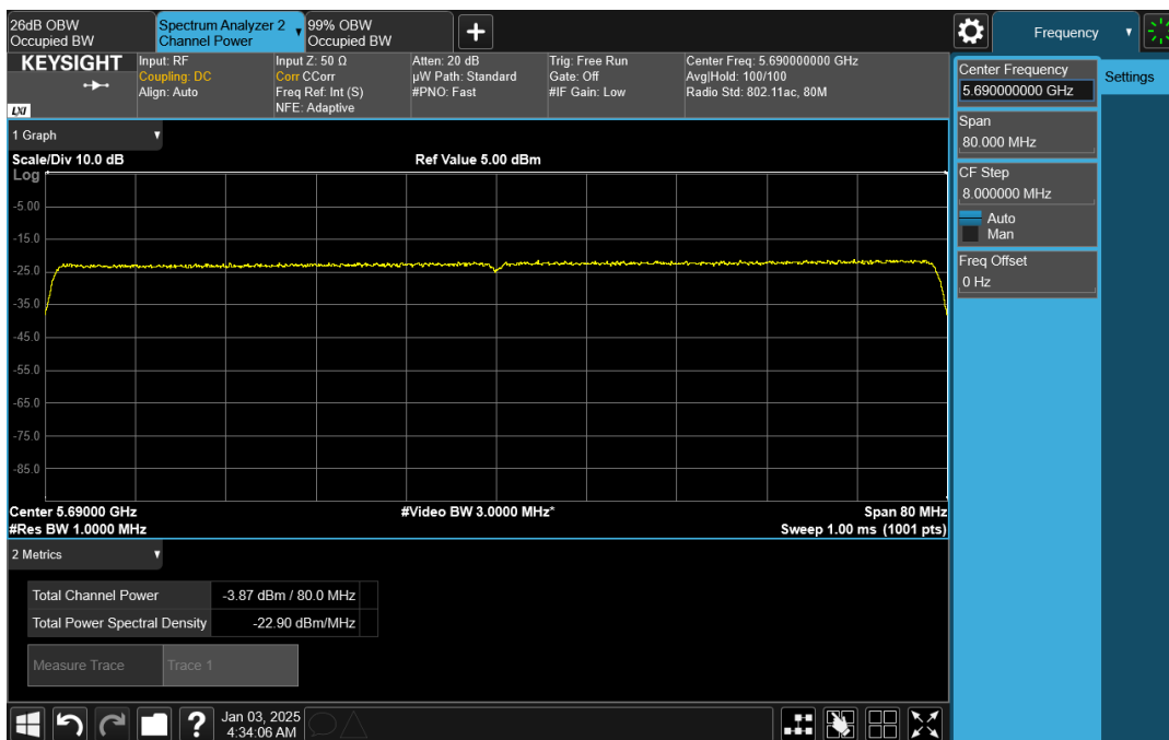
Wave-MLO5_UNII-2C_HE80_5690_CH0
