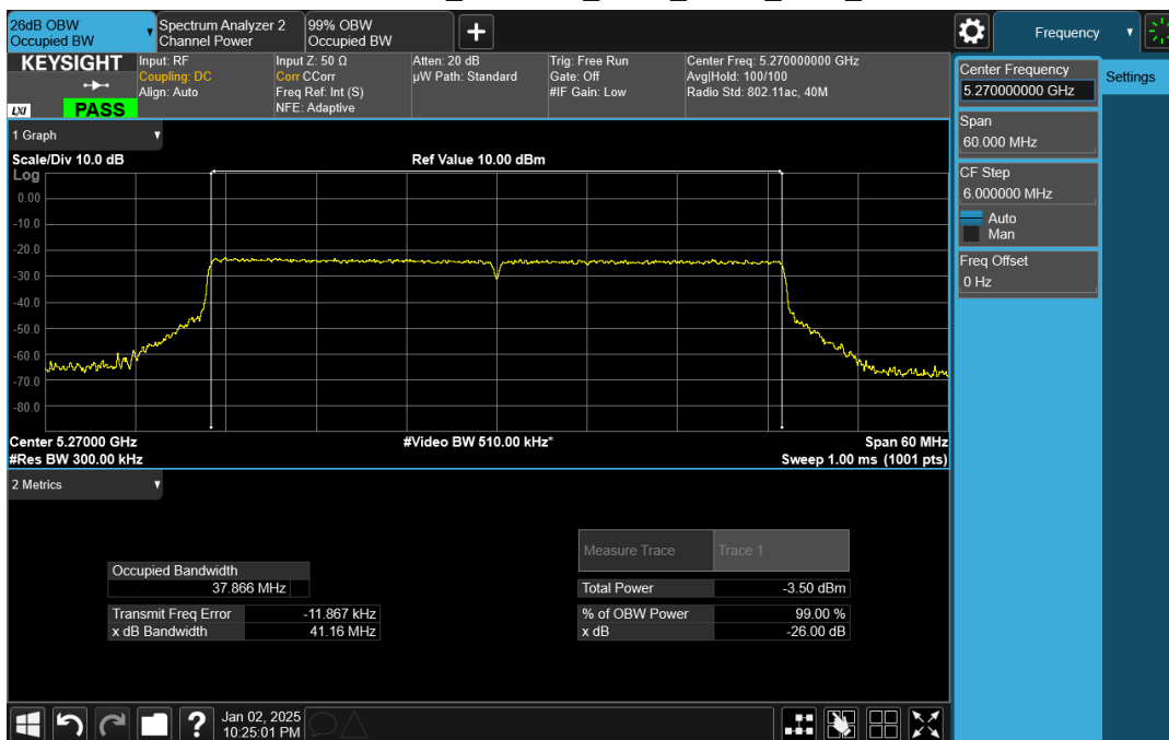
Wave-MLO5_UNII-2A_26dB_HE40_5270_CH0
