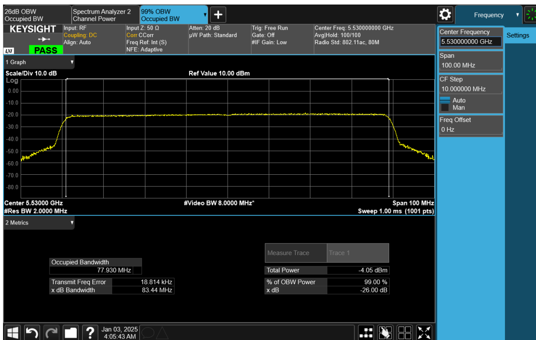
Wave-MLO5_UNII-2C_99_HE80_5530_CH0
