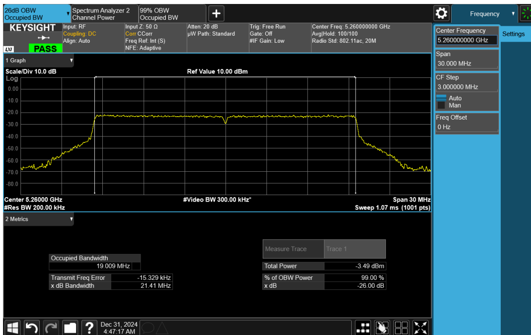
Wave-MLO5_UNII-2A_26dB_HE20_5260_CH0
