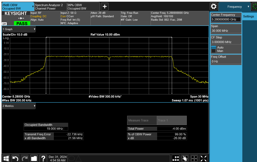
Wave-MLO5_UNII-2A_26dB_HE20_5280_CH1
