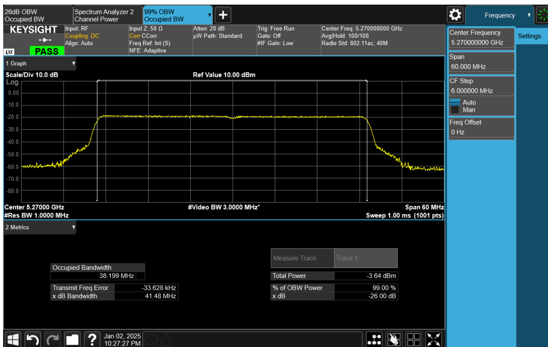
Wave-MLO5_UNII-2A_99_HE40_5270_CH1
