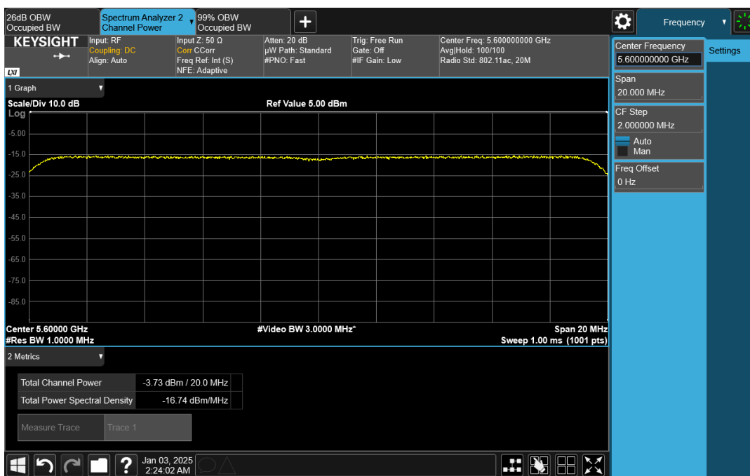
Wave-MLO5_UNII-2C_HE20_5600_CH1
