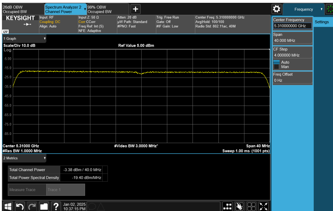
Wave-MLO5_UNII-2A_HE40_5310_CH0
