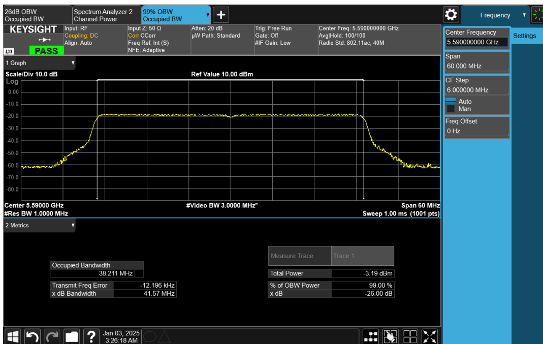
Wave-MLO5_UNII-2C_99_HE40_5590_CH0
