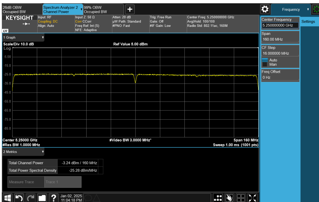
Wave-MLO5_UNII-2A_HE160_5250_CH1
