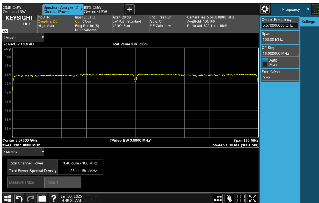
Wave-MLO5_UNII-2C_HE160_5570_CH1
