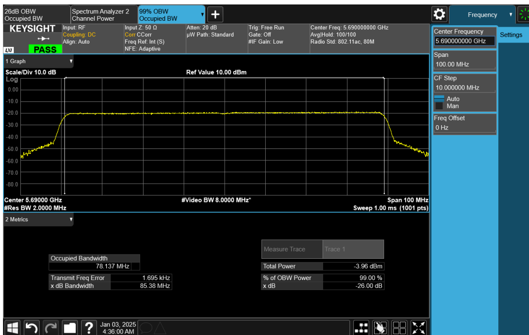
Wave-MLO5_UNII-2C_99_HE80_5690_CH0
