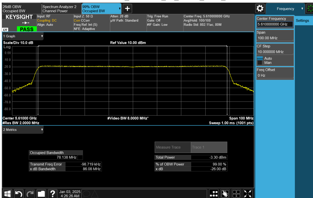
Wave-MLO5_UNII-2C_99_HE80_5610_CH1
