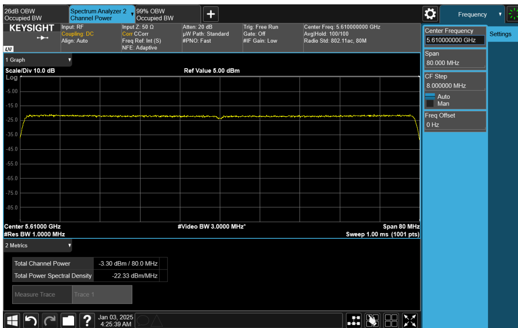
Wave-MLO5_UNII-2C_HE80_5610_CH1
