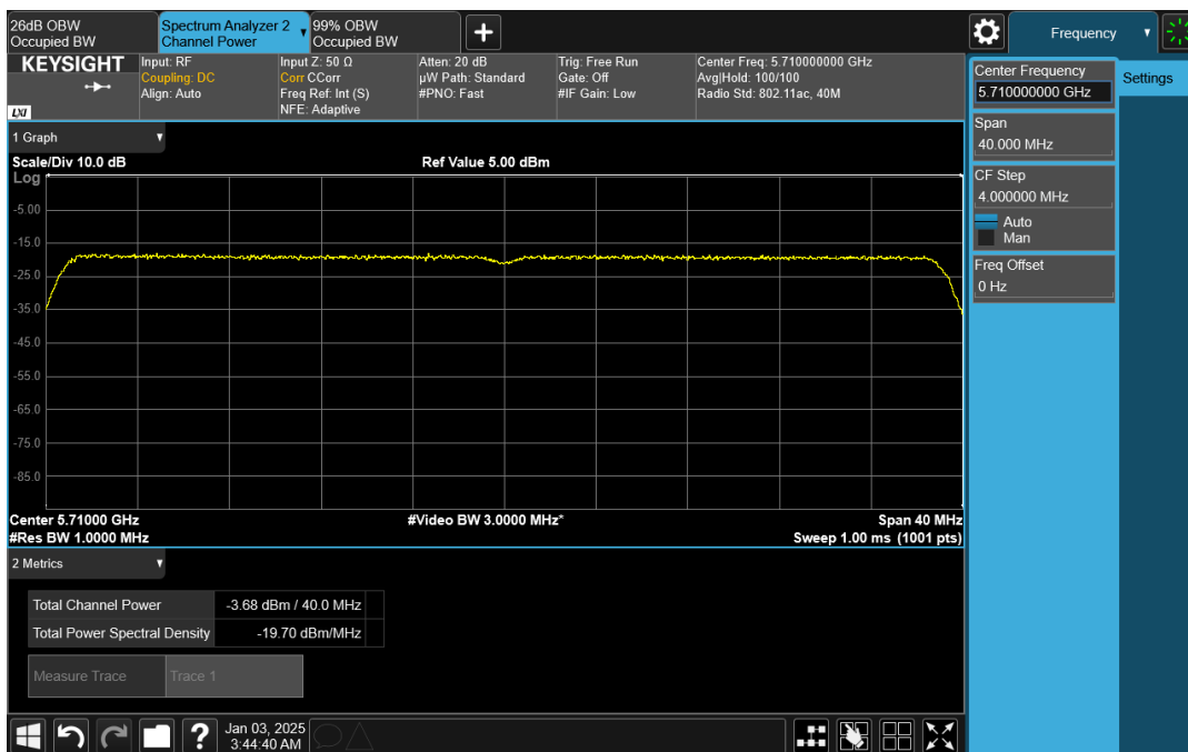
Wave-MLO5_UNII-2C_HE40_5710_CH0
