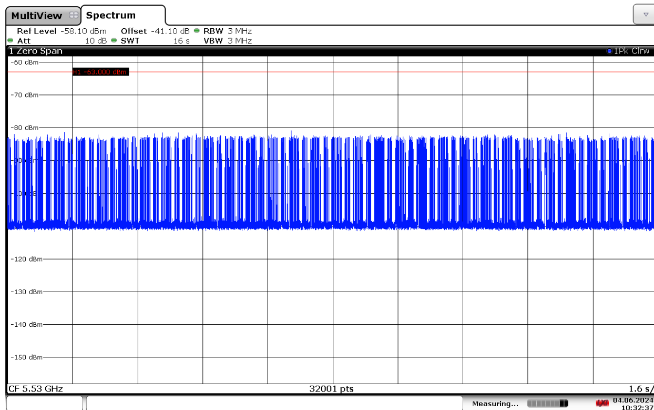
Figure 9-7. 5530MHz - Channel Loading - Mode 3 (80MHz)
