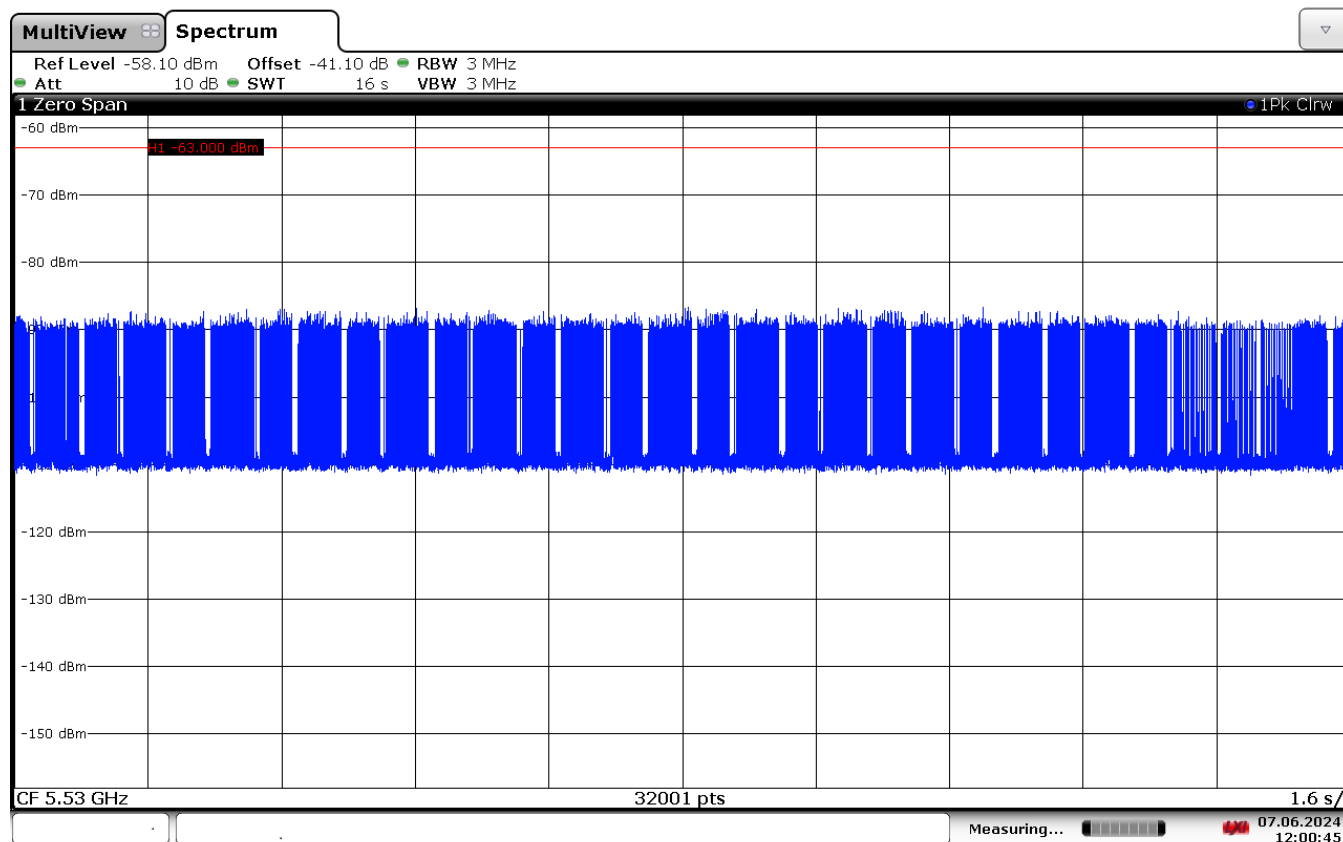
Figure 9-9. 5530 MHz - Channel Loading - Mode 4 (80MHz)
