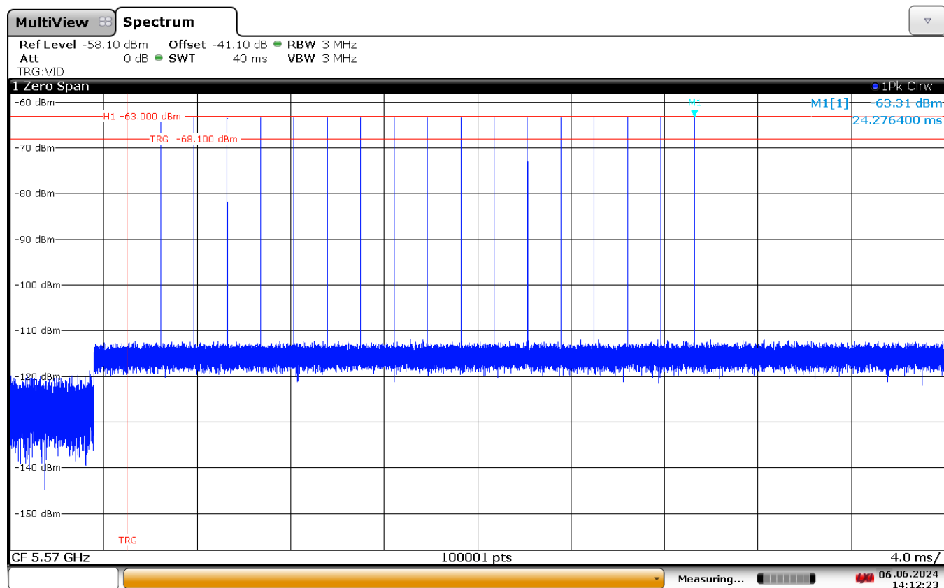
Figure 7-4. 5570MHz – Radar Pulse Type 0 (160MHz)
