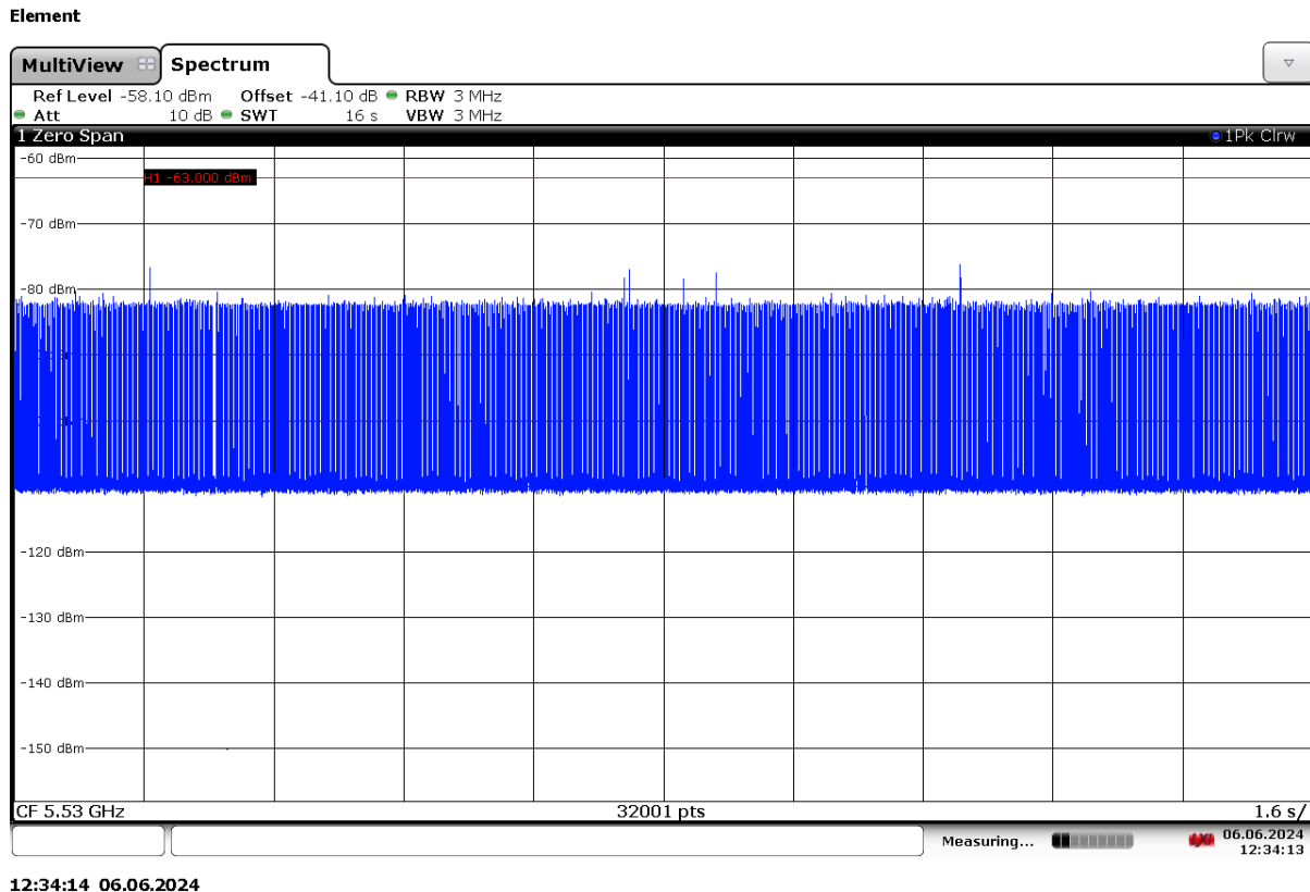
Figure 9-1. 5530MHz - Channel Loading - Mode 1 (80MHz)
