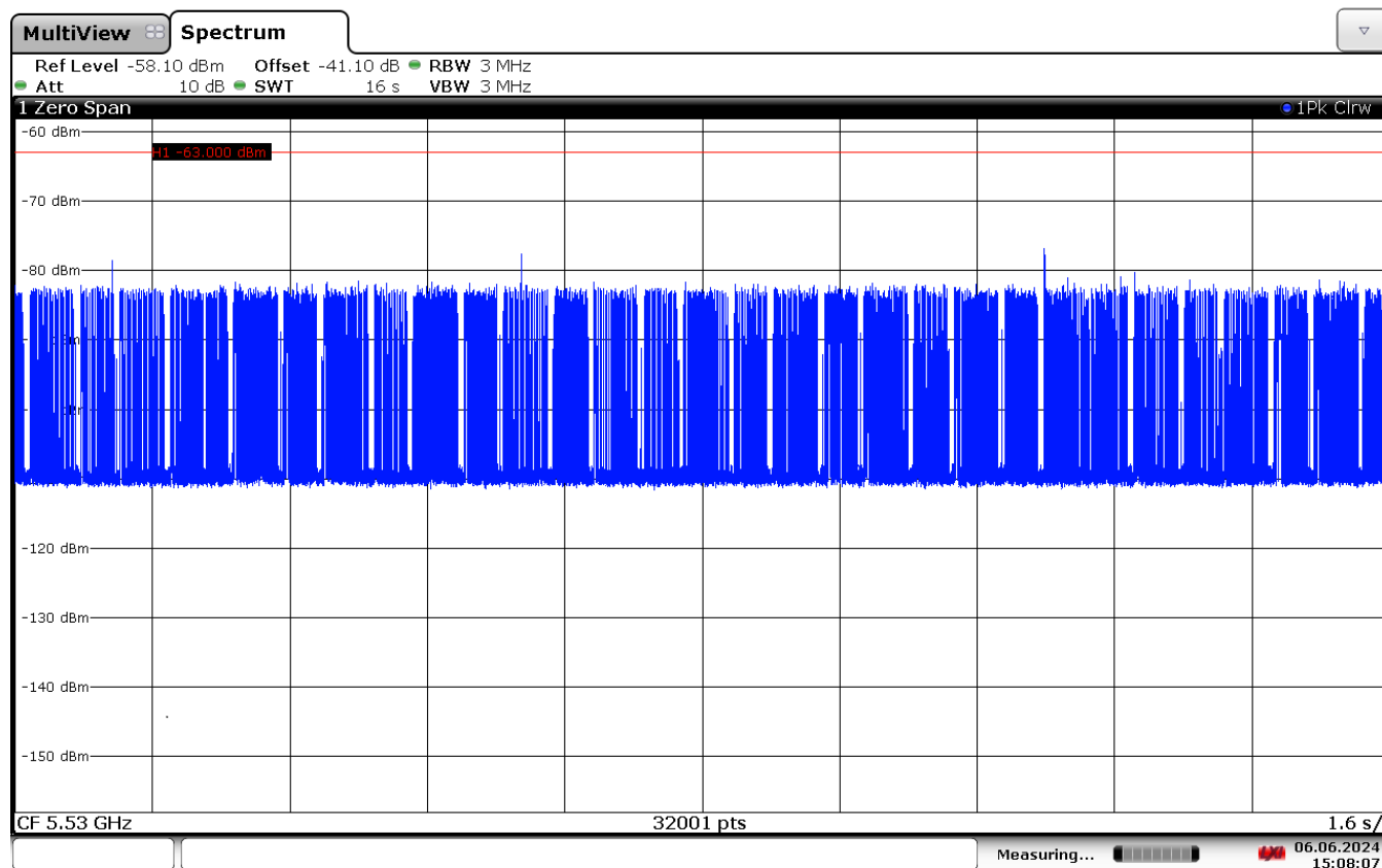
Figure 9-5. 5530MHz - Channel Loading - Mode 2 (80MHz)
