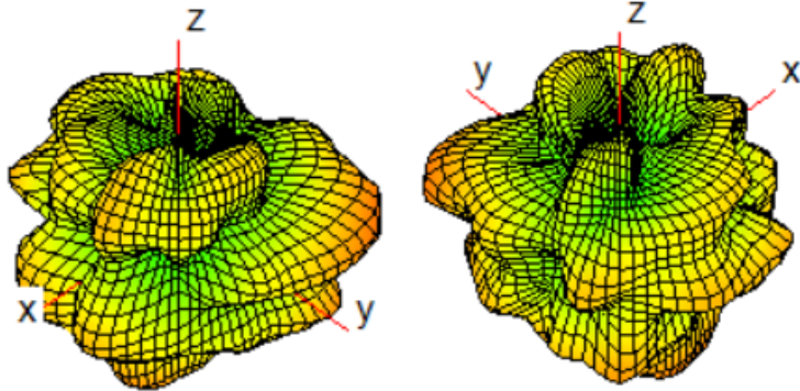
WiFi0_6525MHz
