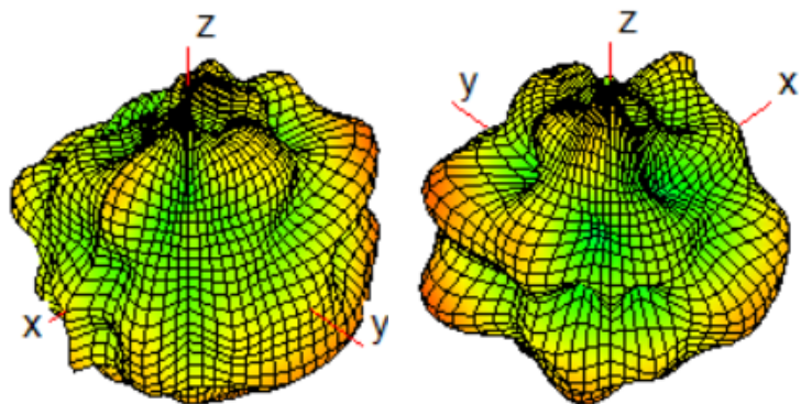
WiFi0_7125MHz
