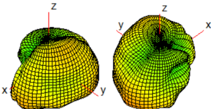
WiFi1_2442MHz
